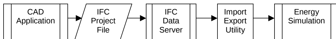
Figure 2. Flow of data from CAD through IFC to energy simulation.
