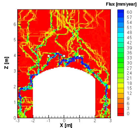
Figure 6. Flow through discrete fracture network and seepage into underground opening (after Finsterle, 2000b).
