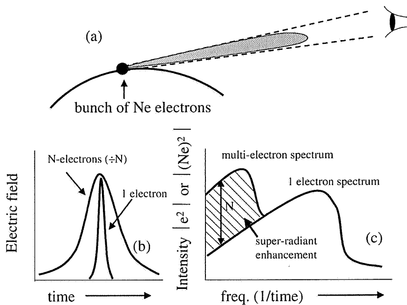
Figure 1. Schematic of the generation of light by relativistic electrons. In (a) the electric field is shown strongly collimated in the forward direction due to relativistic effects. For both one electron and a bunch of N electrons, an electric field is generated as a function of time (b), which yields a broad power spectrum as shown in (c).
