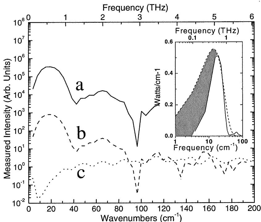
Figure 4. Intensities of light for (a) the JLab source scaled to 4.6 mA, (b) the actual measurement at 0.02 mA and (c) the 1400K thermal source. In the inset we show the measurement on an absolute scale, solid line, compared with the calculation, dashed line. The discrepancy shown by the hashed area is due to diffraction as described in the text.
