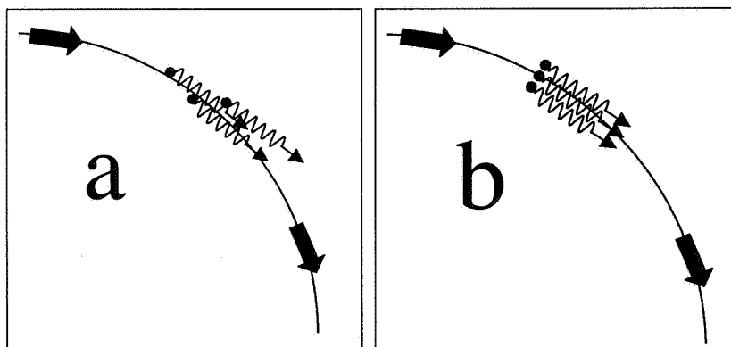
Figure 2. Illustration of the incoherent emission of electrons dispersed in space (a) and compared to the situation (b) in which they lie spatially within a wavelength (longitudinally) of the light being observed. In the latter case the electric fields add coherently and the intensity scales as the square of the number of electrons.
