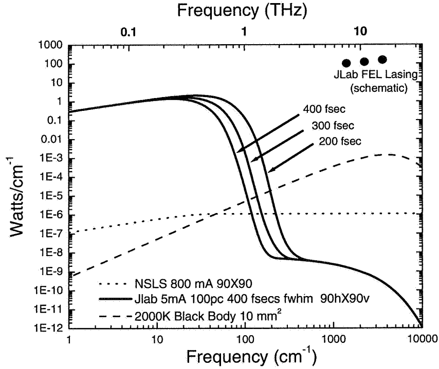
Figure 3. Calculations of the power emitted by 3 sources. For the Jlab source the calculations were performed for several full width half maximum values of bunch length given in fsecs to illustrate the dependence of the enhancement on this parameter.
