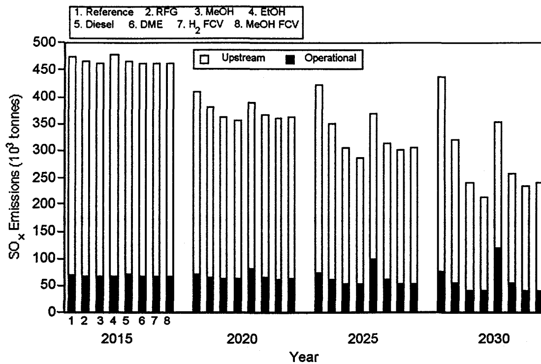
FIGURE 7 Total Fuel-Cycle SO x Emissions of Light-Duty-Vehicles
