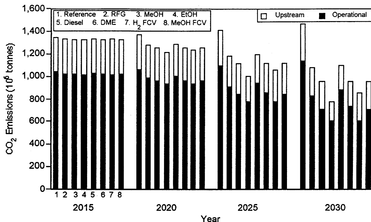
FIGURE 9 Total Fuel-Cycle CO 2 Emissions of Light-Duty-Vehicles
