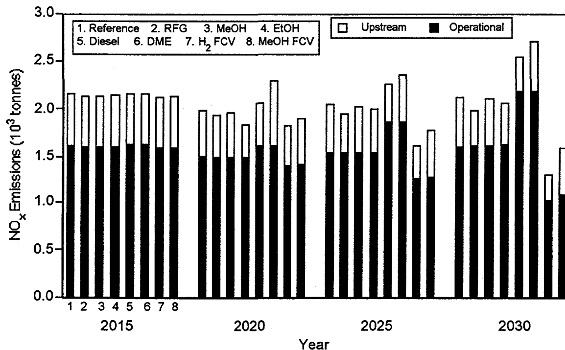
FIGURE 4 Total Fuel-Cycle NO_x Emissions of Light-Duty Vehicles
