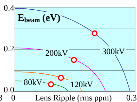
Fig.3. Allowed E_{\text{beam}} at \sigma(I)/I for a 0.5Å information limit at four accelerating voltages. Balanced E_{\text{beam}} points are marked.
