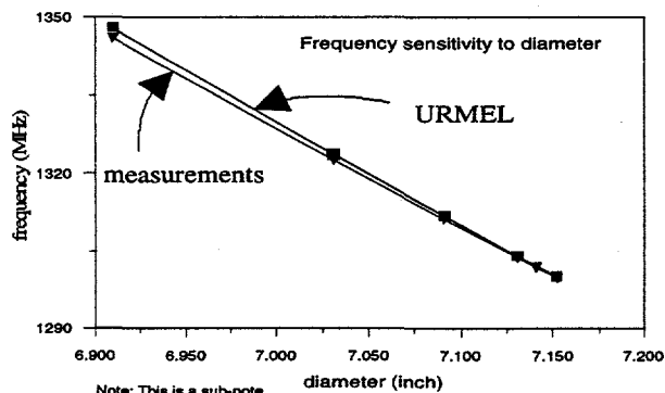
Figure 3: The resonant frequency of the witness gun as a function of the diameter, 2b .
