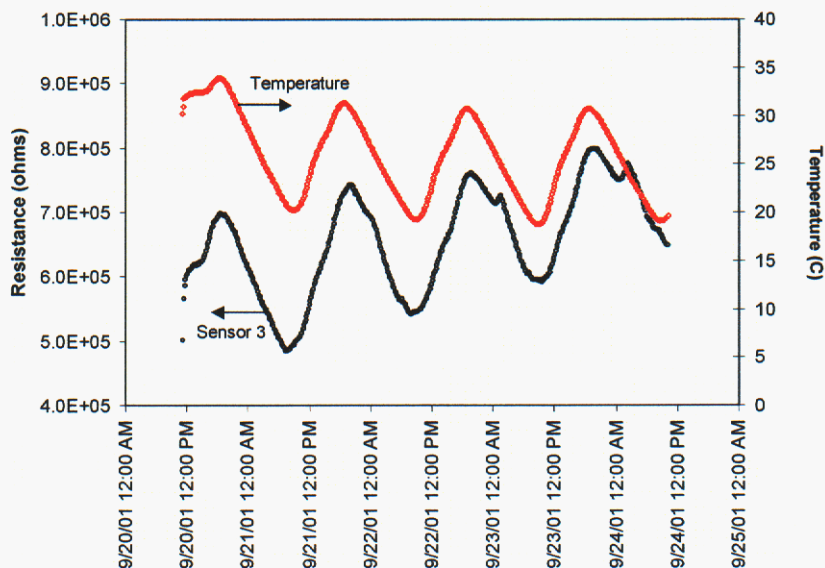
Figure 19. Plot of chemiresistor temperature and resistance during the four-day ambient data-logging period.
