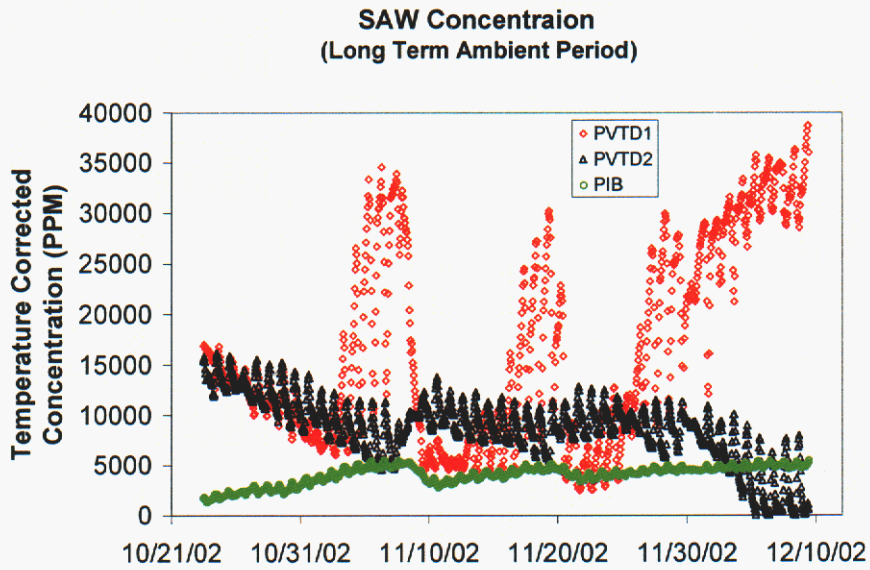
Figure 36. Measured TCE vapor concentration from the SAW sensor array during the long-term ambient monitoring period.
