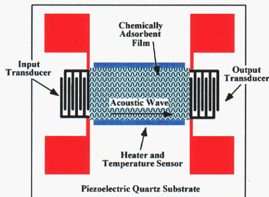
Figure 4. Schematic of SAW device.
