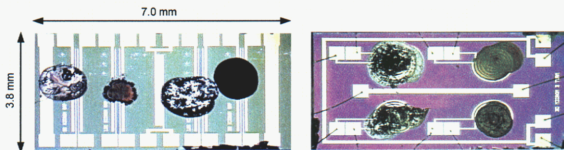
Figure 2. Chemiresistor arrays developed at Sandia with four conductive polymer films (black spots) deposited onto a microfabricated circuit. Left: Linear-electrode design (C4) with a temperature sensor in the middle and heating elements on the ends. Right: New spiral-electrode design (E2) with temperature sensor on the perimeter and heating element in the middle.
