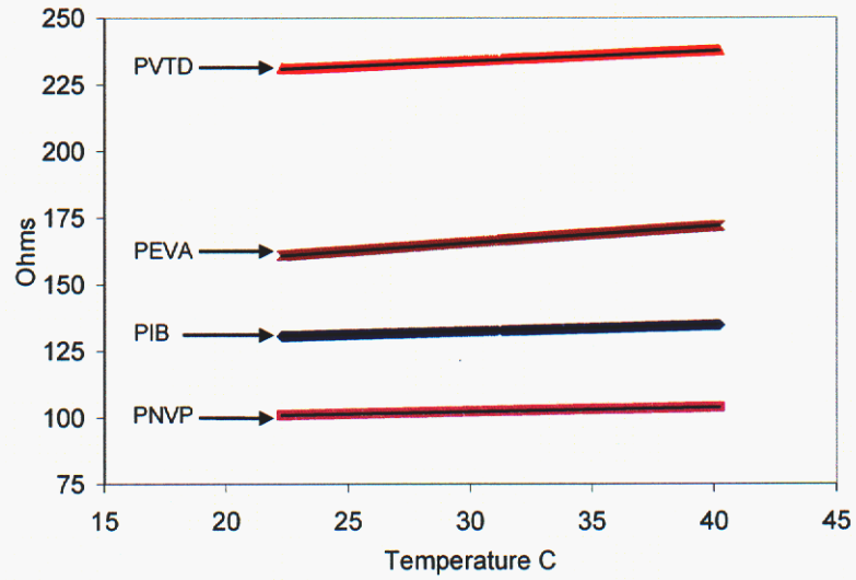
Figure 39. Temperature dependence of chemiresistor E19.
