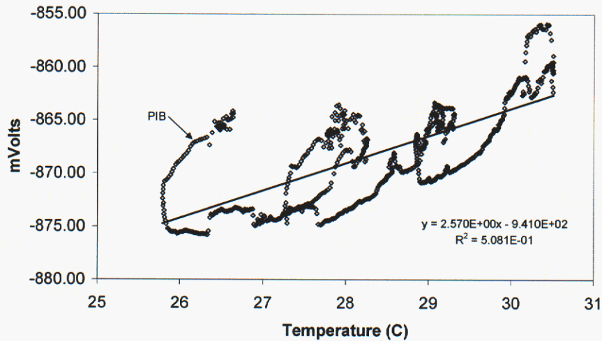
Figure 32. SAW PIB response as a function of temperature
