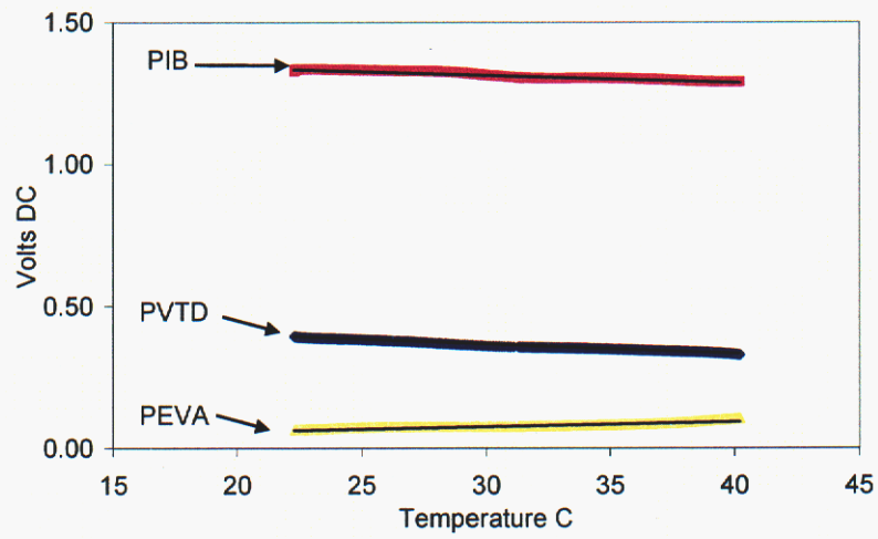
Figure 40. Temperature dependence of SAW UNK
