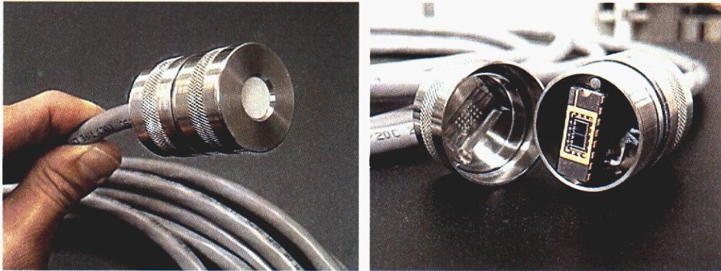
Figure 3. Stainless-steel waterproof package that houses the chemiresistor array. Left: GORE-TEX® membrane covers a small window over the chemiresistors. Right: Disassembled package exposing the 16-pin dual-in-line package and chemiresistor chip.
