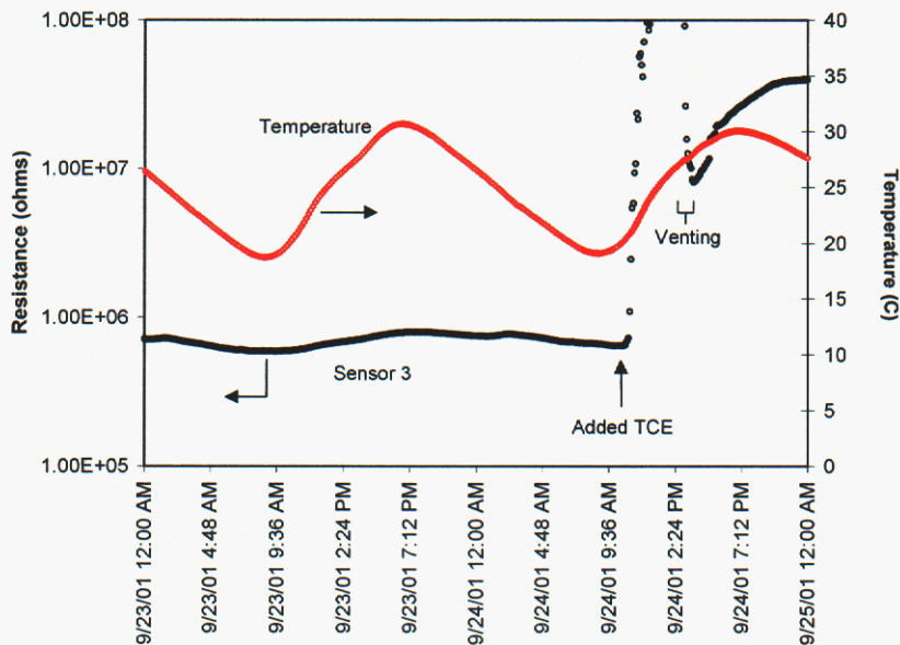
Figure 20. Plot of chemiresistor temperature and resistance during TCE emplacement and ventilation periods. Note that the resistances are clipped at 100\text{ M}\Omega , which is the maximum readout of the data logger.
