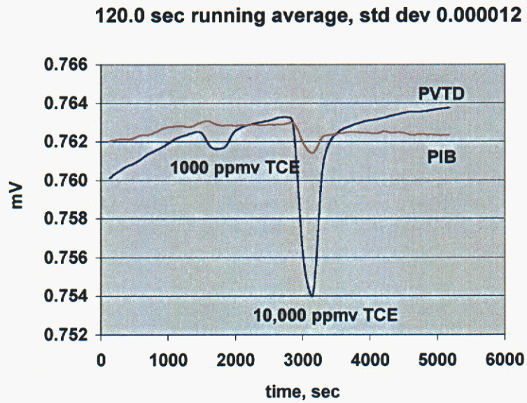
Figure 12. Data of Figure 11 processed as a 120-second running average.
