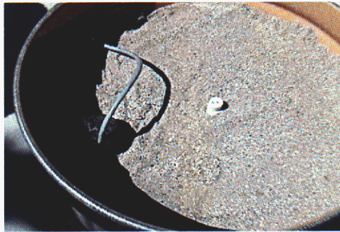
Figure 17. Top view of 55-gallon drum filled with sand. The contaminant reservoir is in the middle of the drum, and the sensor well (with sensor cable) is towards the outside.
