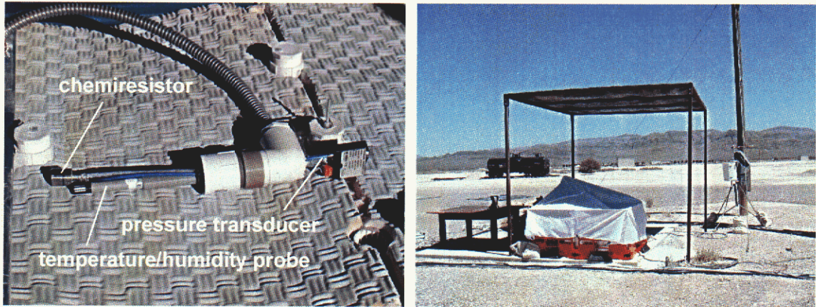
Figure 23. Left: Sensors emplaced in the sandbox. Right: Sandbox shaded from sun.
