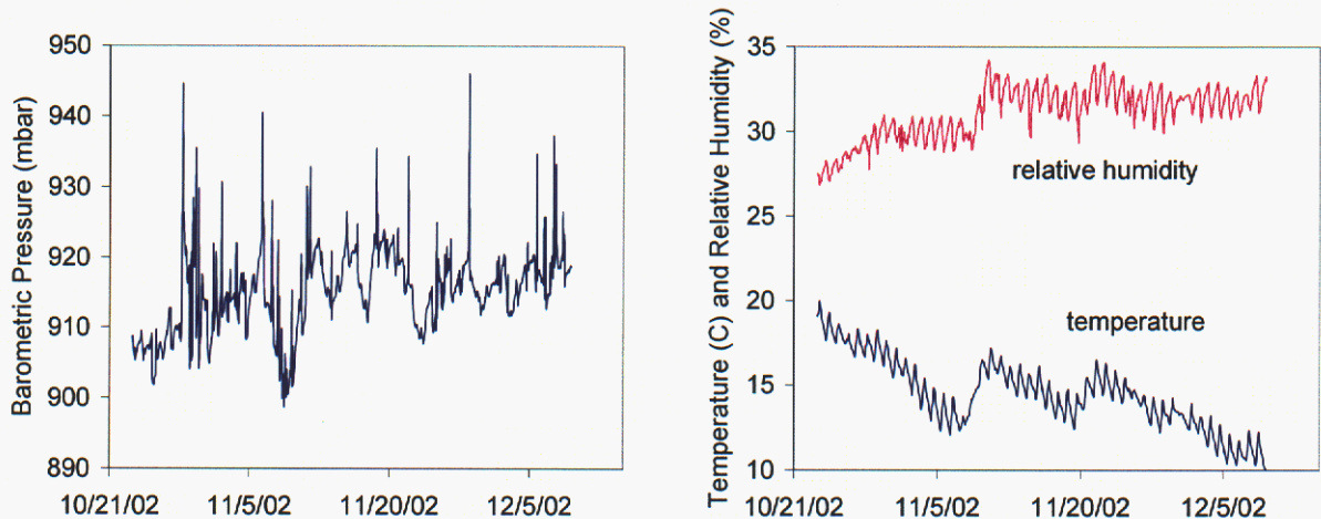
Figure 37. Environmental variable fluctuations during the long-term ambient monitoring period (October-December, 2002).
