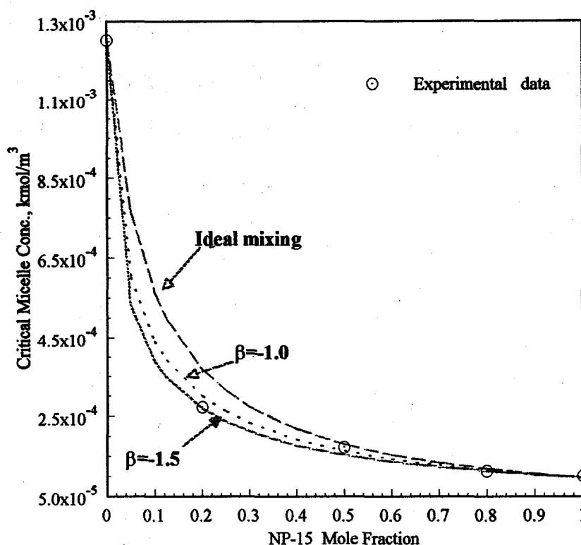
Figure 15 Regular solution and ideal mixing theory for determining the interaction parameter for the tetradecyl trimethylammoniumchloride (TTAC) pentadecylethoxylated nonyl phenol (NP-15) system.
