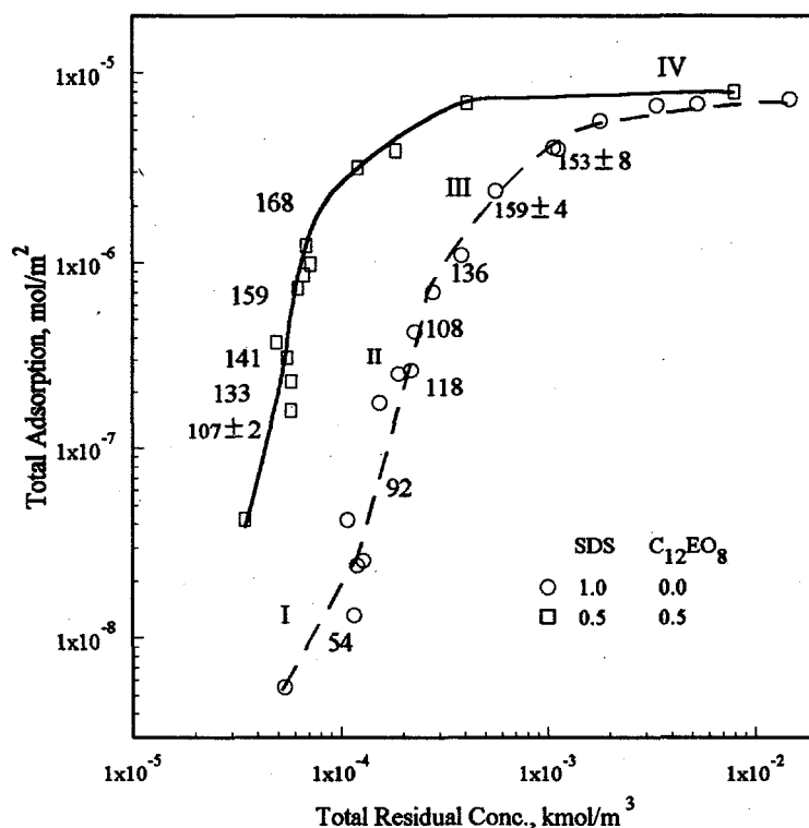
Figure 28 Total adsorption of sodium dodecyl sulfate (SDS) and 1:1 SDS/ C_{12}EO_8 mixtures on alumina and aggregation numbers of surfactant.
