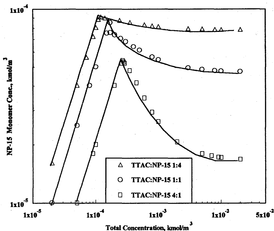
Figure 17 Monomer concentrations of pentadecylethoxylated nonyl phenol (NP-15) in mixtures with tetradecyl trimethylammonium chloride (TTAC) calculated using regular solution theory with an interaction parameter = -1.5.
