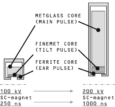
Fig. 7: IBX induction cells will use different core materials to produce the required pulse waveforms shown in figure 6. For longer ion beam pulse lengths and higher gap voltages more core material is needed. This figure demonstrates the impact on size when going from a 250 ns / 100 kV cell to a 1000 ns / 200 kV cell. At the same time the core weight would increase from \sim 200 kg to \sim 4500 kg.
