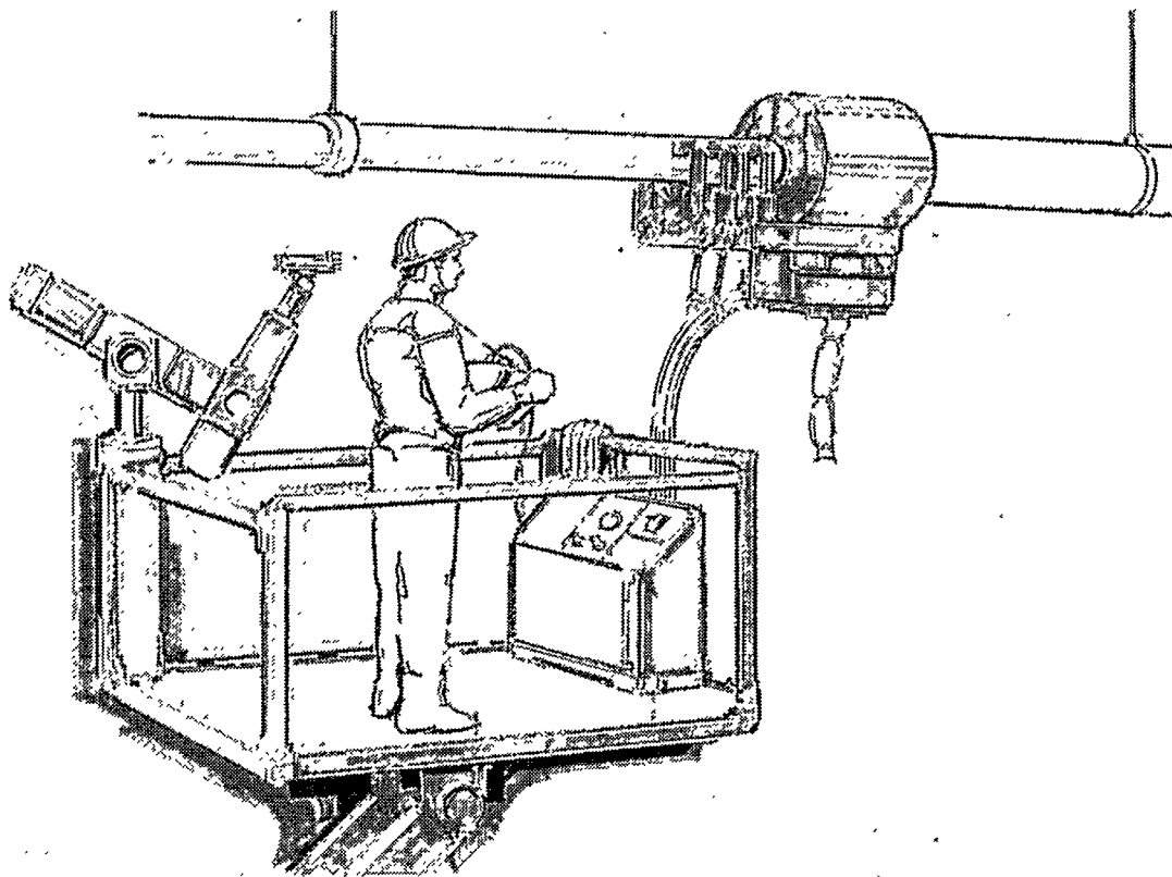
Figure 6-1 : Operational scenario for the pipe-asbestos insulation removal robot system in a fully robotic and human assistance modes, showing the asbestos removal and packaging actions in progress
