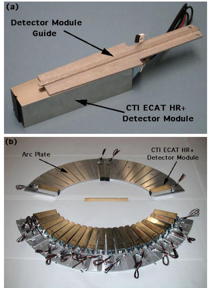
Fig. 4: (a) CTI ECAT HR+ detector module with an aluminum guide epoxied along its midline. (b) Photograph of the top and bottom aluminum arc plates with some of the CTI ECAT HR+ detector modules mounted in place. Each detector module has an aluminum guide that slides along a groove in the arc plate and is stopped (and secured against the arc plate) using a mortise and tenon. The detector modules are individually angled to point towards the center of the camera.
