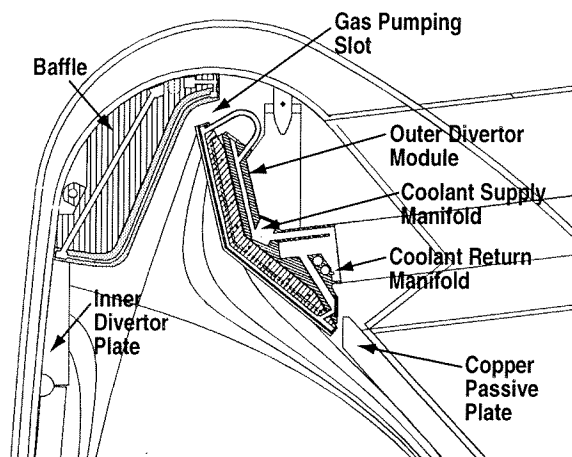
Fig. 1. Cross Section Through FIRE divertor and baffle.
