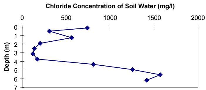
Figure 3a. U3cno (inner) chloride concentration vs. depth.
