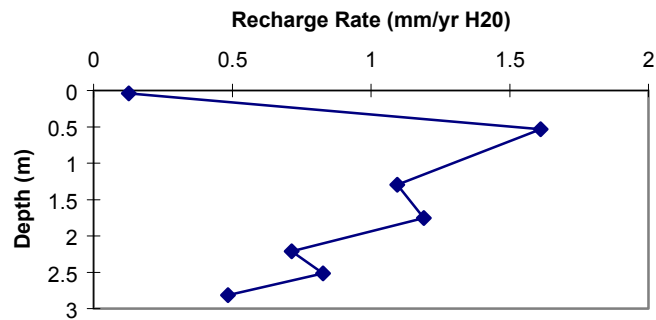
Figure 30c. RV-1 recharge flux vs. depth.
