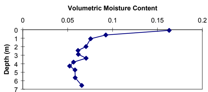
Figure 10b. ER-19-1 (wash on road) volumetric moisture content vs. depth.
