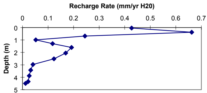
Figure 36c. SPB-2 recharge flux vs. depth.
