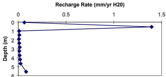
Figure 28c. MV-1 recharge flux vs. depth.
