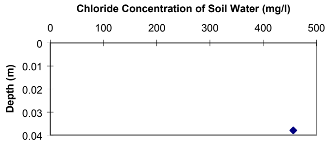
Figure 32a. SPA-1 chloride concentration vs. depth.
