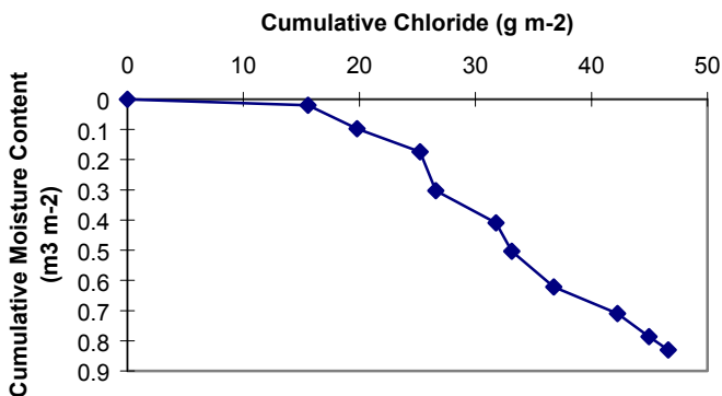
Figure 29d. RM-1 summed chloride concentration vs. volumetric moisture content.
