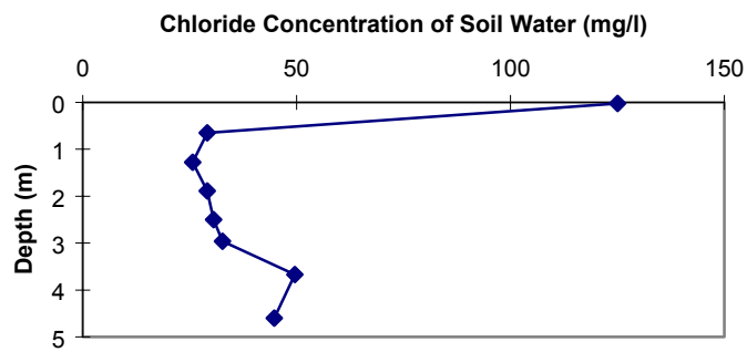
Figure 12a. ER-19-1 (wash) chloride concentration vs. depth.
