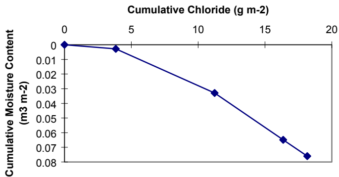
Figure 31d. RV-2 summed chloride concentration vs. volumetric moisture content.
