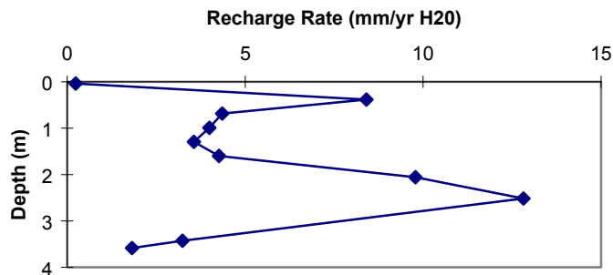
Figure 40c. TMW recharge flux vs. depth.
