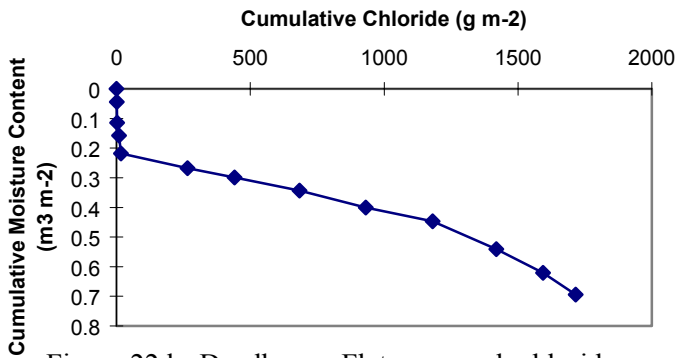
Figure 22d. Deadhorse Flat summed chloride concentration vs. volumetric moisture content.
