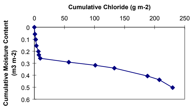
Figure 10d. ER-19-1 (wash on road) summed chloride concentration vs. volumetric moisture content.
