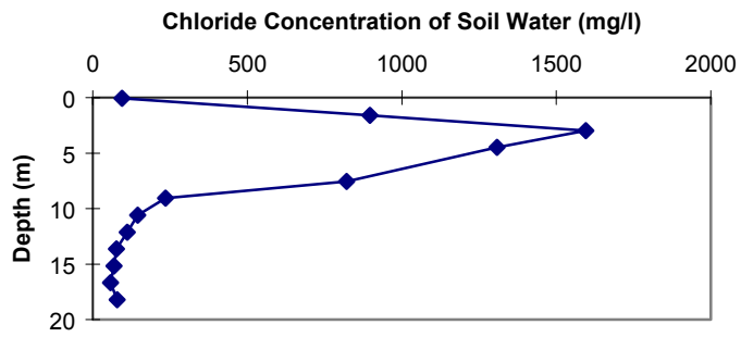
Figure 4a. U5an-2 chloride concentration vs. depth (outside the crater).
