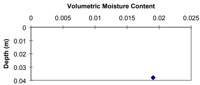
Figure 32b. SPA-1 volumetric moisture content vs. depth.
