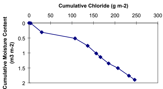
Figure 11d. ER-19-1 (ridge) summed chloride concentration vs. volumetric moisture content.
