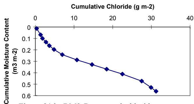
Figure 21d. BM2-B summed chloride concentration vs. volumetric moisture content.
