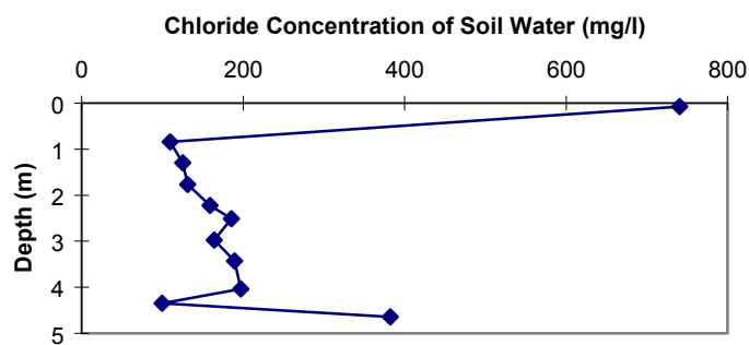
Figure 9a. ER-18-1 (wash) chloride concentration vs. depth.
