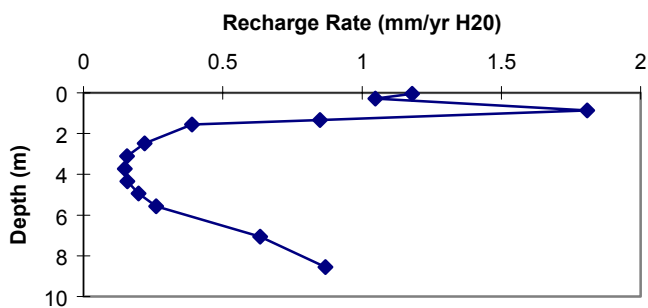
Figure 16c. ER-20-6 recharge flux vs. depth.
