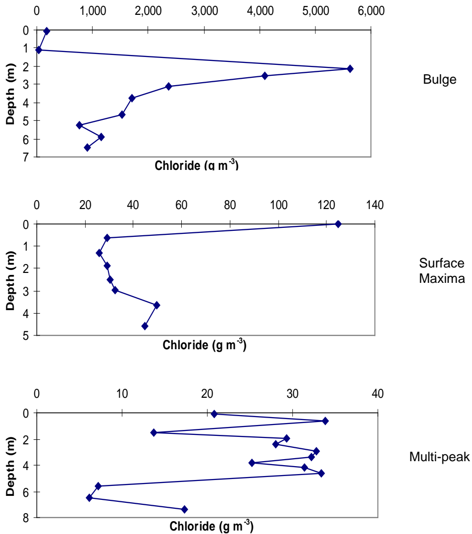
Figure 10. Examples of subsurface chloride profiles obtained during the course of this study.
