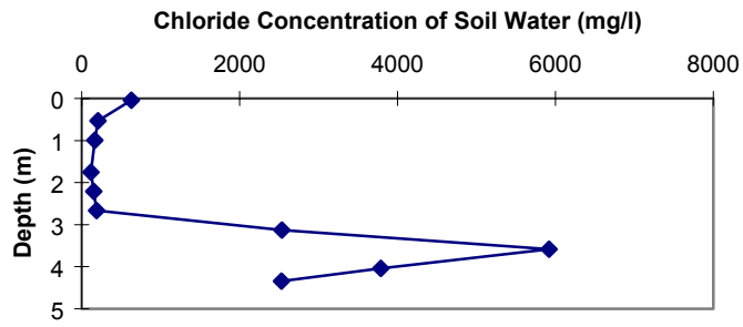
Figure 38a. SW-1 chloride concentration vs. depth.
