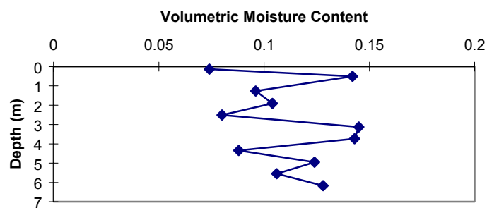
Figure 3b. U3cno (inner) volumetric moisture content vs. depth.
