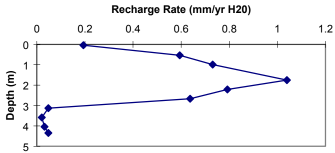
Figure 38c. SW-1 recharge flux vs. depth.
