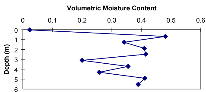
Figure 11b. ER-19-1 (ridge) volumetric moisture content vs. depth.
