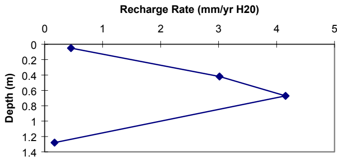
Figure 15c. ER-20-5 recharge flux vs. depth.
