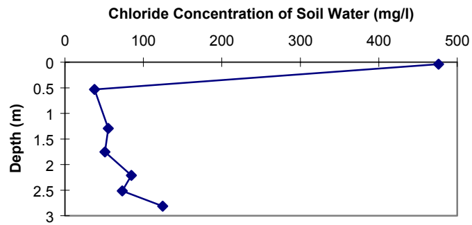
Figure 30a. RV-1 chloride concentration vs. depth.
