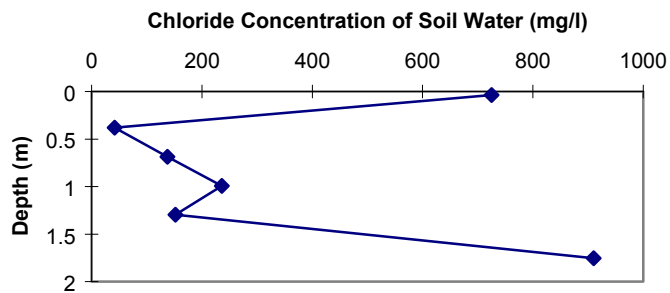
Figure 25a. DHF-5 chloride concentration vs. depth.
