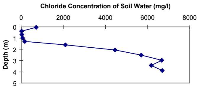
Figure 37a. SPB-3 chloride concentration vs. depth.
