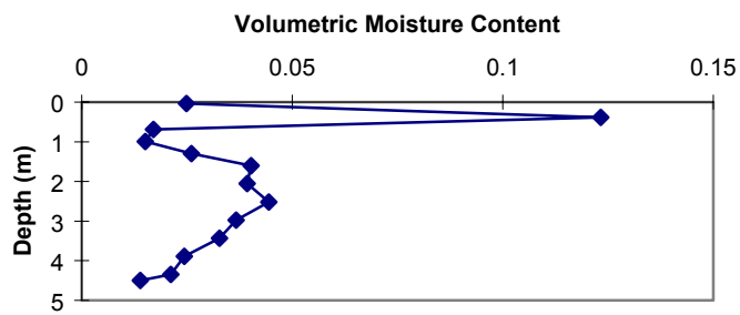
Figure 36b. SPB-2 volumetric moisture content vs. depth.
