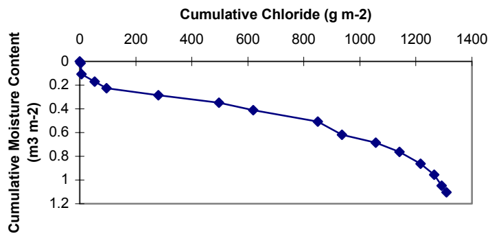
Figure 1d. Ue-1q summed chloride concentration vs. volumetric moisture content.
