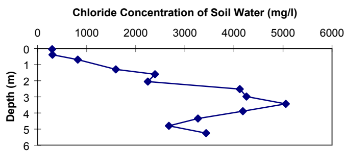
Figure 34a. SPA-3 chloride concentration vs. depth.
