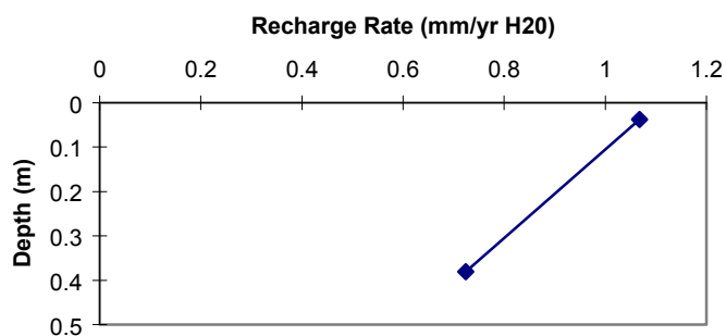
Figure 35c. SPB-1 recharge flux vs. depth.
