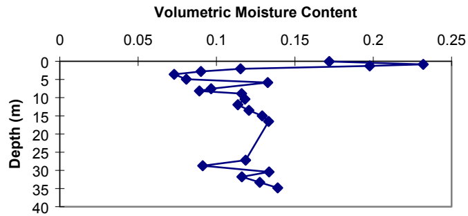
Figure 5b. U5an-1 volumetric moisture content vs. depth (inside the crater).
