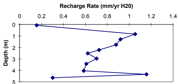
Figure 9c. ER-18-1 (wash) recharge flux vs. depth.
