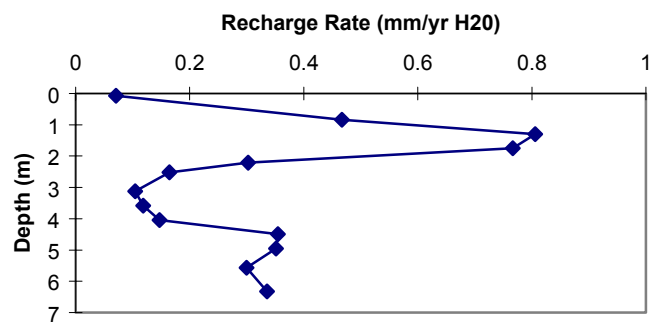
Figure 8c. ER-18-2 (ridge) recharge flux vs. depth.
