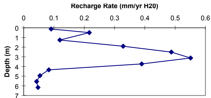
Figure 3c. U3cno (inner) recharge flux vs. depth.
