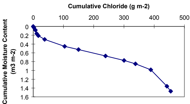
Figure 16d. ER-20-6 summed chloride concentration vs. volumetric moisture content.
