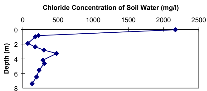
Figure 39a. TM-1 chloride concentration vs. depth.
