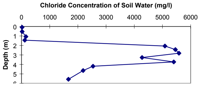
Figure 22a. Deadhorse Flat chloride concentration vs. depth.
