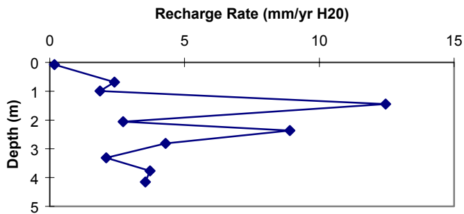
Figure 29c. RM-1 recharge flux vs. depth.
