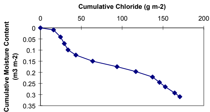
Figure 8d. ER-18-2 (ridge) summed chloride concentration vs. volumetric moisture content.
