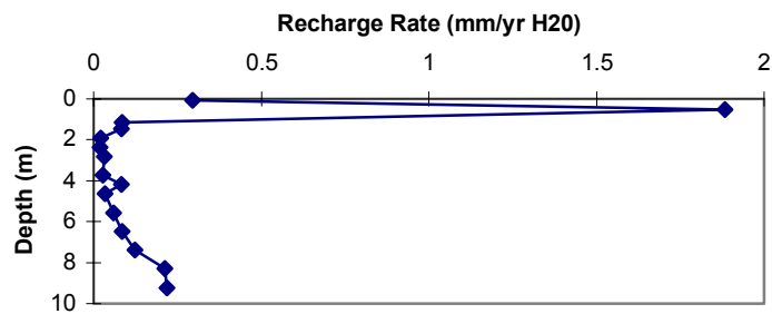
Figure 1c. Ue-1q recharge flux vs. depth.
