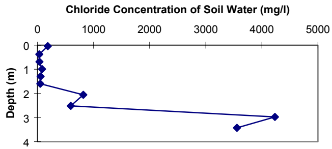
Figure 19a. BM1-B chloride concentration vs. depth.
