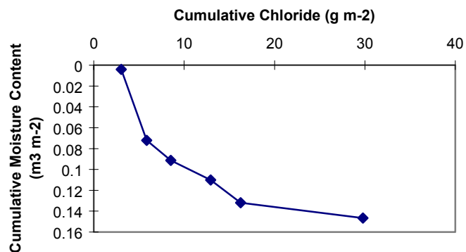
Figure 25d. DH-5 summed chloride concentration vs. volumetric moisture content.
