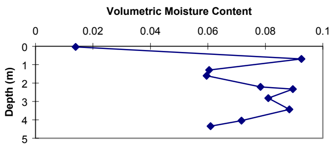
Figure 27b. JF-1 volumetric moisture content vs. depth.
