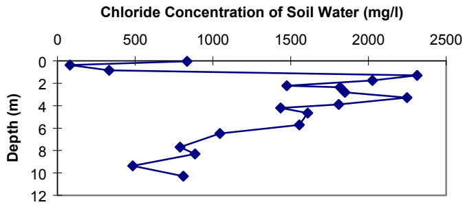
Figure 26a. FF-1 chloride concentration vs. depth.
