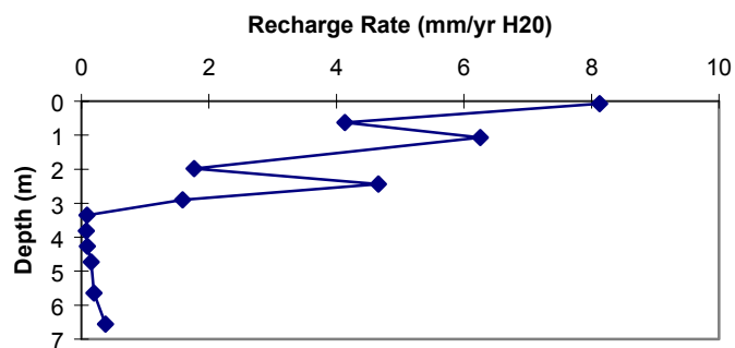
Figure 10c. ER-19-1 (wash on road) recharge flux vs. depth.
