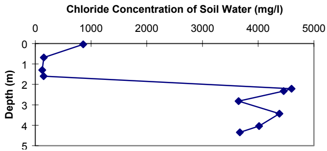
Figure 27a. JF-1 chloride concentration vs. depth.
