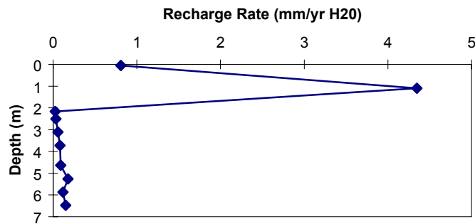
Figure 14c. ER-20-2 recharge flux vs. depth.
