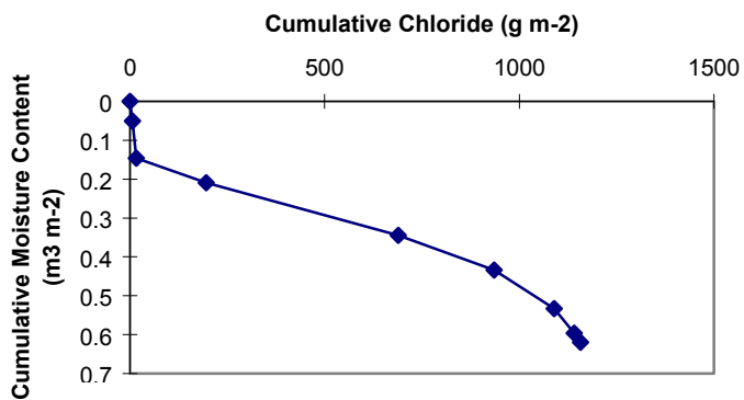
Figure 6d. ER-6-1 summed chloride concentration vs. volumetric moisture content.
