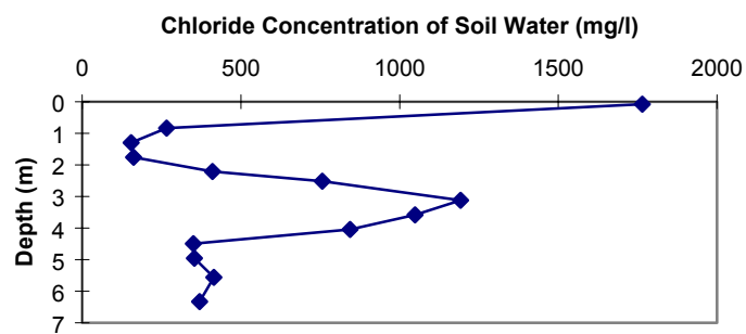
Figure 8a. ER-18-2 (ridge) chloride concentration vs. depth.
