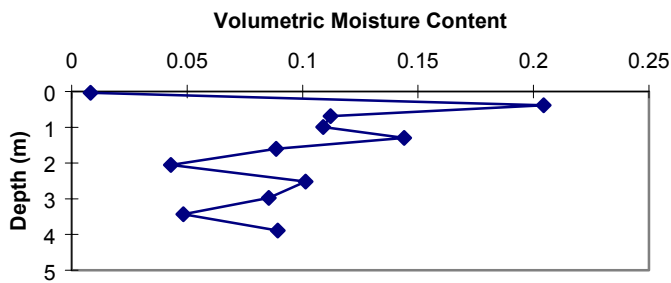
Figure 37b. SPB-3 volumetric moisture content vs. depth.
