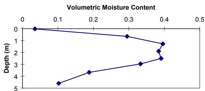
Figure 12b. ER-19-1 (wash) volumetric moisture content vs. depth.
