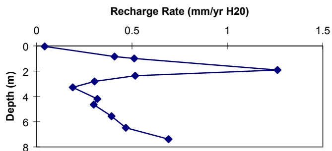
Figure 39c. TM-1 recharge flux vs. depth.
