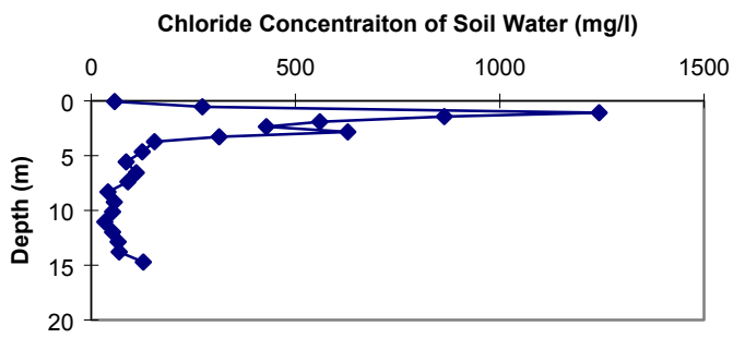
Figure 7a. ER-6-2 chloride concentration vs. depth.
