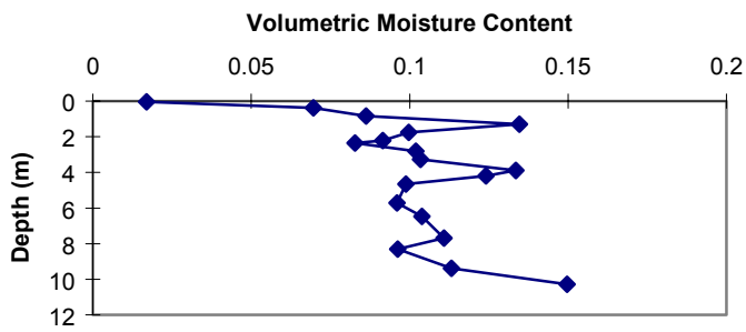
Figure 26b. FF-1 volumetric moisture content vs. depth.
