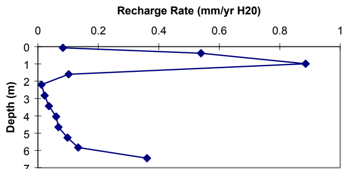
Figure 2c. U3cno (outer) recharge flux vs. depth.
