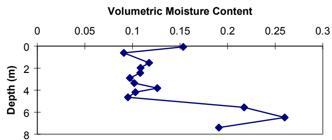
Figure 17b. ER-30-1 volumetric moisture content vs. depth.
