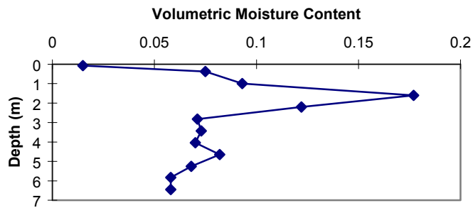
Figure 2b. U3cno (outer) volumetric moisture content vs. depth.
