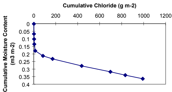
Figure 37d. SPB-3 summed chloride concentration vs. volumetric moisture content.
