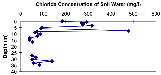
Figure 5a. U5an-1 chloride concentration vs. depth (inside the crater).
