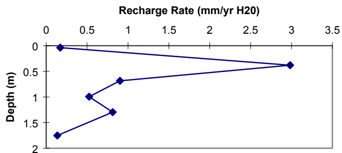
Figure 25c. DHF-5 recharge flux vs. depth.
