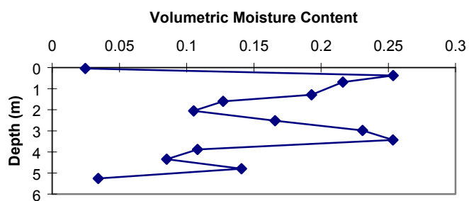
Figure 34b. SPA-3 volumetric moisture content vs. depth.
