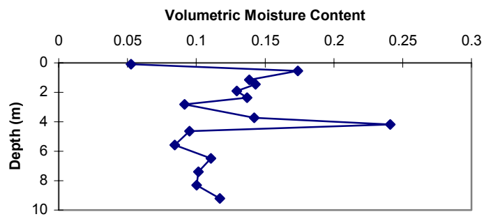
Figure 1b. Ue-1q volumetric moisture content vs. depth.
