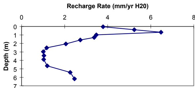
Figure 21c. BM2-B recharge flux vs. depth.
