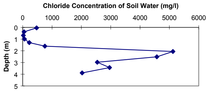
Figure 24a. DHF-4 chloride concentration vs. depth.
