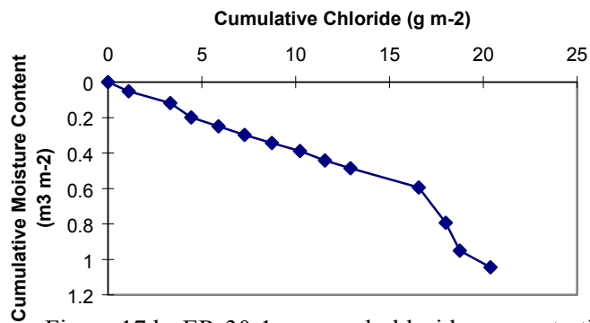
Figure 17d. ER-30-1 summed chloride concentration vs. volumetric moisture content.
