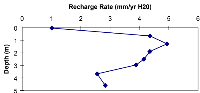
Figure 12c. ER-19-1 (wash) recharge flux vs. depth.
