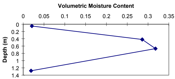
Figure 15b. ER-20-5 volumetric moisture content vs. depth.
