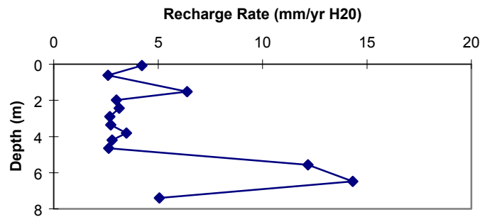
Figure 17c. ER-30-1 recharge flux vs. depth.
