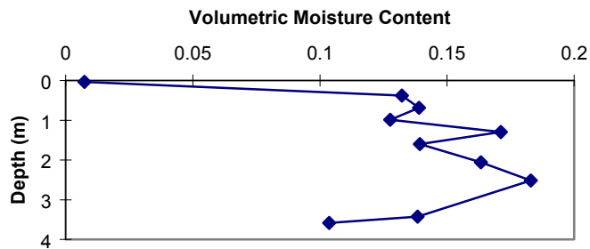
Figure 40b. TMW volumetric moisture content vs. depth.
