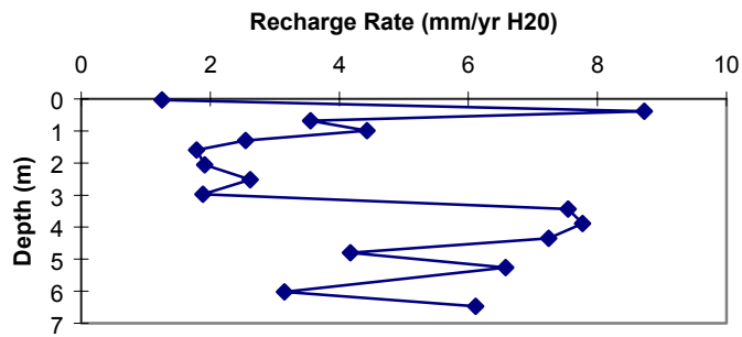
Figure 18c. BM1-A recharge flux vs. depth.
