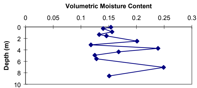
Figure 16b. ER-20-6 volumetric moisture content vs. depth.
