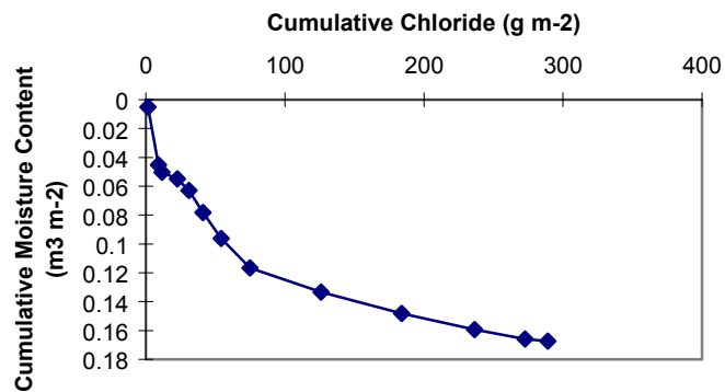
Figure 36d. SPB-2 summed chloride concentration vs. volumetric moisture content.
