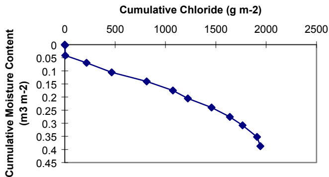
Figure 28d. MV-1 summed chloride concentration vs. volumetric moisture content.
