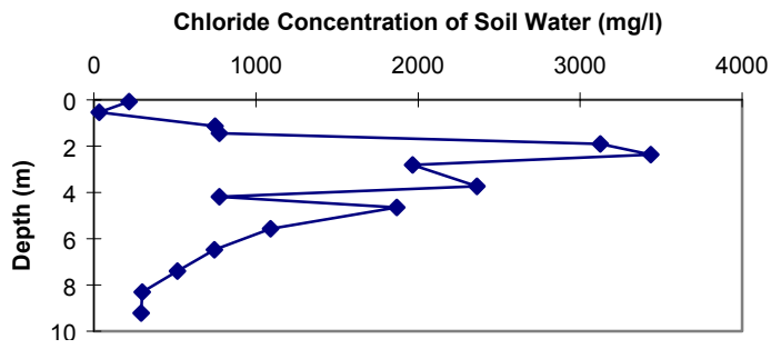
Figure 1a. Ue-1q chloride concentration vs. depth.
