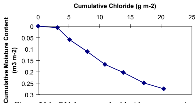
Figure 30d. RV-1 summed chloride concentration vs. volumetric moisture content.
