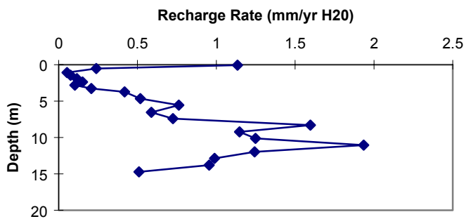
Figure 7c. ER-6-2 recharge flux vs. depth.
