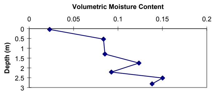
Figure 30b. RV-1 volumetric moisture content vs. depth.
