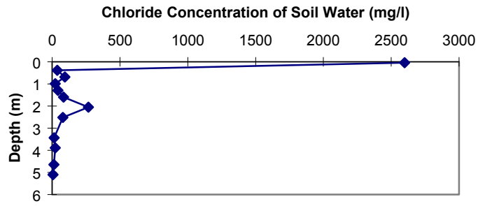
Figure 20a. BM2-A chloride concentration vs. depth.
