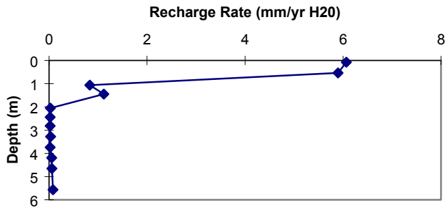
Figure 22c. Deadhorse Flat recharge flux vs. depth.
