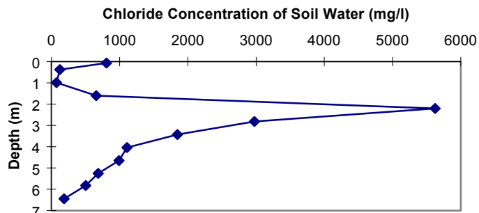
Figure 2a. U3cno (outer) chloride concentration vs. depth.
