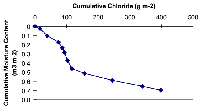
Figure 3d. U3cno (inner) summed chloride concentration vs. volumetric moisture content.
