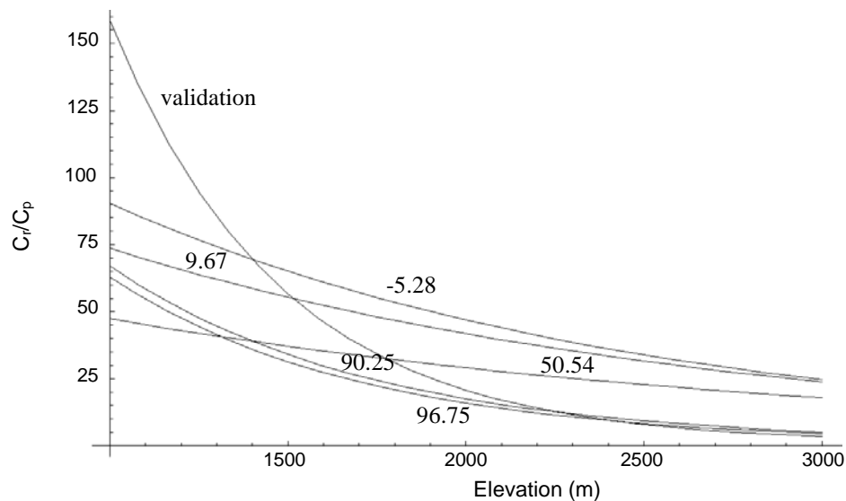
Figure 22. Graph of equations from Table 7 and the validation equation.
