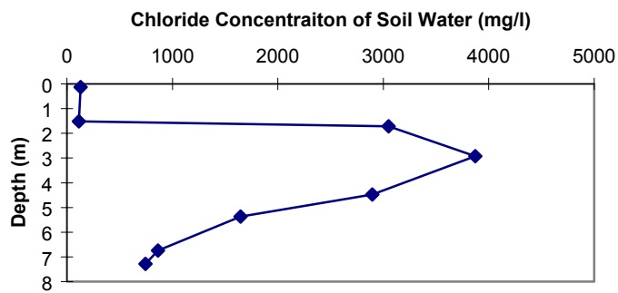
Figure 6a. ER-6-1 chloride concentration vs. depth.
