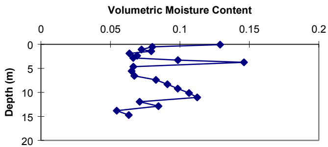
Figure 7b. ER-6-2 volumetric moisture content vs. depth.
