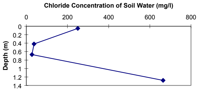
Figure 15a. ER-20-5 chloride concentration vs. depth.
