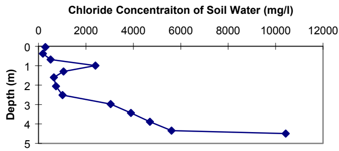
Figure 36a. SPB-2 chloride concentration vs. depth.
