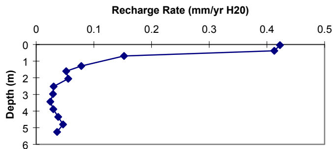
Figure 34c. SPA-3 recharge flux vs. depth.
