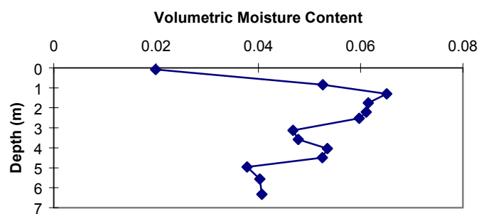
Figure 8b. ER-18-2 (ridge) volumetric moisture content vs. depth.
