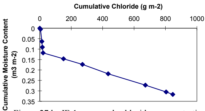
Figure 27d. JF-1 summed chloride concentration vs. volumetric moisture content.
