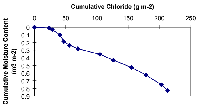
Figure 39d. TM-1 summed chloride concentration vs. volumetric moisture content.
