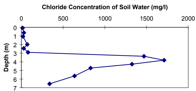
Figure 10a. ER-19-1 (wash on road) chloride concentration vs. depth.
