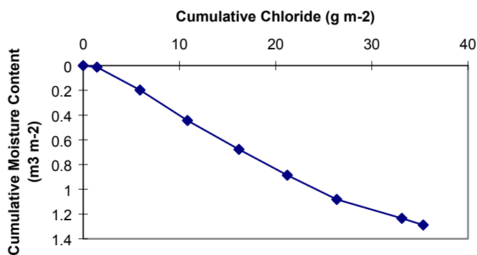
Figure 12d. ER-19-1 (wash) summed chloride concentration vs. volumetric moisture content.
