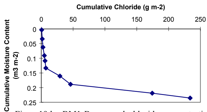
Figure 19d. BM1-B summed chloride concentration vs. volumetric moisture content.
