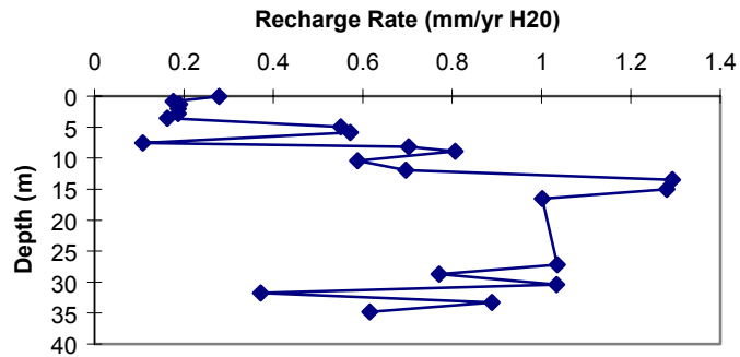
Figure 5c. U5an-1 recharge flux vs. depth (inside the crater).
