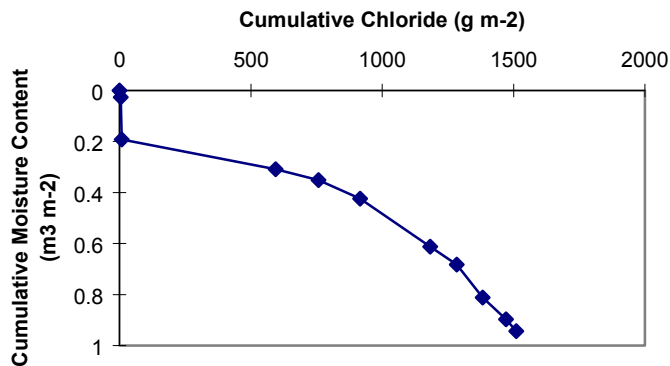
Figure 14d. ER-20-2 summed chloride concentration vs. volumetric moisture content.
