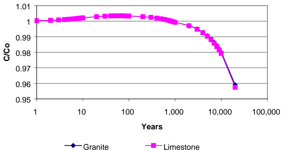
Figure 9. Results of sensitivity of ^{36}\text{Cl}/\text{Cl} to epigenic and hypogenic production over a 20,000-yr period.
