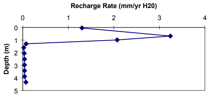
Figure 23c. DHF-3 recharge flux vs. depth.
