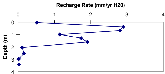
Figure 19c. BM1-B recharge flux vs. depth.
