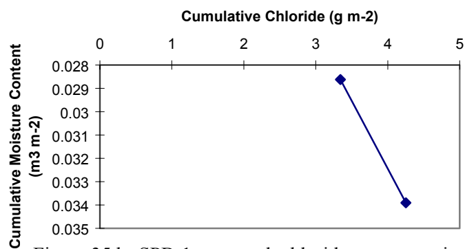
Figure 35d. SPB-1 summed chloride concentration vs. volumetric moisture content.
