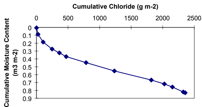
Figure 34d. SPA-3 summed chloride concentration vs. volumetric moisture content.
