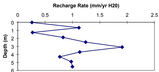
Figure 11c. ER-19-1 (ridge) recharge flux vs. depth.
