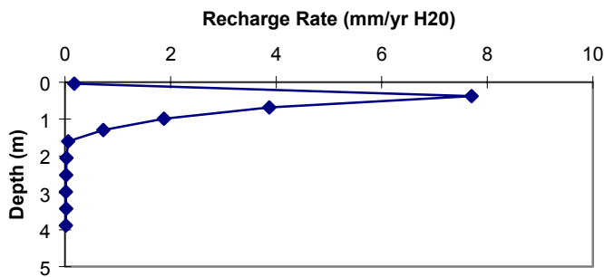
Figure 37c. SPB-3 recharge flux vs. depth.
