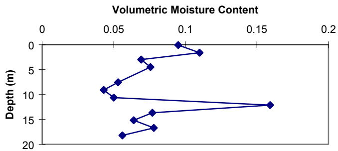
Figure 4b. U5an-2 volumetric moisture content vs. depth (outside the crater).
