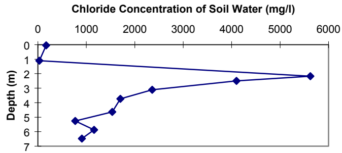
Figure 14a. ER-20-2 chloride concentration vs. depth.
