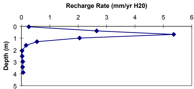
Figure 24c. DHF-4 recharge flux vs. depth.
