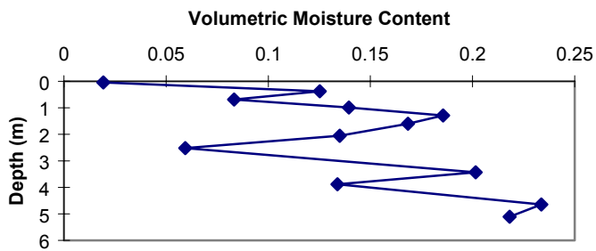
Figure 20b. BM2-A volumetric moisture content vs. depth.
