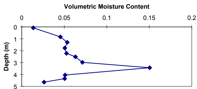
Figure 9b. ER-18-1 (wash) volumetric moisture content vs. depth.
