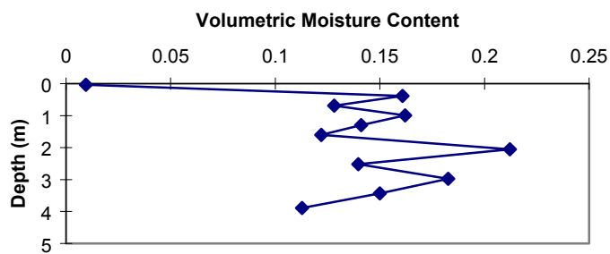
Figure 24b. DHF-4 volumetric moisture content vs. depth.
