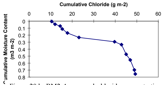
Figure 20d. BM2-A summed chloride concentration vs. volumetric moisture content.
