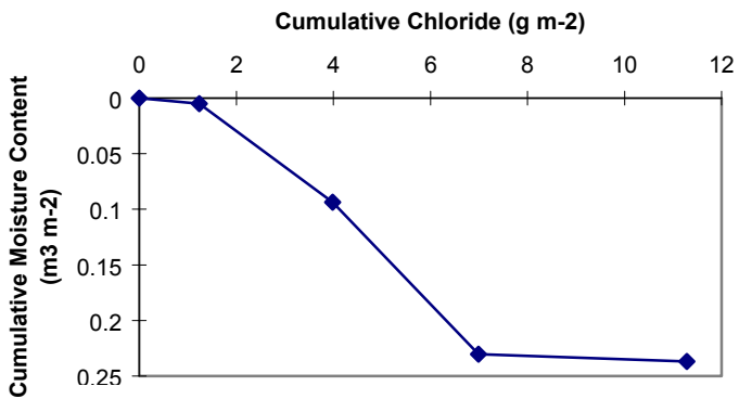
Figure 15d. ER-20-5 summed chloride concentration vs. volumetric moisture content.
