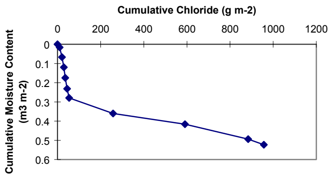
Figure 38d. SW-1 summed chloride concentration vs. volumetric moisture content.
