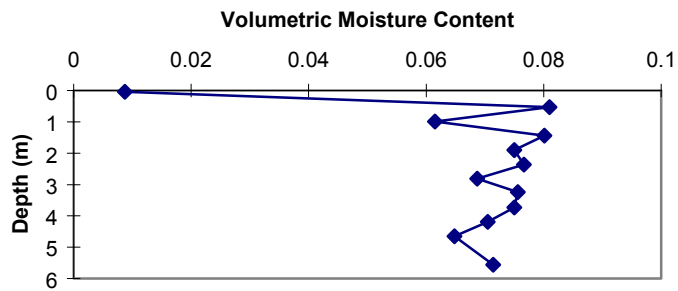
Figure 28b. MV-1 volumetric moisture content vs. depth.
