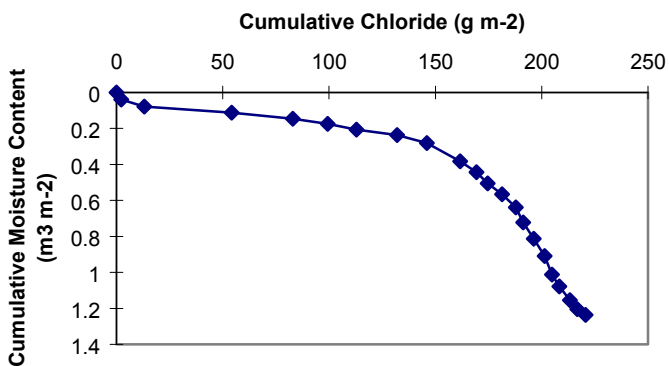
Figure 7d. ER-6-2 summed chloride concentration vs. volumetric moisture content.
