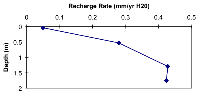
Figure 31c. RV-2 recharge flux vs. depth.
