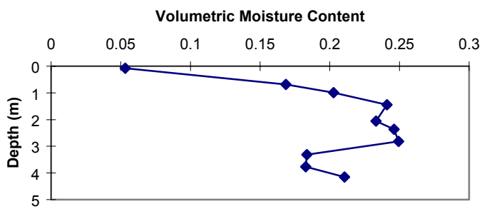
Figure 29b. RM-1 volumetric moisture content vs. depth.
