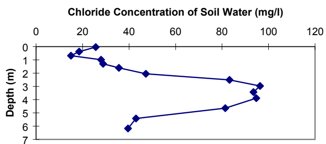
Figure 21a. BM2-B chloride concentration vs. depth.
