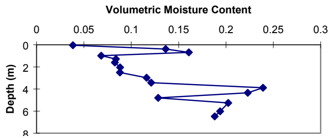
Figure 18b. BM1-A volumetric moisture content vs. depth.
