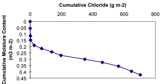
Figure 13d. ER-19-2 (barrow pit) summed chloride concentration vs. volumetric moisture content.
