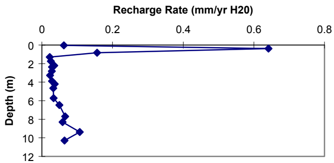
Figure 26c. FF-1 recharge flux vs. depth.
