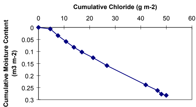
Figure 9d. ER-18-1 (wash) summed chloride concentration vs. volumetric moisture content.
