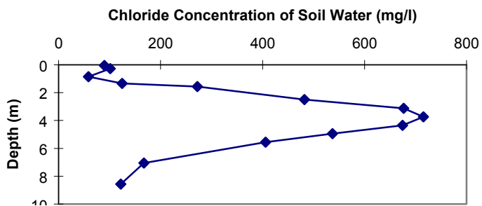
Figure 16a. ER-20-6 chloride concentration vs. depth.
