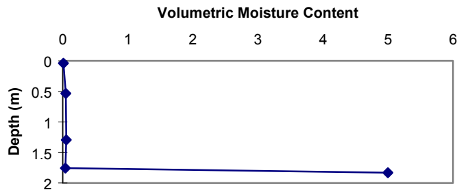
Figure 31b. RV-2 volumetric moisture content vs. depth.
