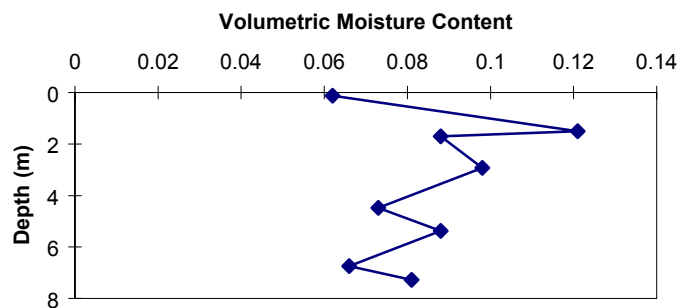
Figure 6b. ER-6-1 volumetric moisture content vs. depth.
