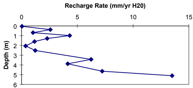
Figure 20c. BM2-A recharge flux vs. depth.
