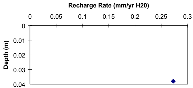
Figure 32c. SPA-1 recharge flux vs. depth.
