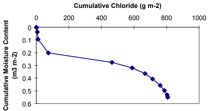
Figure 2d. U3cno (outer) summed chloride concentration vs. volumetric moisture content.
