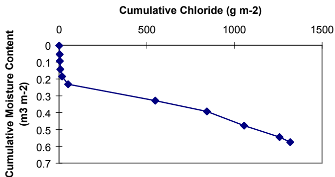
Figure 24d. DHF-4 summed chloride concentration vs. volumetric moisture content.
