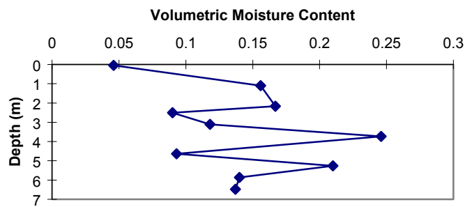
Figure 14b. ER-20-2 volumetric moisture content vs. depth.
