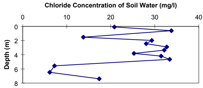
Figure 17a. ER-30-1 chloride concentration vs. depth.
