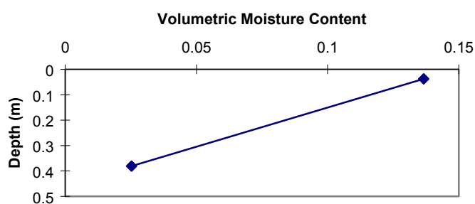
Figure 35b. SPB-1 volumetric moisture content vs. depth.
