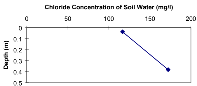
Figure 35a. SPB-1 chloride concentration vs. depth.
