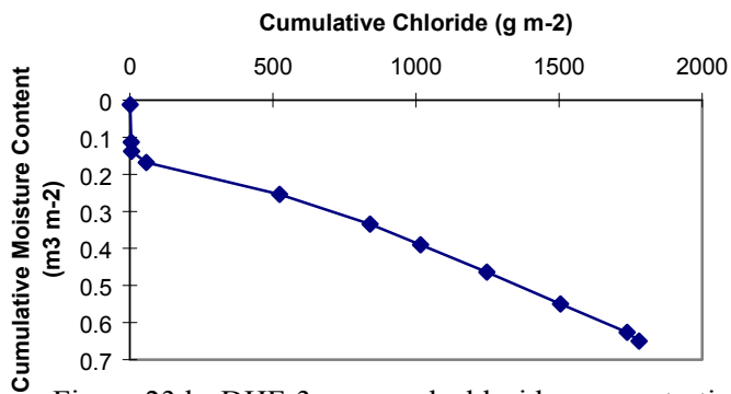
Figure 23d. DHF-3 summed chloride concentration vs. volumetric moisture content.
