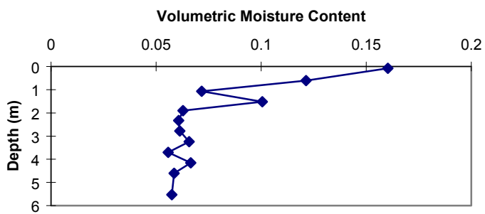
Figure 13b. ER-19-2 (barrow pit) volumetric moisture content vs. depth.
