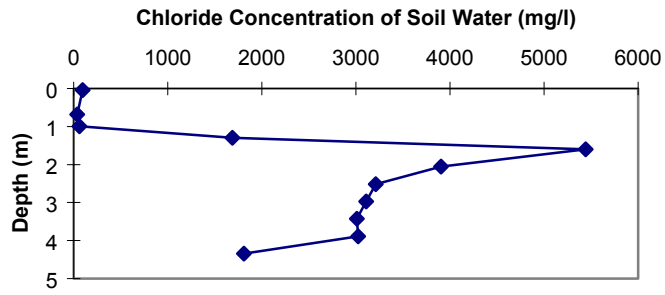
Figure 23a. DHF-3 chloride concentration vs. depth.
