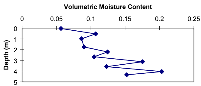
Figure 38b. SW-1 volumetric moisture content vs. depth.
