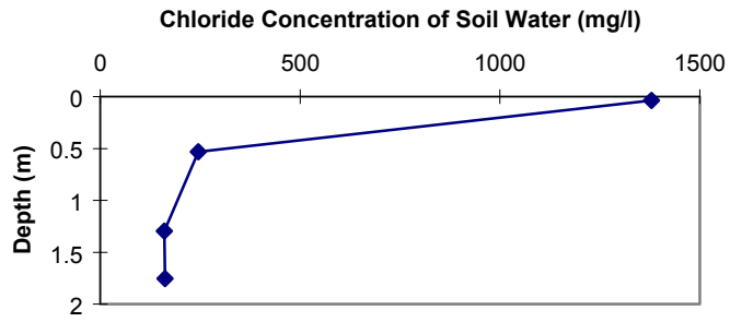
Figure 31a. RV-2 chloride concentration vs. depth.
