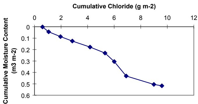
Figure 40d. TMW summed chloride concentration vs. volumetric moisture content.
