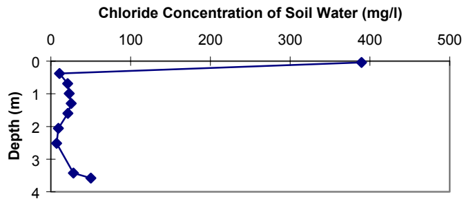
Figure 40a. TMW chloride concentration vs. depth.
