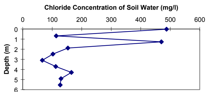
Figure 11a. ER-19-1 (ridge) chloride concentration vs. depth.
