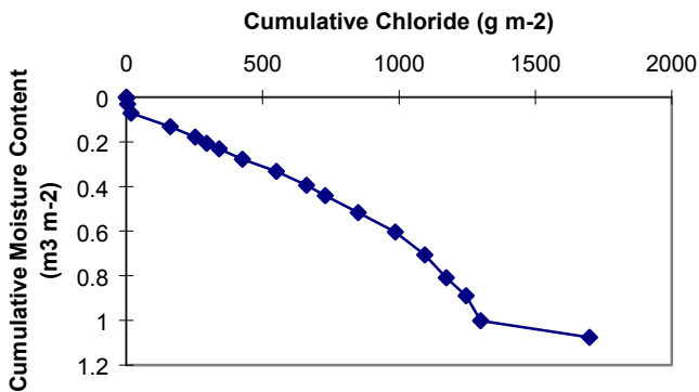
Figure 26d. FF-1 summed chloride concentration vs. volumetric moisture content.
