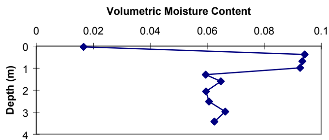
Figure 19b. BM1-B volumetric moisture content vs. depth.
