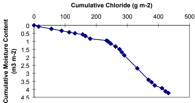
Figure 5d. U5an-1 summed chloride concentration vs. volumetric moisture content (inside the crater).
