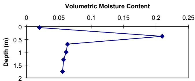
Figure 25b. DHF-5 volumetric moisture content vs. depth.
