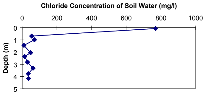
Figure 29a. RM-1 chloride concentration vs. depth.
