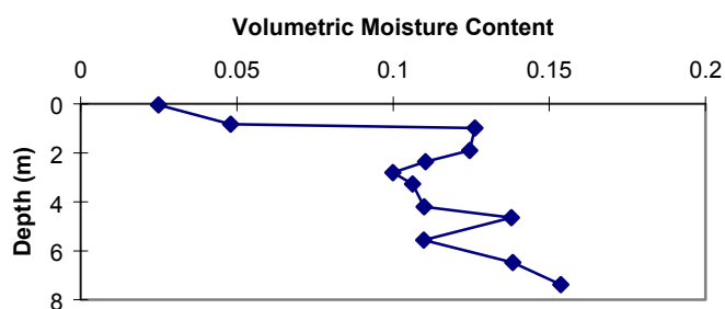
Figure 39b. TM-1 volumetric moisture content vs. depth.
