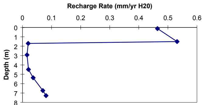
Figure 6c. ER-6-1 recharge flux vs. depth.
