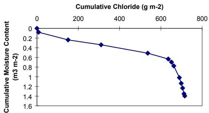
Figure 4d. U5an-2 summed chloride concentration vs. volumetric moisture content (outside the crater).
