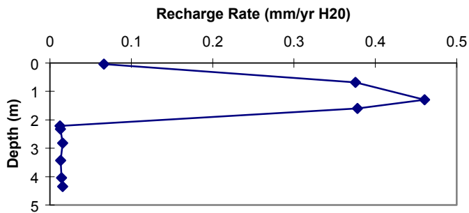
Figure 27c. JF-1 recharge flux vs. depth.
