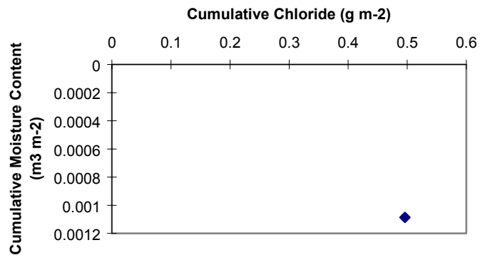
Figure 32d. SPA-1 summed chloride concentration vs. volumetric moisture content.
