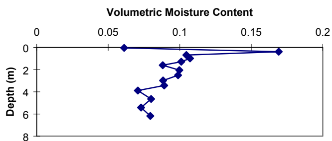
Figure 21b. BM2-B volumetric moisture content vs. depth.
