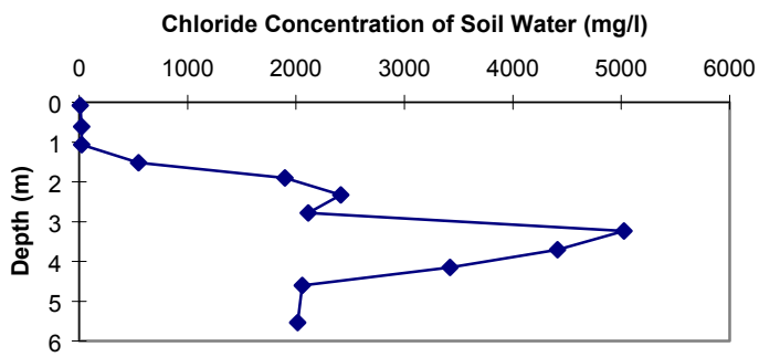
Figure 13a. ER-19-2 (barrow pit) chloride concentration vs. depth.
