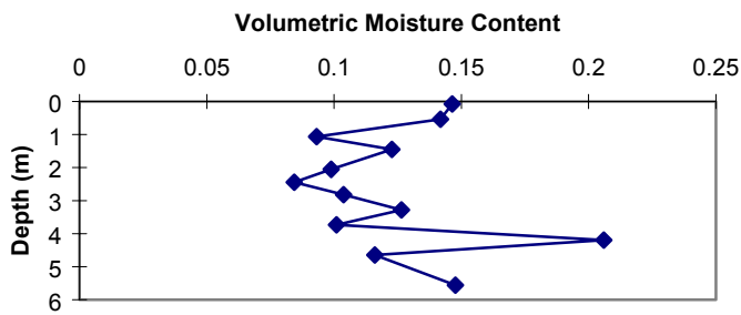
Figure 22b. Deadhorse Flat volumetric moisture content vs. depth.
