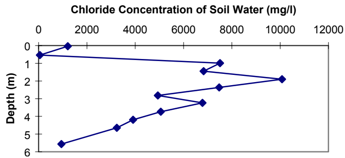
Figure 28a. MV-1 chloride concentration vs. depth.
