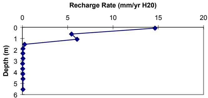
Figure 13c. ER-19-2 (barrow pit) recharge flux vs. depth.
