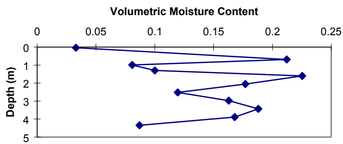
Figure 23b. DHF-3 volumetric moisture content vs. depth.
