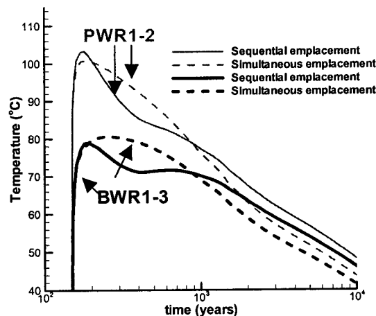
Figure 9. Waste-package temperature histories are given for a PWR and a BWR CSNF waste package at a location emplaced during the latter portion of the emplacement period ( P4E_{\text{CENTER}} ). The case that assumes simultaneous emplacement of waste results in slightly lower peak temperatures than those predicted for the case accounting for sequential emplacement.
