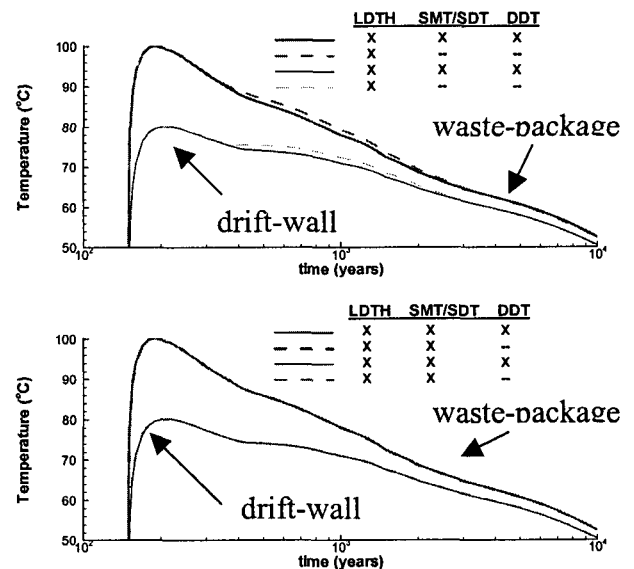
Figure 5. Waste-package temperatures and drift-wall temperatures for the P4E CENTER location are compared for three different approaches to representing repository-scale K_{th} heterogeneity.
