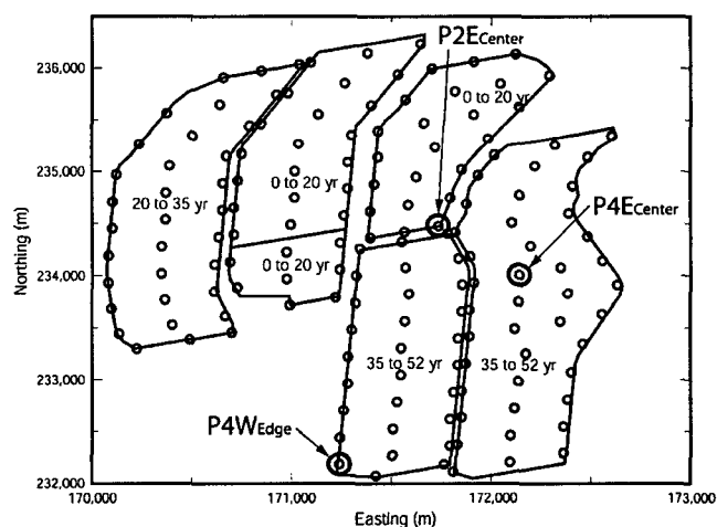
Figure 4. A total of 156 LDTH/SDT-submodel locations are available for a full macro-abstraction analysis. The loading time, e.g. '20 to 35 yr' of each panel is indicated. For this paper, the circled locations are discussed (P2E CENTER , an early-loaded location; P4E CENTER , a late-loaded center location; and P4W EDGE , a late-loaded edge location).
