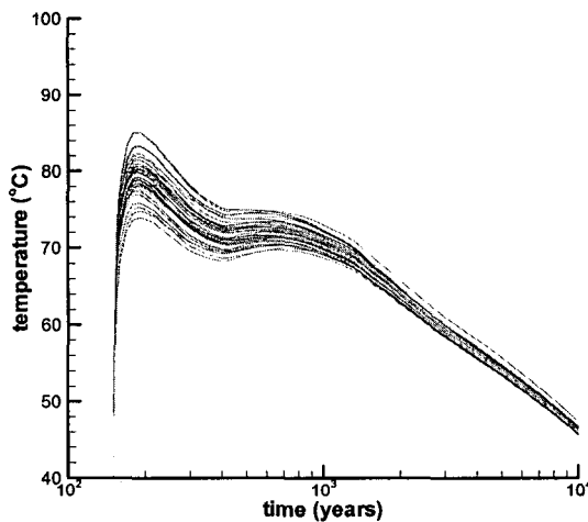
Figure 11. For waste-package temperature at 180 yr, the 50 repository-scale heterogeneous K_{th} realizations at location P4E CENTER result in a spread of 11.5°C for the DHLW-L2 waste package. Note that this waste package has the lowest heat output of those considered in these analyses.
