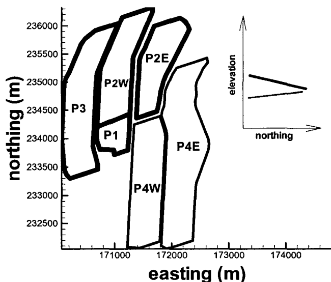
Figure 1. The repository layout considered in a recent MSTHM study in Nevada Coordinates [10]. This layout includes non-parallel emplacement planes labeled as: P1, P2E, P2W, P3, P4E, and P4W. Western panels P1, P2E, and P2W lie in one plane (see inset's heavy sloping line). Eastern panels P4E and P4W lie in a second plane (see the inset's lighter sloping line). Note that an additional panel (P5) south of P3 was considered a 'contingency' panel for this modeling exercise and, therefore, not included in this analysis.
