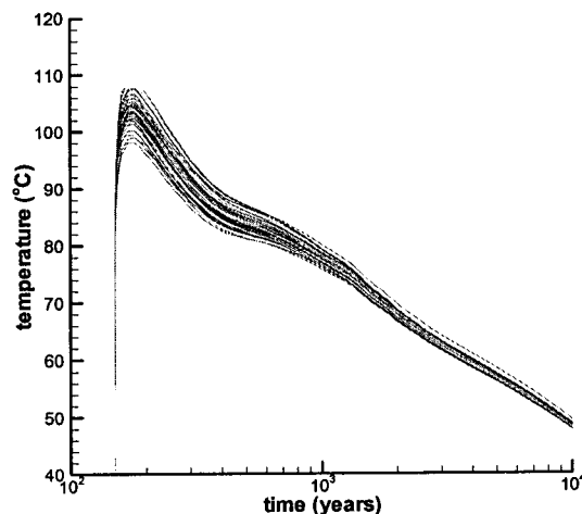
Figure 10. For waste-package temperature at 180 yr, the 50 repository-scale heterogeneous K_{th} realizations at location P4E_{\text{CENTER}} result in a spread of 11.4^{\circ}\text{C} for the PWR1-2 CSNF waste package. Note that this waste package has the highest heat output of those considered in these analyses.
