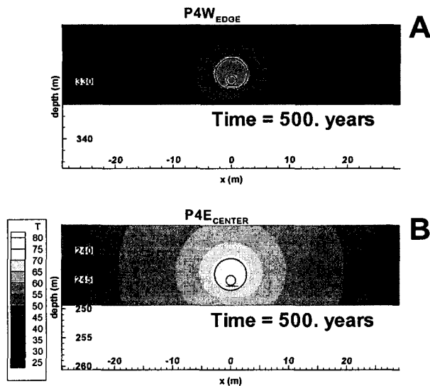
Figure 7. A vertical cross section of temperatures with x=0 at the drift center and depth from surface. Plot A: at 500 yr for the P4W EDGE location, which is near the repository edge and where waste packages are emplaced towards the end of the emplacement period. Plot B: at 500 yr for the P4E CENTER location, which is near the center of the repository and where waste packages are emplaced towards the end of the emplacement period. Temperatures are "line-averaged" for a sequence of 10 waste packages.
