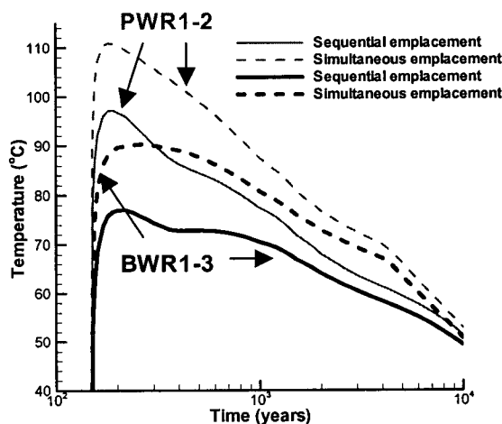
Figure 8. Waste-package temperature histories are given for a PWR and a BWR CSNF waste package at a location emplaced during the early portion of the emplacement period ( P2E_{\text{CENTER}} ). The case that assumes simultaneous emplacement of waste results in higher peak temperatures than a case accounting for sequential emplacement.
