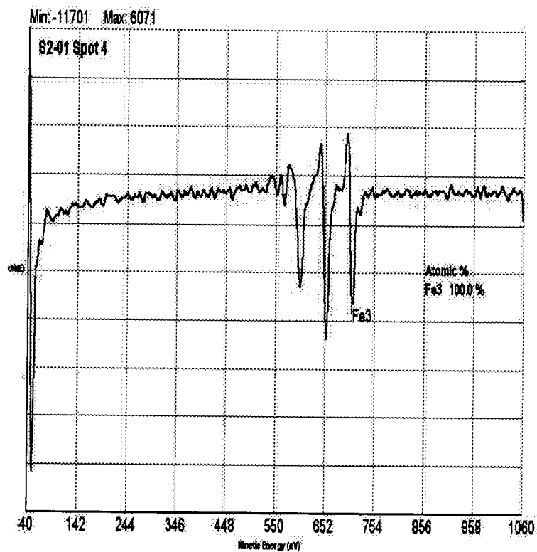
Figure 66. Auger spectrum of a cleavage facet (steel S2)
