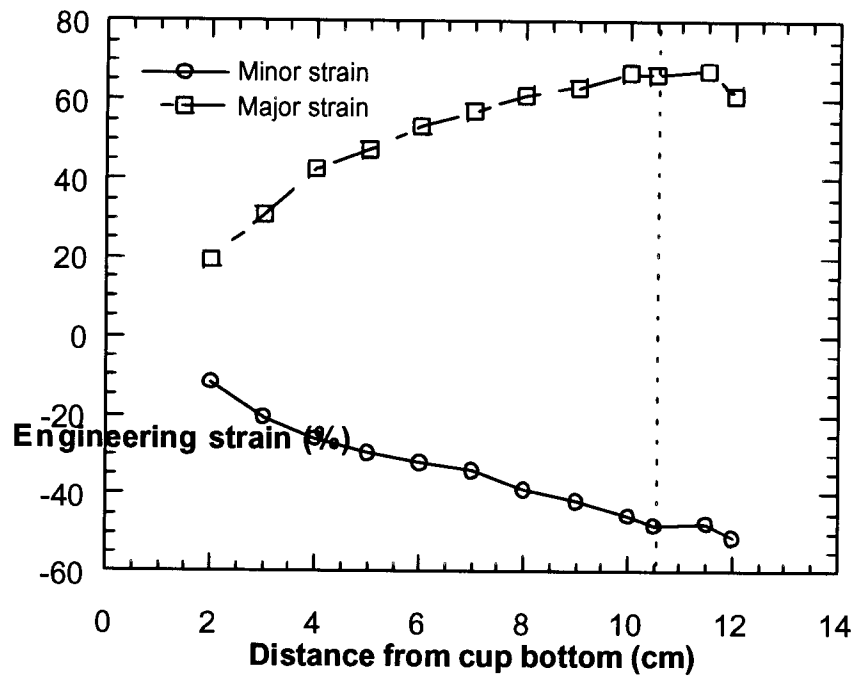
Figure 21. Strain distribution in the cup wall of a 6-inch as-drawn cup. (Legend: ○ – Minor strain; □ – Major strain)
