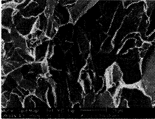
a) Steel S1, DBTT: -55^{\circ}\text{C} ; 4% IG
