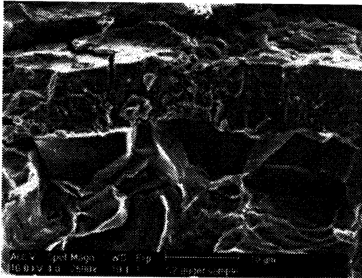
Figure 65. Intergranular fracture underneath the Zn coating in specimen S2 fracture in-situe in Auger.
