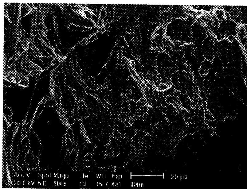
Fig. A-18. Fatigue fracture surface showing mixed intergranular/transgranular crack growth with secondary cracking – deep-drawn condition – transverse orientation at 0.3% applied strain amplitude (specimen B4).
