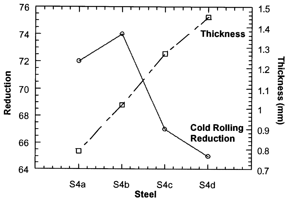
Figure 31. Cold reduction (%) and sheet thickness of series S4 steels
