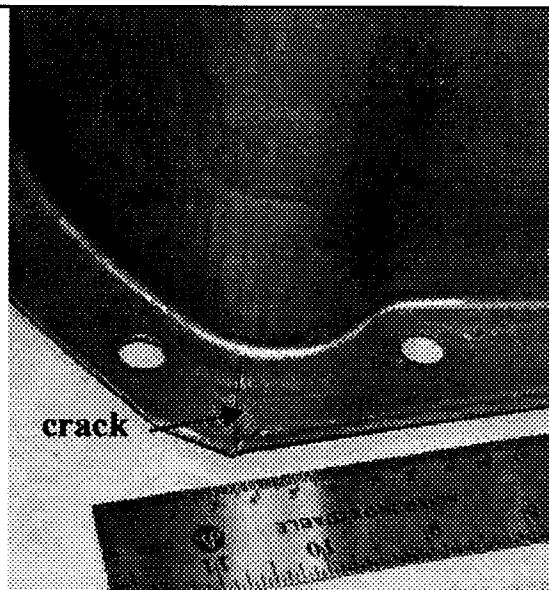
Figure 39 (d). Crack in a corner of a large diesel engine oil pan shown in Fig. 39(c).
