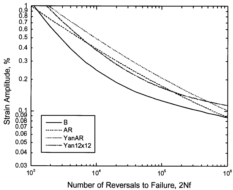
Fig. A-25. Strain – life curves for as-rolled and prestrained conditions for this study and Yan et al. [5].
