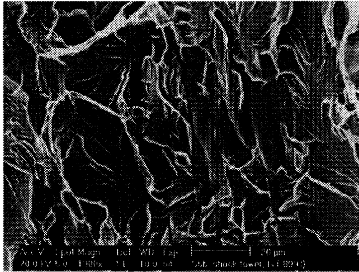
a) Fracture surface in an area with 50-60% strain, specimen fractured at -80°C
