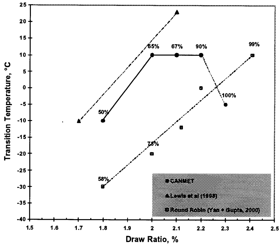
Figure 74. Transition temperature as a function of draw ratio
