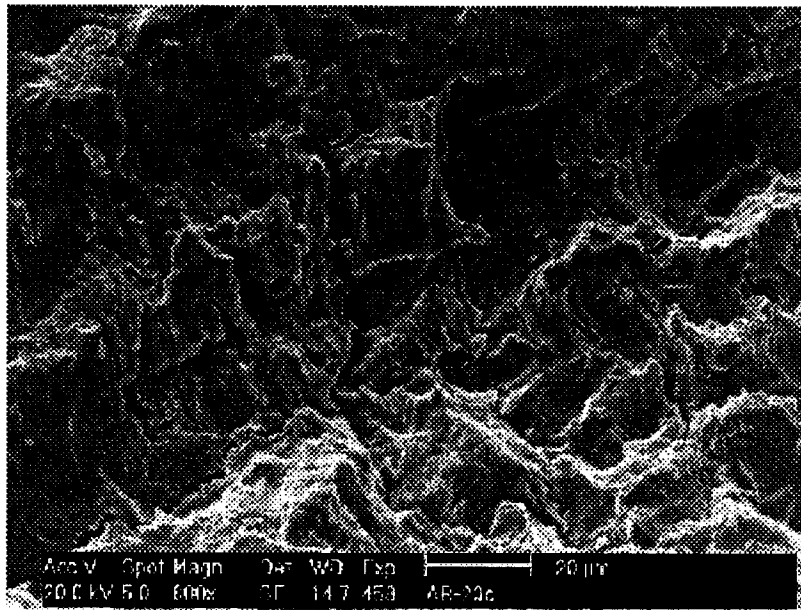
Fig. A-16. Fatigue fracture surface showing transgranular crack growth with secondary cracking – as-rolled condition at 0.4% applied strain amplitude (specimen AR20).
