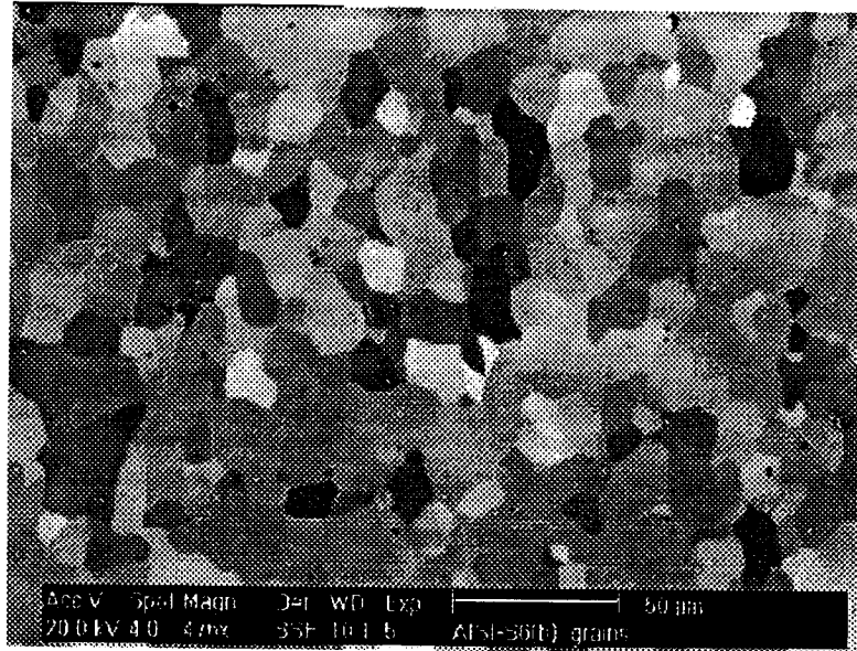
Fig. A-3. Grain structure of as-received steel S6b revealed using SEM back scattered electron imaging
