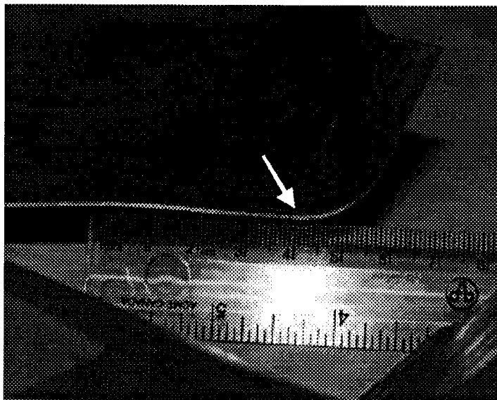
Figure 75. Crack initiation location in flange area of shock tower
