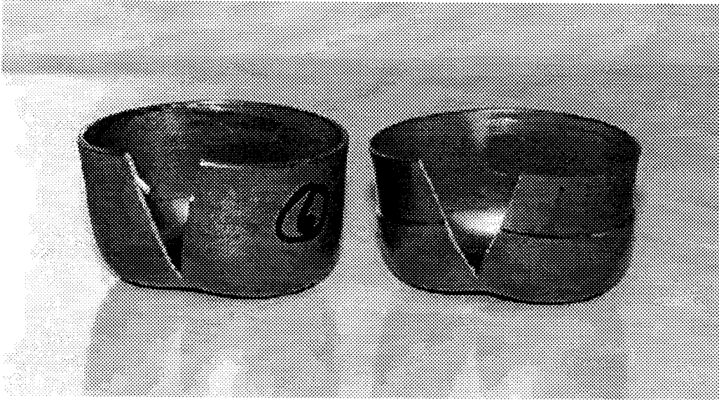
Figure 32. As-drawn and reduced-wall cups after trimming.
