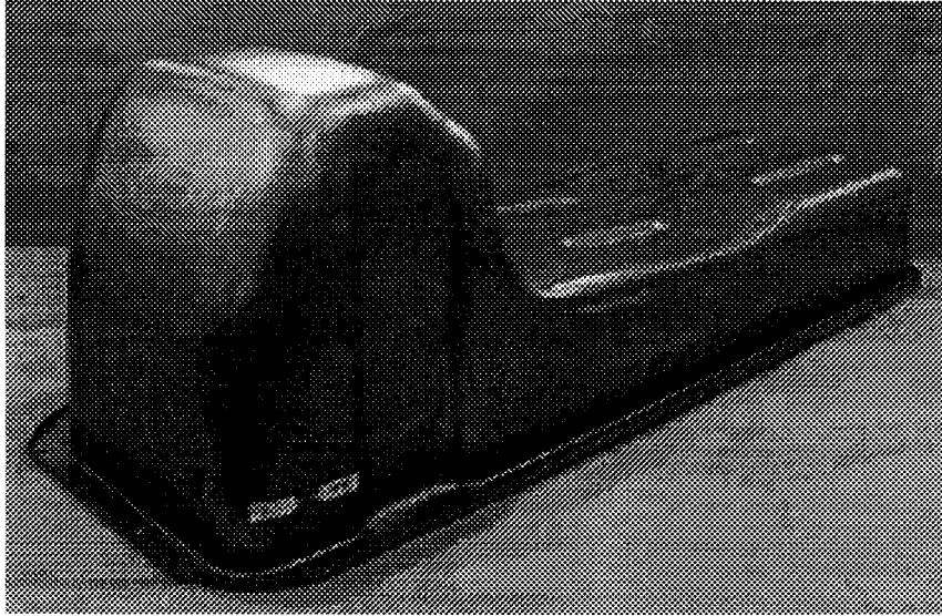
Fig. A-1. General view of oil pan in steel S6b showing general location of fatigue specimens.
