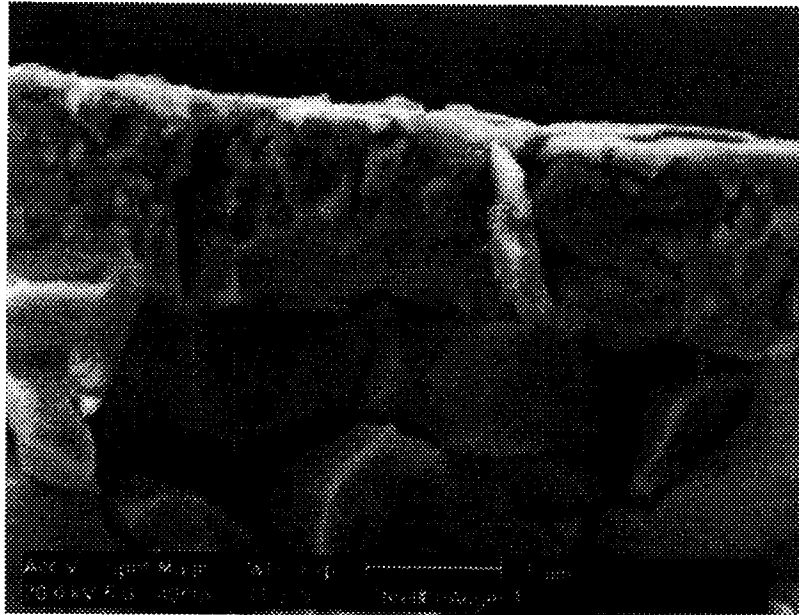
Figure 63. Intergranular fracture in S3 steel Auger specimen (upper part of image shows the galvaneal coating).
