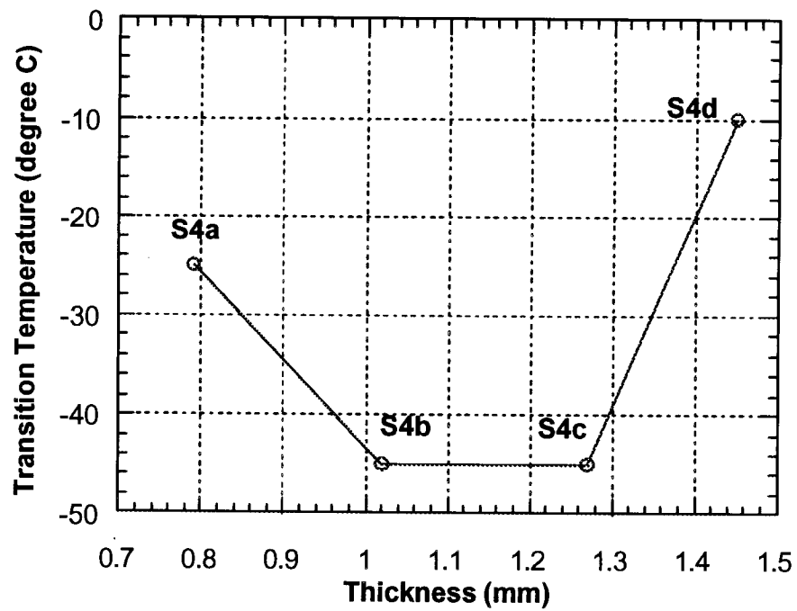
Figure 30. DBTT cup/expansion results obtained in 4 steels with different thickness.
