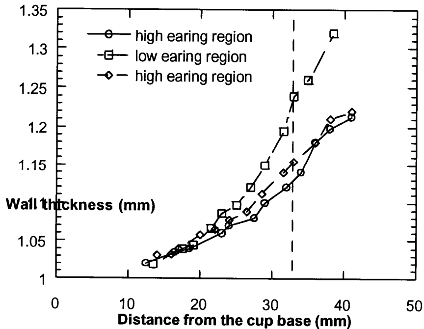
Figure 20. Wall thickness distribution at three angular positions in a as-drawn 2-inch cup (steel S4b). (Legend: o – high earing region; - low earing region; ◇- high earing region)
