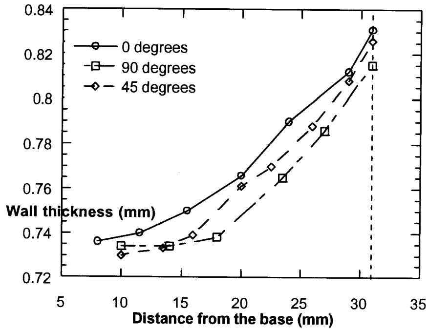
Figure 19. Wall thickness distribution at three angular positions in a 2-inch cup trimmed at 31 mm (steel S3) (Legend: o – 0 degrees; - 90 degrees; ◇- 45 degrees)
