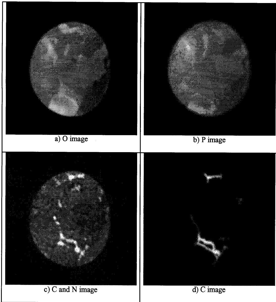
Figure 69. SIM images of steel S1 (100 \mu m diameter)
