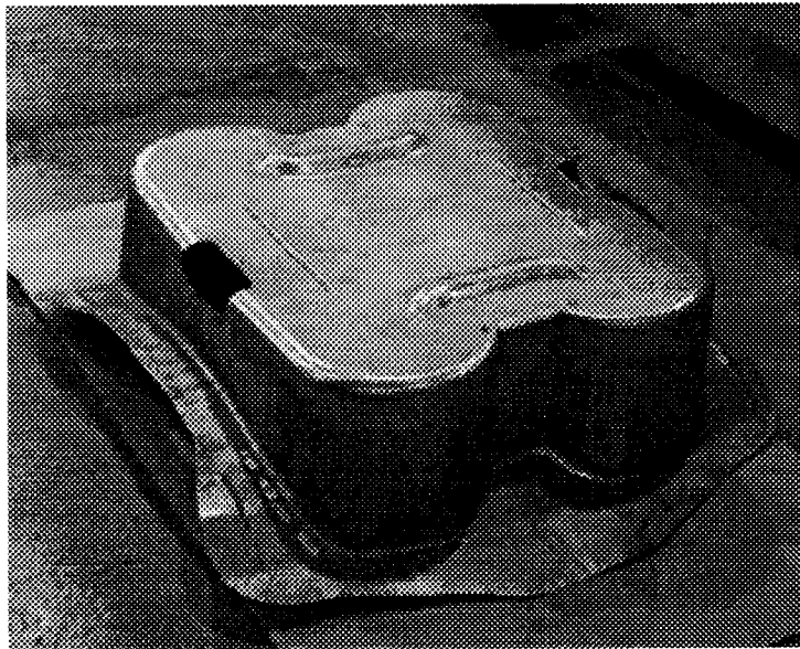
Figure 7. Shock towers after stamping
