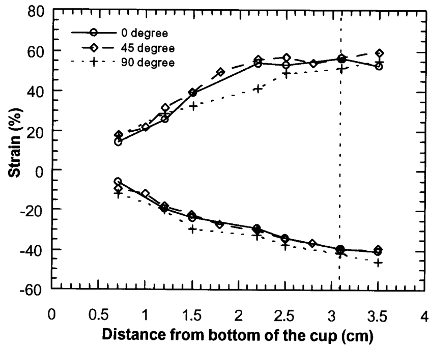
Figure 18. Strain in 2-inch cup wall with DR of 2.0 (steel S3, 0.74 mm thick).
