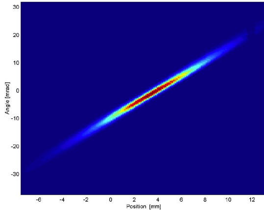
Figure 2 – Measured vertical RFQ emittance with a size of 0.260 \pi mm mrad, for a 20-mA beam.
