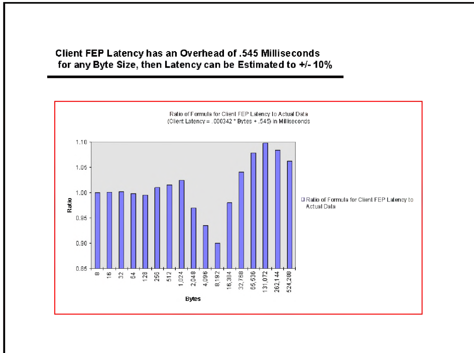
Figure 2-8. Client FEP latency can be estimated to +/- 10%.
