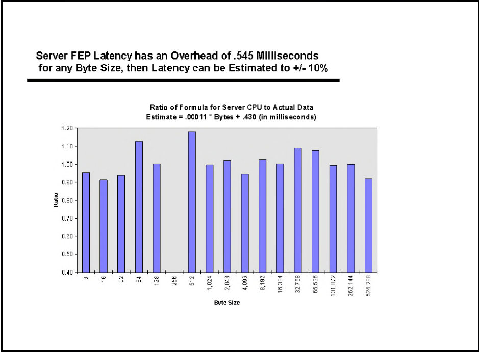
Figure 2-9. Server FEP latency can be estimated to +/- 10%.
