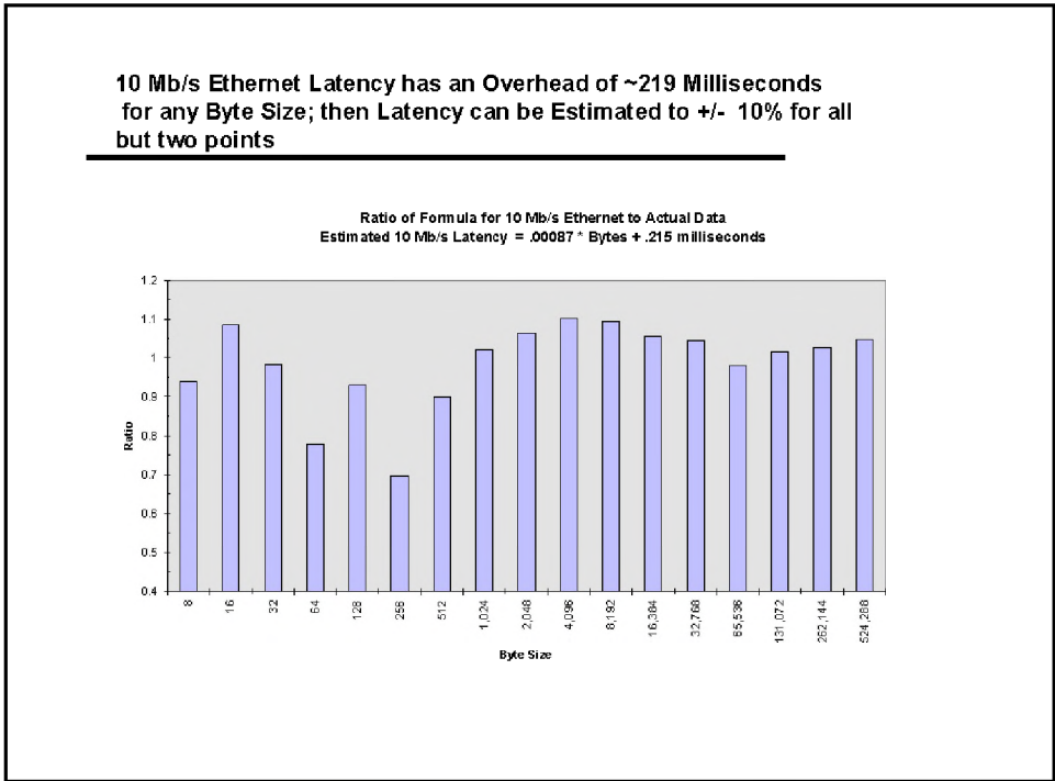
Figure 2-10. 10 Mb/s ethernet latency can be estimated to +/- 10% for all
