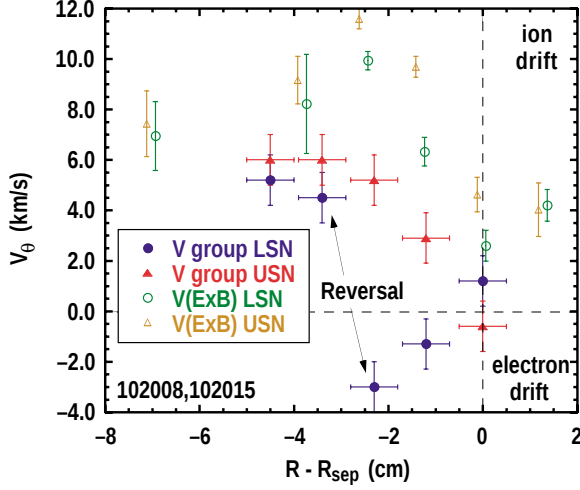
Fig. 3. Poloidal group velocity of the density fluctuations measured by BES and E_r \times B_T velocity determined from CER measurements.
