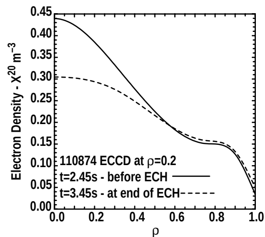
Fig. 5. Density peaking control with ECH 110874, 2.3 MW ECH at \rho \sim 0.2
