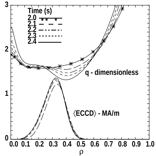
Fig. 3. q profile evolution at start of ECH for experiment design: 2.5 MW ECH at \rho=0.35 with fixed \chi , n_e , and Z_{\text{eff}}
