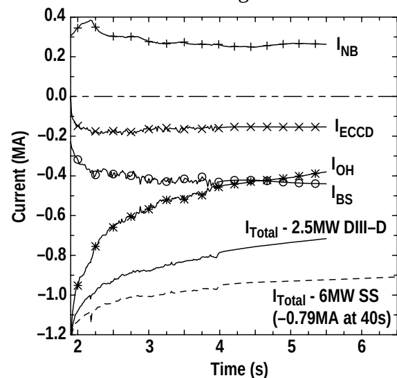
Fig. 2. Design simulation to explore steady-state operation. Solid curves for DIII-D condition at 2.5 MW. Dashed curve is 6 MW steady-state simulation to 40 s.
