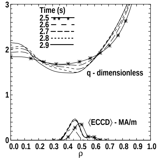
Fig. 4. Ohm's law analysis of 110854, 2.2 MW of ECH at \rho=0.45 , using measured density and temperature profiles.
