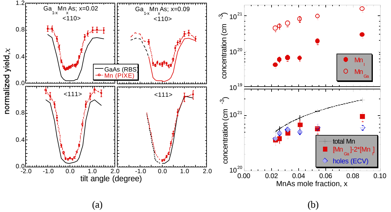
Figure 1. (a) Mn and GaAs angular scans about the <110> and <111> channels for Ga 1-x Mn x As alloys with x=0.02 and 0.09. (b) The concentrations of interstitial and substitutional Mn (top panel) and the net uncompensated Mn acceptor concentration ([Mn Ga ]-2x[Mn i ]) (lower panel) as measured by channeling experiments together with the hole concentration obtained by electrochemical capacitance-voltage (ECV) profiling for x ranging from 0.02 to 0.09.
