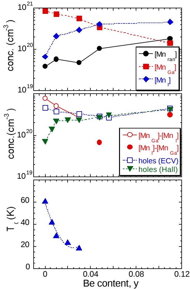
Figure 4. The concentration of Mn atoms in the various different lattice sites, as measured from the angular scans (a), the net uncompensated concentration of Mn ( [Mn_{Ga}] - [Mn_I] ) together with the hole concentration measured by ECV and Hall (b), and the Curie temperature T_C (c) for the Ga_{1-x-y}Mn_xBe_yAs films with increasing BeAs mole fraction y .
