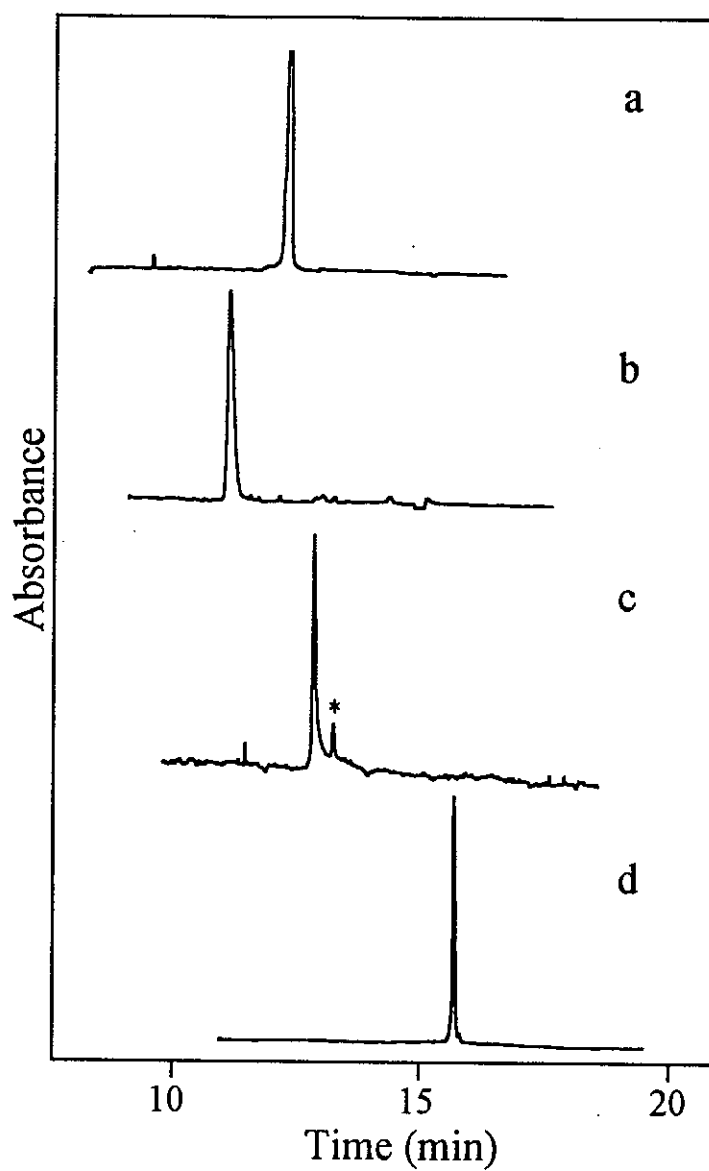
Figure A-3. Room-temperature absorbance electropherograms acquired during CE-separation of the HPLC pre-separated DB[a,I]PDE-derived adduct standards: a) (+)- trans-syn -DB[a,I]PDE-N 6 dA; b) (+)- cis-syn -DB[a,I]PDE-N 6 dA; c) (-)- trans-anti -DB[a,I]PDE-N 6 dA; and d) (-)- cis-anti -DB[a,I]PDE-N 6 dA. The asterisk marks an impurity in the trans-anti -dA adduct.
