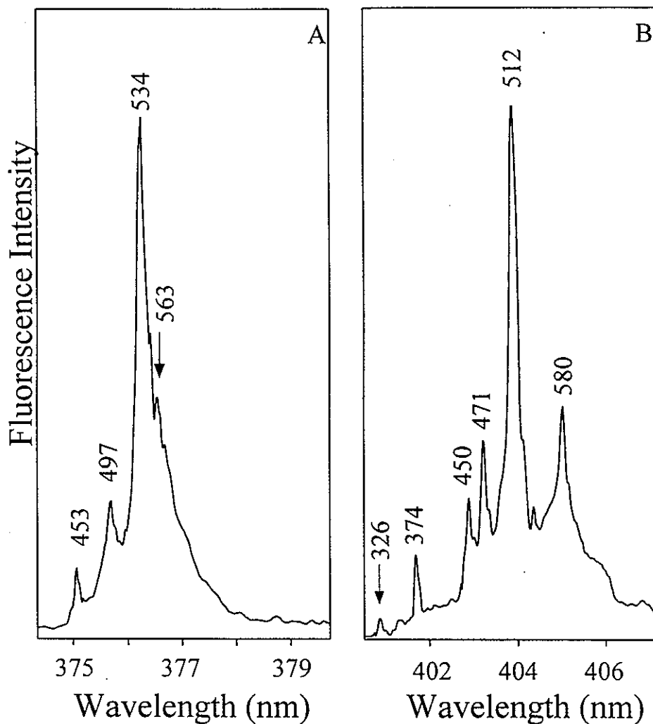
Figure 6-5. Frame A; On-line FLN spectrum of the peak at \sim 25 minutes in the chromatogram of Figure 6-2. The vibrational frequencies ( \lambda_{\text{ex}} = 368.9 nm) identify the peak at 25 minutes as B[e]P. The spectrum was taken at with a gate-width of 200 ns and a 0 ns delay time. Frame B; FLN spectrum of the peak at \sim 27 minutes in the chromatogram. The vibronic modes ( \lambda_{\text{ex}} = 395.7 nm) identify the 27-min peak as B[a]P; 200 ns gate-width, 20 ns delay. The vibronic modes are labeled with their excited-state frequencies, in \text{cm}^{-1} .
