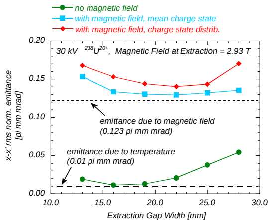
Figure 2: Ion beam emittance vs. extraction gap. Results of an IGUN simulation without and with axial magnetic field present.
