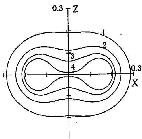
Fig. 9 The shapes of gas cavity at the end of compression stage in the case of initial perturbation: R(t=0, \theta)=1+0.05P_2(\cos(\theta)) .
