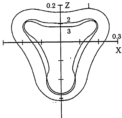
Fig. 11 The shapes of gas cavity at the end of compression stage in the case of initial perturbation: R(t=0, \theta)=1+0.05P_3(\cos(\theta)) .
