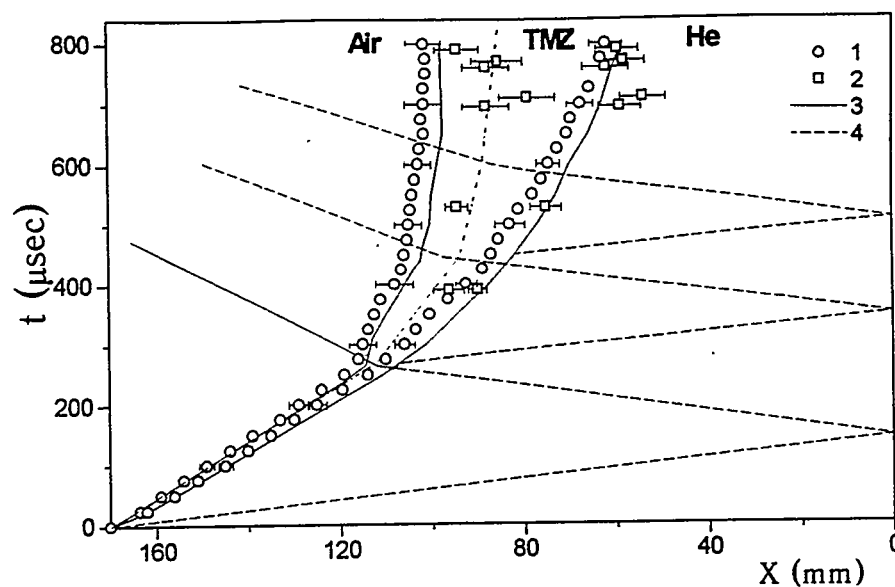
Fig.26. Flow x-t diagram in experiments using geometry as shown in fig. 22. Points- experimental results: 1- shadow technique; 2- laser knife. Solid curves- VIKHR calculations. Dashed and dot-dash lines - interface and shock-waves trajectories, respectively, calculated without turbulent mixing involved.
