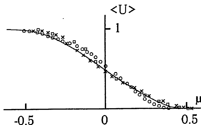
Fig.33. Averaged velocity profile. Direct 2D modeling of turbulent mixing in shear flows EGAK code ( task №1): □ - t=2.21 ; X - t=2.52 ; O - t=3.77 ; ——— -semiempirical model.
