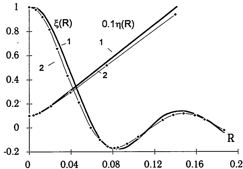
Fig 1. Plane shock front and interface perturbation amplitude versus travel paths of the shock front and interface, respectively..
