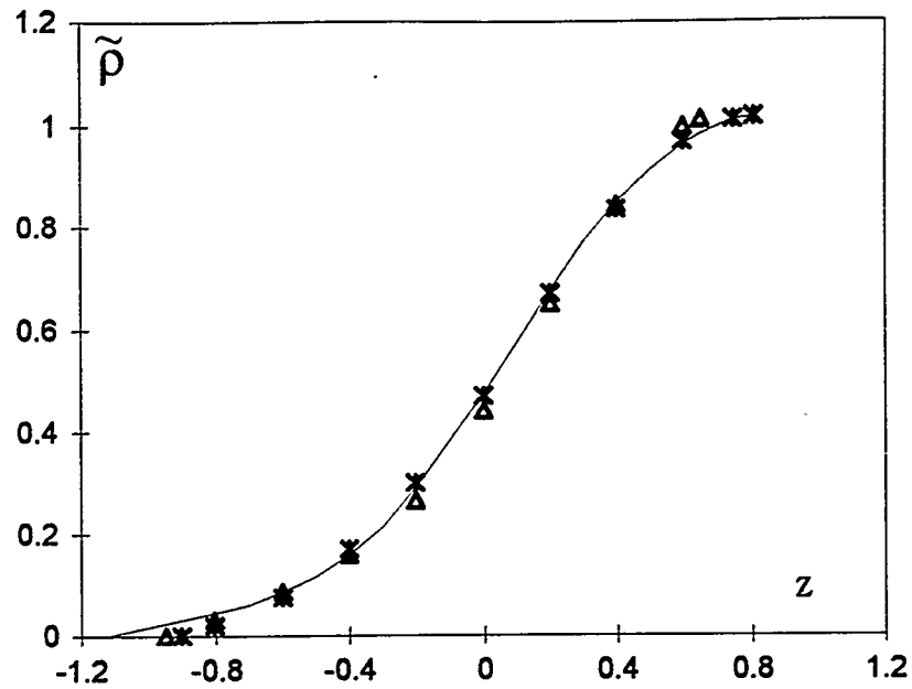
Fig.39. Self similar density profile. Gravitational turbulent mixing calculations. — - VIKHR code; x - e-Q model ( \delta=3 ); \Delta - e-Q model ( \delta=10 ).
