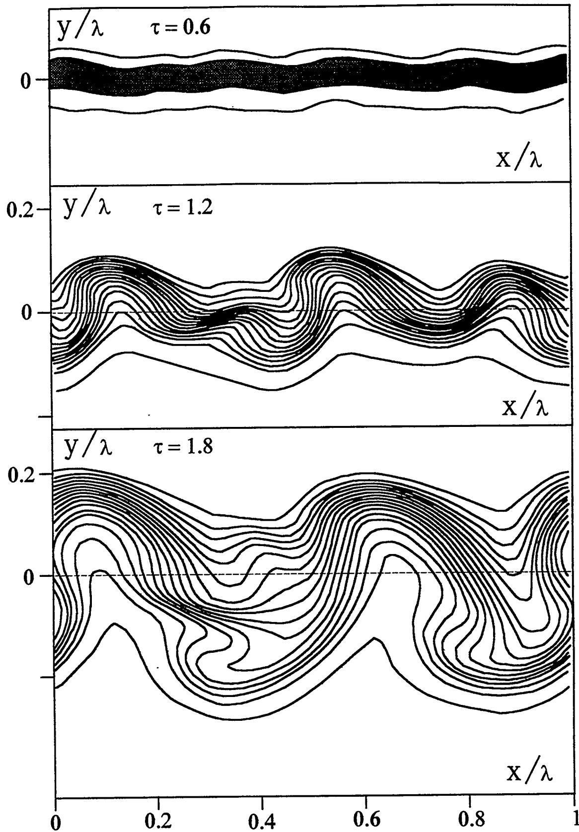
Fig.32. Direct 2D EGAK code modeling of turbulent mixing in shear flows. (problem № 4). Isodenses with \Delta\rho=0.667 .
