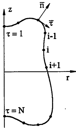
Fig.2. Contour shape description for BIE method.
