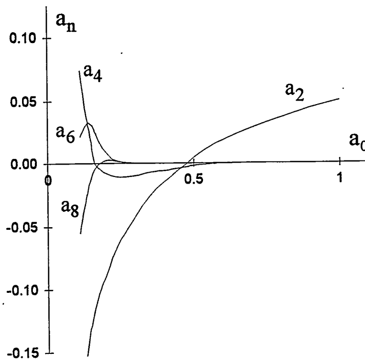
Fig.13. Harmonic amplitudes dependence on cavity radius a_0 . Initial perturbation was in the form r(t=0, \theta)=1+0.05P_2(\cos(\theta)) .
