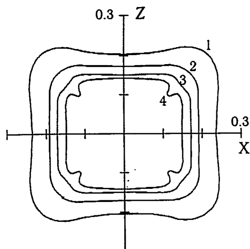
Fig. 10 The shapes of gas cavity at the end of compression stage in the case of initial perturbation: R(t=0, \theta)=1+0.05P_4(\cos(\theta)) .
