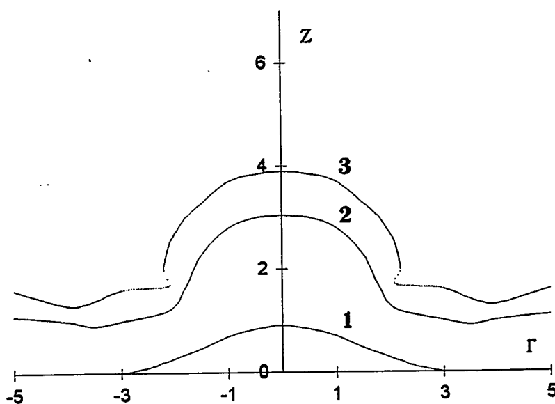
Fig.14. Local perturbation interface shapes calculated with BIE method at different moments. 1 - initial shape, 2 - t=1.5 , 3 - t=1.8 .
