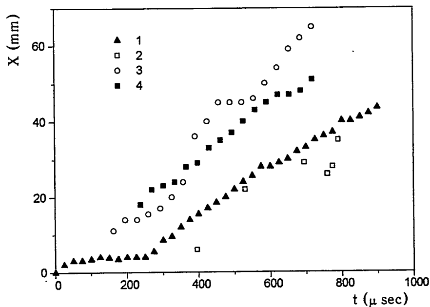
Fig.28. TMZ thickness vs. time for horizontal and vertical shock-tube experiments using different measurement techniques. Horizontal shock-tube experiments with thin-film gas separation. 1 - data obtained by shadow technique and averaged for 9 experiments (system sensitivity is below critical); 2 - laser knife measurements (each point represents an individual experiment); 3 - shadow visualization, for sensitivity above critical value; 4 - vertical shock-tube experiment, for short time delay t_{\text{del}} \approx 2 \div 13 ms.
