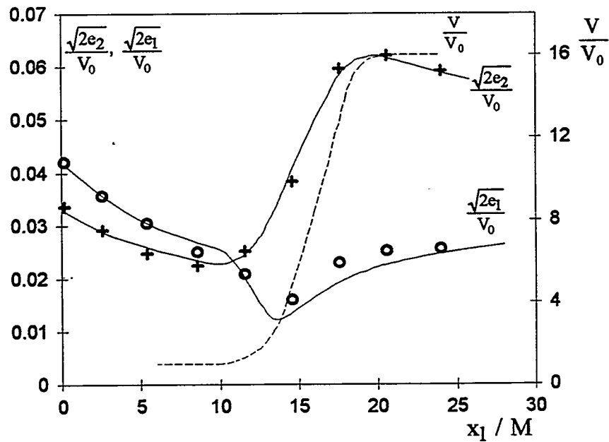
Fig.50. Values of \sqrt{e_1}/V_0 , \sqrt{e_2}/V_0 , V/V_0 as function of x_1/M for S_1/S_2=16 .
