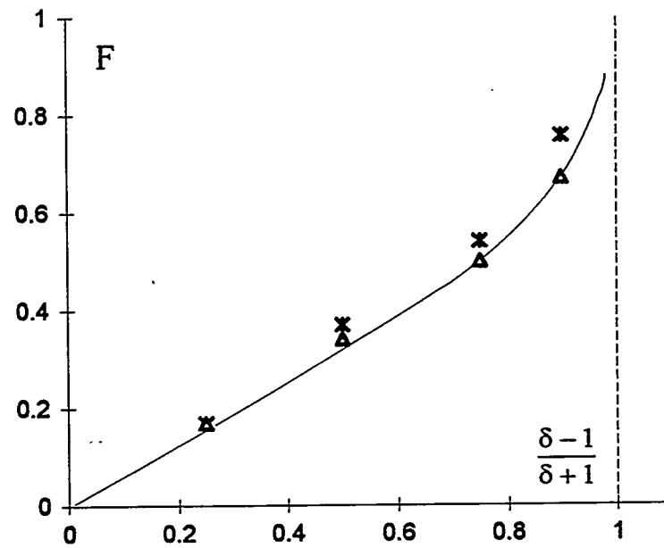
Fig.38. Value F dependence on Atwood number.
