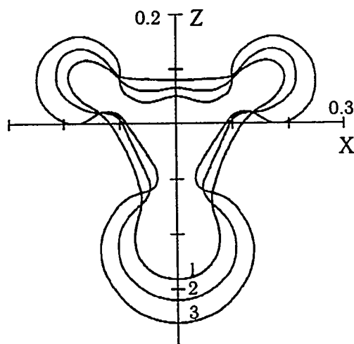
Fig. 12 The shapes of gas cavity in the beginning of expansion stage in the case of initial perturbation: R(t=0, \theta)=1+0.05P_3(\cos(\theta)) .
