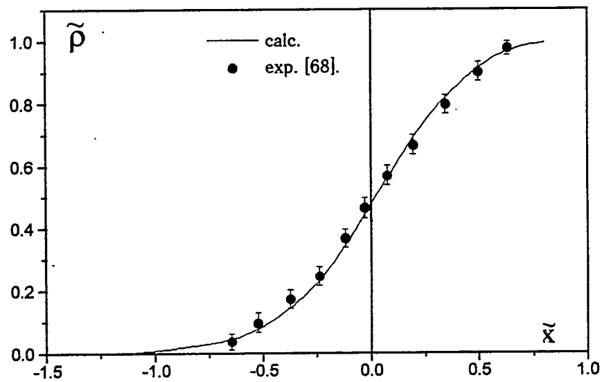
Fig.52. Density profile in self-similar problem.
