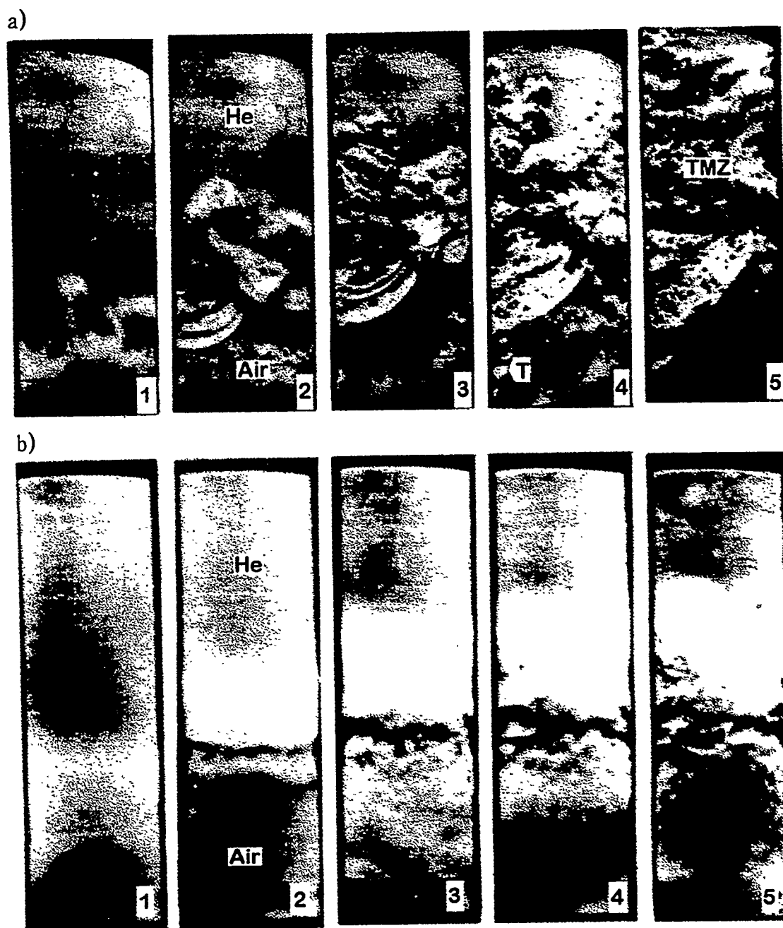
Fig. 25 Turbulent zone development in vertical shock tube experiments: a) time delay t_{del} \sim 2 \div 13 mc; b) time delay t_{del} \sim 1 c. TMZ - turbulent mixing zone; T - "train".
