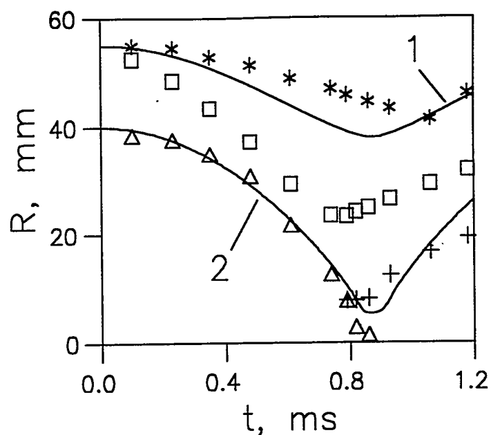
Fig. 49. R - t diagram of collapsing jelly ring. 1, 2-outer and inner ring surfaces (regular hydrodynamic calculation), *, \square - mixing zone surfaces at outer boundary, +, \Delta - mixing zone surfaces at inner boundary of the ring (jelly ring experiment of \sim 0.1 \text{ kg/cm}^2 strength).
