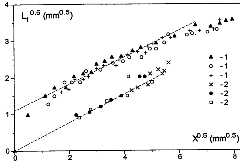
Fig. 58. \sqrt{L_1} as function of \sqrt{X} . 1 - one layer experiments; 2 - two layer experiments; (the second layer accelerated by the compressed air).
