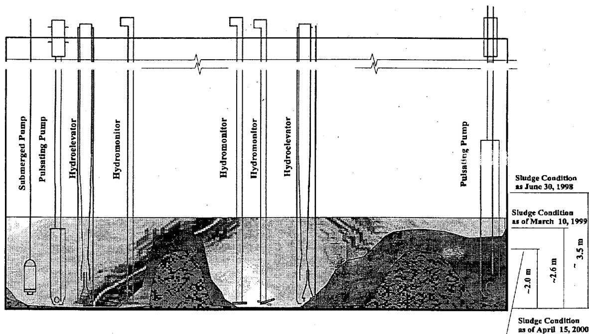
Fig. 2. Illustration of the condition of sludges in a 3200-m 3 tank as a function of time.
