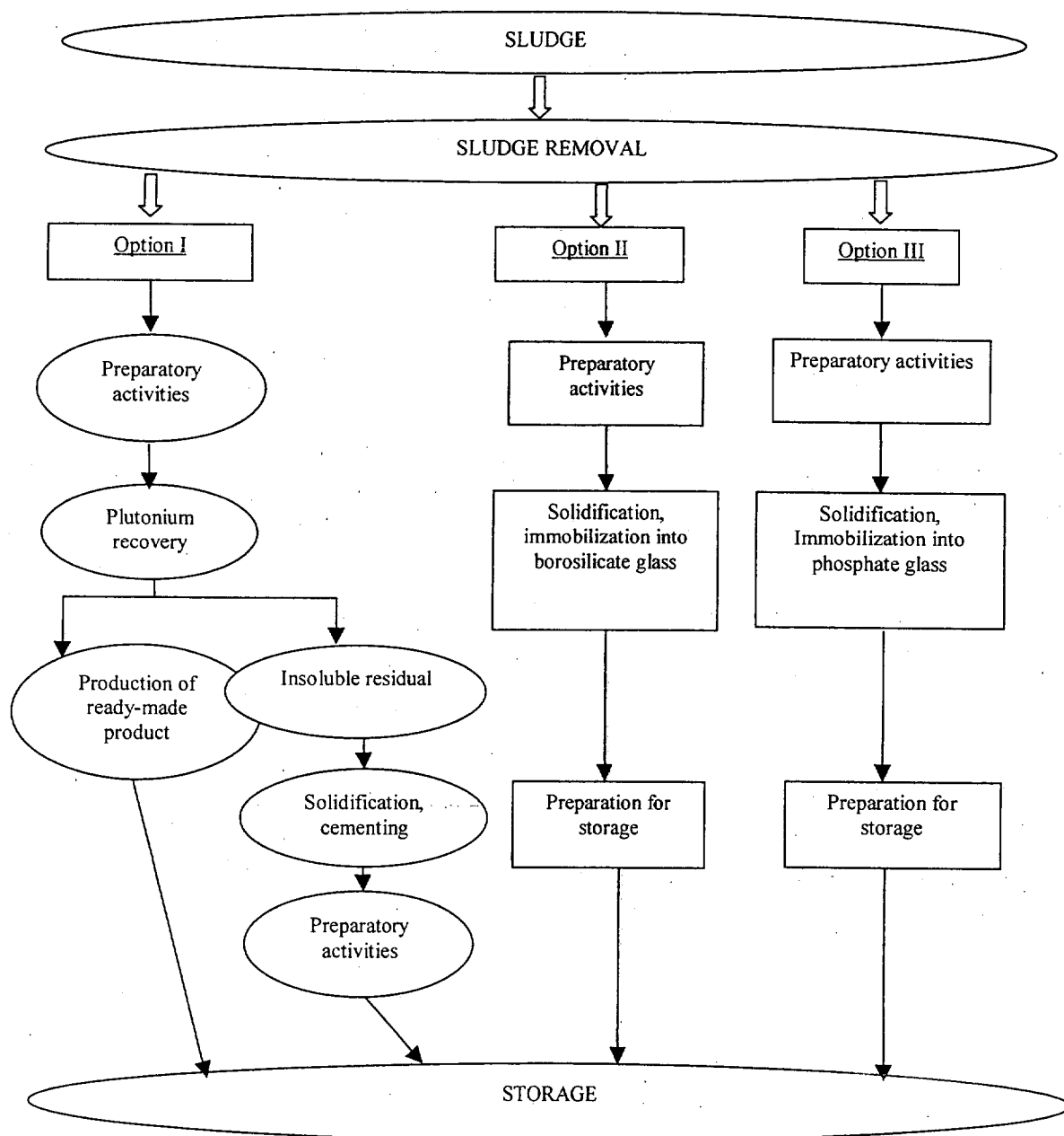
Fig. 1. Schematic diagram of Pu-sludge processing.
