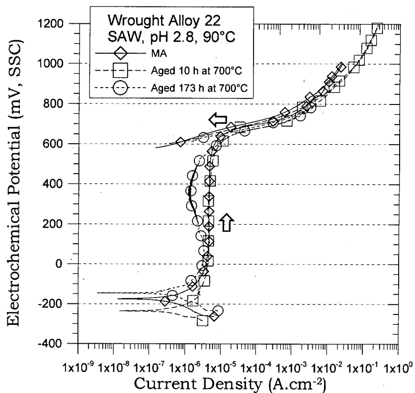
FIGURE 4: Cyclic polarization curve of Alloy 22 in SAW at 90^{\circ}\text{C} .
