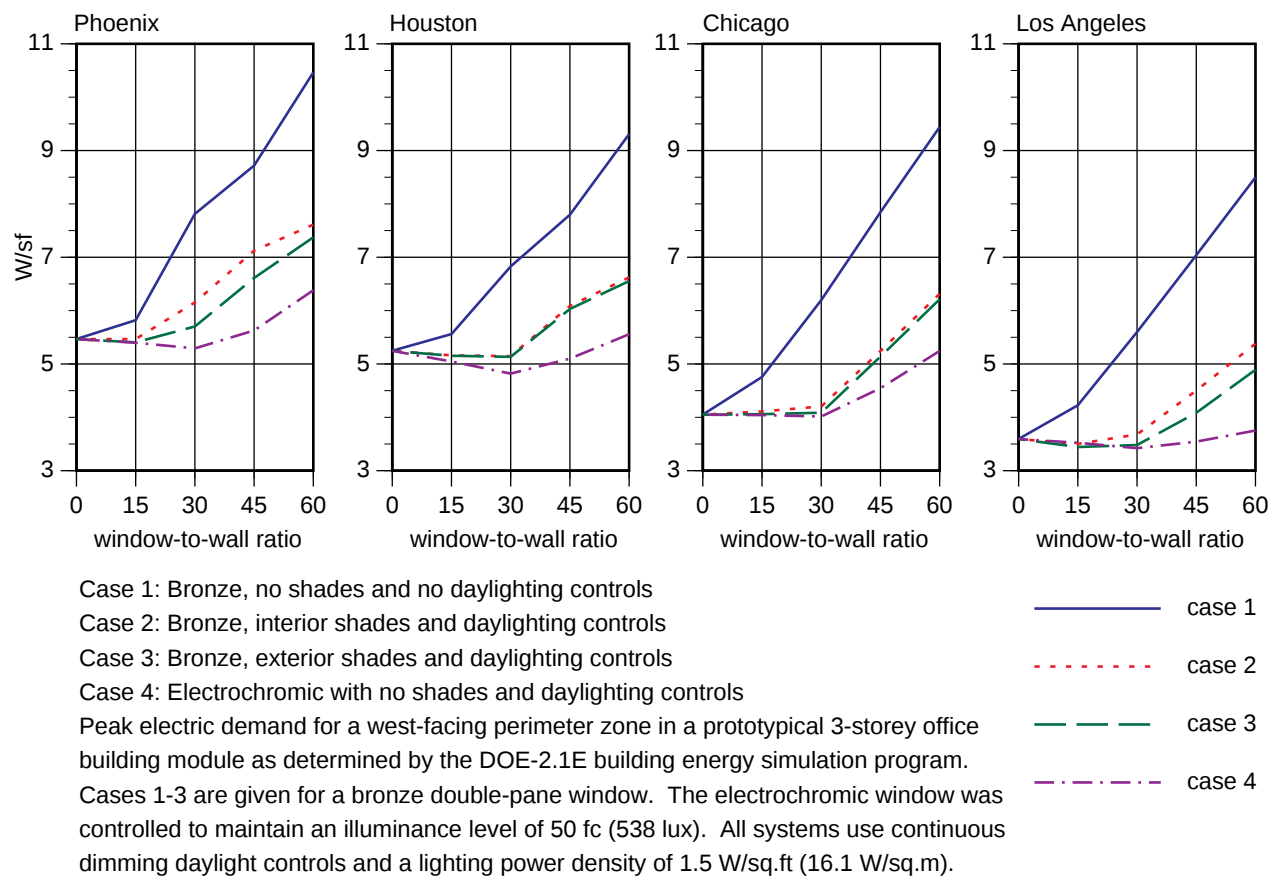
Figure 1. Peak electric demand ( \text{W}/\text{ft}^2 ) for a west-facing perimeter zone
