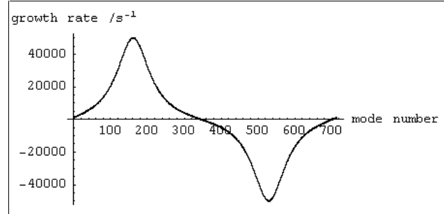
Figure 5: Coupled-bunch growth rates resulting from the electron cloud long-range wake.
