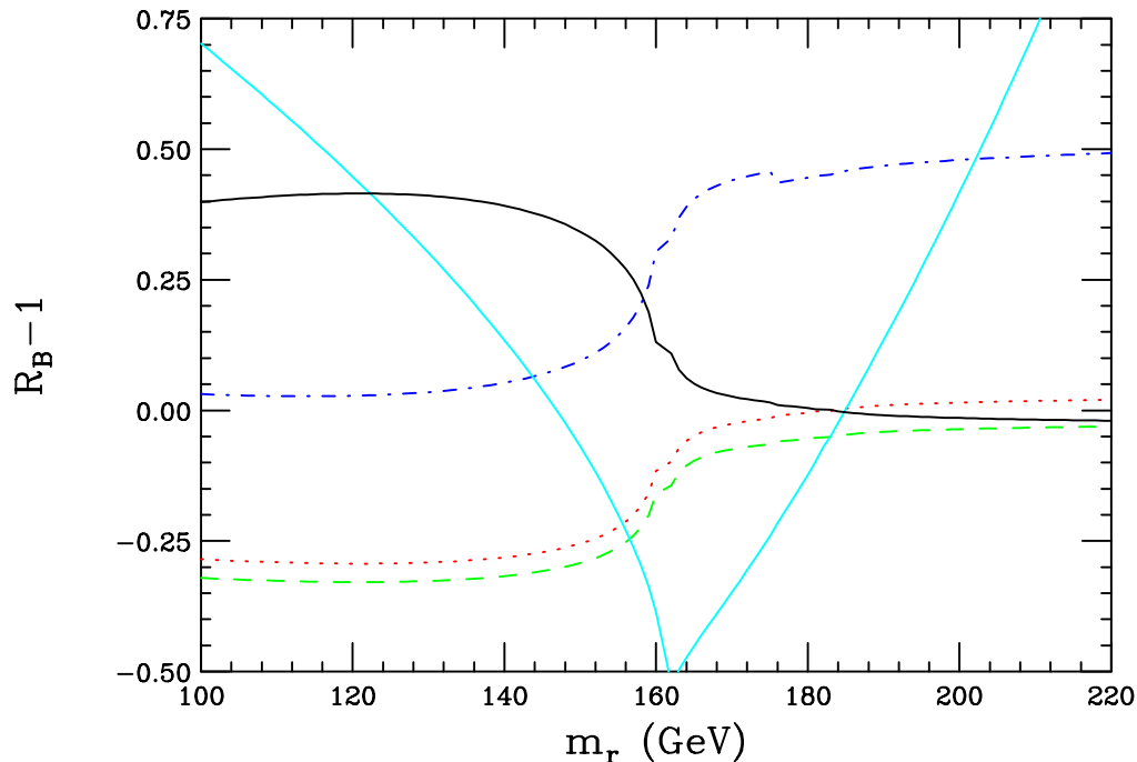
Figure 2: The ratios for the branching ratios of the radion into bulk states versus the corresponding wall states as a function of the radion mass. The approximately horizontal curves are, from top to bottom on the left-hand side of the figure, for the total width(solid), and the gg (dash-dotted), \bar{b}b (dots) and W^+W^-/ZZ (dashes) final states. The V-shaped curve is for the \gamma\gamma final state. Radion decay to Higgs boson pairs has been neglected. The values of \Lambda_r and k/M_{pl} are as in the previous figure.
