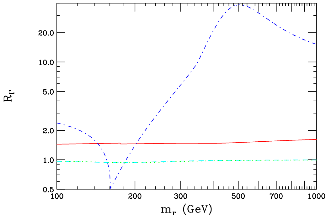
Figure 1: The ratios for the partial widths of the radion into SM fields when they are bulk states versus the corresponding case when they are wall states as a function of the radion mass. The solid(dashed-dotted, dashed,dotted) curve is for the gg(\gamma\gamma, W^+W^-, 2Z) final state. \Lambda_r , whose value only influences the radion decays to massive gauge bosons, has been taken to be 1.5 TeV along with k/M_{pl} = 0.1 . No alteration occurs in the case of \bar{f}f or two Higgs boson final states, i.e. , R_\Gamma(\bar{f}f, hh) = 1 .
