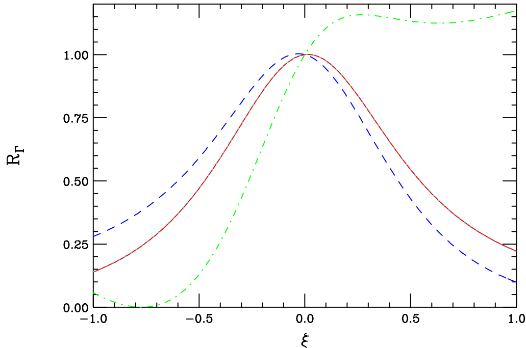
Figure 3: The effect of mixing on the partial widths of a 125 GeV Higgs boson, described by the parameter \xi , assuming v/\Lambda_r = 0.2 and a radion mass of 300 GeV as discussed in the text. The solid(dash-dotted, dashed, dotted) corresponds to the W^+W^-/2Z(gg, \gamma\gamma, \bar{f}f) final states.
