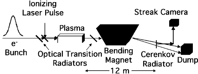
FIG. 2. Schematic of the experimental set-up. Not shown are two 75 m beryllium windows (located between the upstream OTR foil and the SiO_2 pellicle, and after the downstream OTR foil) that isolate the linac vacuum from the plasma chamber.
