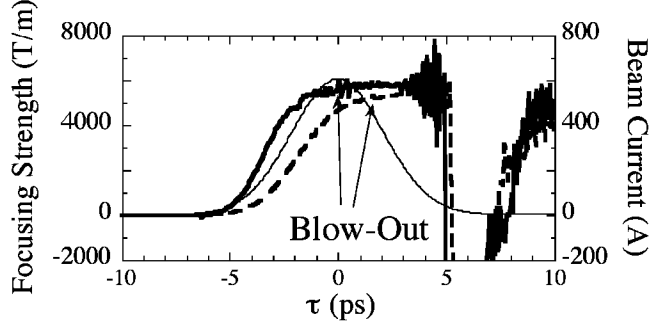
FIG. 1. Transverse focusing strength of the wake excited by an electron bunch (thin line) with the parameters of Table 1 with \sigma_r = 35\mu m (continuous line) and \sigma_r = 70\mu m (dashed line) in a plasma with n_p = 2 \times 10^{14} cm^{-3} as obtained from PIC numerical simulations. The peak defocusing field strength is greater than -16000 T/m at \approx 5.5 ps (not visible).
