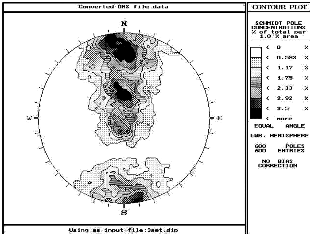
Figure 3-39 Contour Plot of Test Data with Three Fracture Sets
