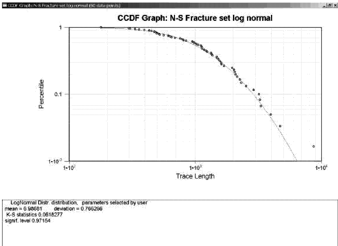
Figure 3-148 Trace Length Distribution, NS Lineaments
