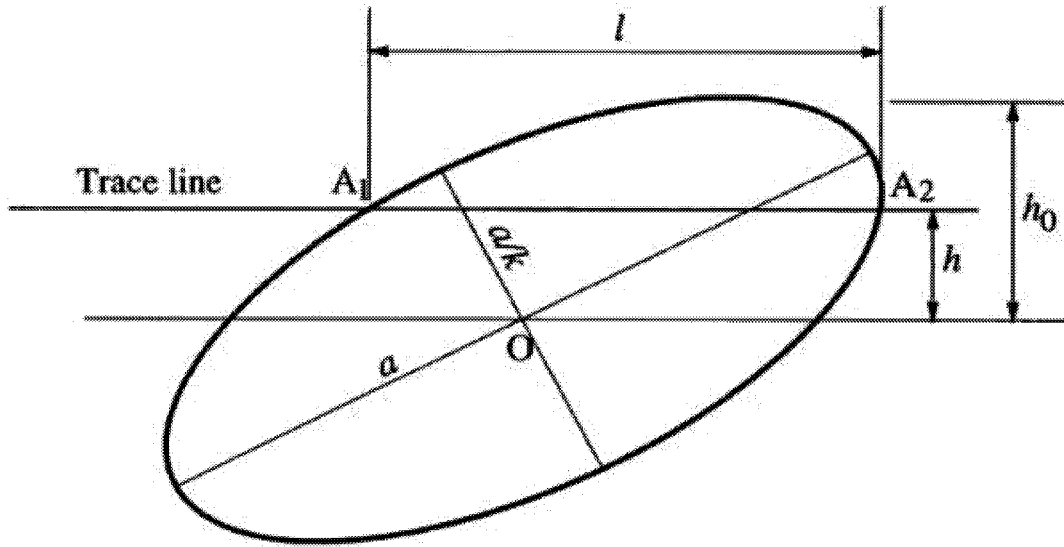
Figure 3-17 Relationship between h , l , and a
