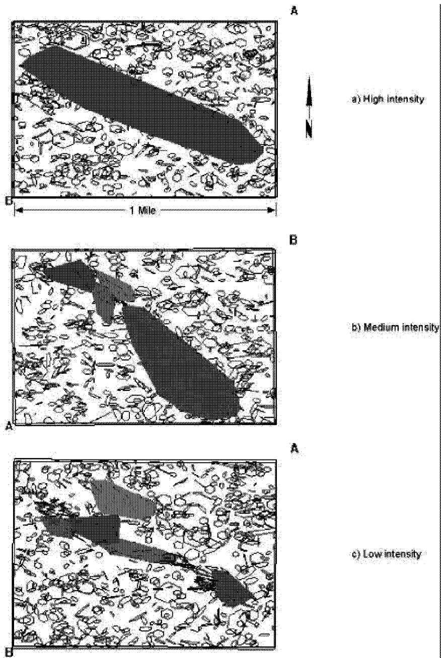
Figure 3-101 Compartments in Stoney Point DFN
