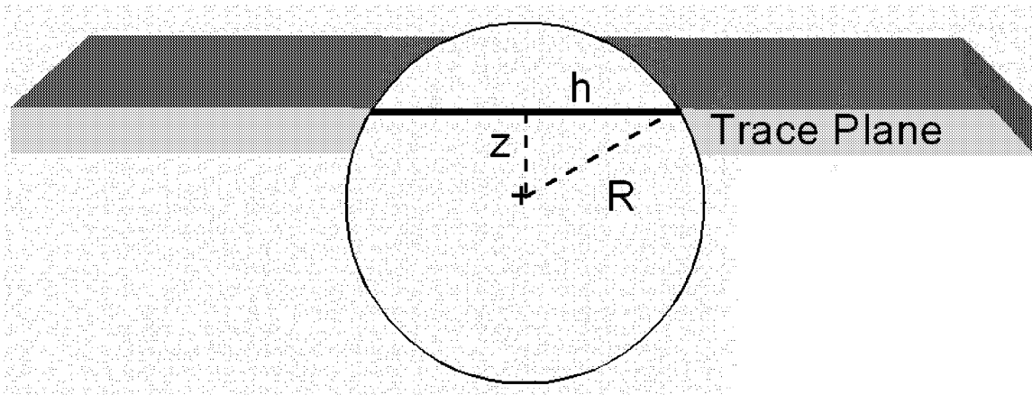
Figure 3-44 Fracture Intersection with Trace Plane
