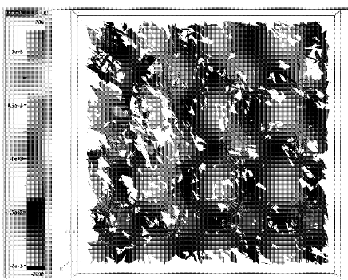
Figure 3-172: North Oregon Basin DFN model before gel treatment
