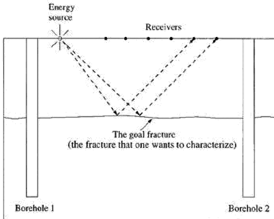
Figure 3-3 VSP Identification for Fracture Size
