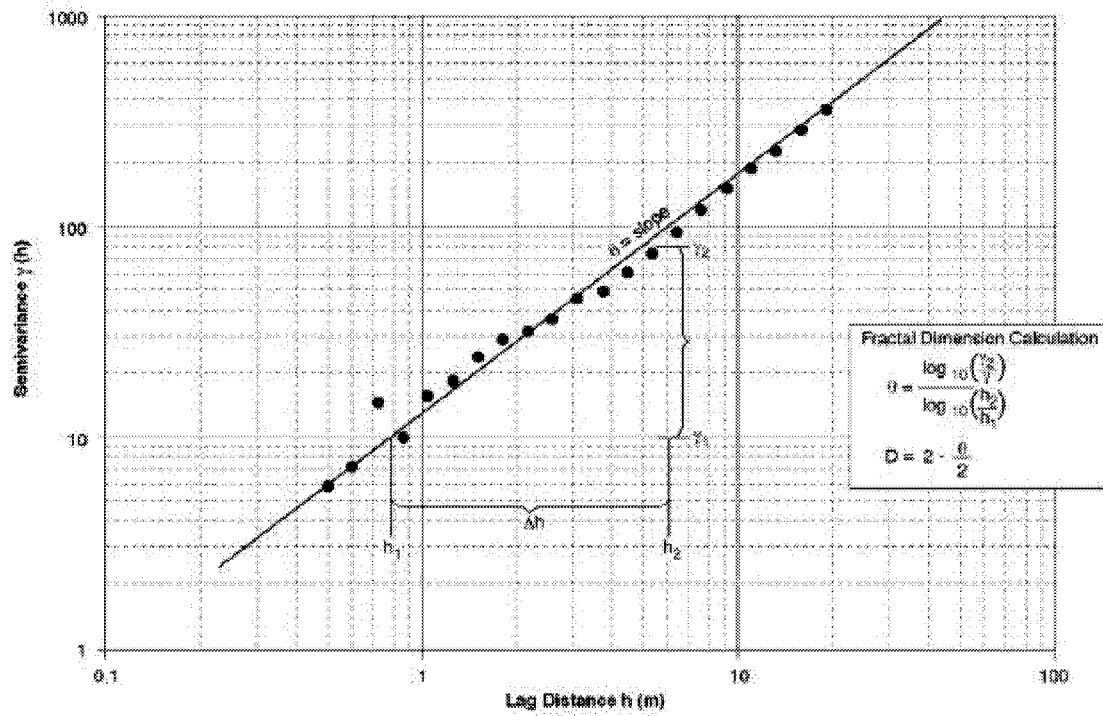
Figure 3-58 Fractal Dimension Calculation
