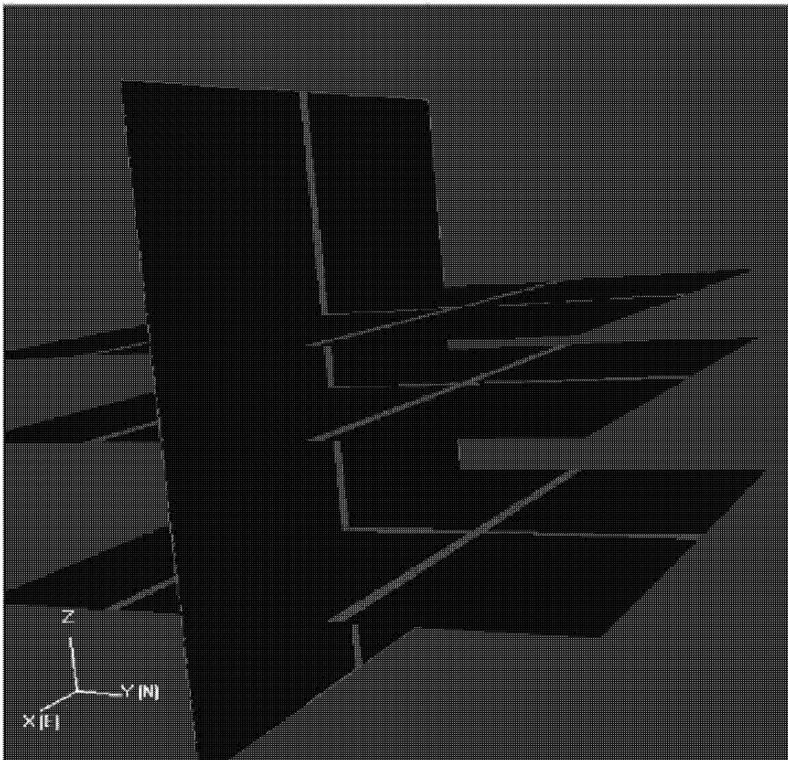
Figure 3-50 Channels in Faults and Fractures
