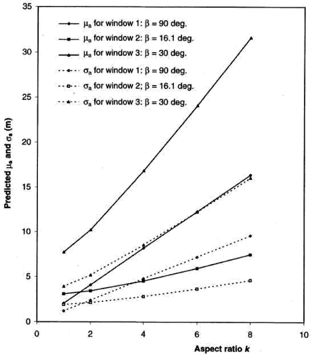
Figure 3-26 Variation of \mu_a and \sigma_a with aspect ratio k for assumed major axis orientation 1 ( 0^\circ/0^\circ ): assuming a Gamma distribution form of g(a)
