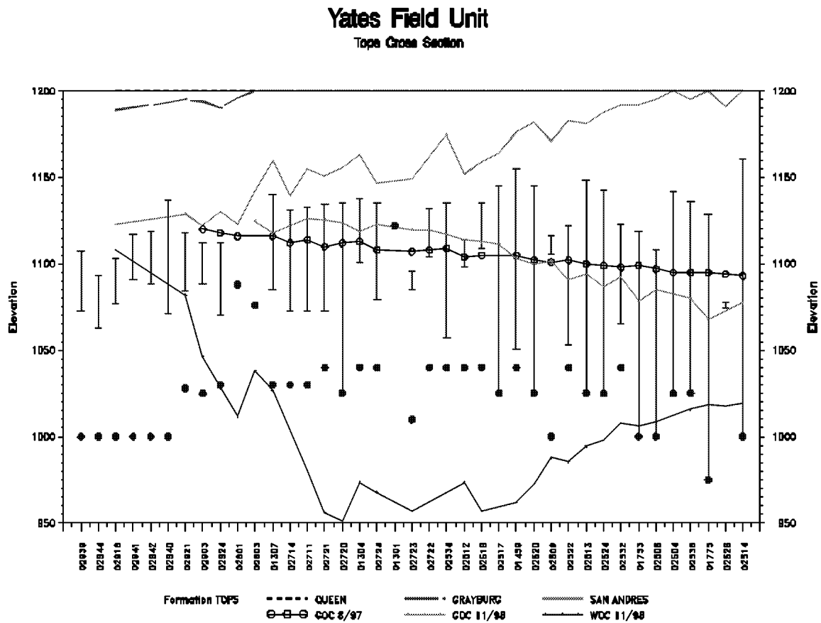
Figure 3-62 Yates Tops Cross Section
