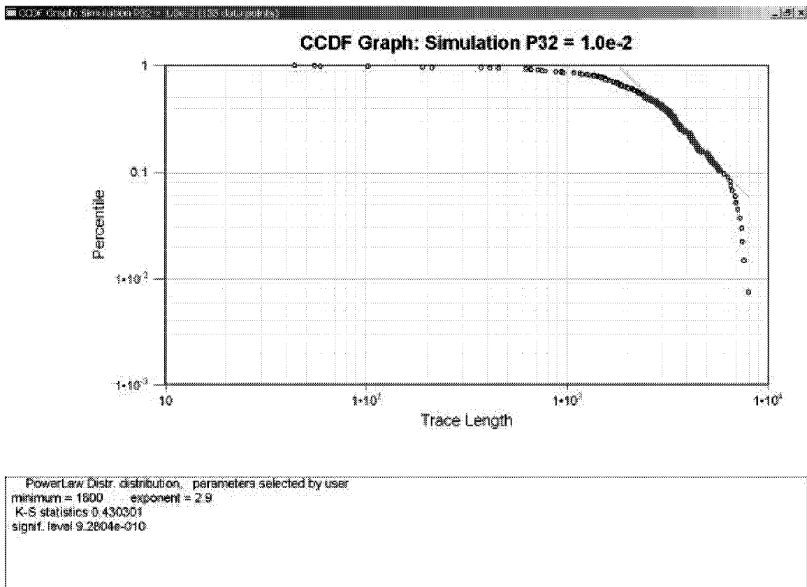
Figure 3-159: Simulation of ESE Lineaments, Intensity P_{32} = 0.01 \text{ m}^2/\text{m}^3
