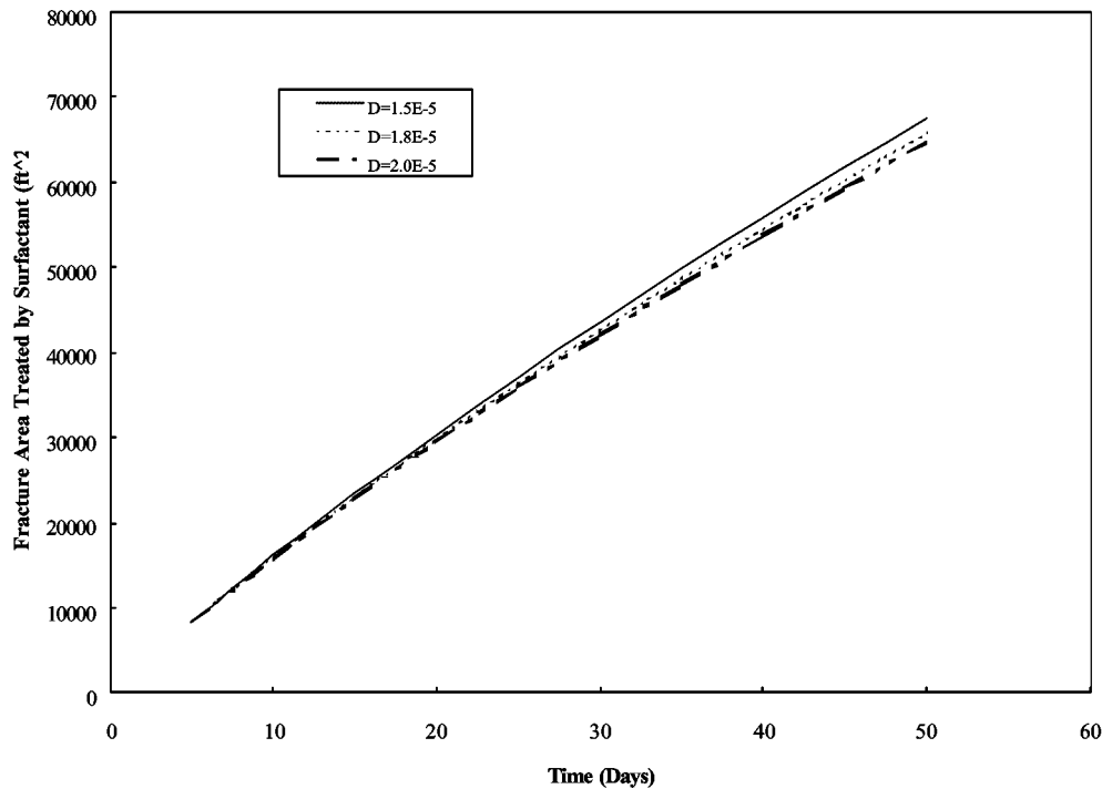
Figure 3-86 Effects of Molecular Diffusion on Fracture Area Treated
