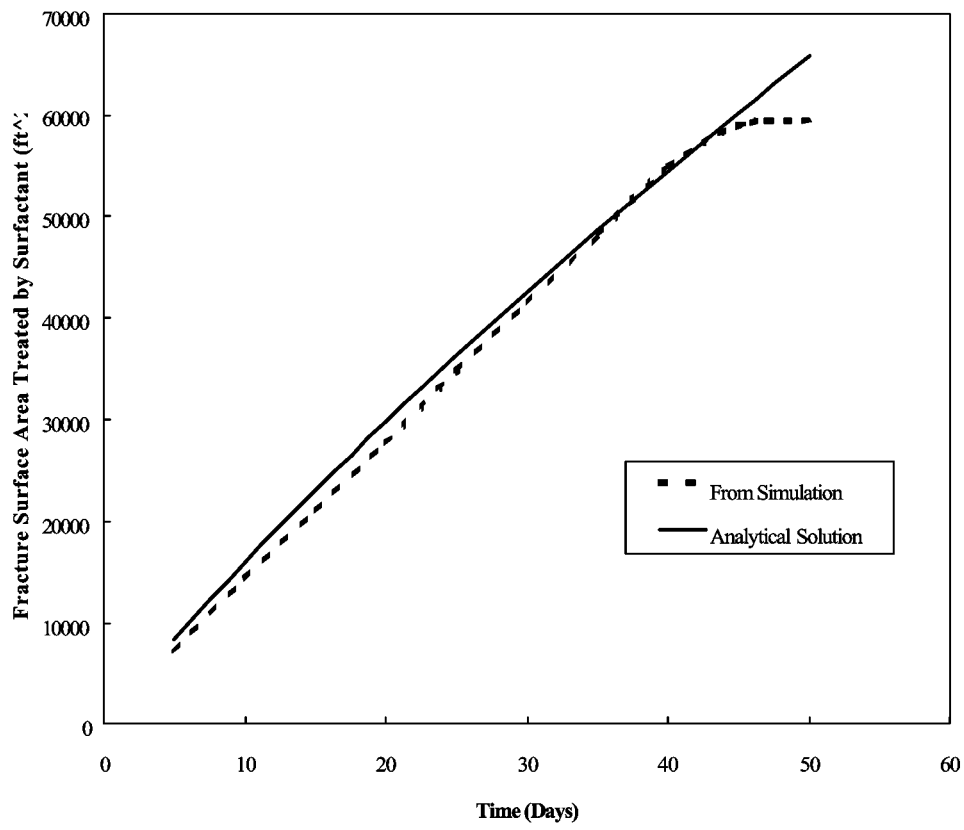
Figure 3-84 Comparison of Results from Simulation and Analytical Model
