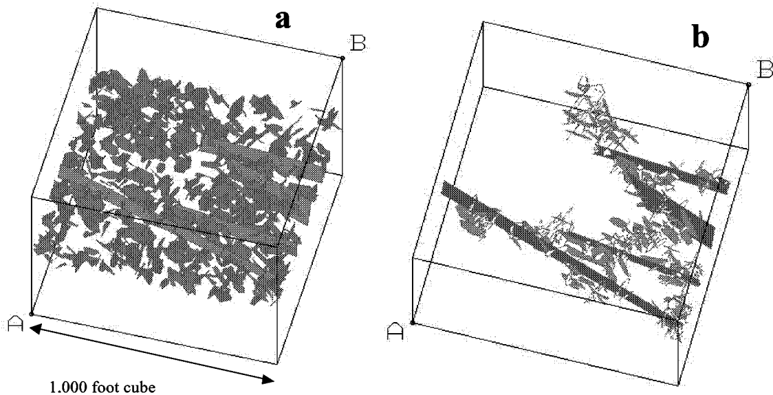
Figure 3-77 DFN Model Illustrating Surfactant Imbibition
