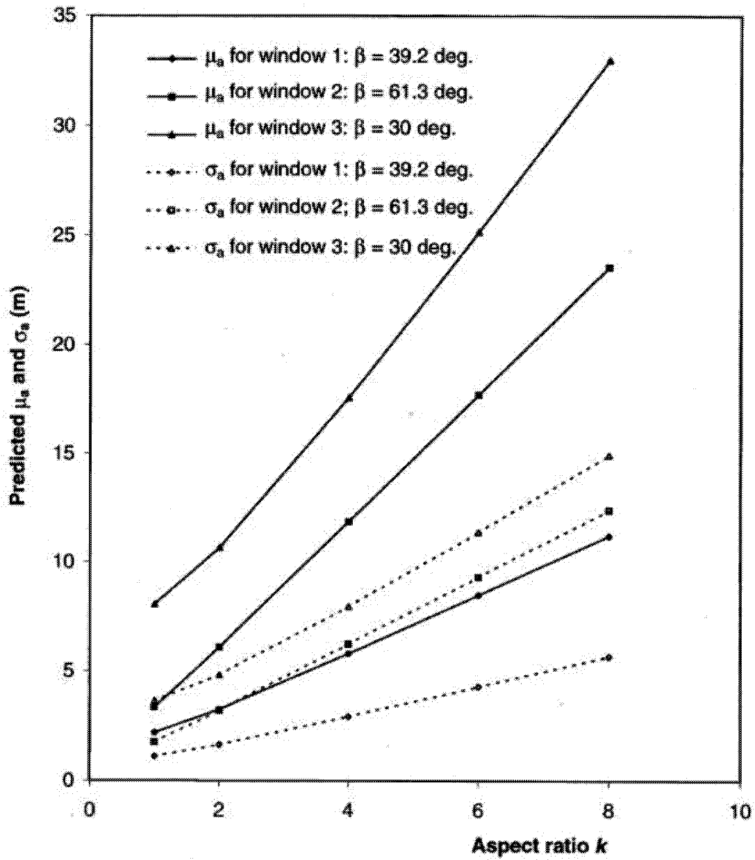
Figure 3-30 Variation of \mu_a and \sigma_a with aspect ratio k for assumed major axis orientation 3 ( 60^\circ/0^\circ ): assuming a lognormal distribution form of a
