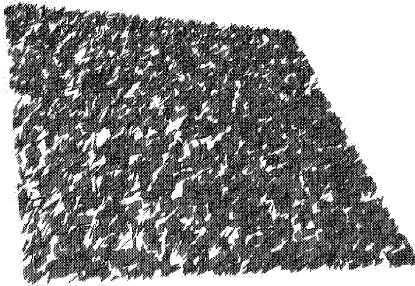
Figure 3-162: Matrix Discrete Features for South Oregon Basin Simulation
