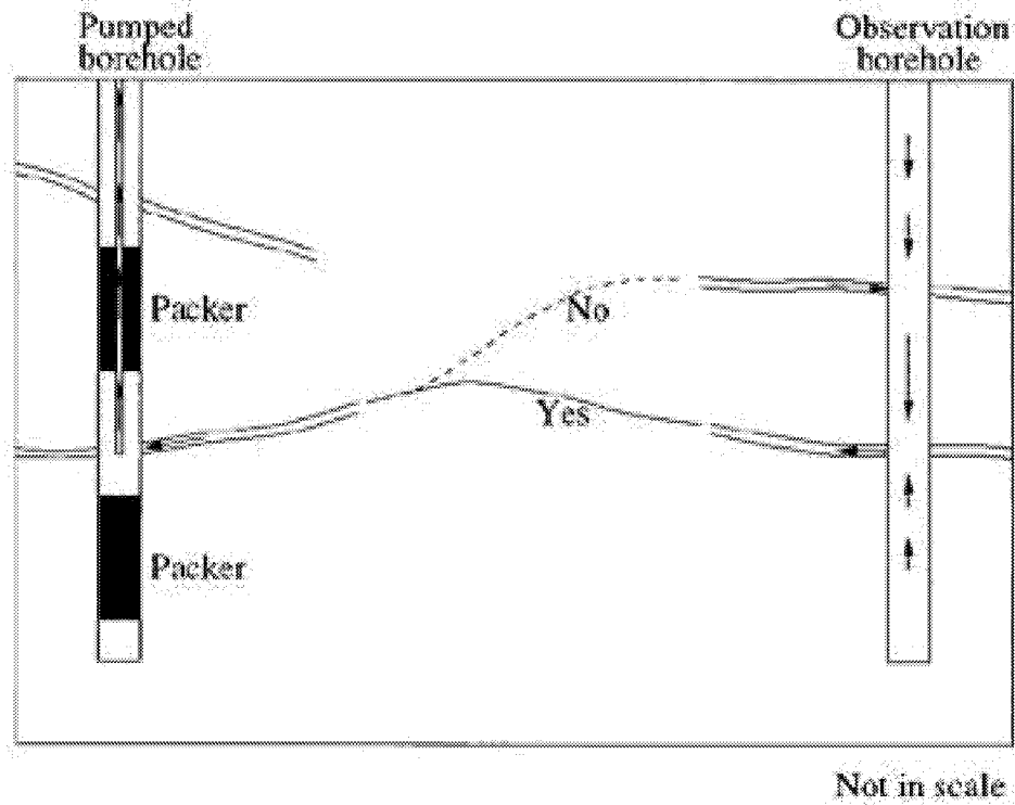
Figure 3-12 Fracture Network Effects
