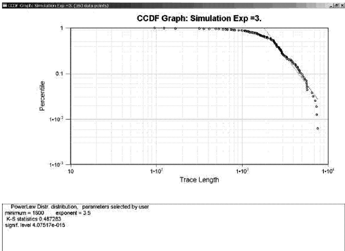
Figure 3-156: Simulation of ESE Lineaments, Exponent 3
