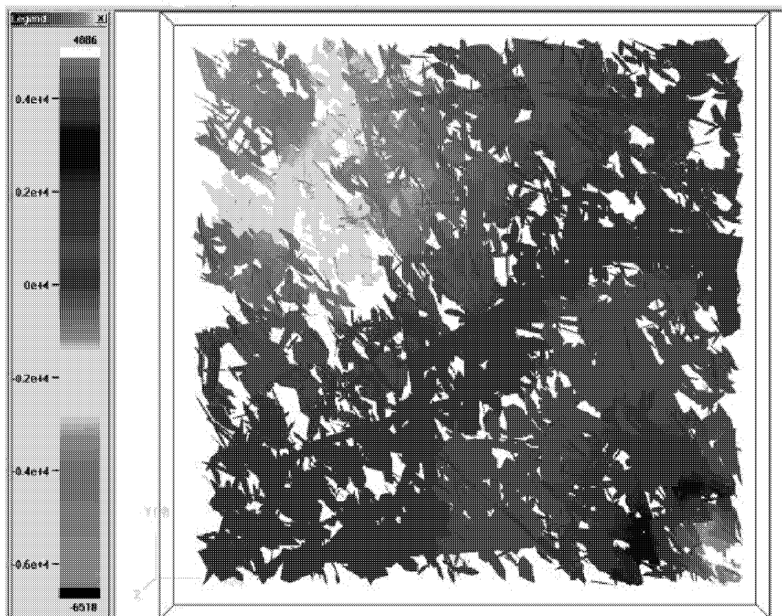
Figure 3-173: North Oregon Basin DFN model after gel treatment
