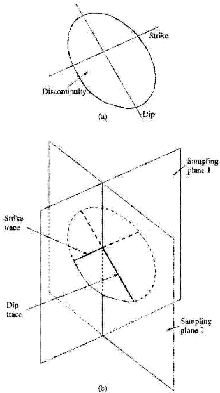
Figure 3-34 (a) Strike and dip of a discontinuity; and (b) Strike and dip traces
