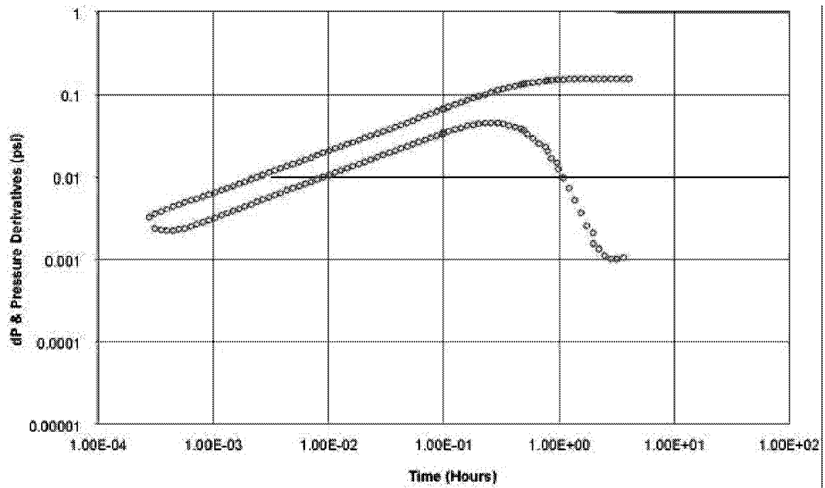
Figure 3-52 Productivity Test with Single Channel, Well on Channel
