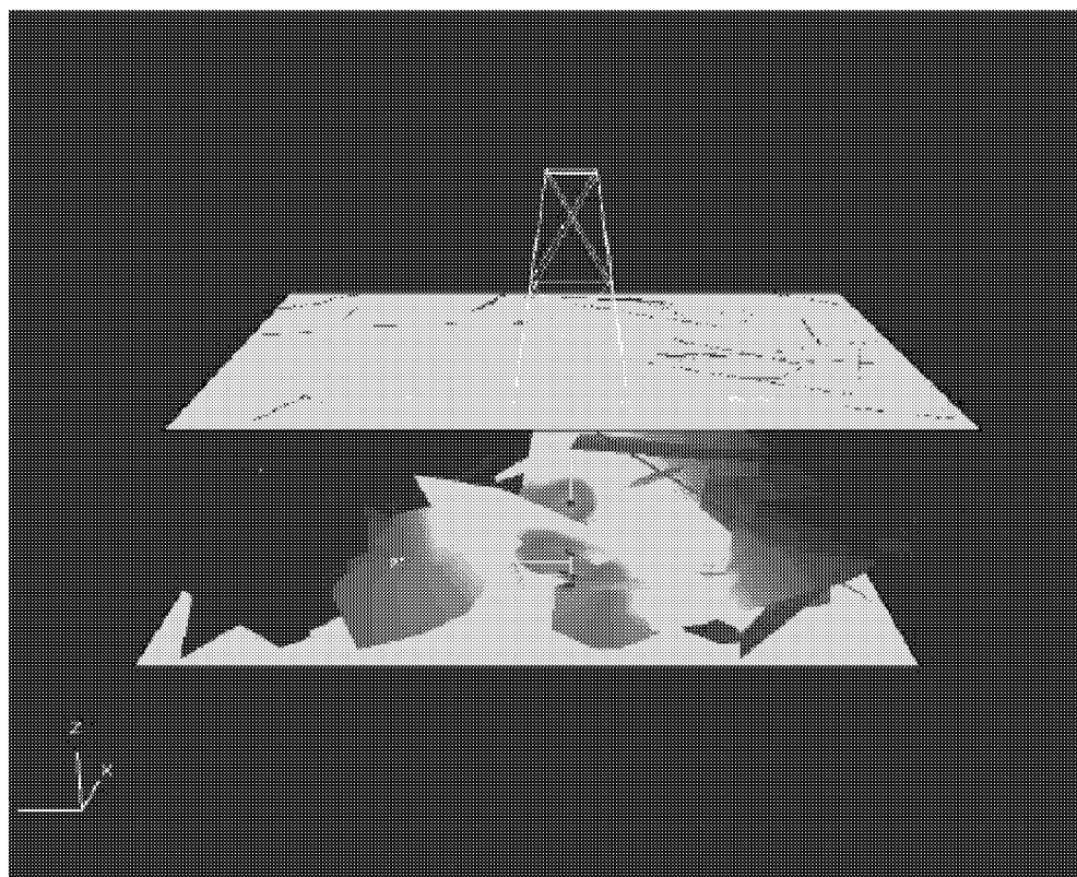
Figure 3-72 Geomechanical Modeling of 3D Fracture Populations
