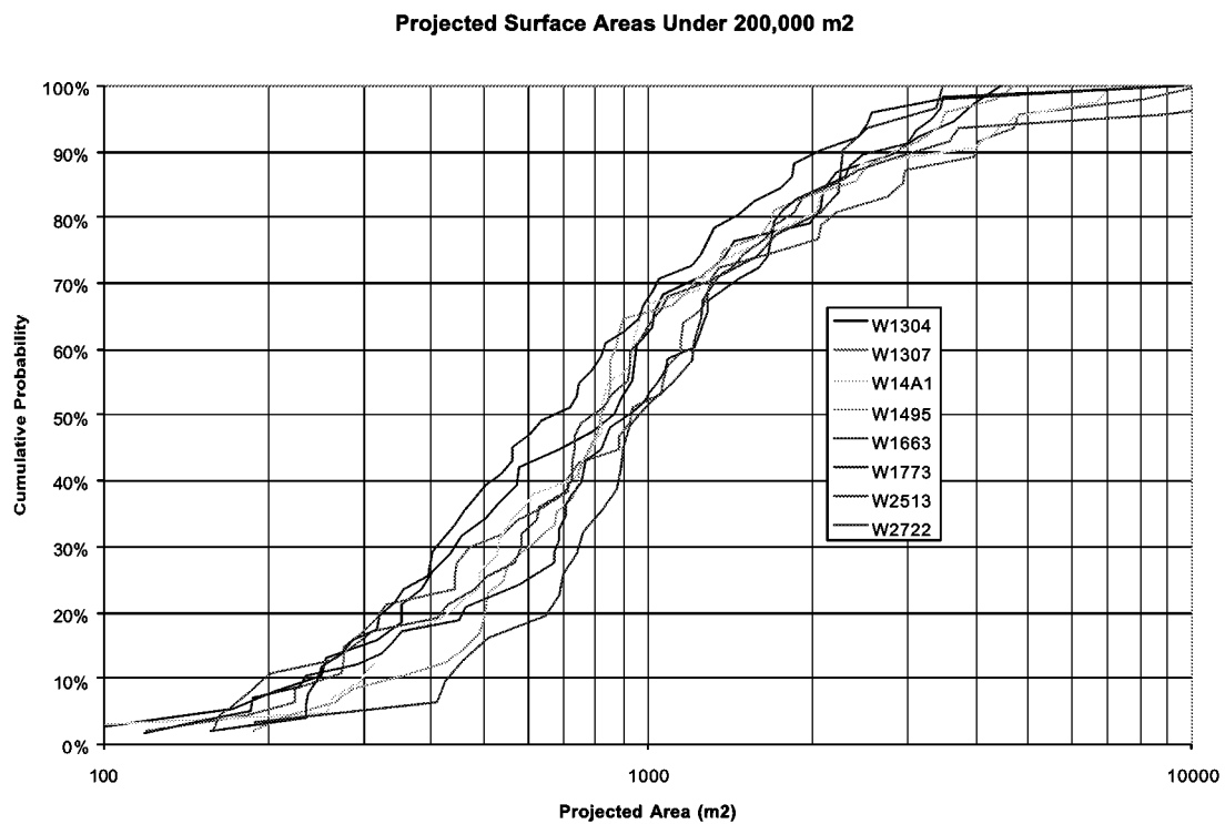
Figure 3-91 Compartment Projected Area Distribution, Yates Deepening Candidates
