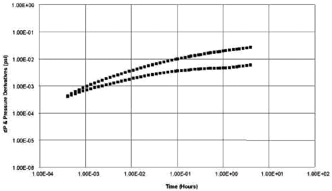
Figure 3-54 Production Test with Single Channel, Well in Background Fractures
