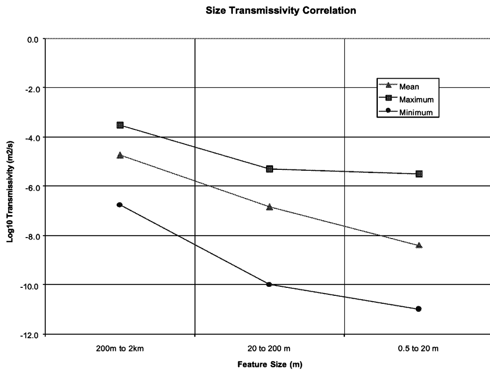
Figure 3-55 Size Transmissivity Relationship at Äspö Sweden
