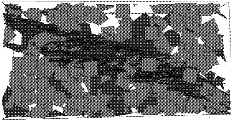
Figure 3-132: Simulation Volume (800x400x189m ) Stoney Point DFN Model (Fractures and Matrix Features)
