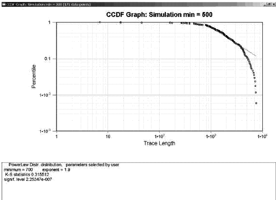
Figure 3-151: Simulation of ESE Lineament, 500 ft. Scale
