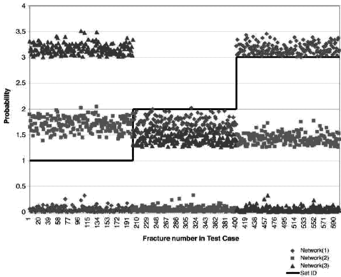
Figure 3-40 Neural Net Performance Results for 3 Set Test Case
