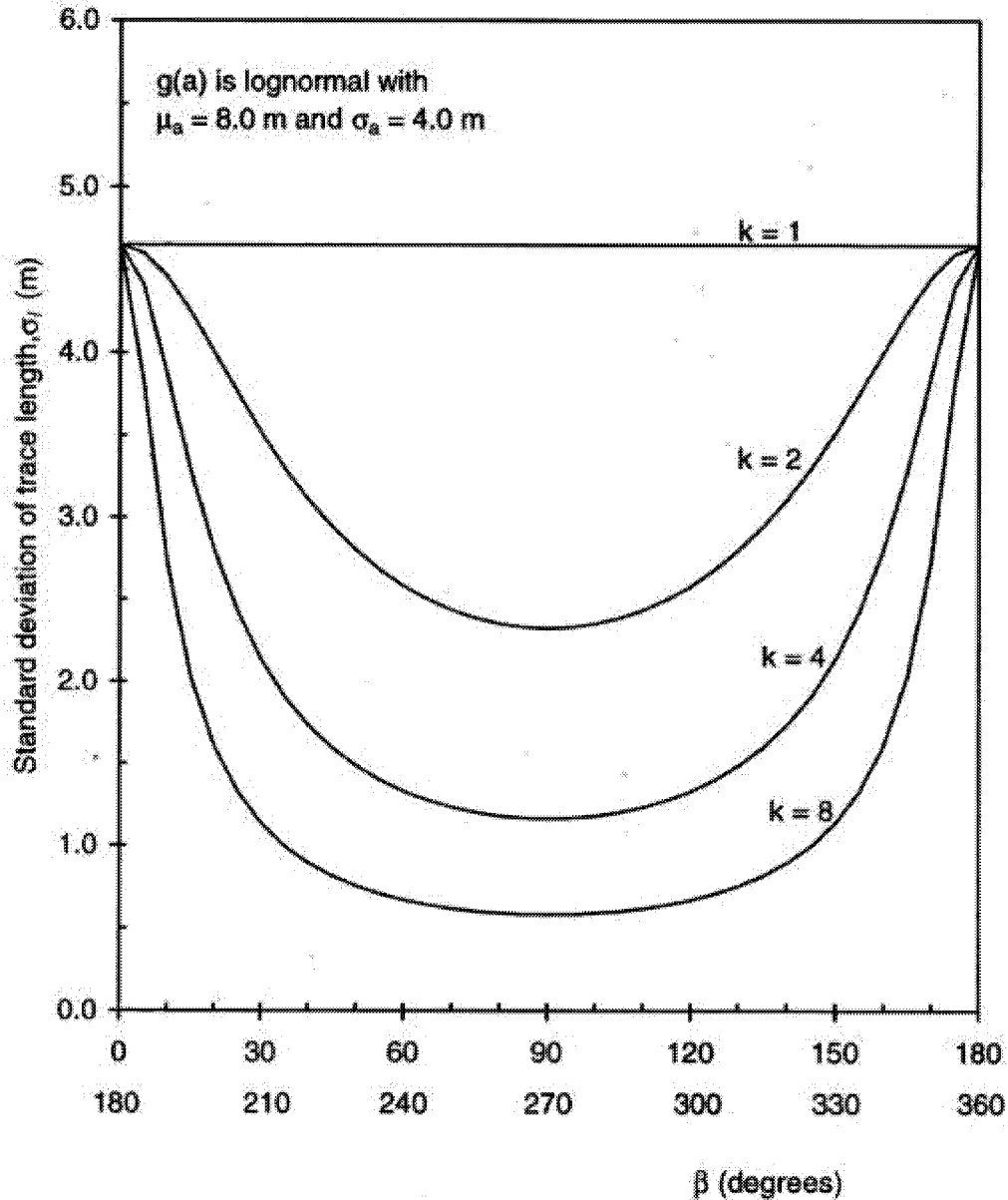
Figure 3-20 Variation of standard deviation of trace length with \beta
