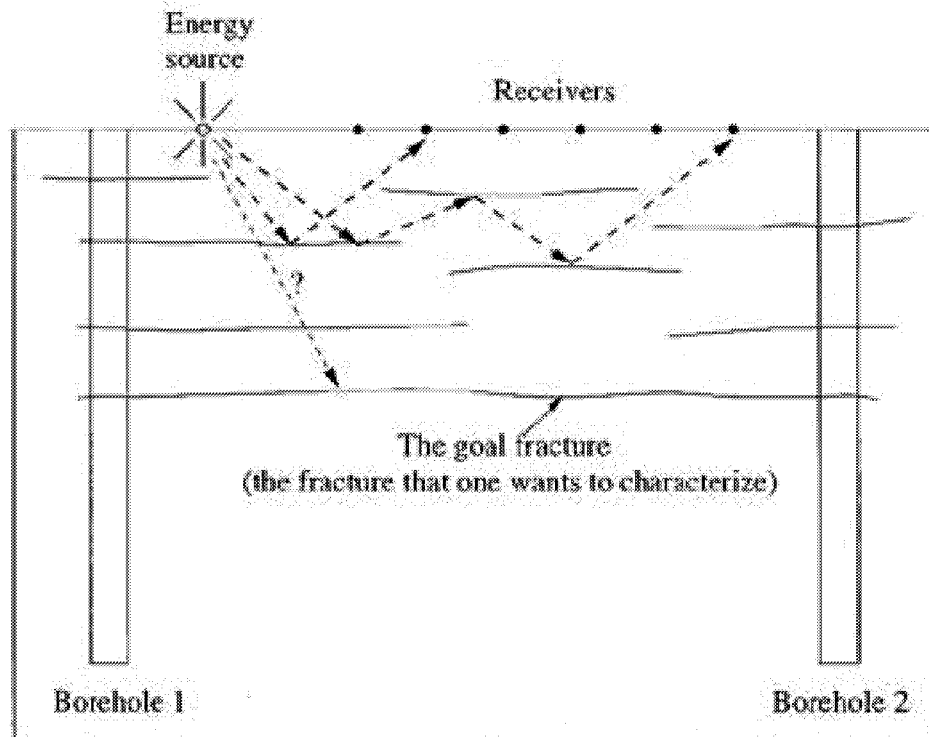
Figure 3-6 Seismic Wave Reflection by Features of Multiple Scales
