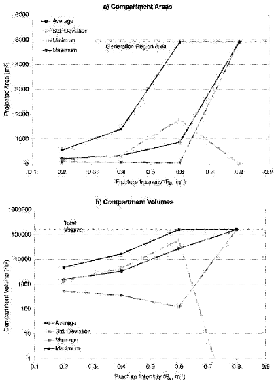
Figure 3-116 North Oregon Basin Compartmentalization Analysis
