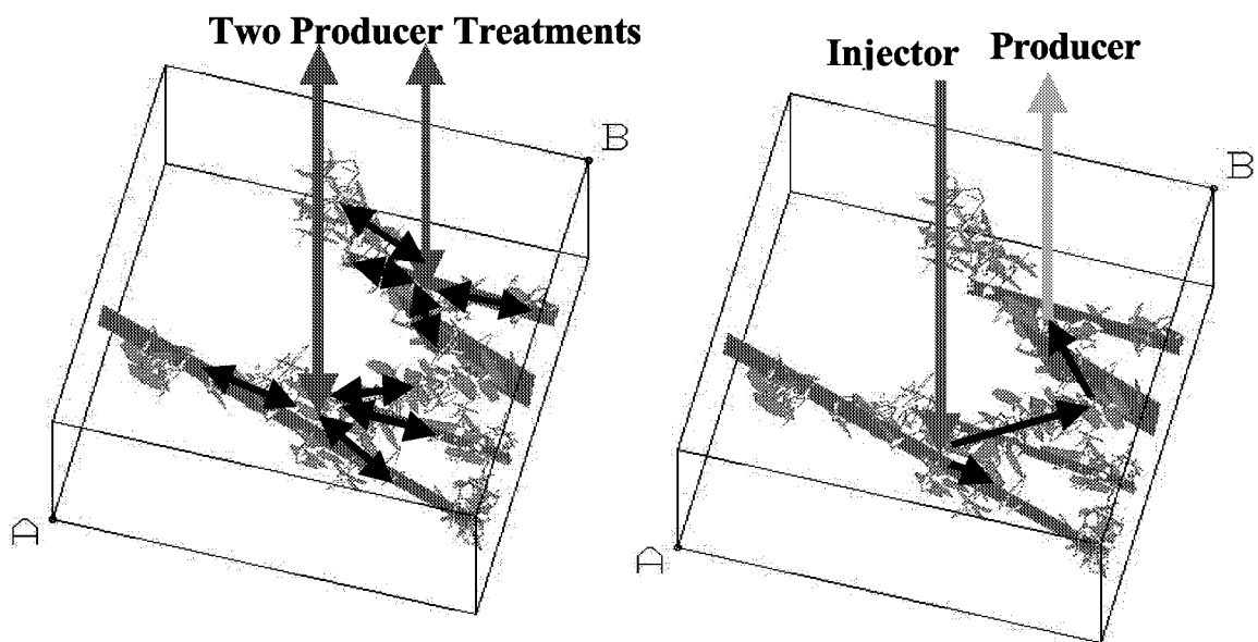
Figure 3-78 Surfactant Injection Strategies
