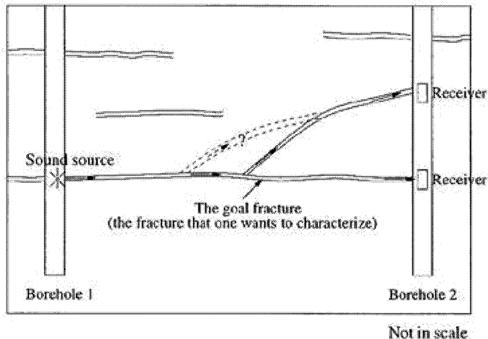
Figure 3-9 Wellbore Seismic Surveys
