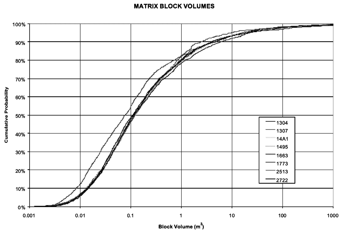
Figure 3-93: Block Volume Distribution
