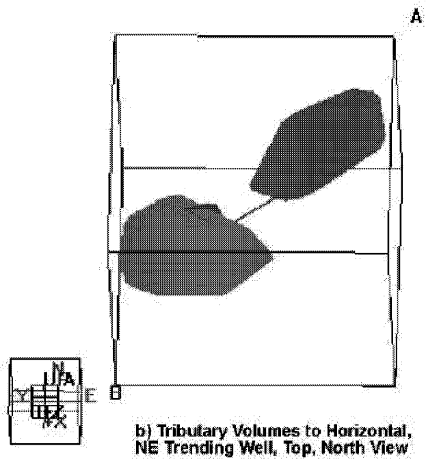
Figure 3-117 North Oregon Basin Model with P_{32} = 0.2
