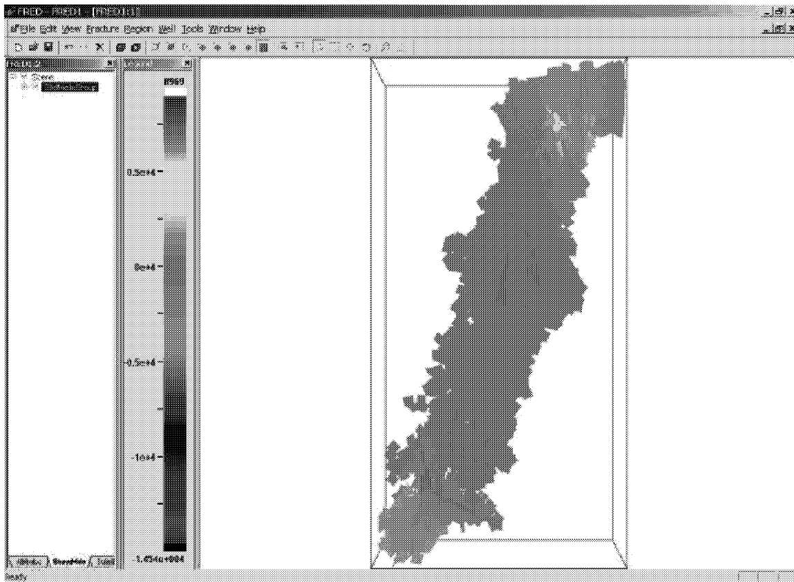
Figure 3-137 Stoney Point Pressure field at 0.1 hours after gel-treatment reduces permeability by a factor of 100
