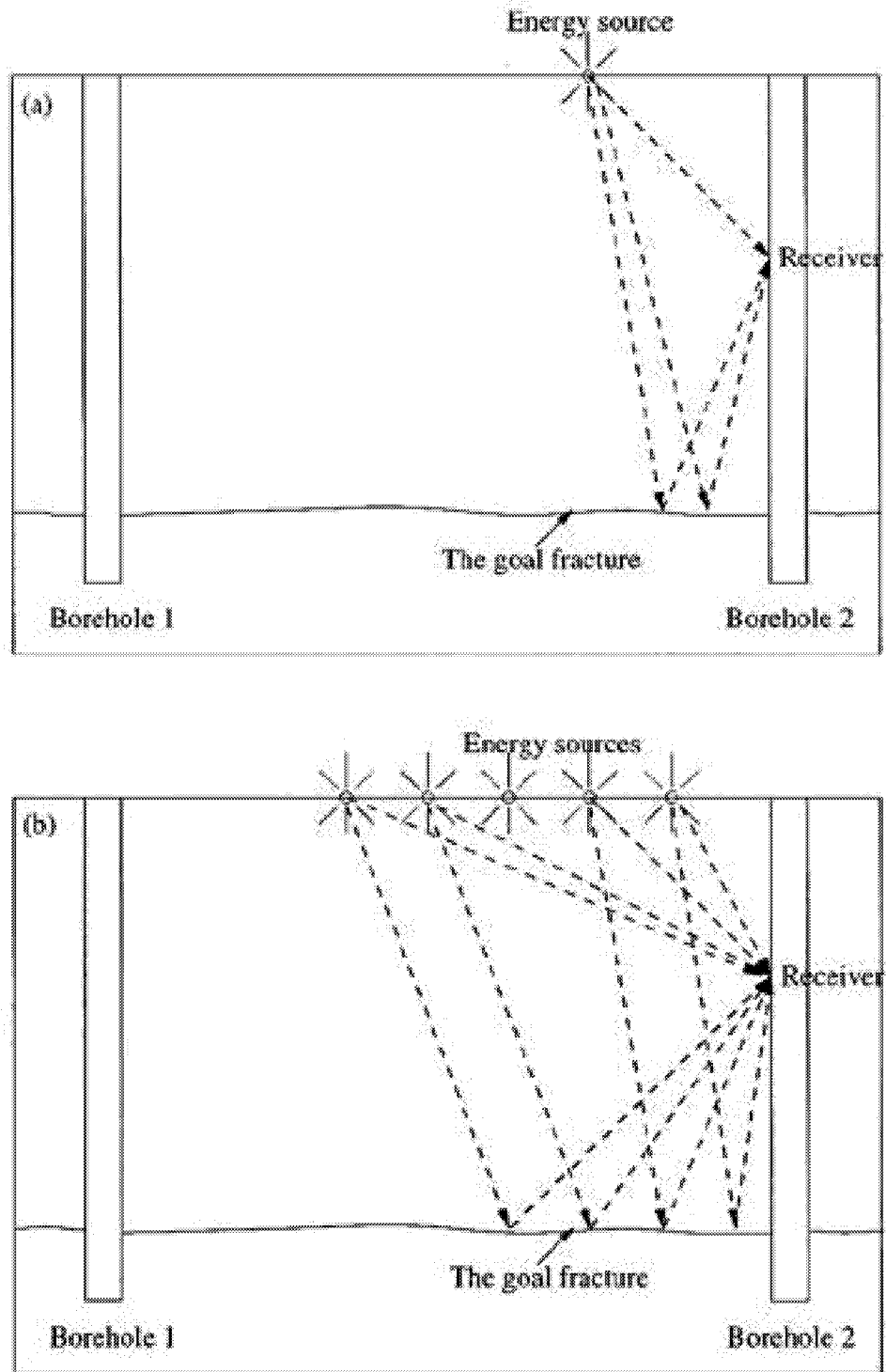
Figure 3-5 VSP Approaches (a) Offset and (b) Walkway
