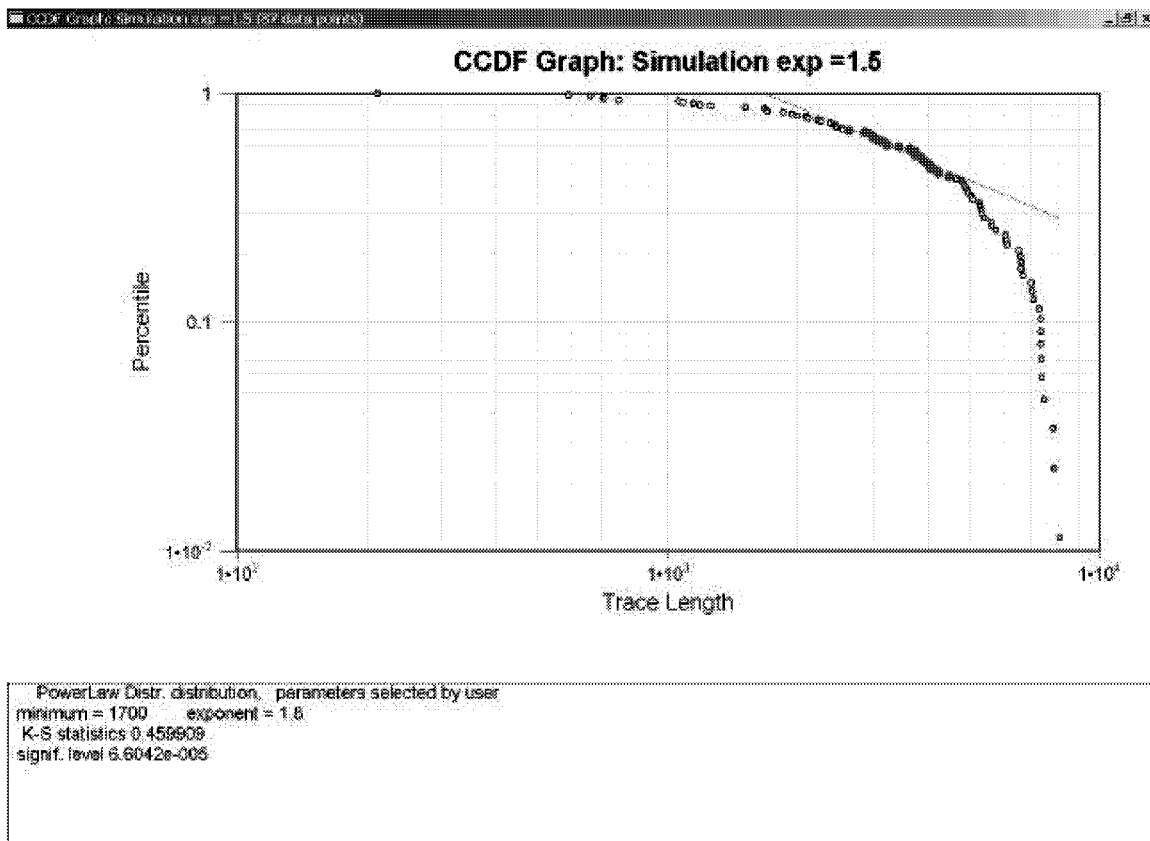
Figure 3-154 Simulation of ESE Lineaments, Exponent 1.5
