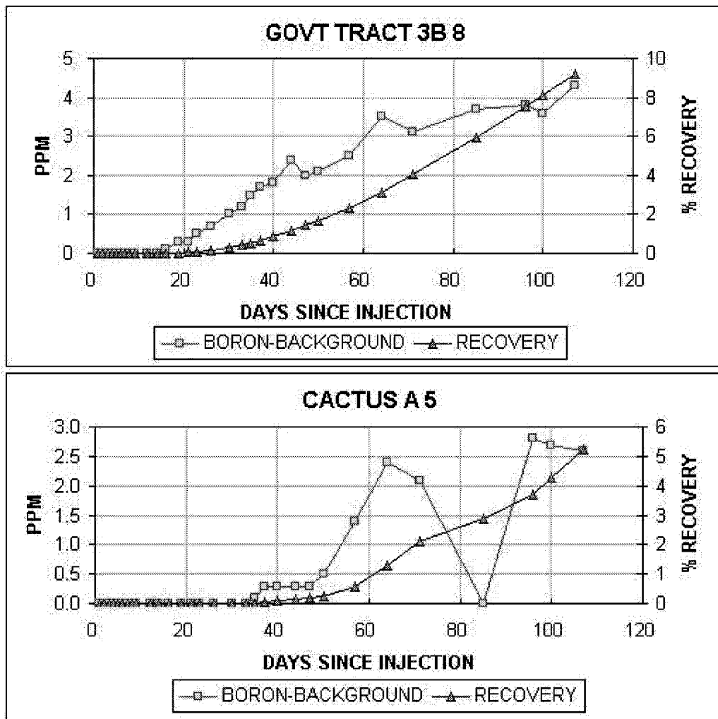
Figure 3-60 Example Tracer Breakthrough Curves from North Oregon Basin
