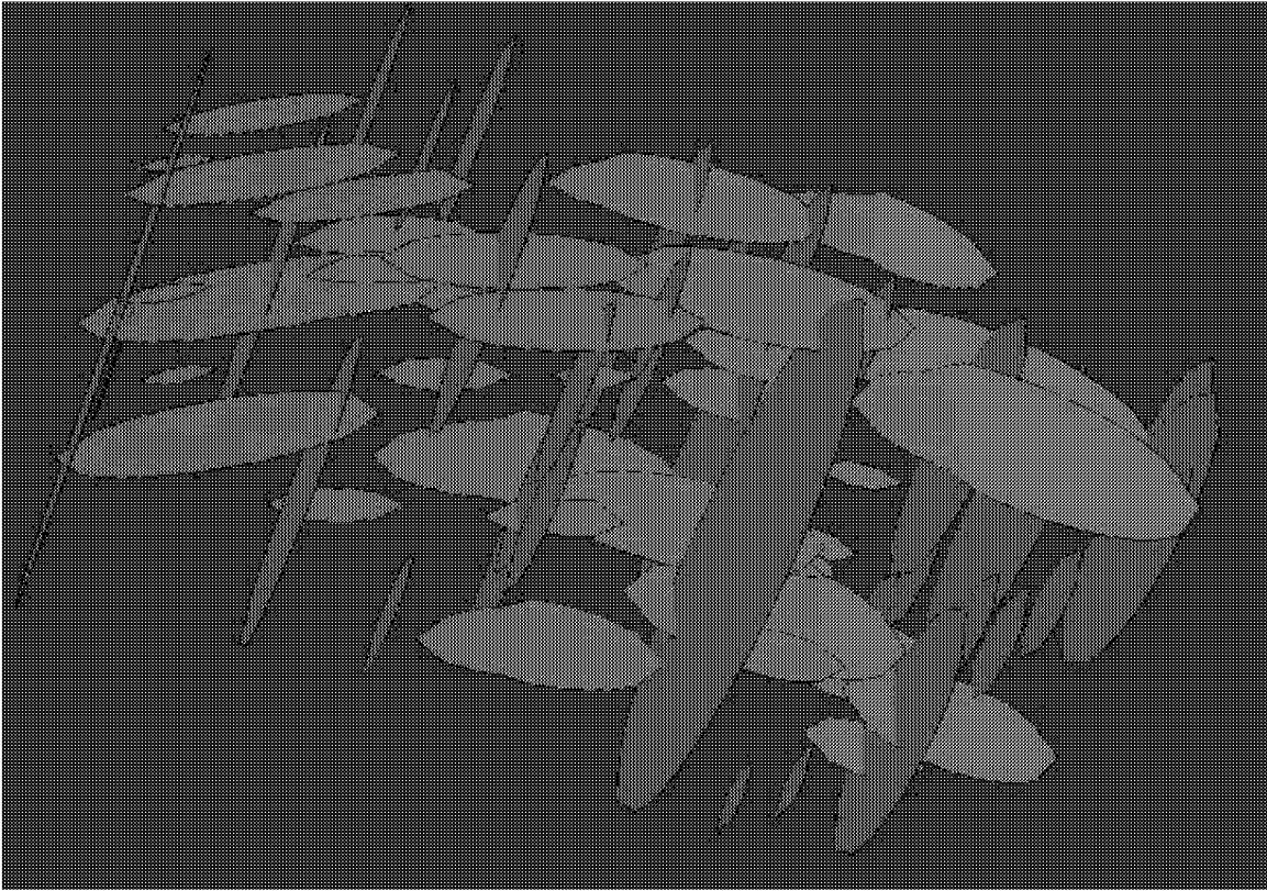
Figure 3-68 Fracture Growth Model (after Swaby and Rawnsly, 1996)
