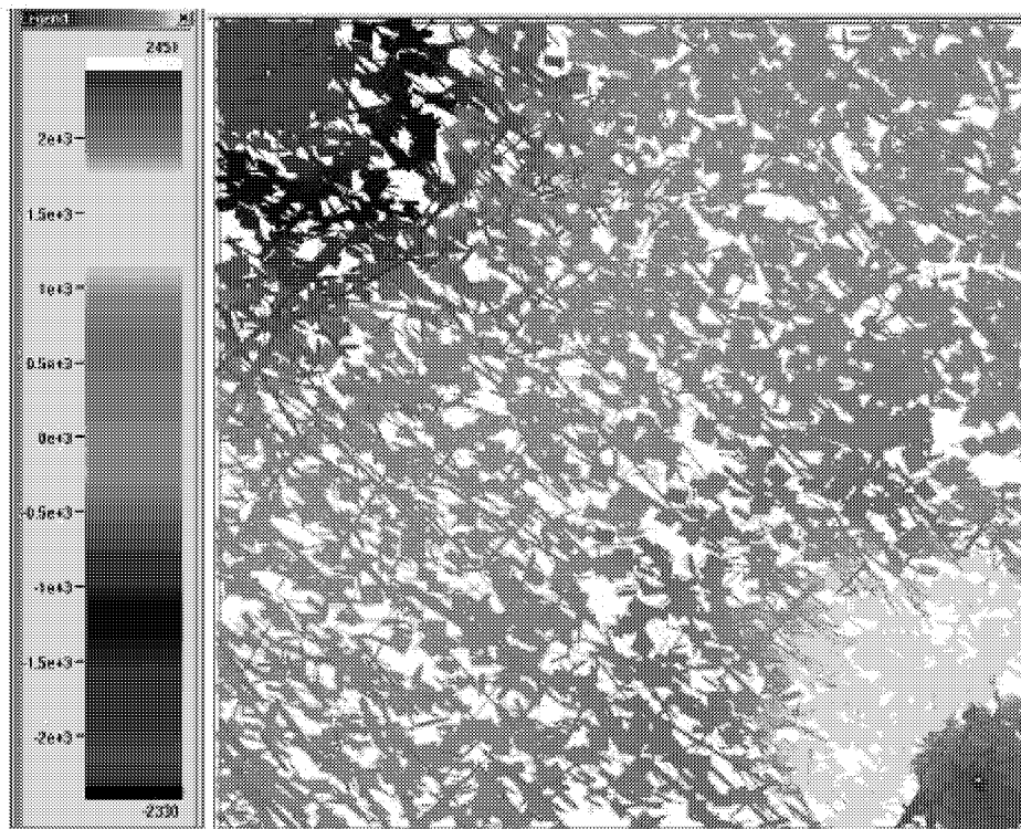
Figure 3-169: South Oregon Basin simulation after gel treatment reduces fracture permeability 3 orders of magnitude
