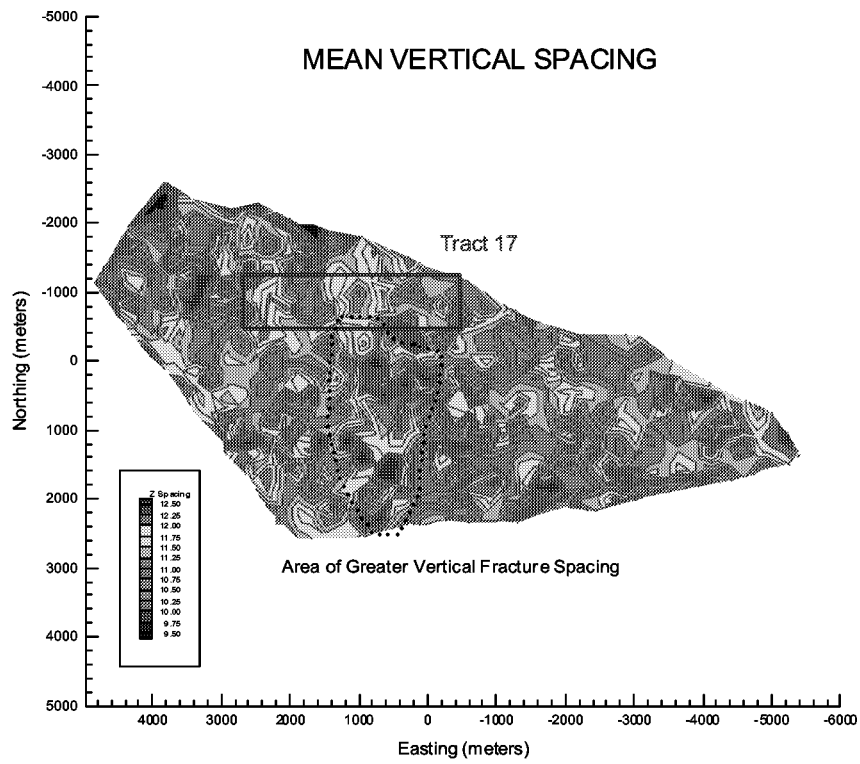
Figure 3-122: Mean Vertical Fracture Spacing
