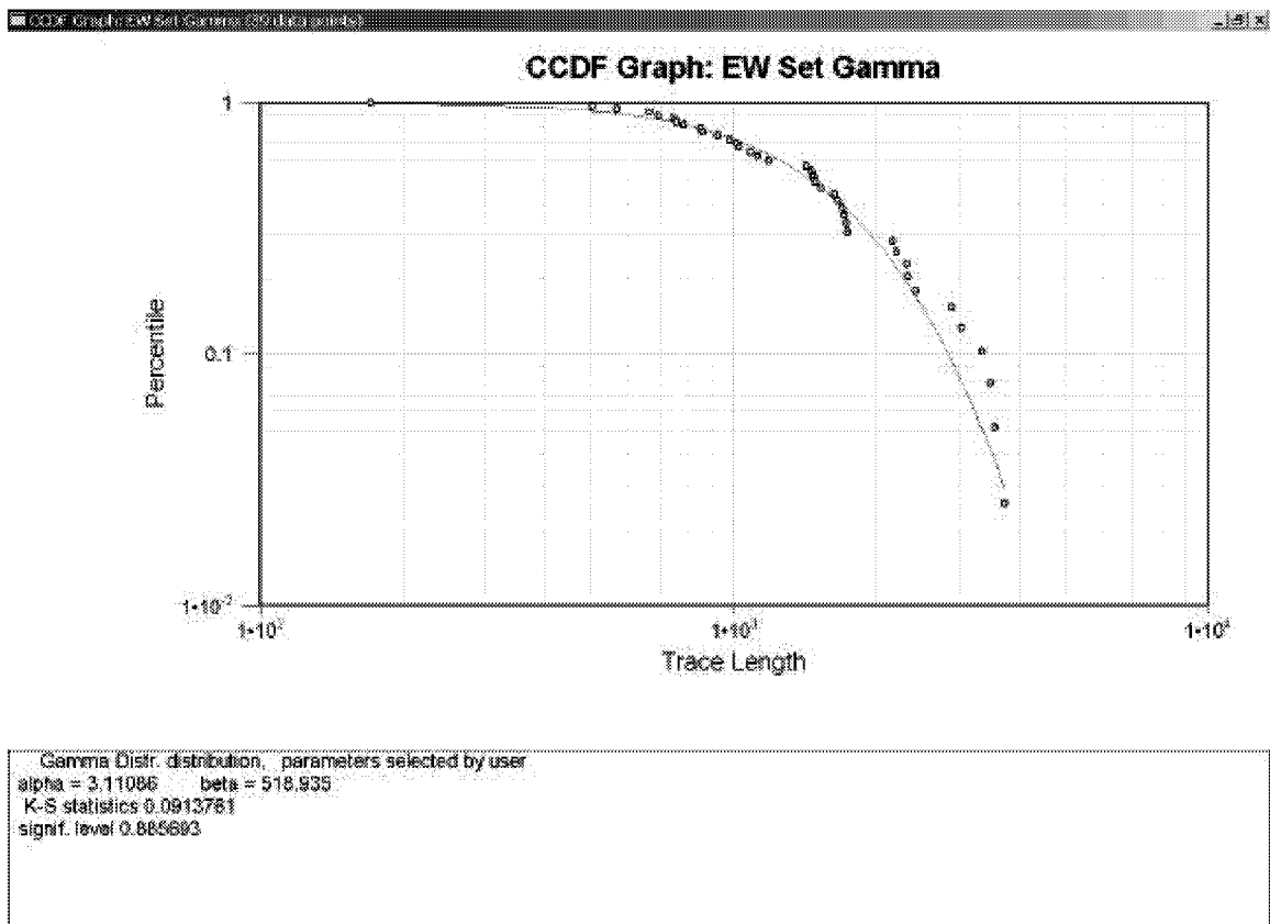
Figure 3-145: Trace Length Distribution, EW Lineaments
