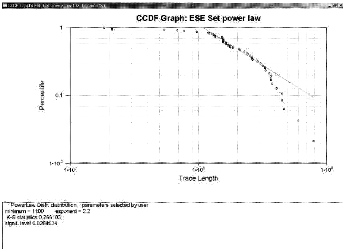
Figure 3-146: Trace Length Distribution, ESE Lineament
