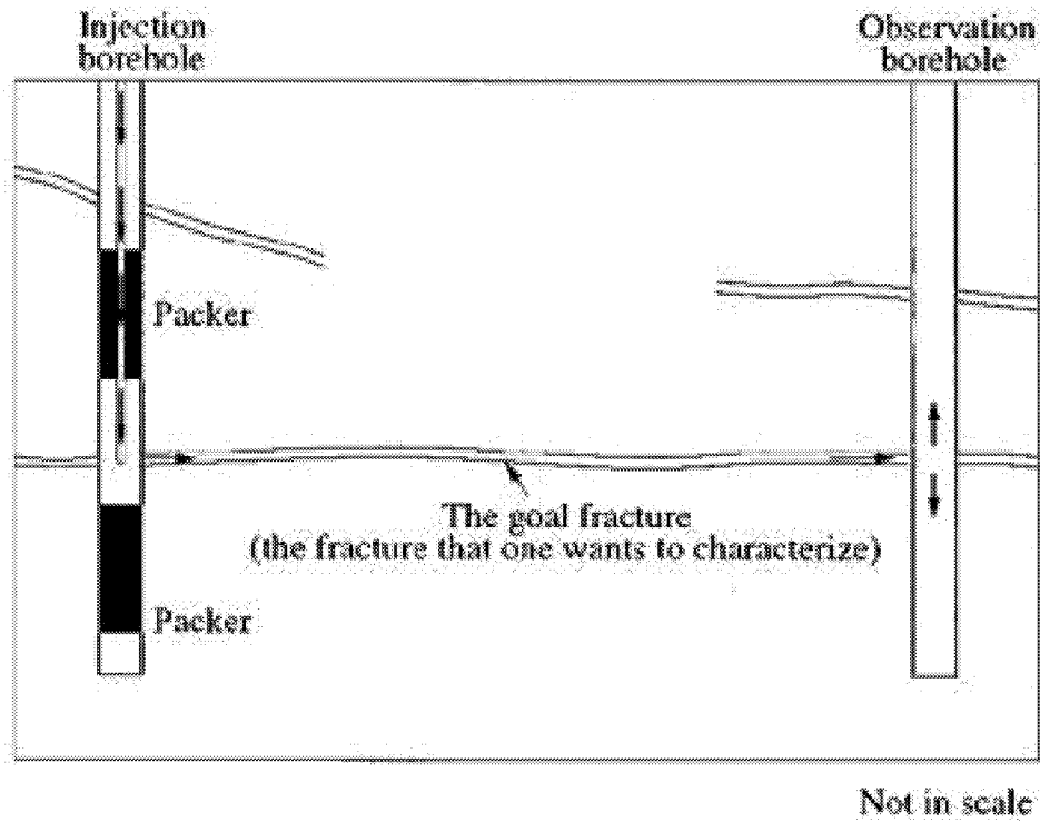
Figure 3-13 Packer Testing
