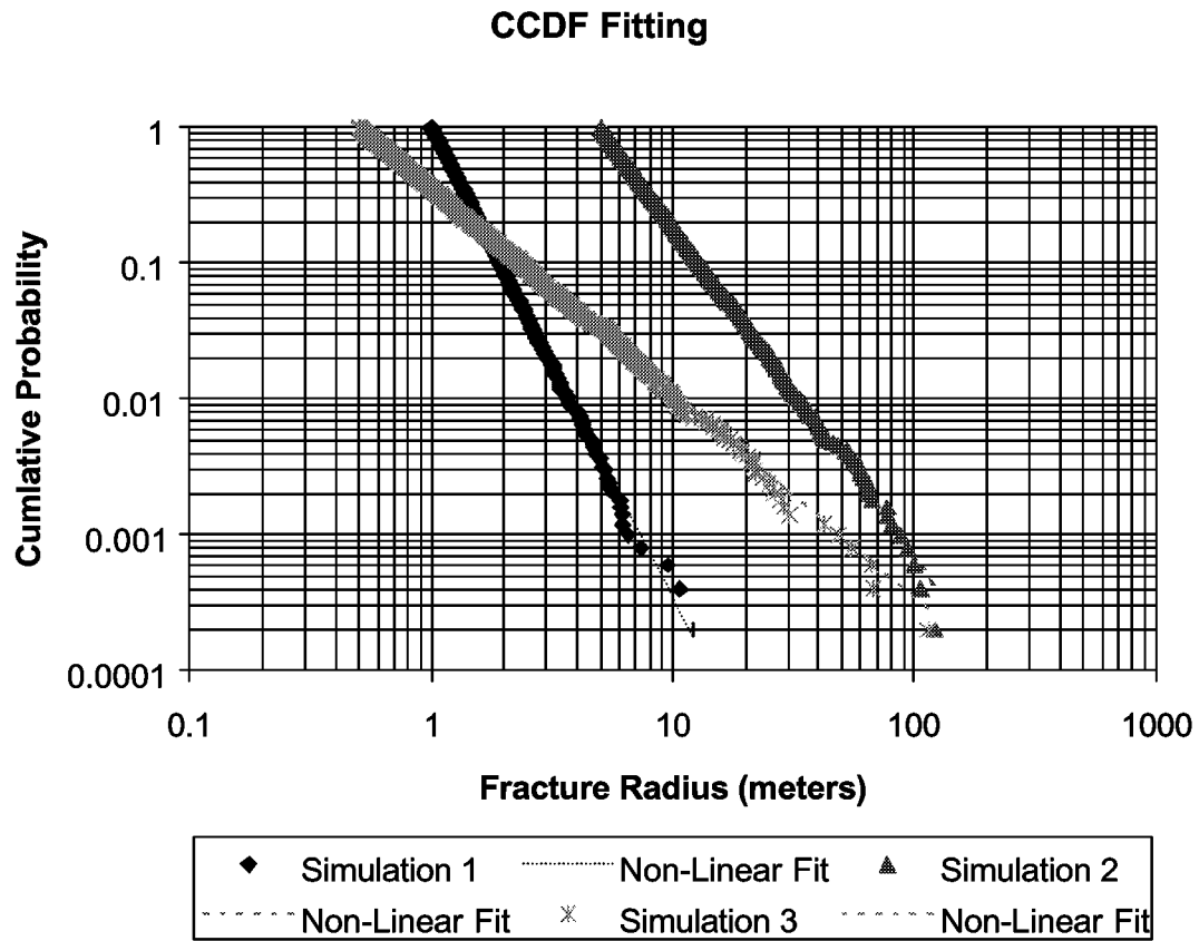
Figure 3-46 Complementary Cumulative Density Functions (CCDF) for Fracture Radius
