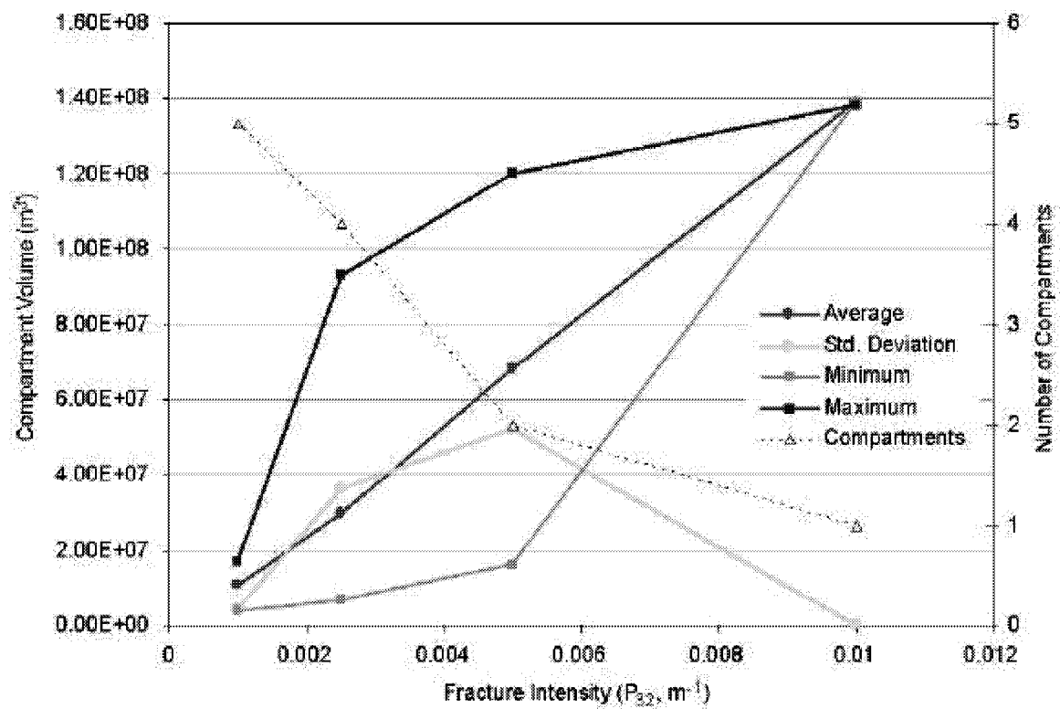
Figure 3-103 Volumes of Compartments in Stoney Point Model
