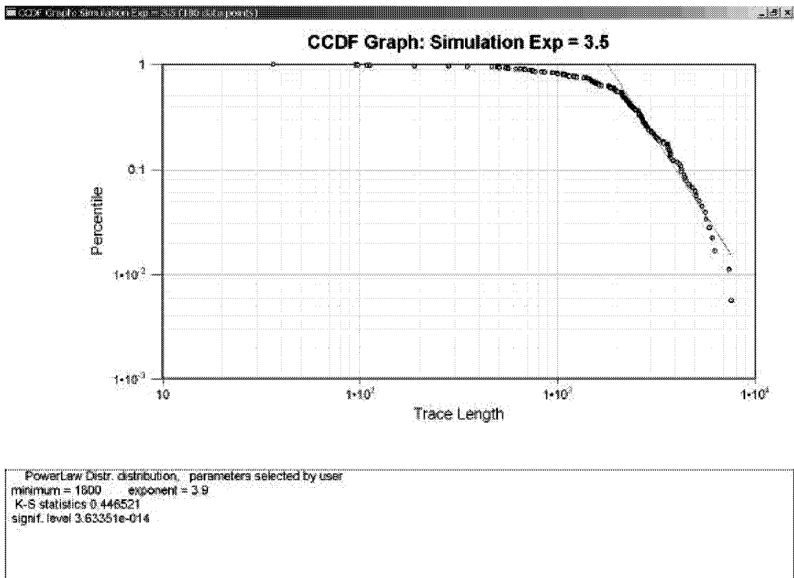
Figure 3-157: Simulation of ESE Lineaments, Exponent 3.5
