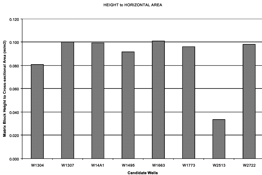
Figure 3-98 Median Ratio of Height to Horizontal Area
