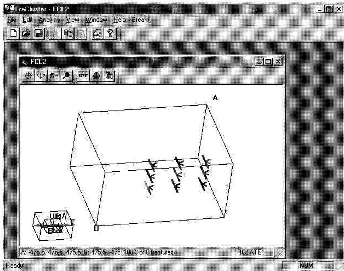
Figure 3-104 Well Configuration for Tributary Volume Analysis of Stoney Point Model
