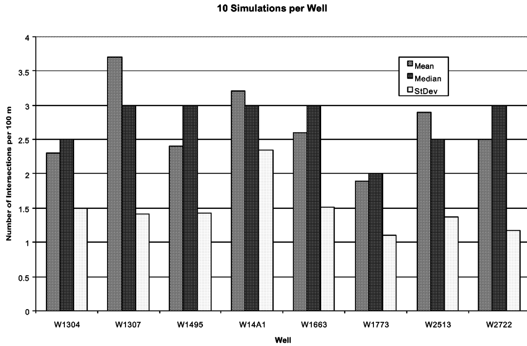
Figure 3-87 Intersection Statistics for Deepening Candidate Wells
