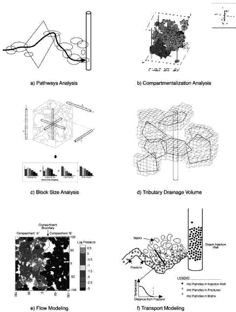
Figure 2-2: DFN Approaches for IOR
