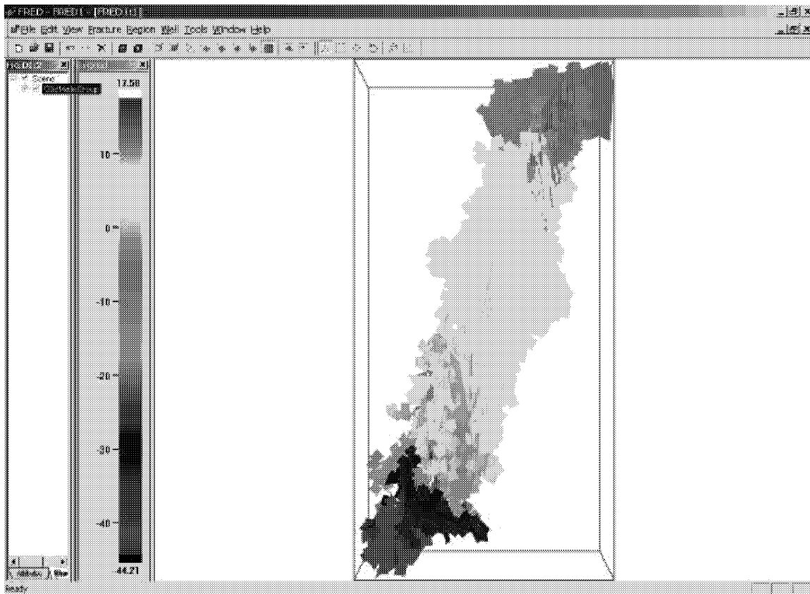
Figure 3-134: Flow solution after 0.1 hours, pre-gel treatment. Note pressure has connected directly from injector to producer
