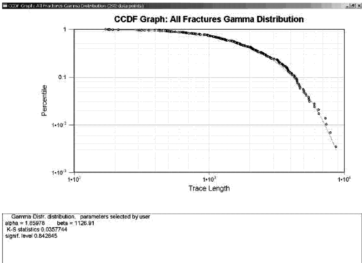
Figure 3-144: Trace Length Distribution, All Lineaments
