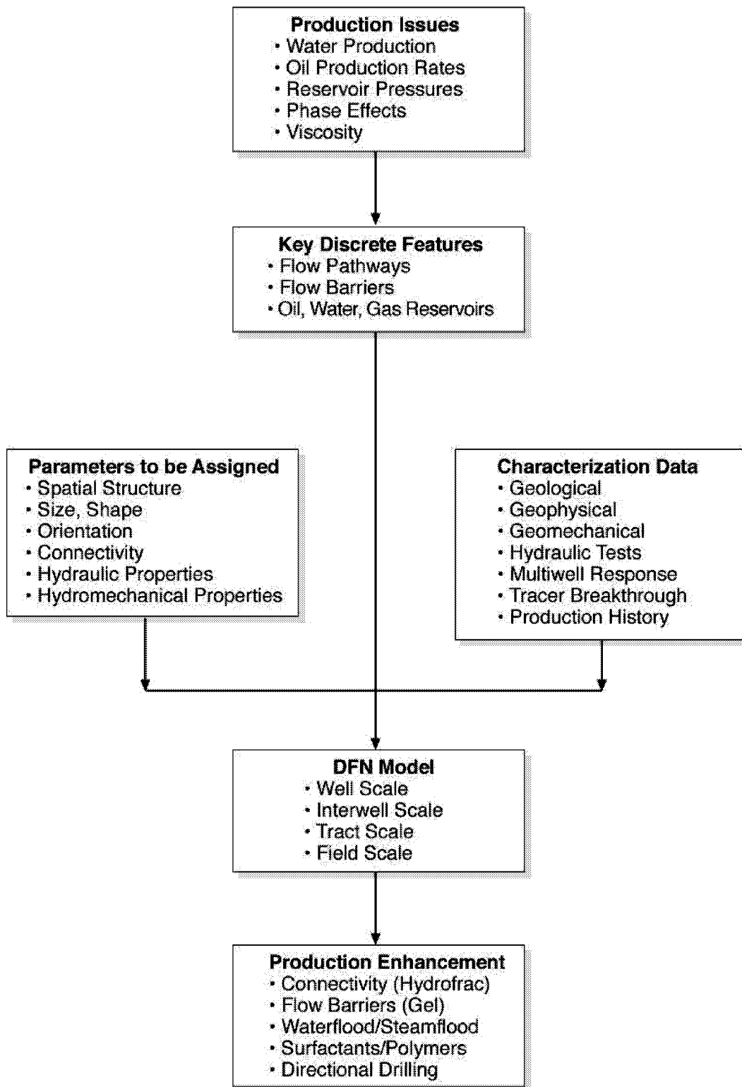
Figure 2-1: DFN Approach for Reservoir Characterization and Engineering
