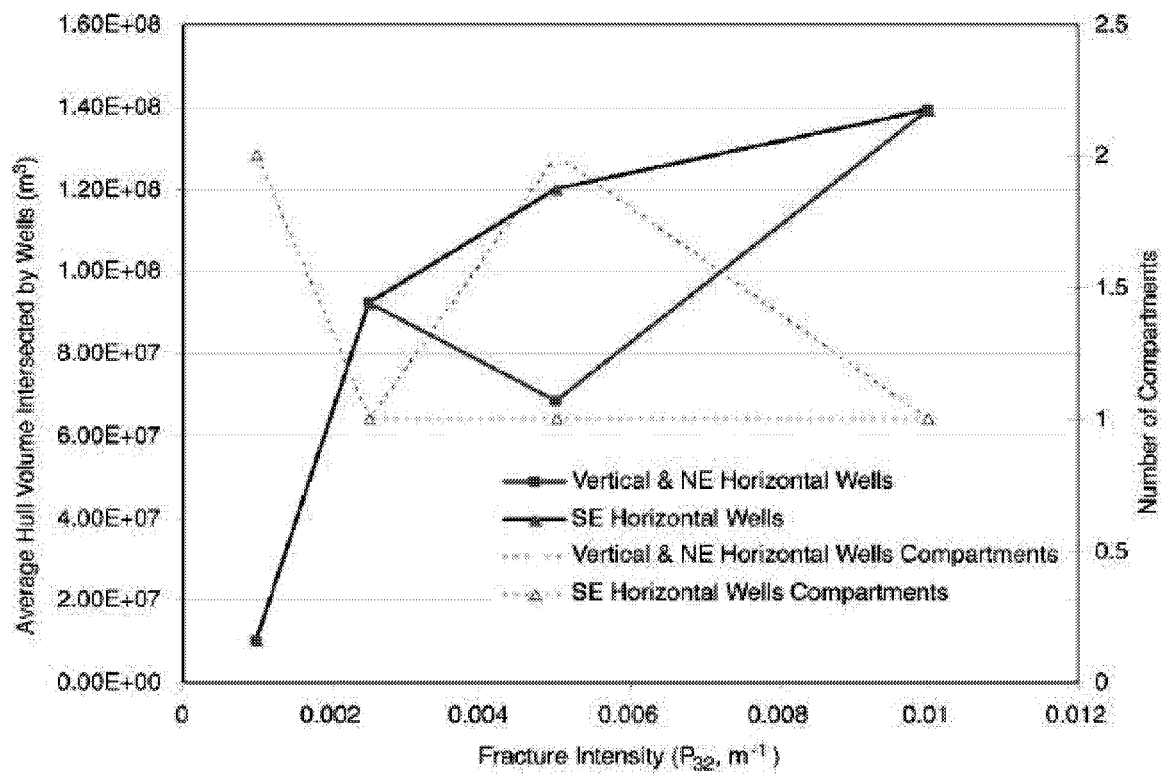
Figure 3-105 Tributary Volumes of Stoney Point Model
