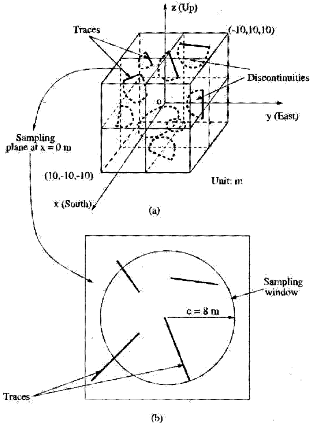
Figure 3-21 (a) Simulation volume is a box, i.e., the elliptical discontinuities are generated inside the box; (b) Sampling window at x = 0 m
