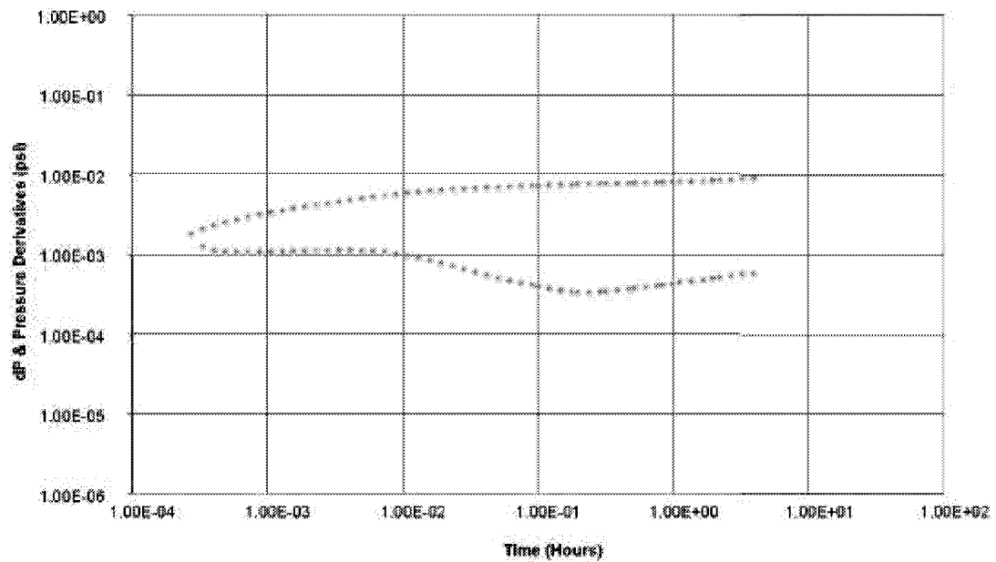
Figure 3-53 Production Test with Single Channel, Well on Fault
