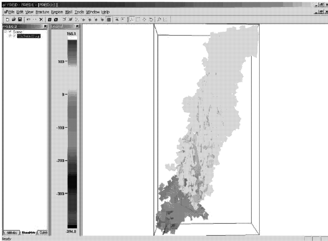
Figure 3-136 Stoney Point: Pressure after 0.1 with gel treatment reducing the fracture permeability by a factor of 10.
