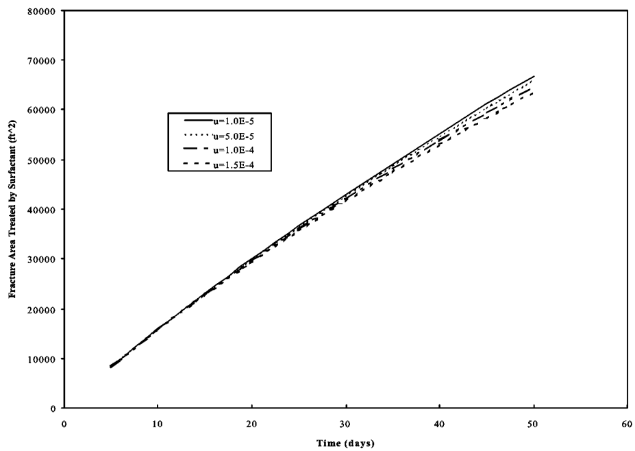
Figure 3-85 Effects of Convection Rate on Fracture Area Treated
