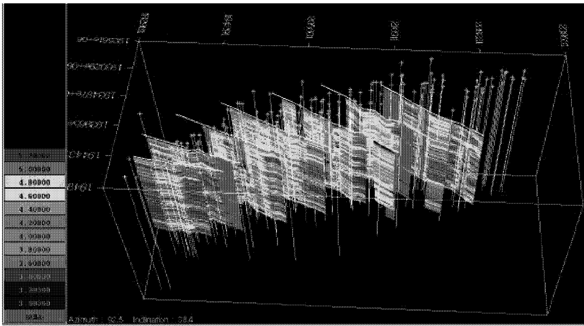
Figure 3-66: Stoney Point, Geophysical Cross Sections
