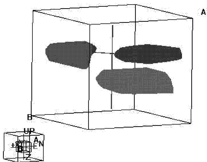
Figure 3-118 Side View of Tributary Volumes of Vertical and Horizontal Wells in North Oregon Basin Model with P_{32} = 0.2
