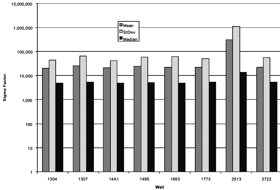
Figure 3-94 Block Sigma Factor Statistics
