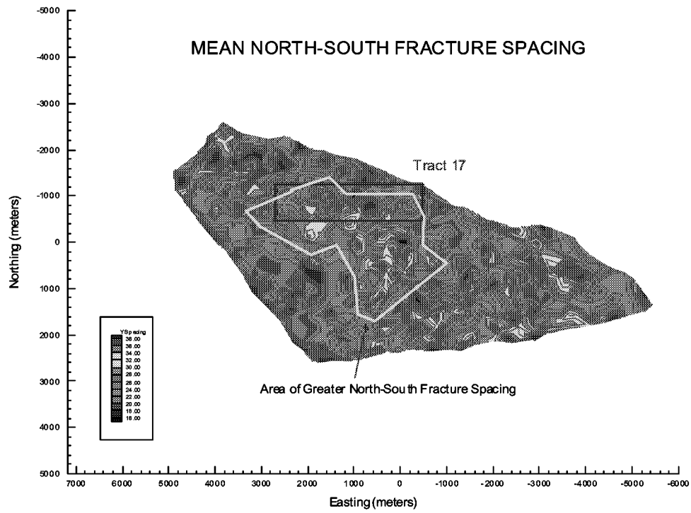
Figure 3-121: Mean North-South Fracture Spacing
