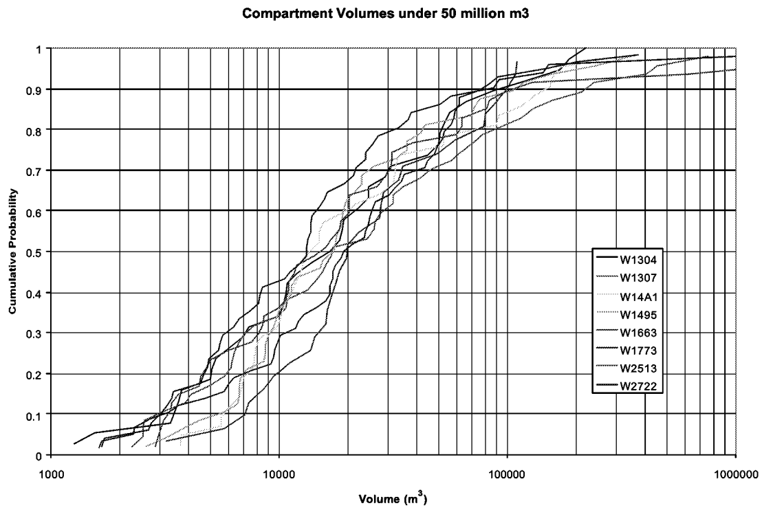
Figure 3-90 Compartment Volume, Yates Deepening Candidates
