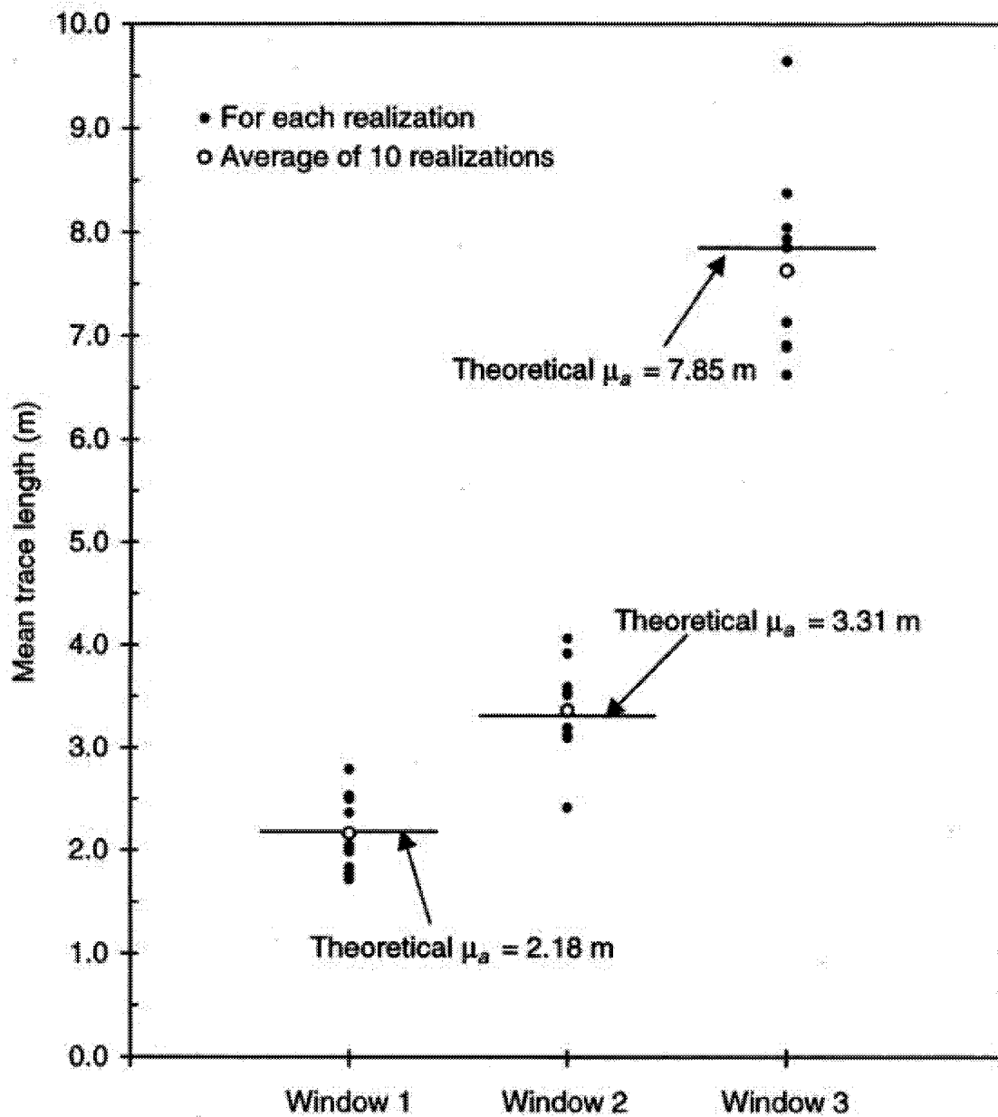
Figure 3-22 Comparison of theoretical mean trace lengths with predicted mean trace lengths from simulations
