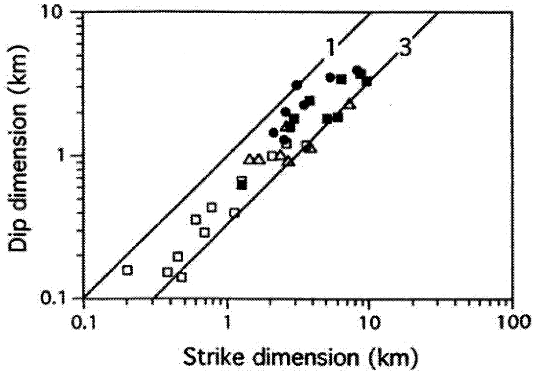
Figure 3-35 Dip dimension vs. strike dimension for nominally unrestricted faults from four regions (see Table 3-15) (from Nicol et al. 1996)
