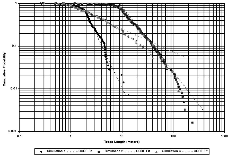
Figure 3-47 Fitted Trace Length Distributions
