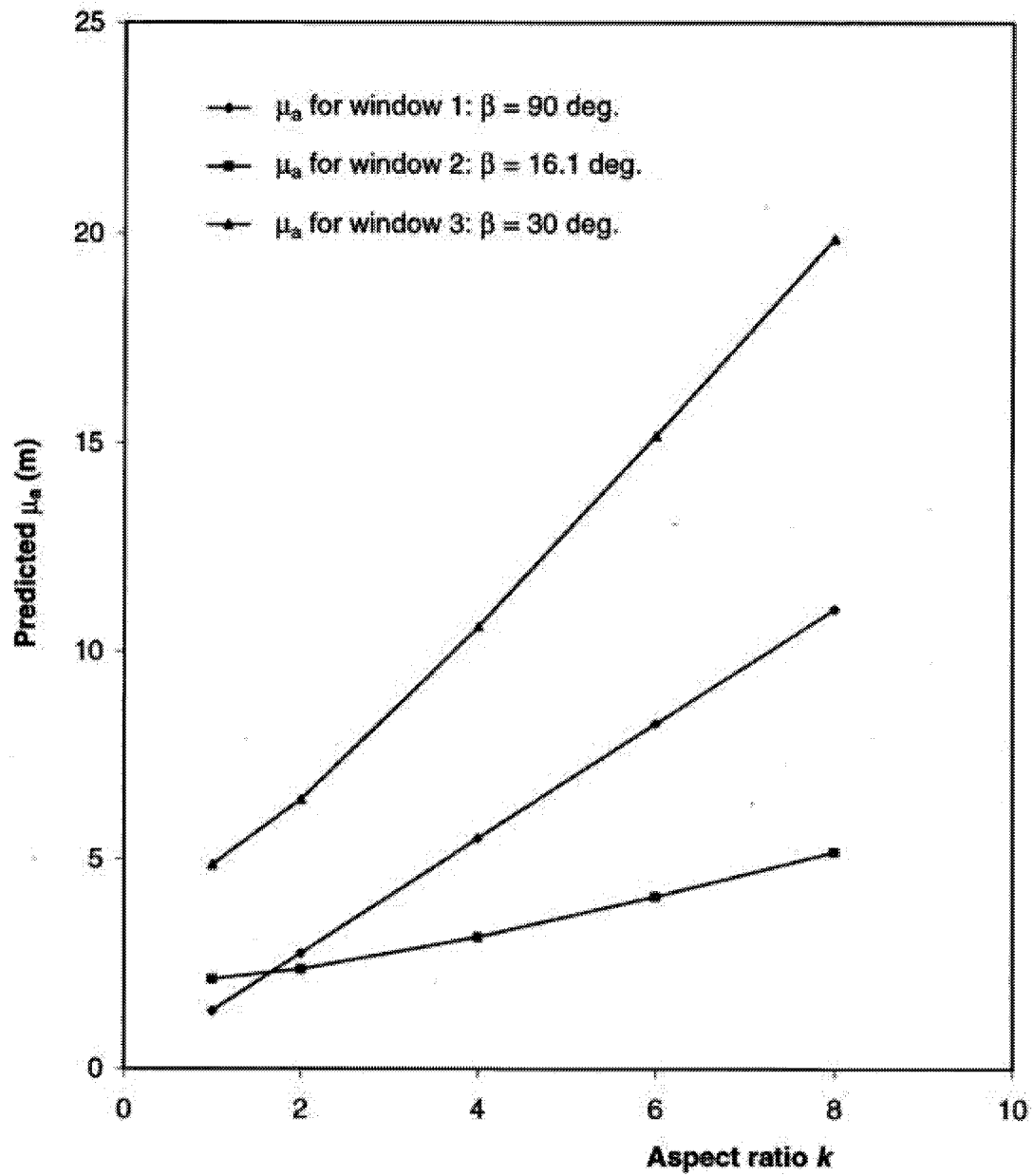
Figure 3-25 Variation of \mu_a with aspect ratio k for assumed major axis orientation 1 ( 0^\circ/0^\circ ): assuming a negative exponential distribution form of g(a)
