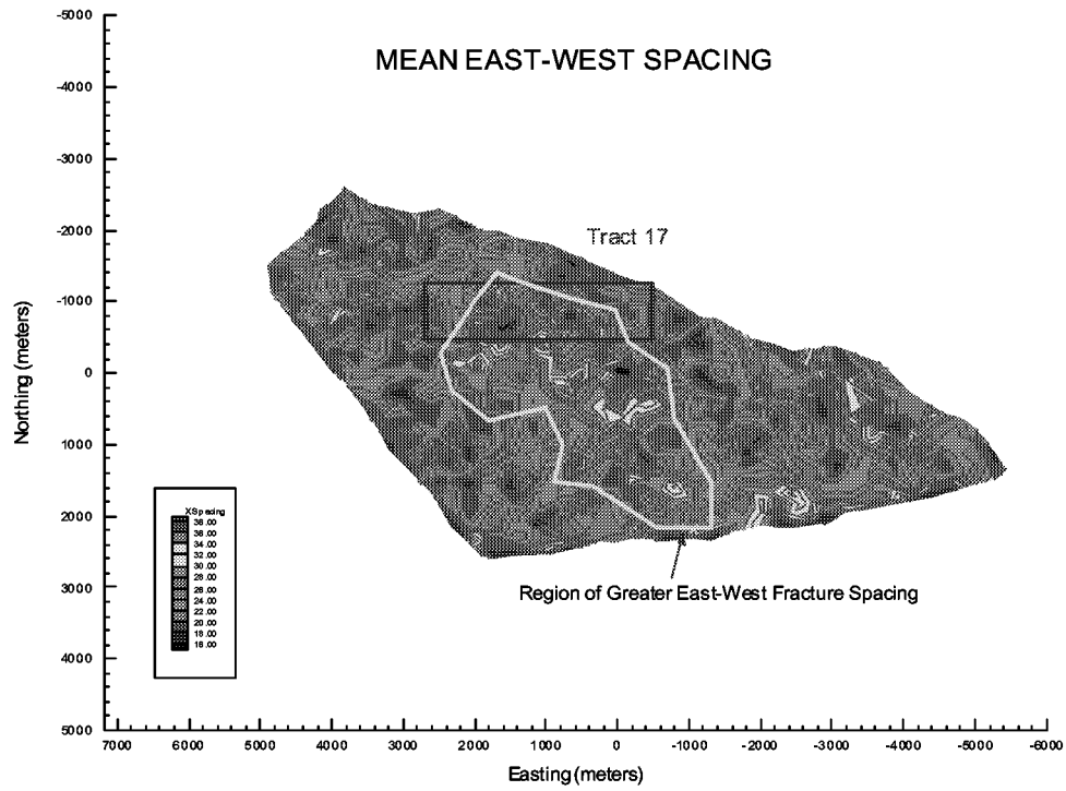
Figure 3-120: Mean East/West Fracture Spacing
