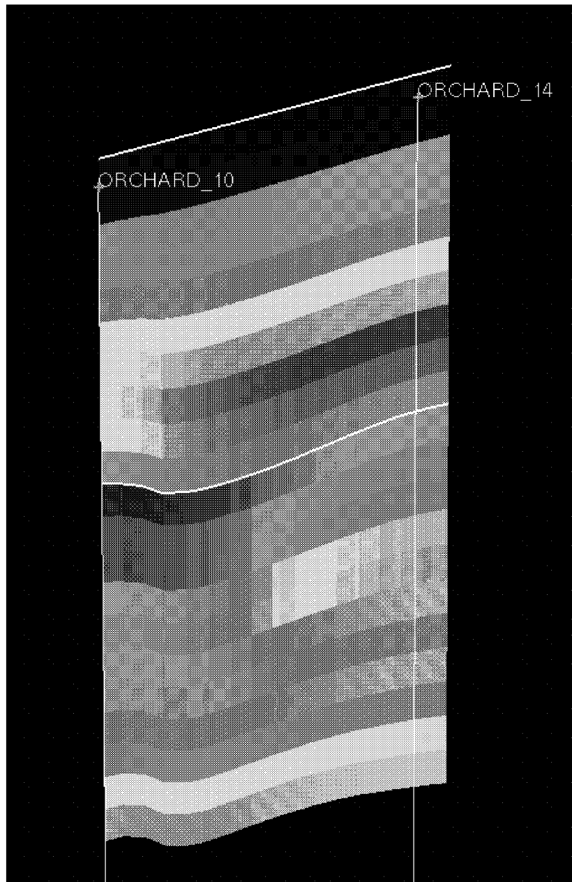
Figure 3-64 South Basin Geocellular ModelExample
