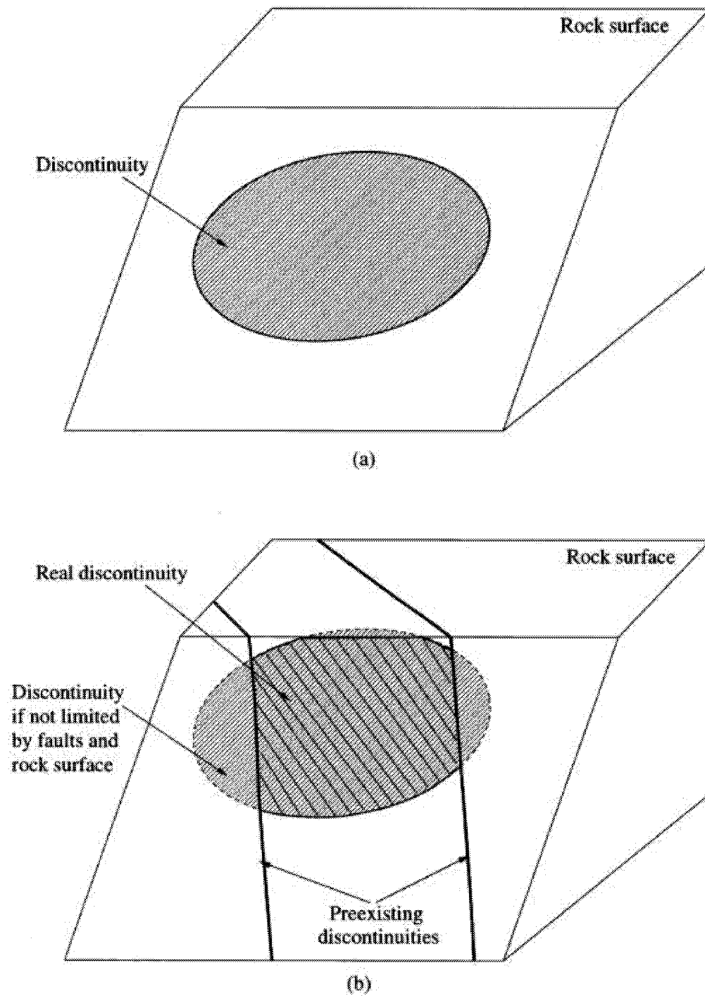
Figure 3-33 (a) An unrestricted discontinuity; and (b) A restricted discontinuity
