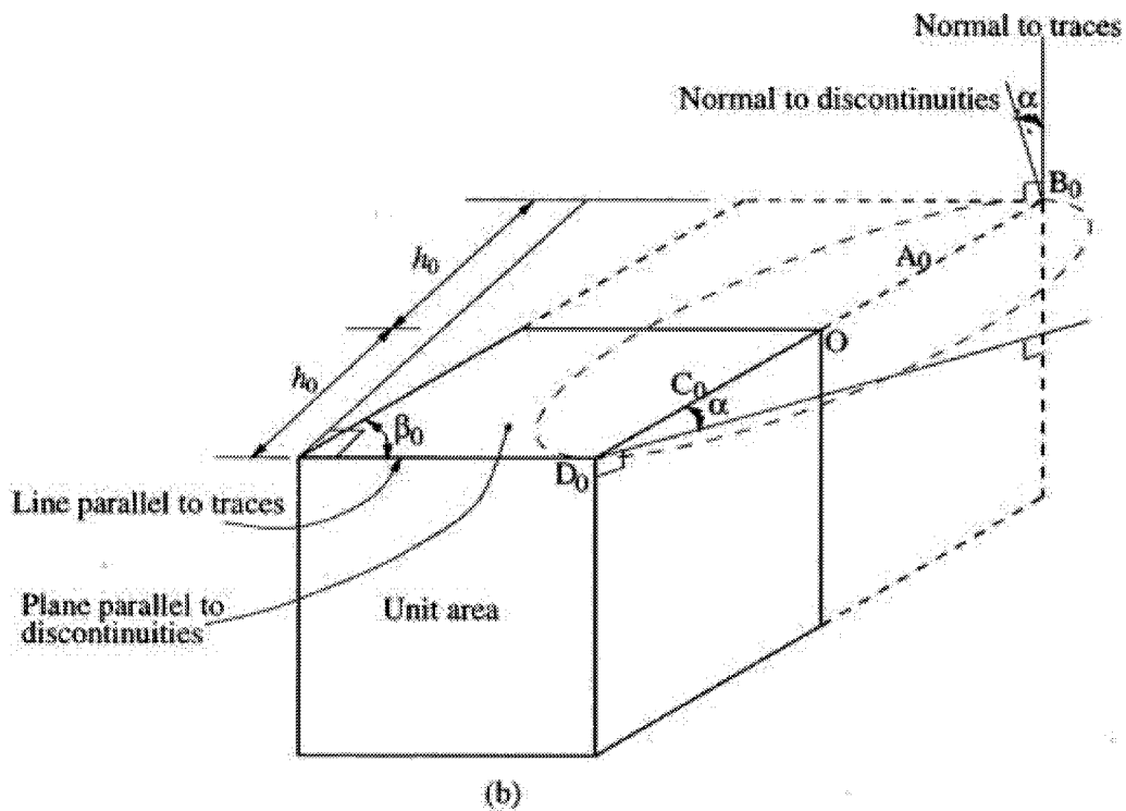
Figure 3-16 Construction used in derivation of relationship between discontinuity size distribution and trace length distribution
