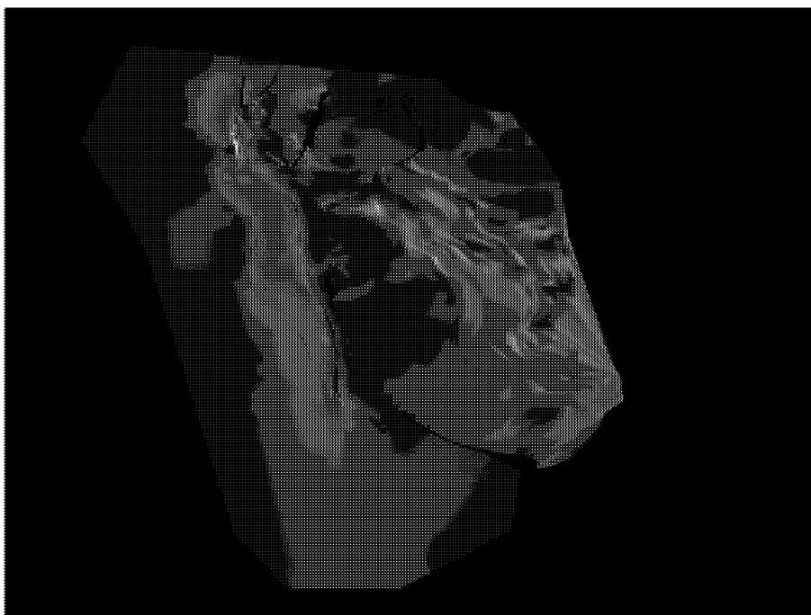
Figure 3-71 Strain Fields for Fracture Generation
