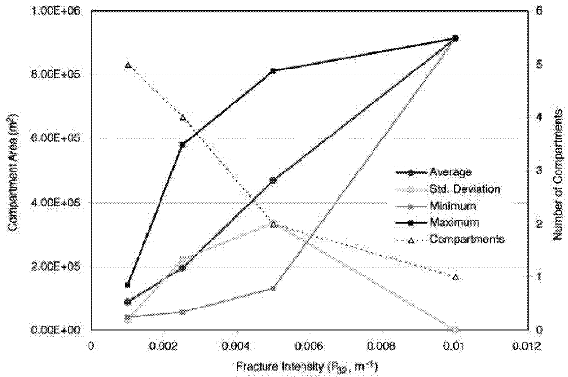
Figure 3-102 Projected Areas of Compartments
