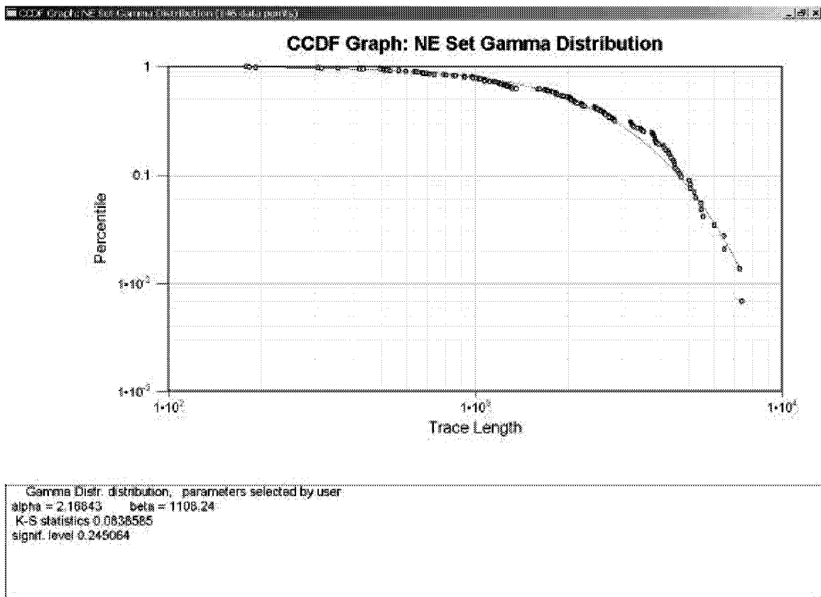
Figure 3-147: Trace Length Distribution, NE Lineaments
