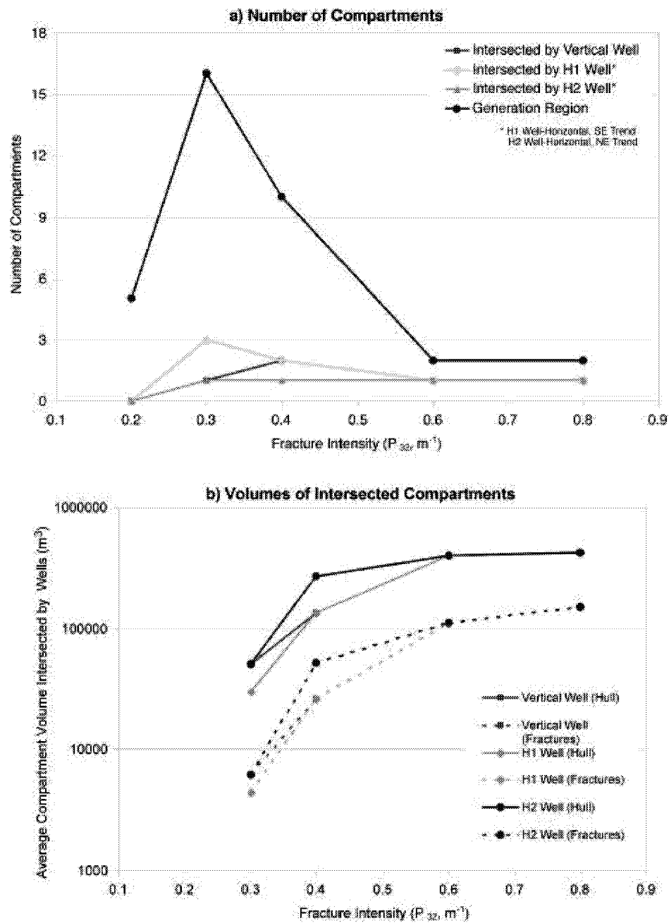
Figure 3-113 South Oregon Basin Tributary Volume Analysis
