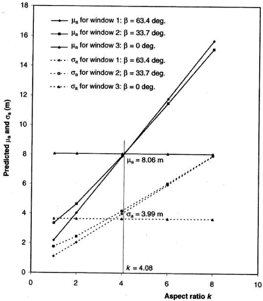
Figure 3-27 Variation of \mu_a and \sigma_a with aspect ratio k for assumed major axis orientation 2 ( 30^\circ/0^\circ ): assuming a lognormal distribution form of a
