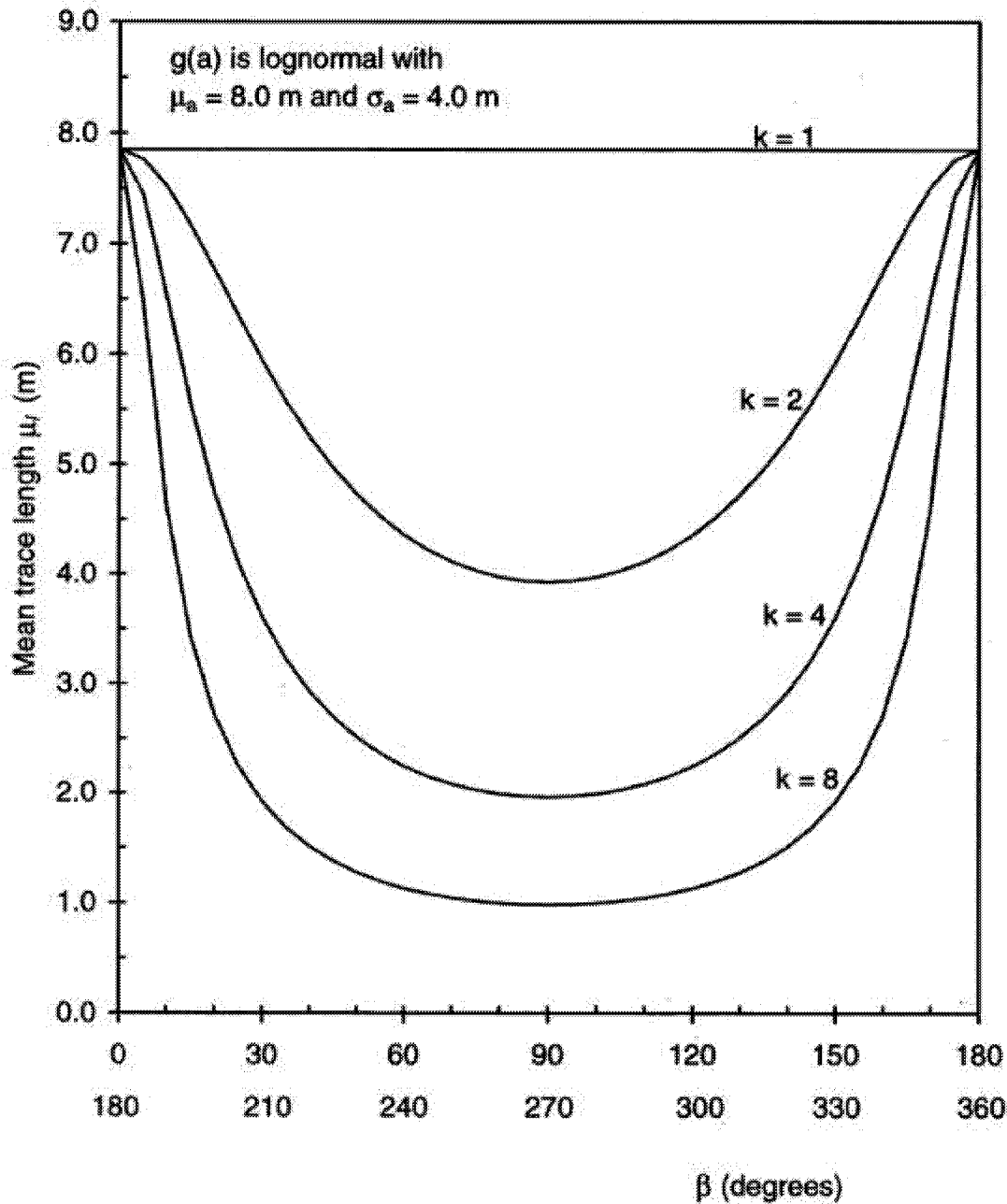
Figure 3-19 Variation of mean trace length with \beta
