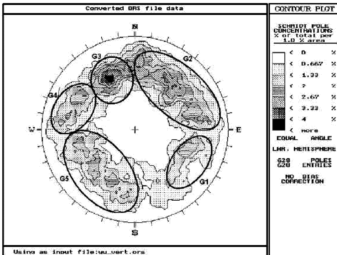
Figure 3-42 Contour Plot of Sets Identified by Structural Geologist
