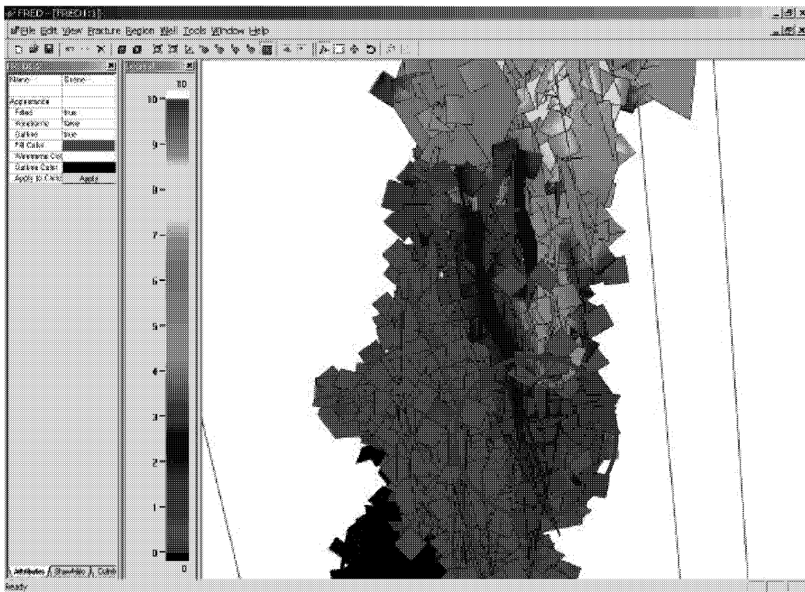
Figure 3-135: Stoney Point Flow Solution Pre-Gel treatment: Close up showing pressure bypassing matrix through fractures
