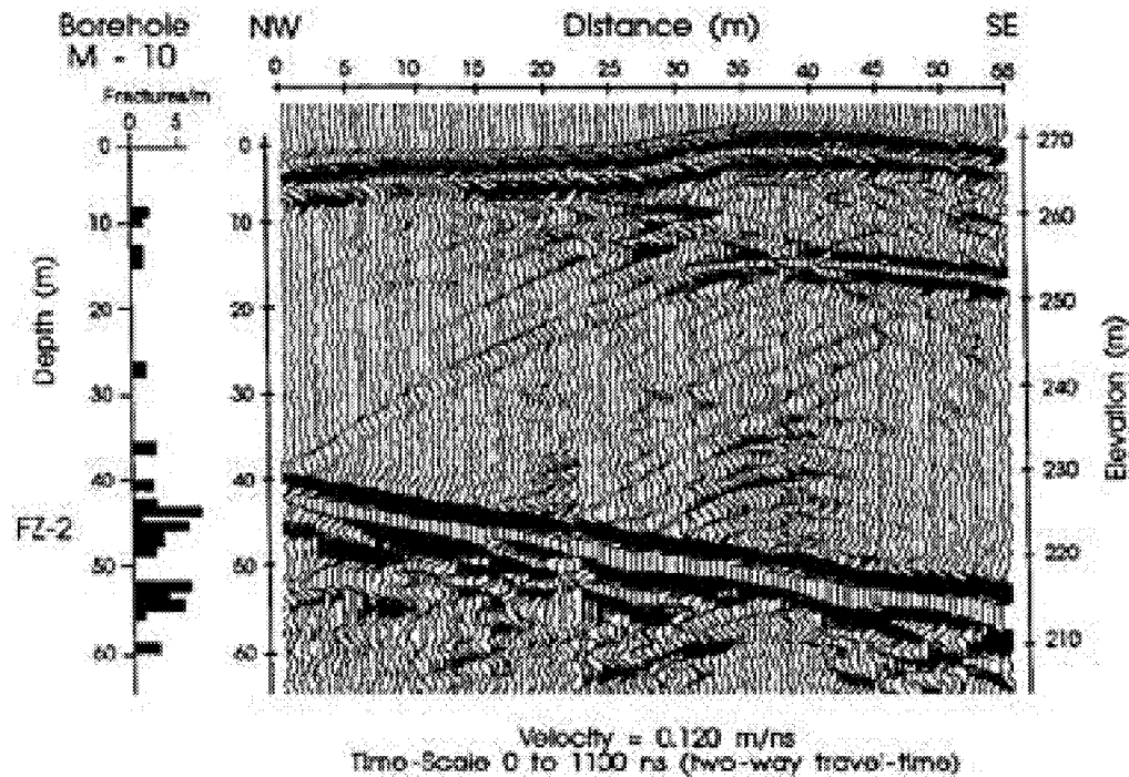
Figure 3-10 Radar Tomography
