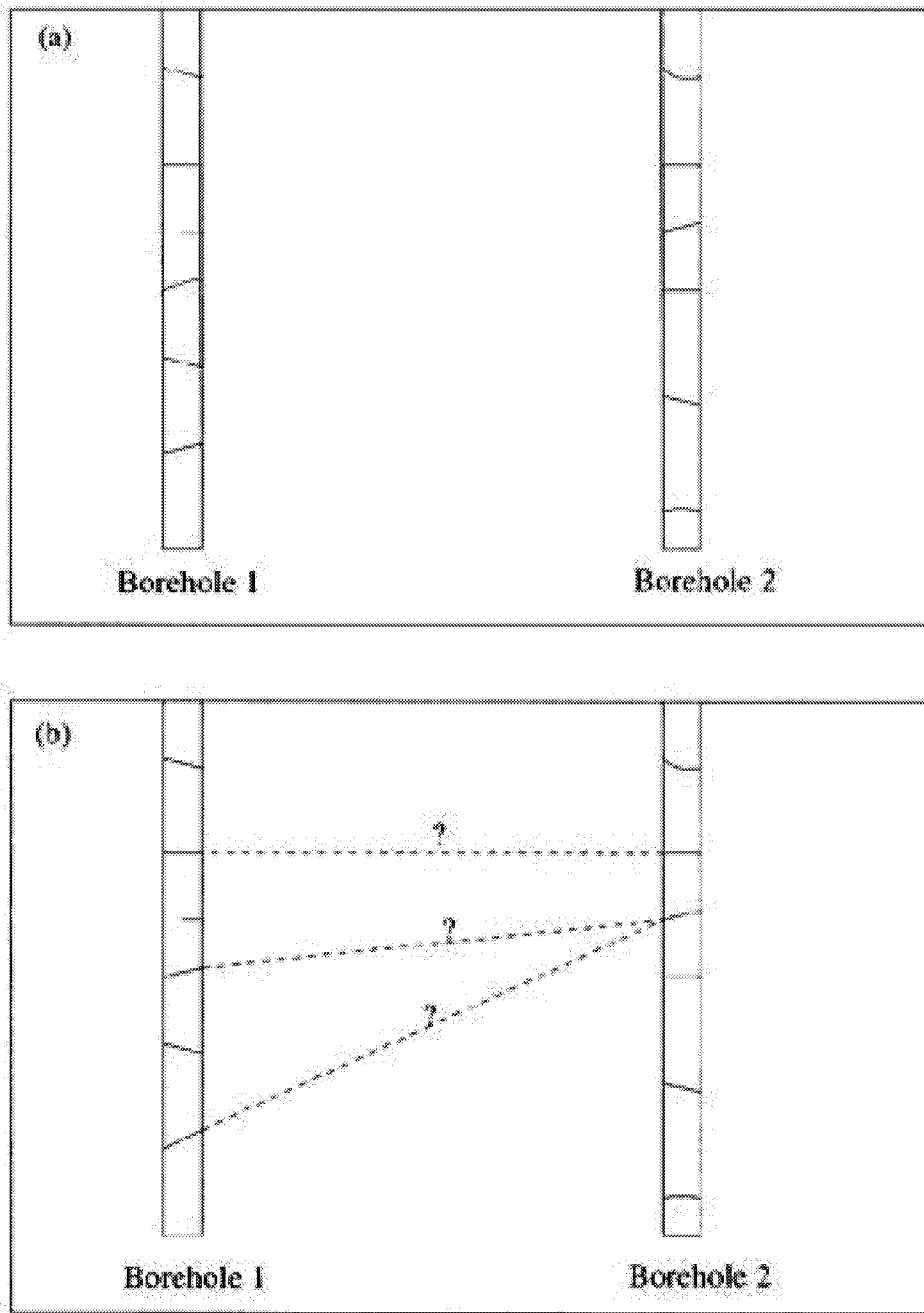
Figure 3-1 Fracture Interpolation
