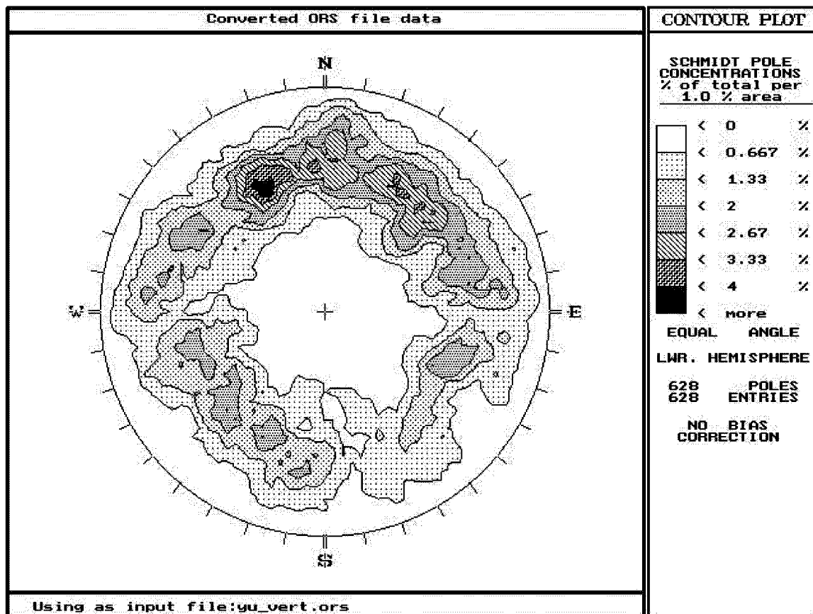
Figure 3-41 Contour Plot of Joint Orientations in Three Yates Wells
