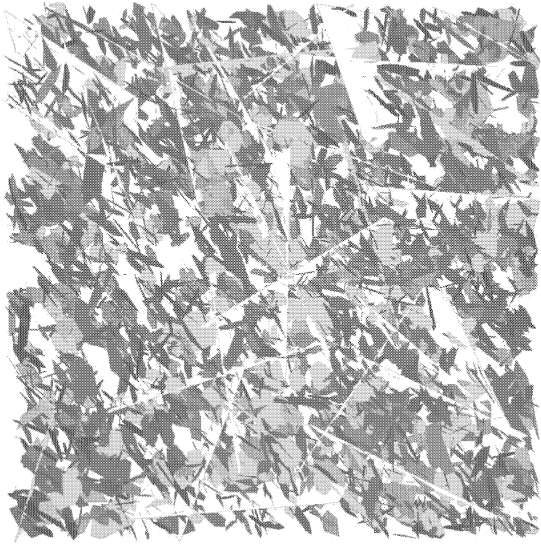
Figure 3-171: North Oregon Basin DFN model
