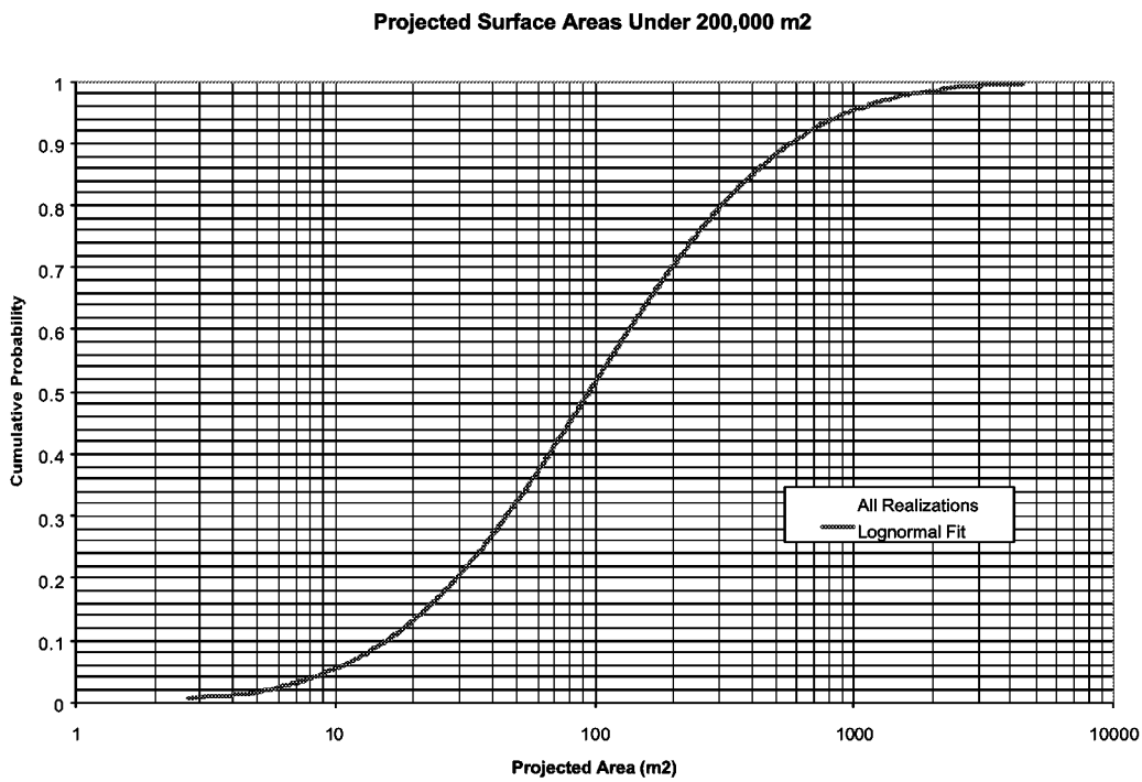
Figure 3-89 Compartment Projected Area Distribution, W1304
