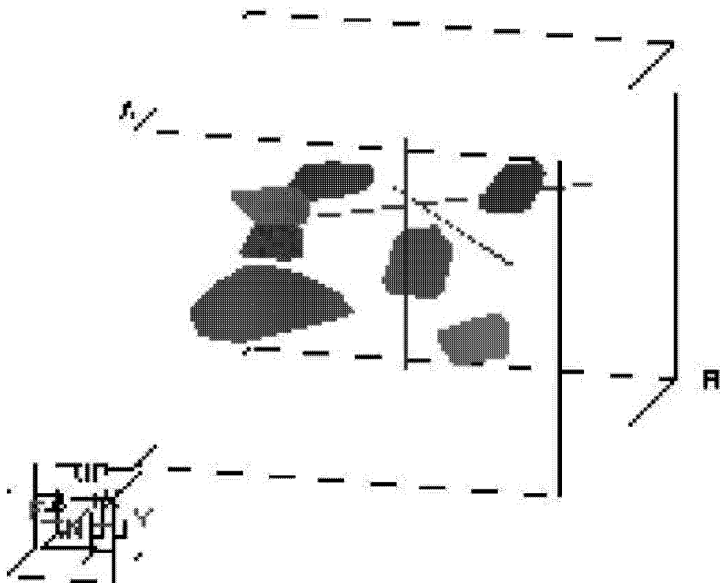
Figure 3-115 Compartments in North Oregon Basin Model with P_{32}=0.2
