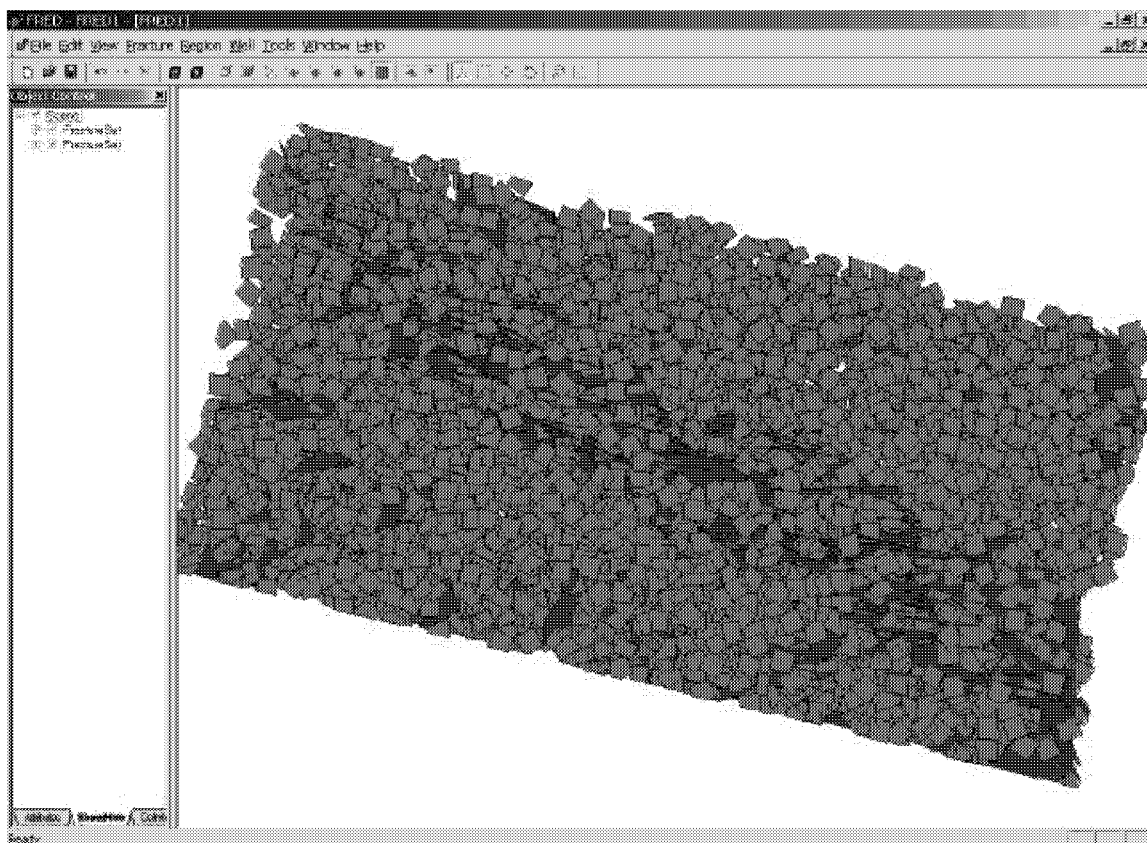
Figure 3-133: Full Fracture Set for Stoney Point, Fractures, and Matrix
