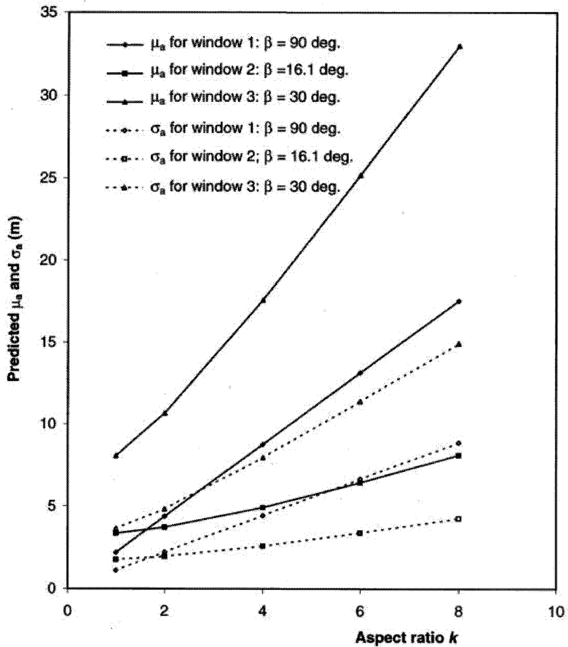
Figure 3-24 Variation of \mu_a and \sigma_a with aspect ratio k for assumed major axis orientation 1 ( 0^\circ/0^\circ ): assuming a lognormal distribution form of g(a)
