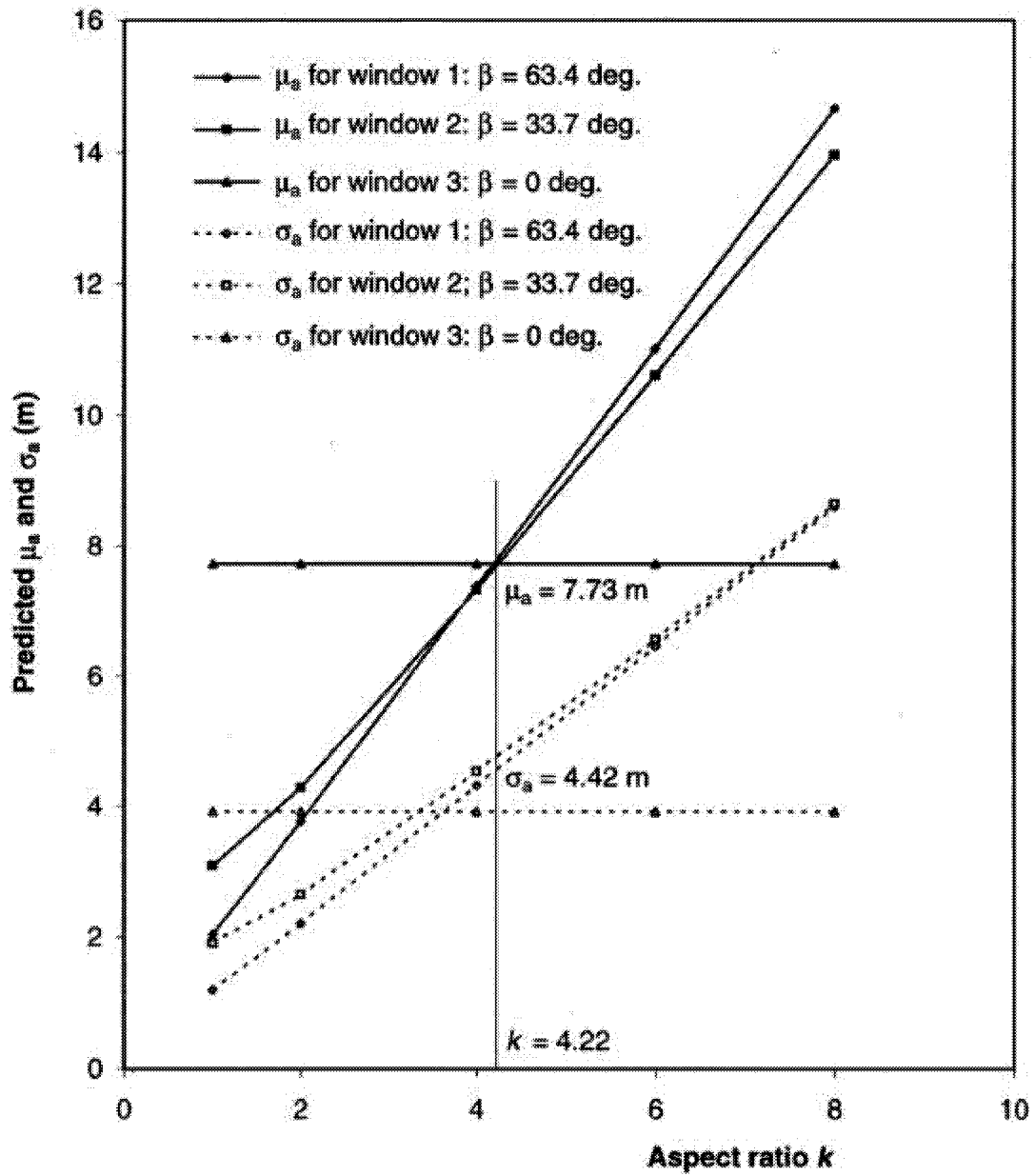
Figure 3-29 Variation of \mu_a and \sigma_a with aspect ratio k for assumed major axis orientation 2 ( 30^\circ/0^\circ ): assuming a Gamma distribution form of a
