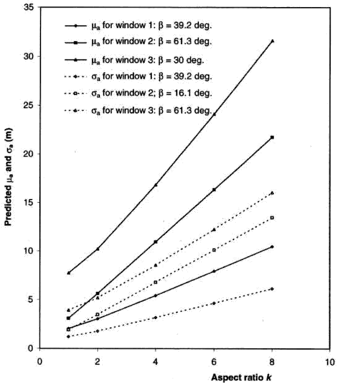
Figure 3-32 Variation of \mu_a and \sigma_a with aspect ratio k for assumed major axis orientation 3 ( 60^\circ/0^\circ ): assuming a Gamma distribution form of a
