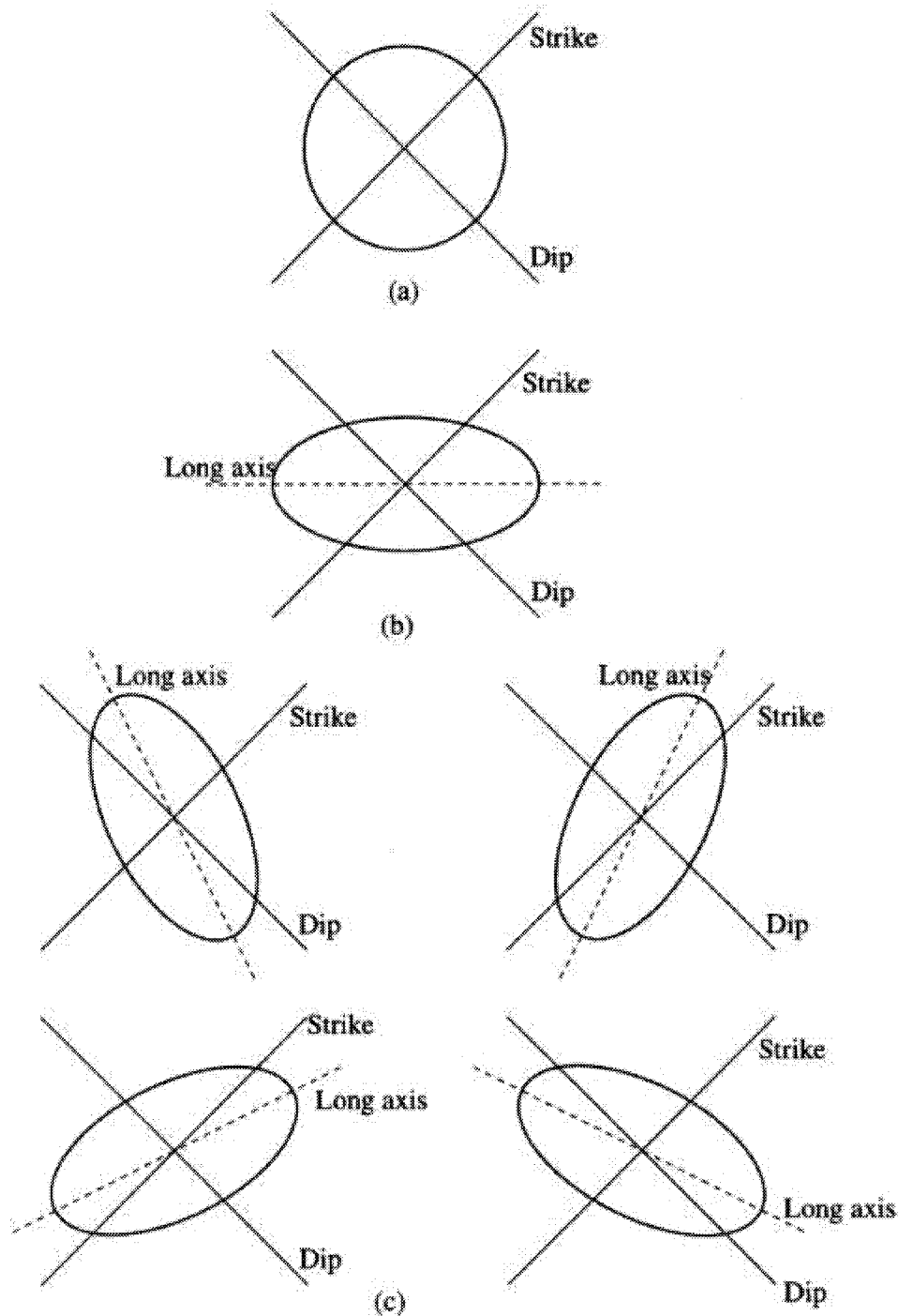
Figure 3-37 Three possible cases at which the average strike length is about equal to the average dip length: (a) Discontinuities are equidimensional (circular); (b) discontinuities are non-equidimensional (elliptical) with long axes in a single orientation. The discontinuities are oriented so that the average strike length is about equal the average dip length; and (c) Discontinuities are non-equidimensional with long axes such randomly oriented that the average strike length is about equal to the average dip length.
