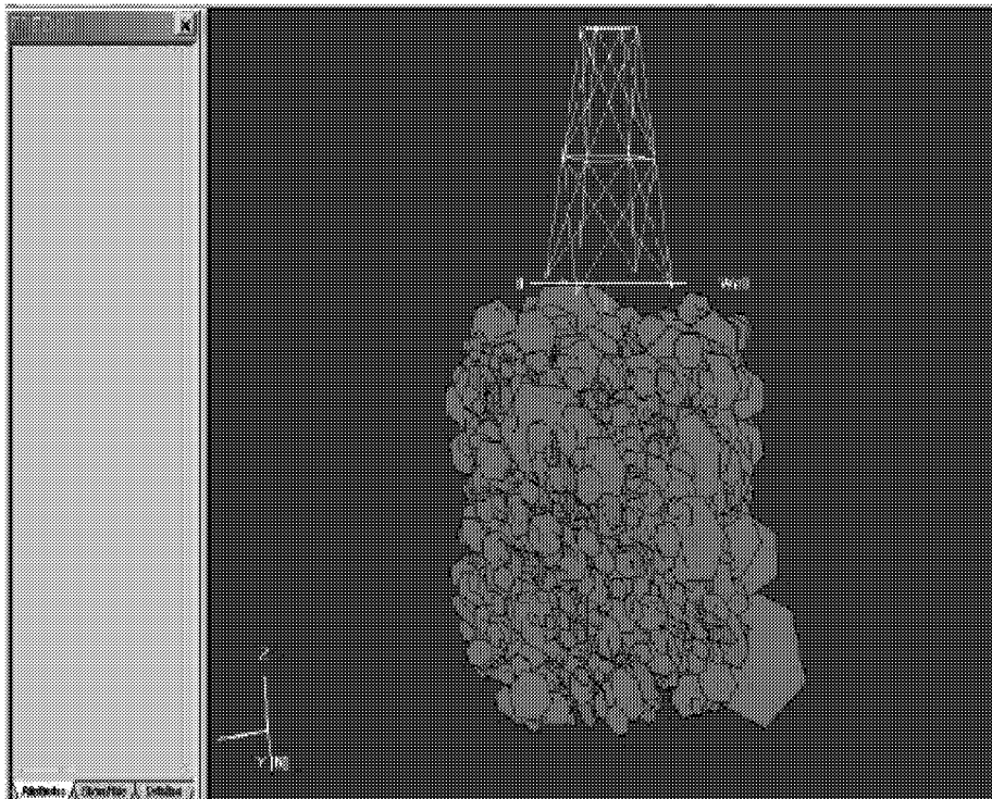
Figure 3-114 Tensleep Formation Water Injection DFN Study.
