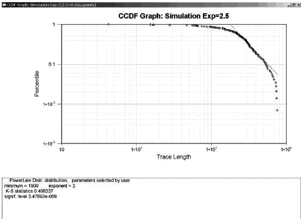
Figure 3-155 Simulation of ESE Lineaments, Exponent 2.5
