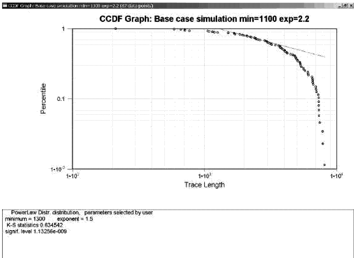
Figure 3-152 Simulation of ESE Lineaments, 1300 ft. Scale
