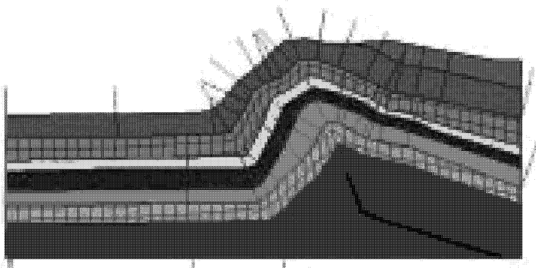
Figure 3-70 Goesec2D Palinspastic Reconstruction
