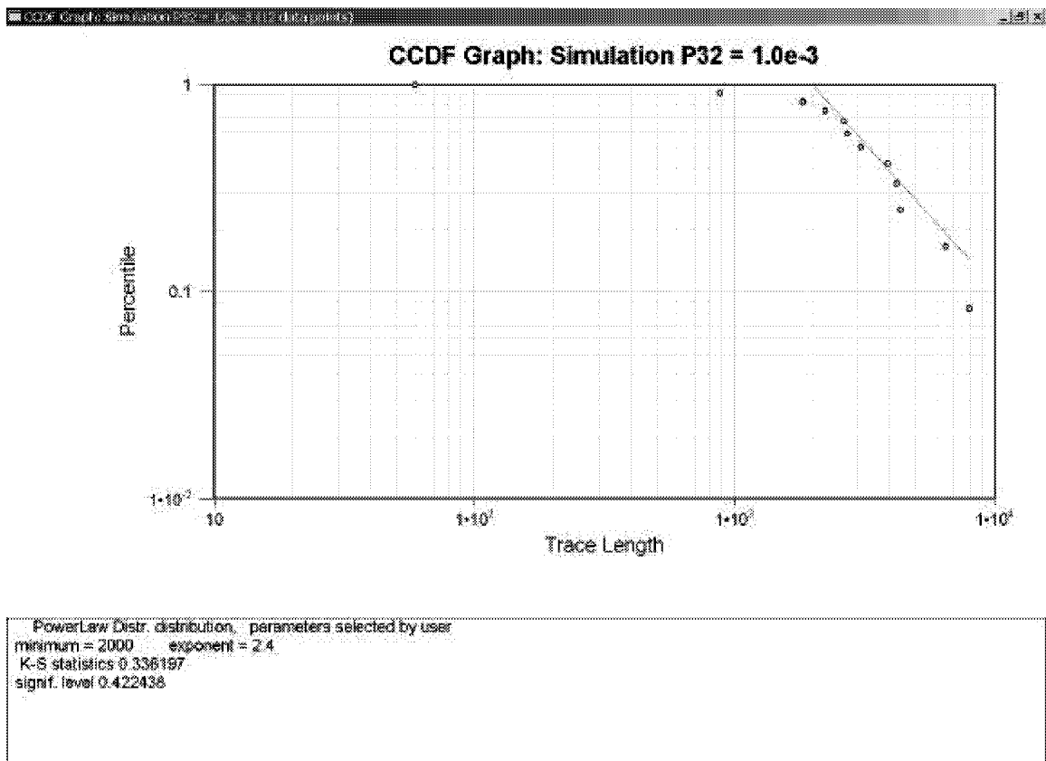
Figure 3-158: Simulation of ESE Lineaments, Intensity P_{32} = 0.001 \text{ m}^2/\text{m}^3
