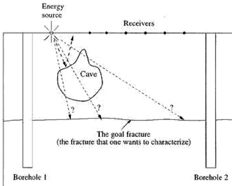
Figure 3-7 Loss of Seismic Signals Due to Karsts and Inclusions
