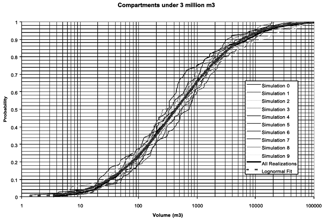
Figure 3-88 Compartment Volume Distribution, W1304
