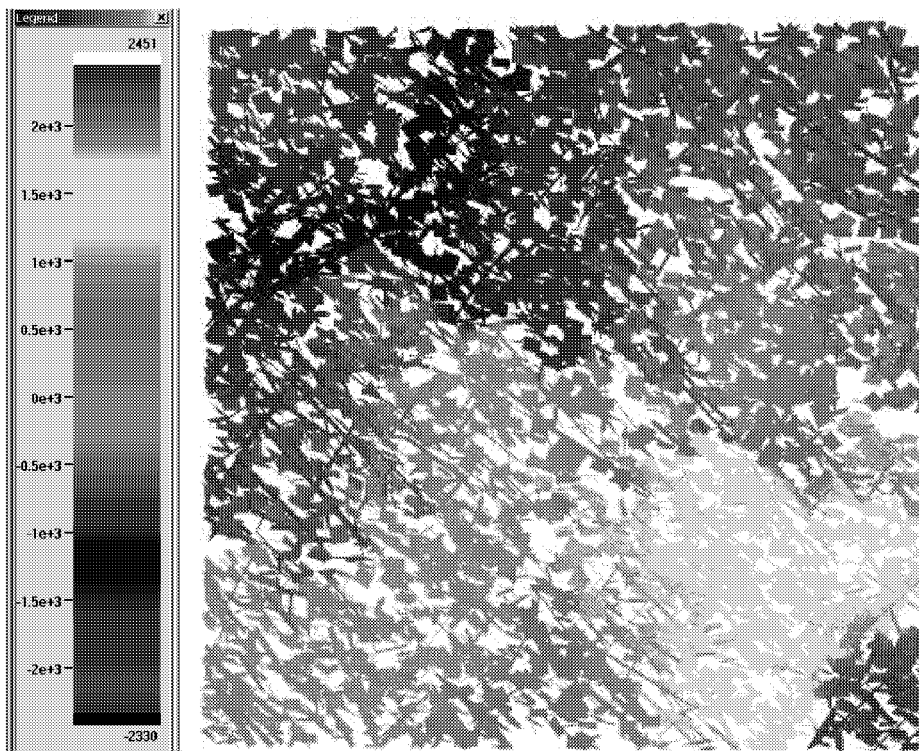
Figure 3-166: South Oregon Basin simulation pre gel. Time = 1 Hour
