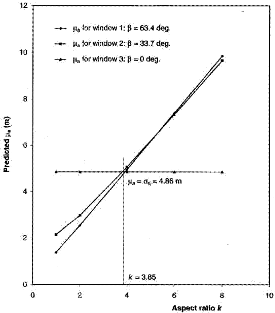
Figure 3-28 Variation of \mu_a with aspect ratio k for assumed major axis orientation 2 ( 30^\circ/0^\circ ): assuming a negative exponential distribution form of a
