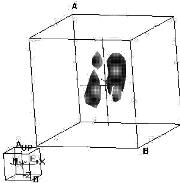
Figure 3-111 Tributary Volumes in South Oregon Basin Model for P_{32} = 0.2 Model
