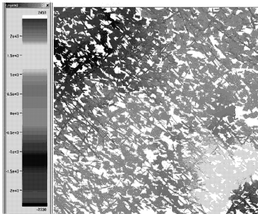
Figure 3-167: South Oregon Basin simulation after gel treatment reduces fracture permeability 1 order of magnitude
