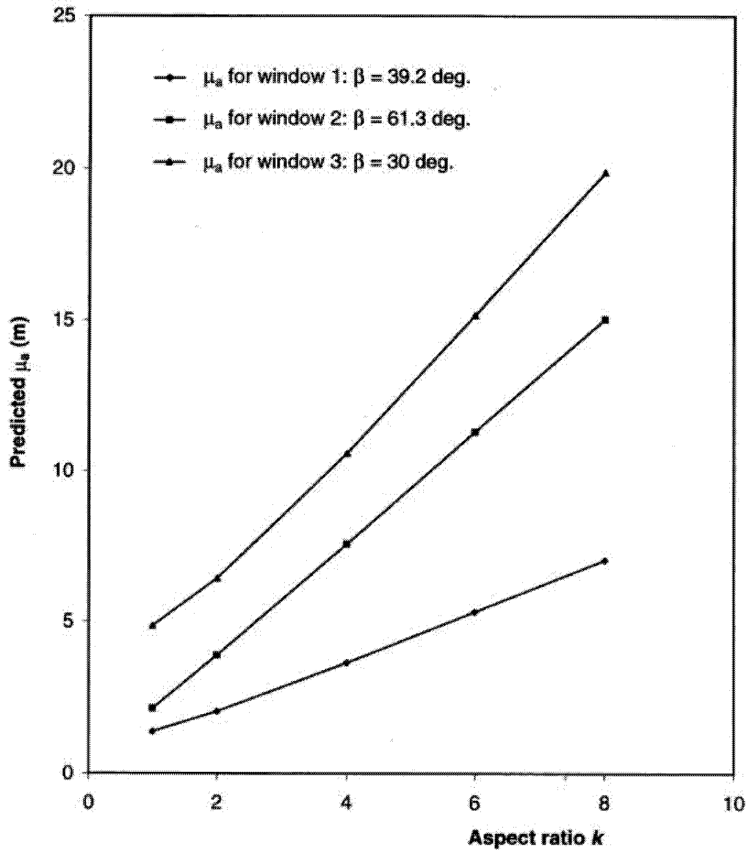
Figure 3-31 Variation of \mu_a with aspect ration k for assumed major axis orientation 3 ( 60^\circ/0^\circ ): assuming a negative exponential distribution form of a
