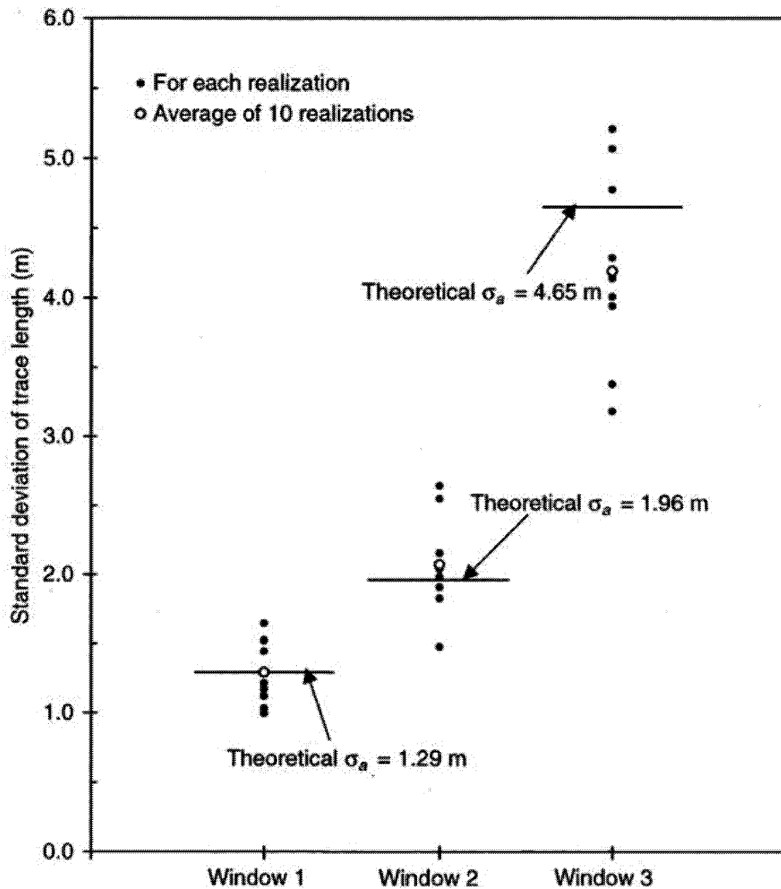
Figure 3-23 Comparison of the theoretical standard deviation of trace lengths with predicted standard deviation of trace lengths from simulations
