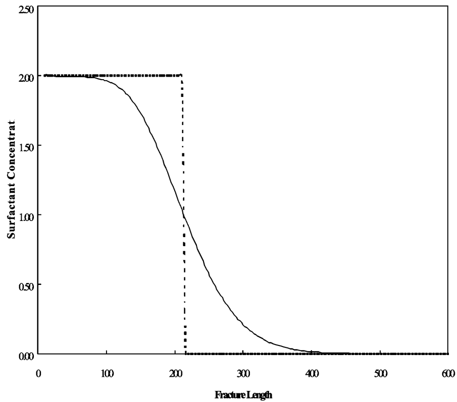
Figure 3-82 Surfactant Concentration Profile in Fracture
