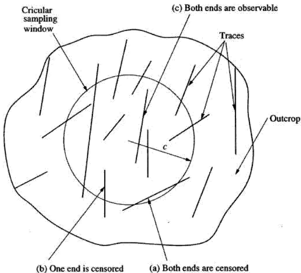
Figure 3-18 Discontinuities intersect a circular sampling window in three ways
