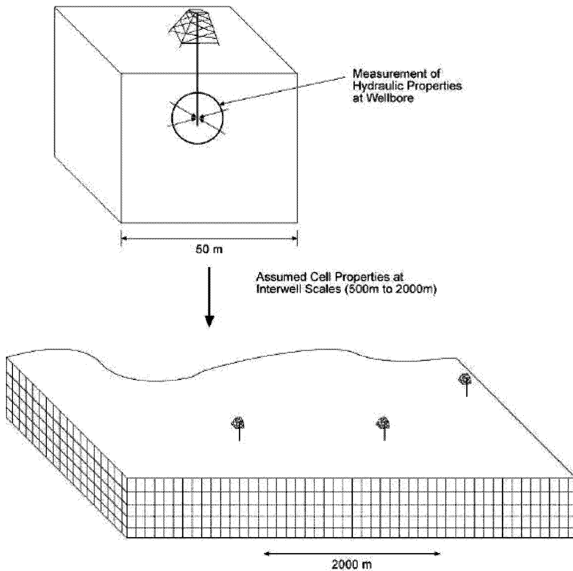
Figure 3-56 Data Scaling for Continuum Approaches
