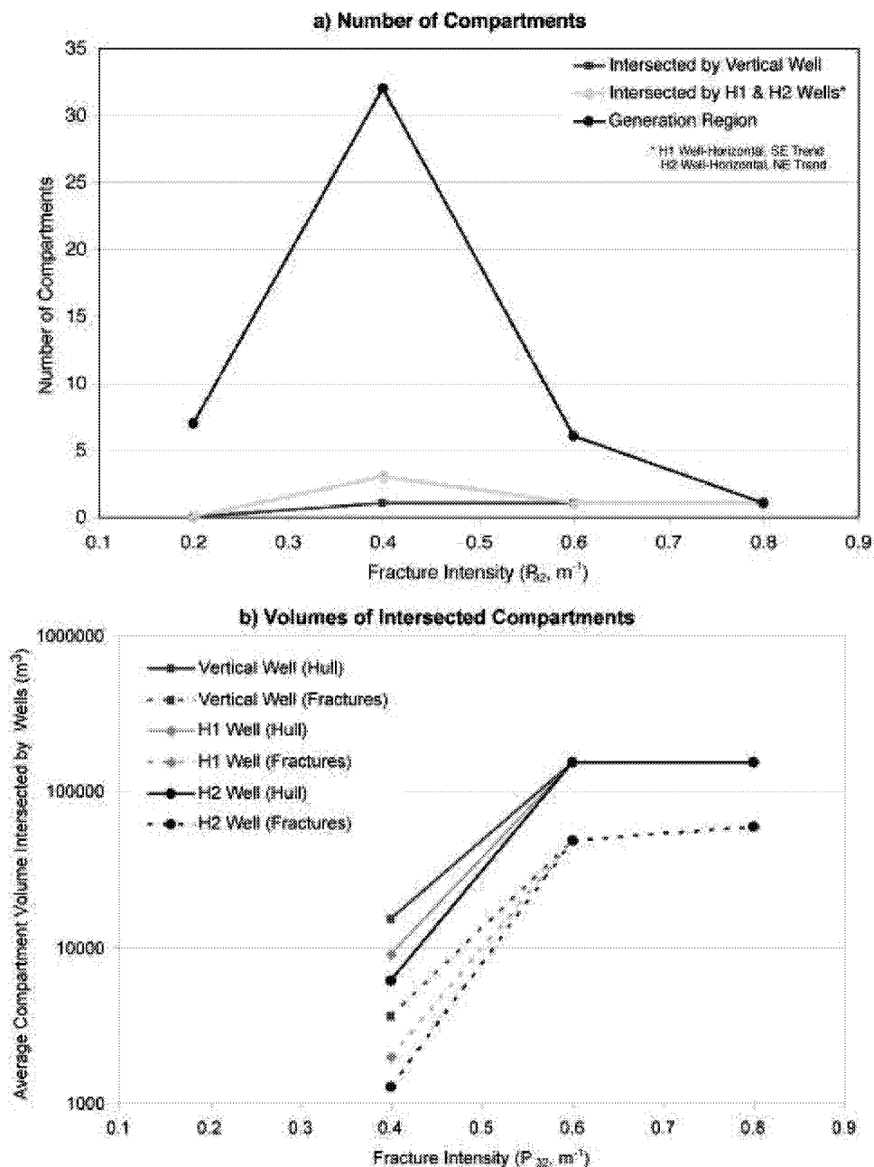
Figure 3-119 North Oregon Basin Tributary Volume Analysis
