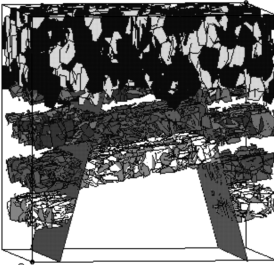
Figure 3-45 Example DFN Model for Size Analysis
