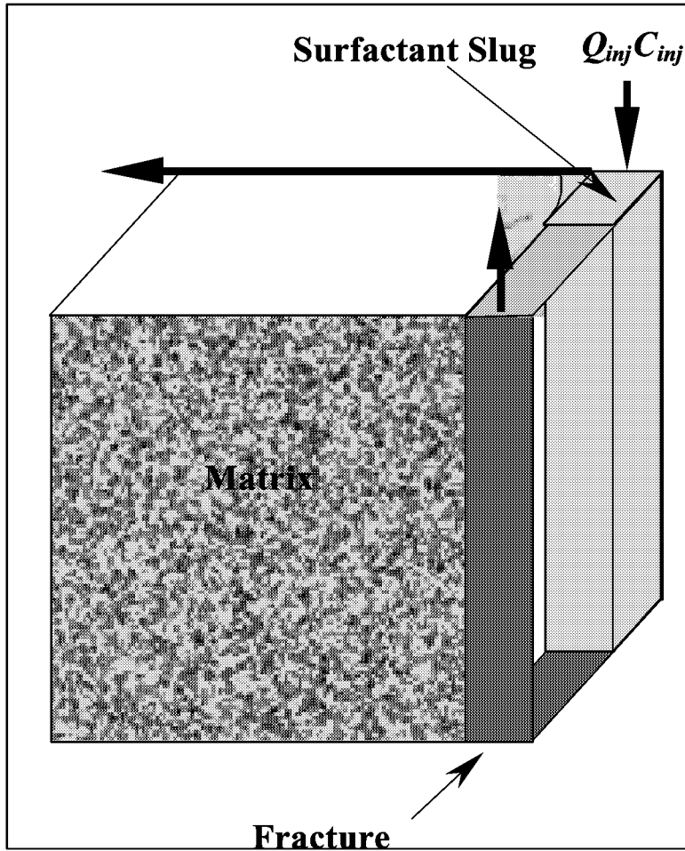
Figure 3-81 Conceptual Fracture Model
