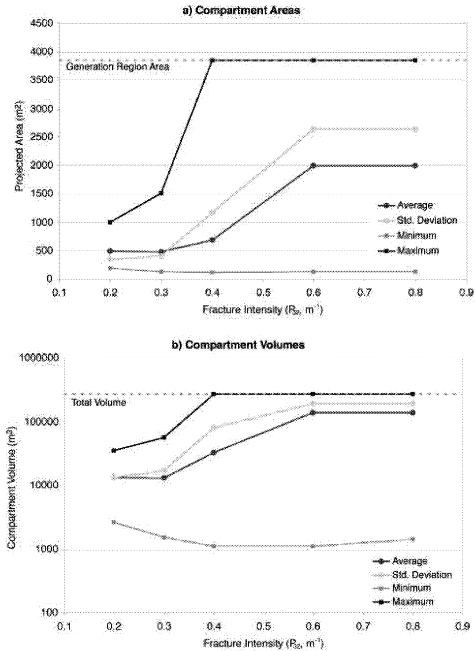
Figure 3-110 South Oregon Basin Compartmentalization Analysis
