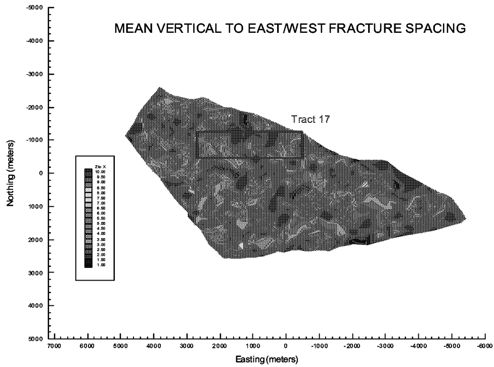
Figure 3-123: Mean Vertical to East/West Fracture Spacing
