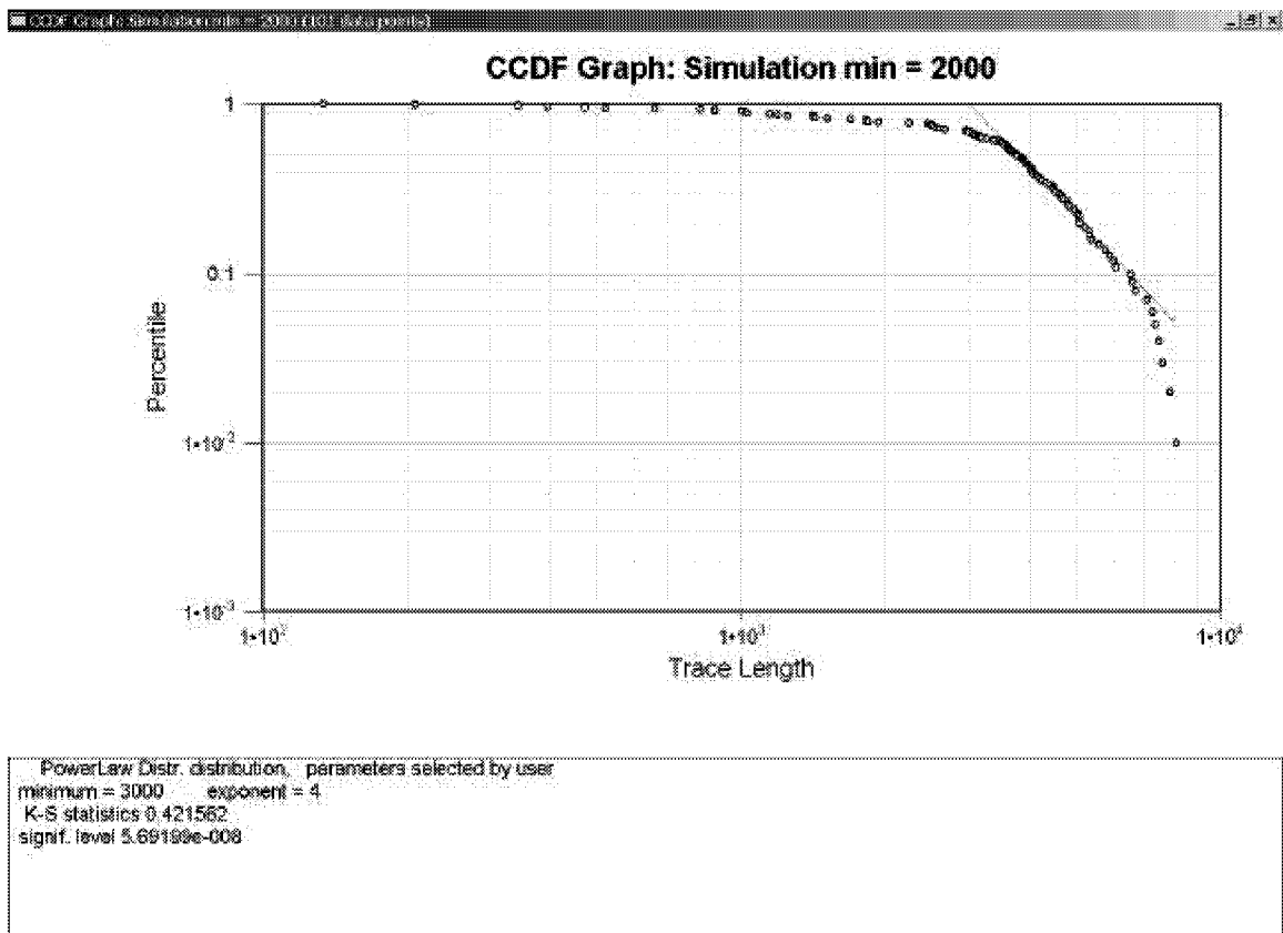
Figure 3-153: Simulation of ESE Lineaments, 2000 Ft. Scale
