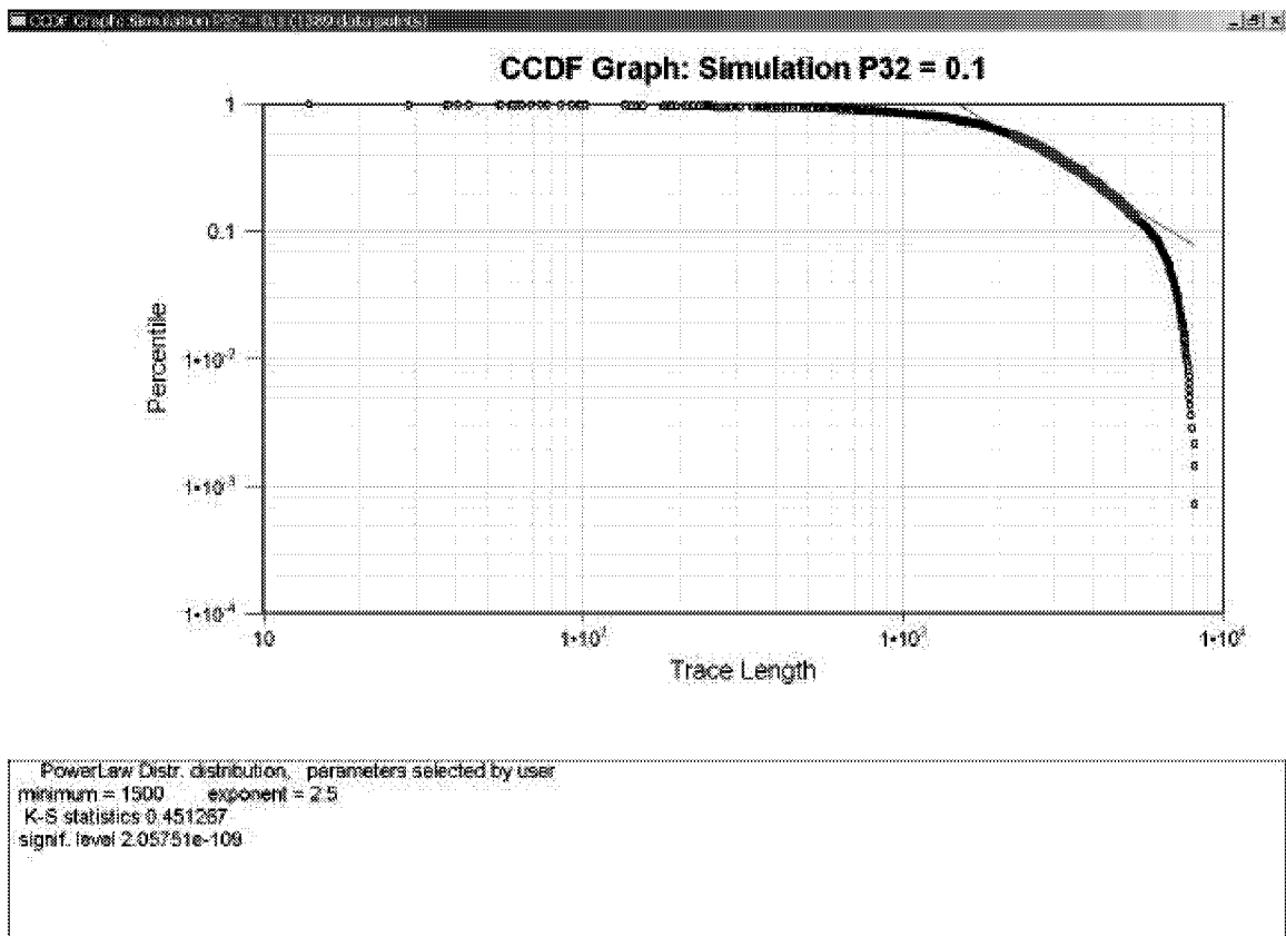
Figure 3-160: Simulation of ESE Lineaments, Intensity P_{32} = 0.01 \text{ m}^2/\text{m}^3
