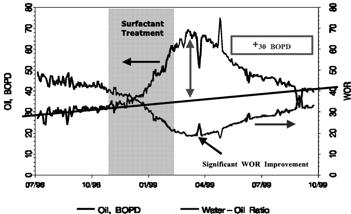
Figure 3-80 Response to injection over one mile away is observed almost immediately at a well which is producing at an elevation over 100 feet above the fracture flow feature taking the surfactant in the injection well
