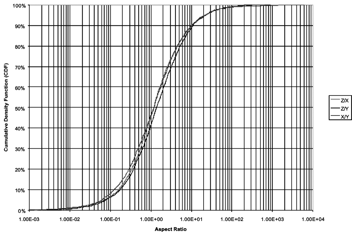
Figure 3-97 Distribution of Block Aspect Ratio
