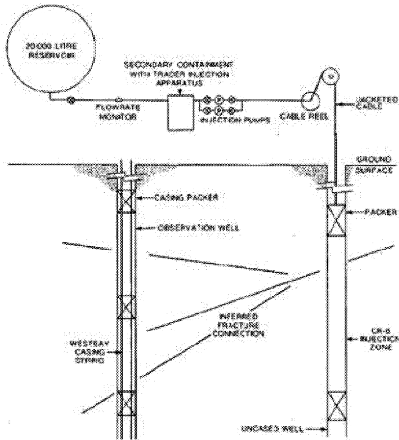
Figure 3-14 Tracer Testing at URL (Novakowski et al., 1985)
