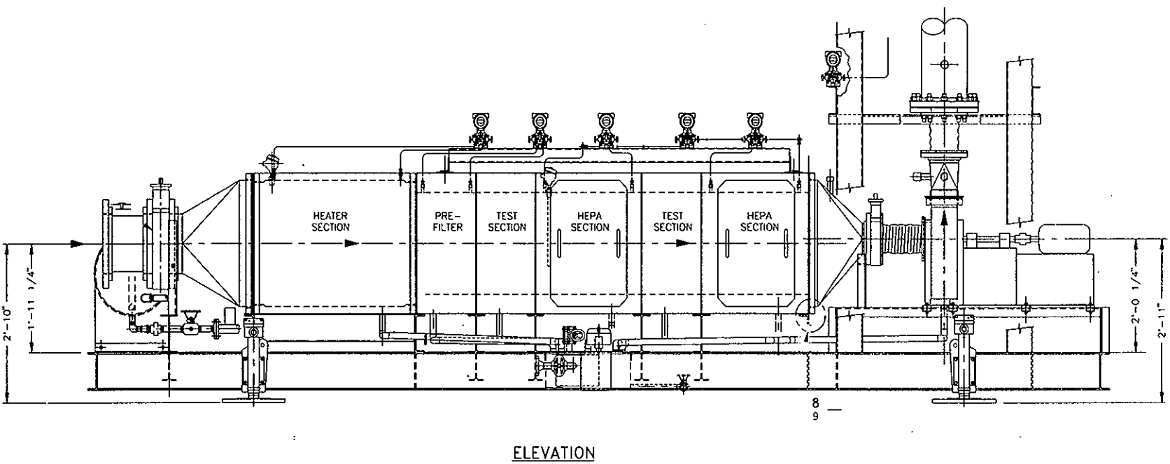
Figure 8-4. Ventilation Control System Diagram--Elevation View.
