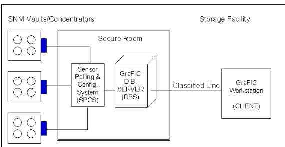
Figure 1 Typical Installation
