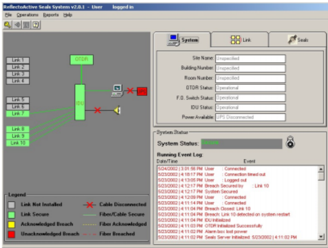
Figure 3 – ReflectoActive™ Seals User Interface
