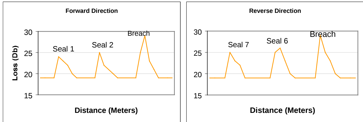
Figure 1 – Examples Of OTDR Plot (Seals 4 and 5 not secure)
