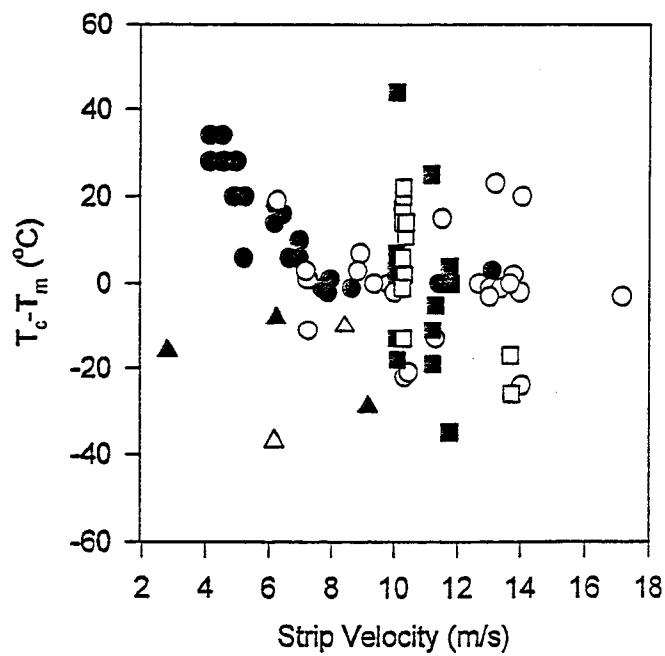
Figure 1.14. Comparison of predicted coiling temperature with mill measurement for A36 steel grades.
