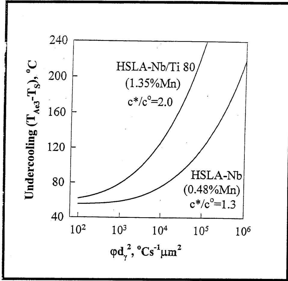
Figure 2.4.4: Effect of Mn on the transformation start temperature.
