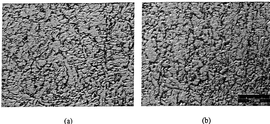
Figure 2.5.2: Comparison of (a) the microstructure for the HSLA-Nb/Ti80 steel obtained in a torsion test rolling simulation with (b) that of an industrially hot-rolled coil.
