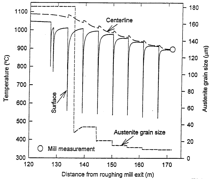
Figure 1.7 Predictions of thermal history and austenite grain size for a HSLA-Nb steel coil (Coil #565695)
