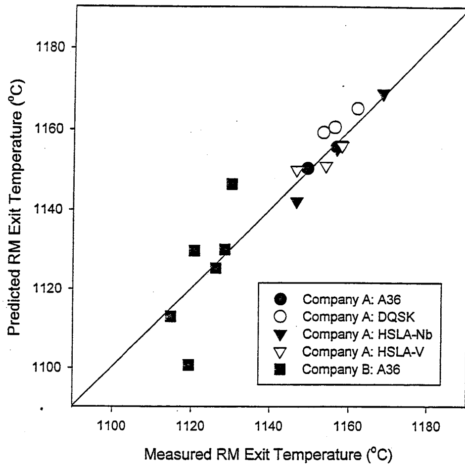
Figure 1.4 Comparison of predicted roughing mill exit temperature with mill measurements
