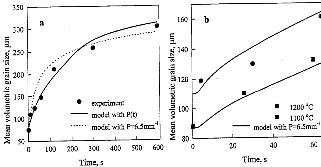
Figure 2.1.4: Comparison of predicted and measured grain growth in the HSLA-Nb/Ti 80 steel for reheating at 1250 °C (a) and after recrystallization (b).
