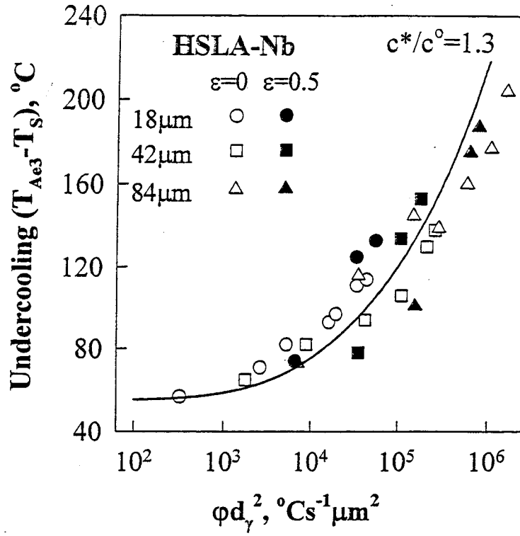
Figure 2.4.3: Effect of retained strain on the transformation start temperature, T_s , in HSLA-Nb steel as a function of the cooling rate, \phi , and the austenite grain size, d_\gamma .
