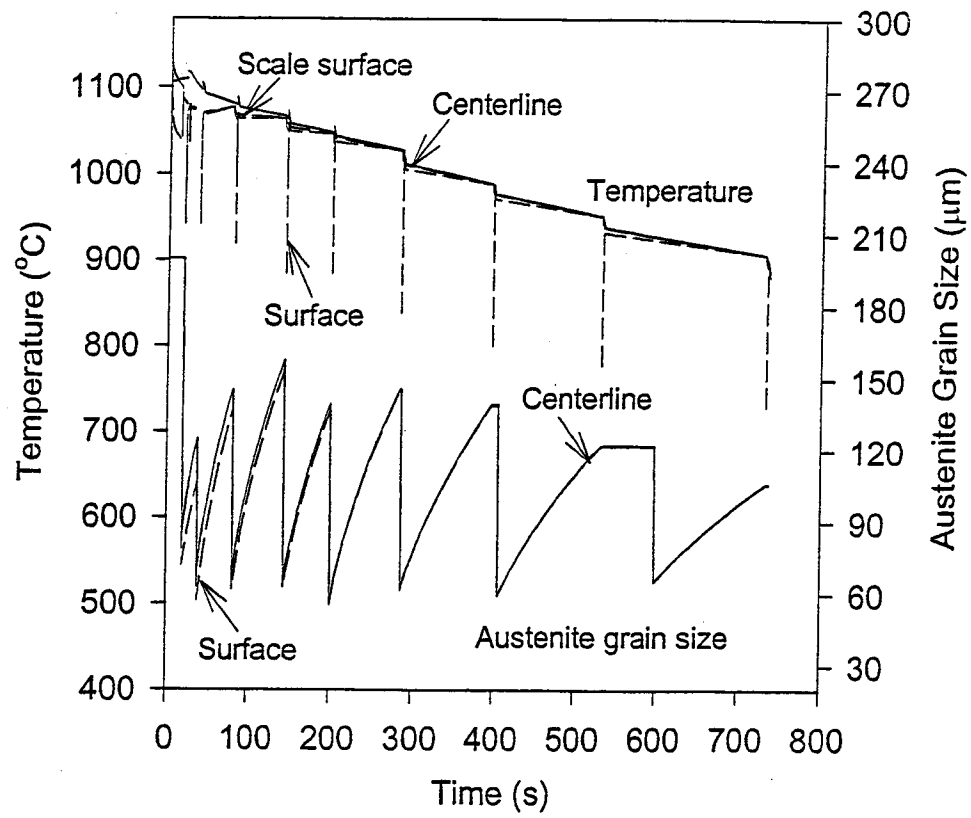
Figure 1.17 Time-temperature profile predicted by Steckel mill model for a Steckel mill rolling schedule.
