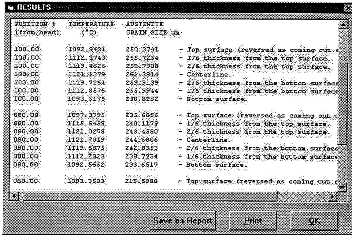
Figure 1.6. Temperature through the workpiece thickness at the coilbox exit.
