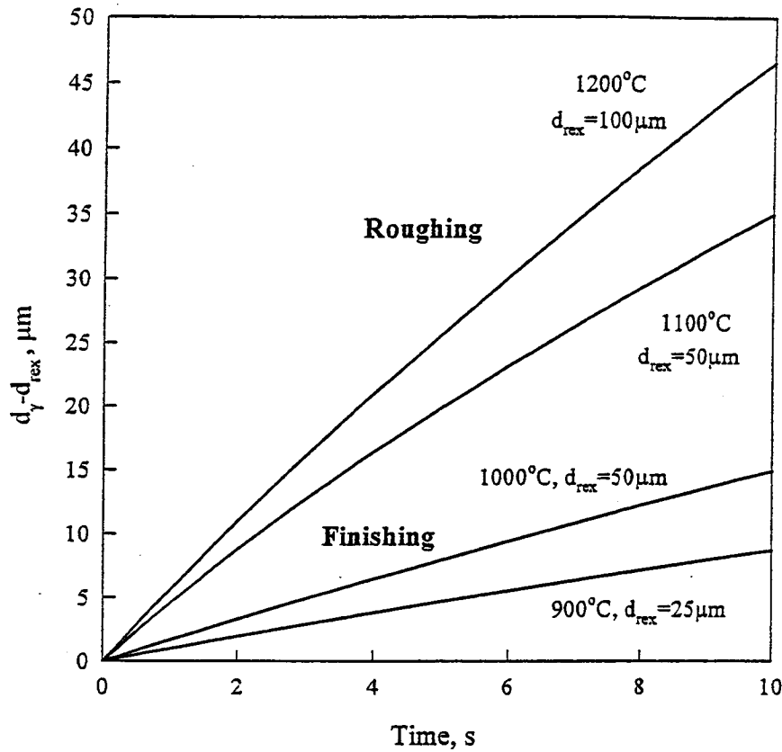
Figure 2.1.2: Estimation of grain growth after completion of recrystallization for rough and finish mill conditions for the DQSK steel.
