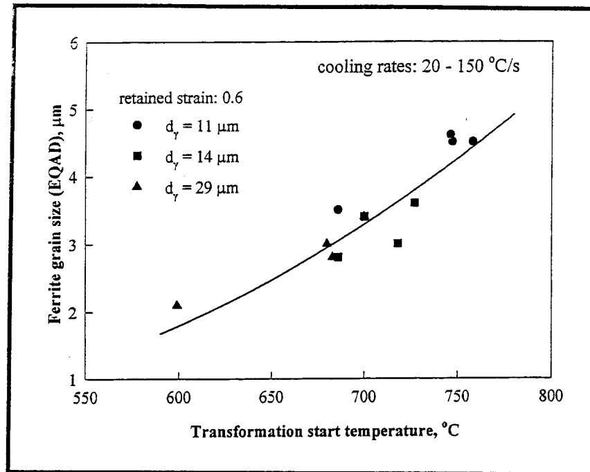
Figure 2.4.6: Ferrite grain size in the HSLA-Nb/Ti80 steel as a function of the transformation start temperature; solid line indicates the model prediction.
