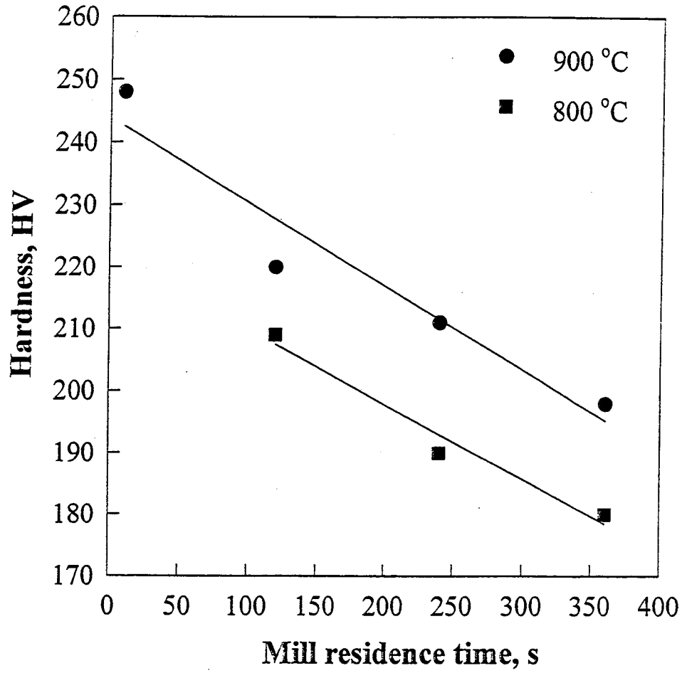
Figure 2.3.1: Strength of HSLA-Nb/Ti80 as a function of rolling temperature and mill residence time, as observed in torsion simulations.
