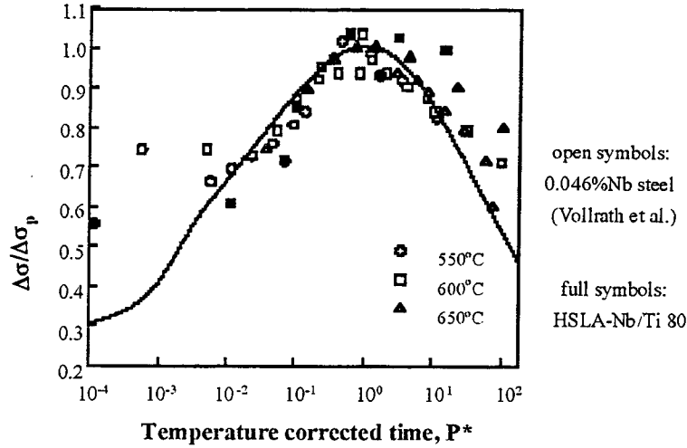
Figure 2.3.3: Precipitation hardening in Nb containing HSLA steels.
