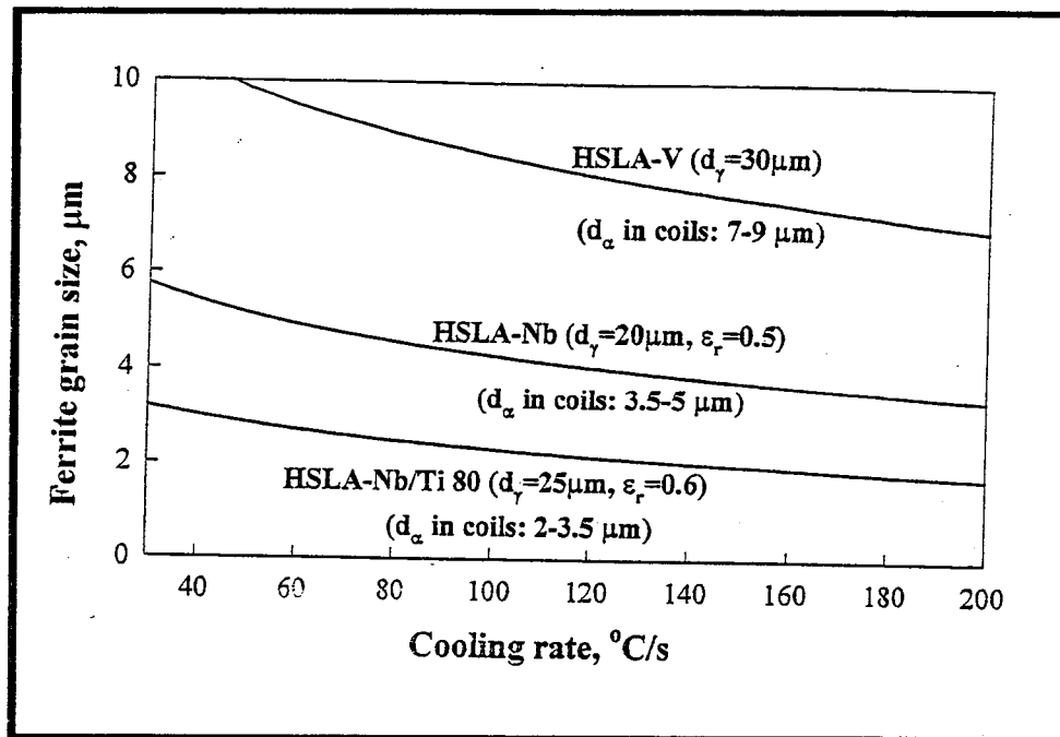
Figure 2.4.7: Ferrite grain size predictions for three classes of HSLA steels.
