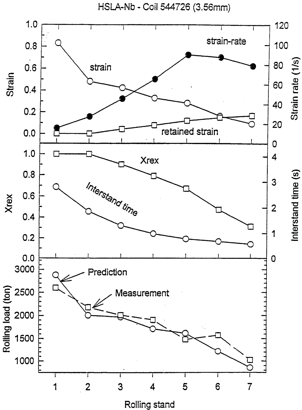
Figure 1.9 Predictions of strain, strain-rate, retained strain, fraction of recrystallization, and rolling loads during 7-pass finishmill rolling.
