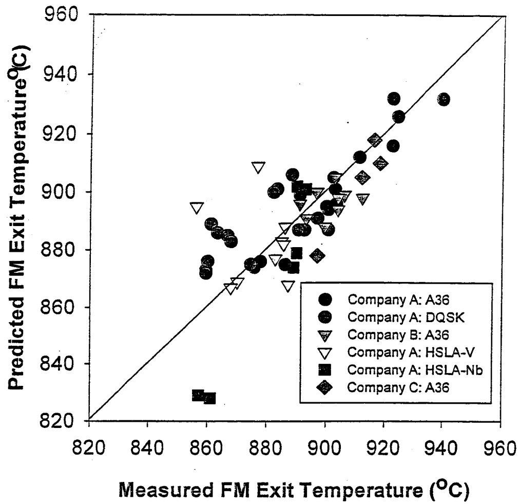
Figure 1.8 Comparison of predicted and measured finishmill exit temperature.
