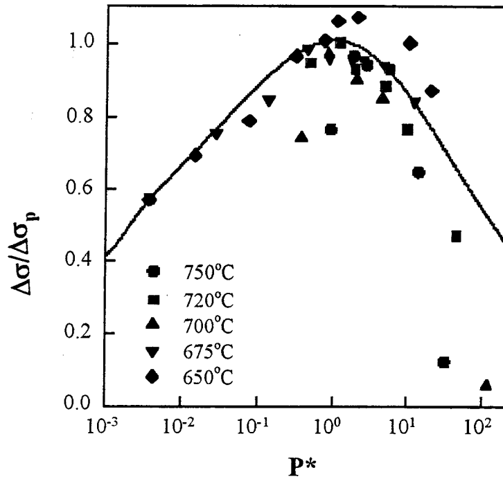
Figure 2.3.2: Precipitation hardening in the HSLA-V steel.
