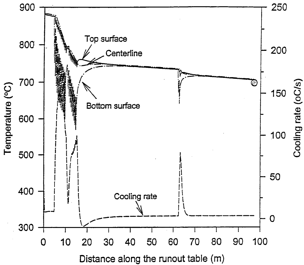
Figure 1.15 Predictions of thermal profile of strip during runout table cooling for HSLA-V steel coil #480733 (4.0mm).
