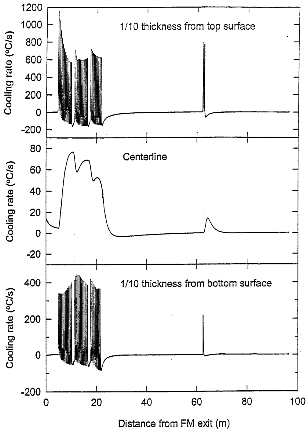
Figure 1.13 Cooling rate at the different position through the thickness for 0.17 pct. Carbon steel during ROT Cooling (9.8mm).
