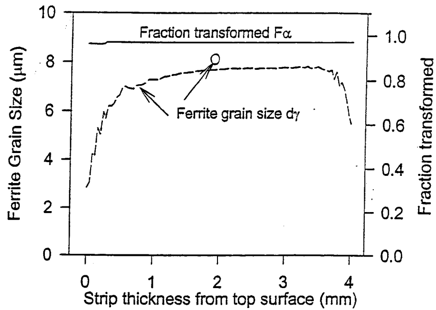
Figure 1.16a Predictions of Ferrite grain size and fraction of ferrite transformed for acHSLA-V steel coil #480733 (4.0mm).
