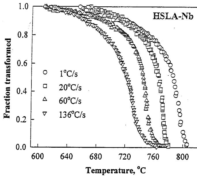
Figure 2.4.1: Austenite decomposition kinetics for different cooling rates in HSLA-Nb steel without retained strain and d_v = 18 \mu\text{m} .
