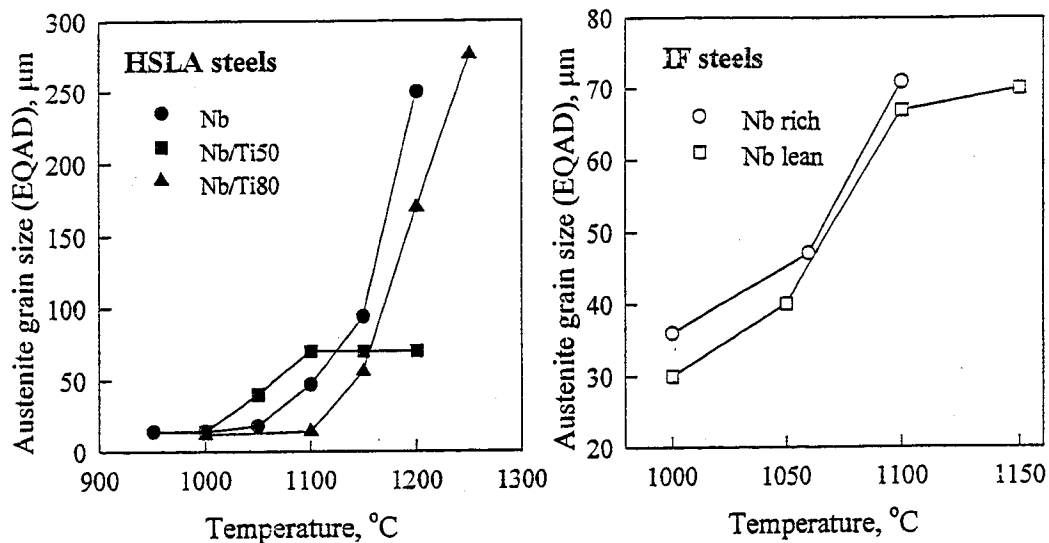
Figure 2.1.3: Austenite grain size as a function of temperature for holding times of 600 s for HSLA steels and IF steels.
