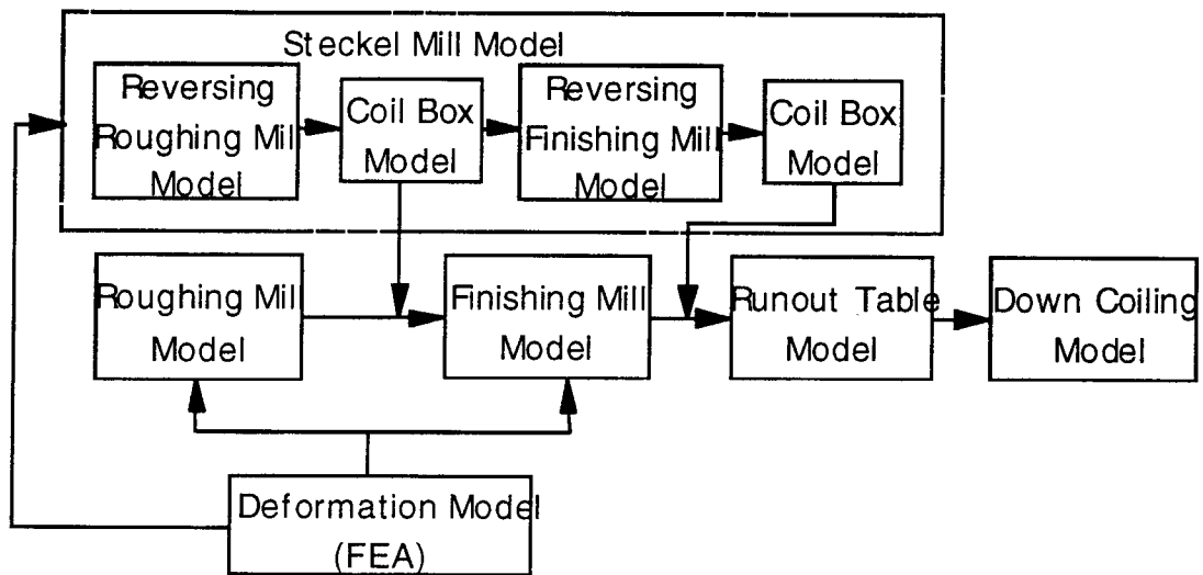
Figure 1.2. The structure of Hot Strip Mill Model
