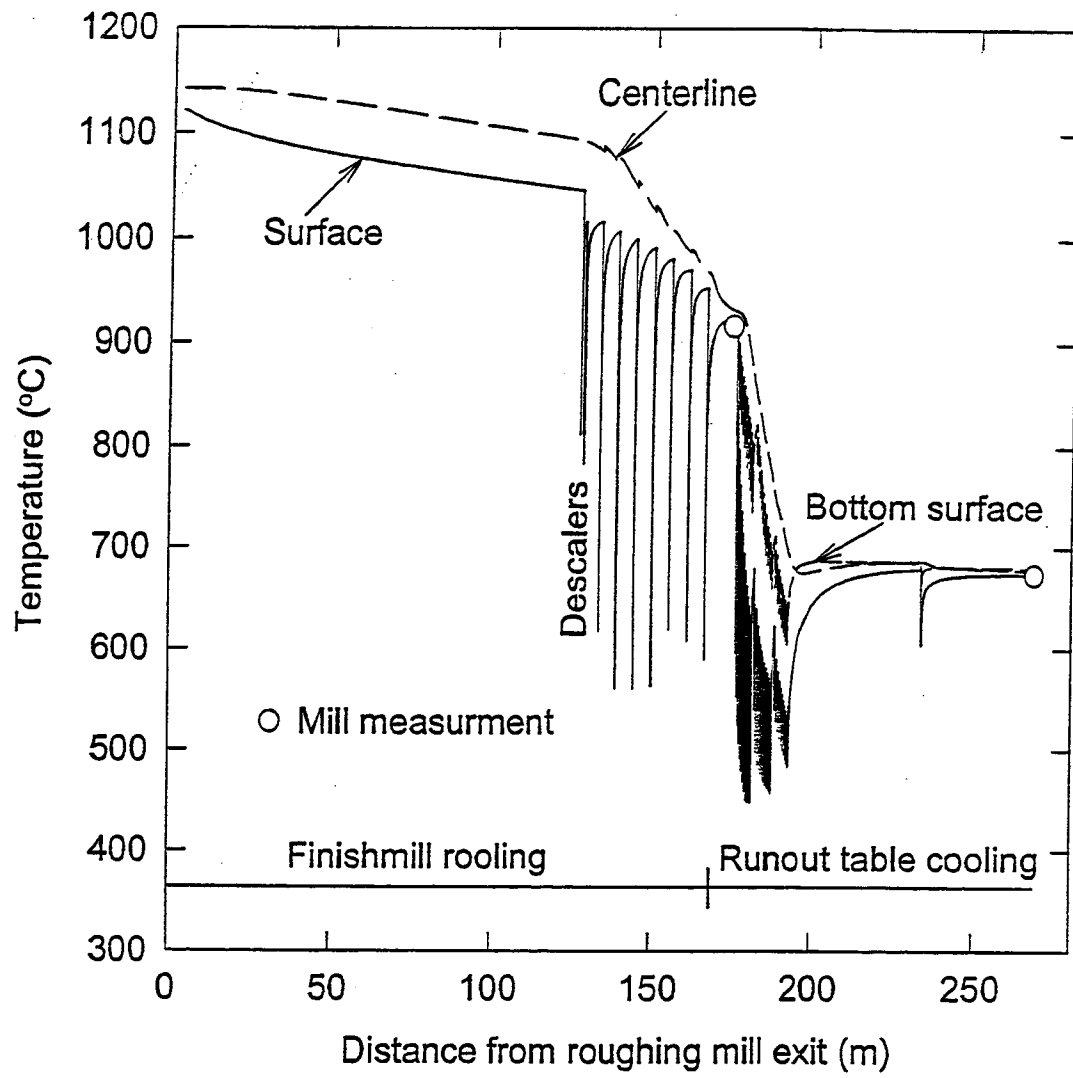
Figure 1.10 Thermal history from finishmill rolling to runout table cooling for 0.17% carbon steel with regular rolling schedule and temperature 1121° C at roughing exit.
