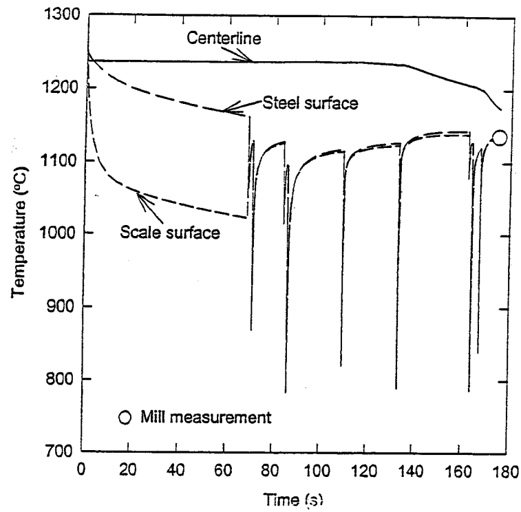
Figure 1.3 Thermal history during rough rolling for HSLA-Nb steel. (Coil #544726, USS)
