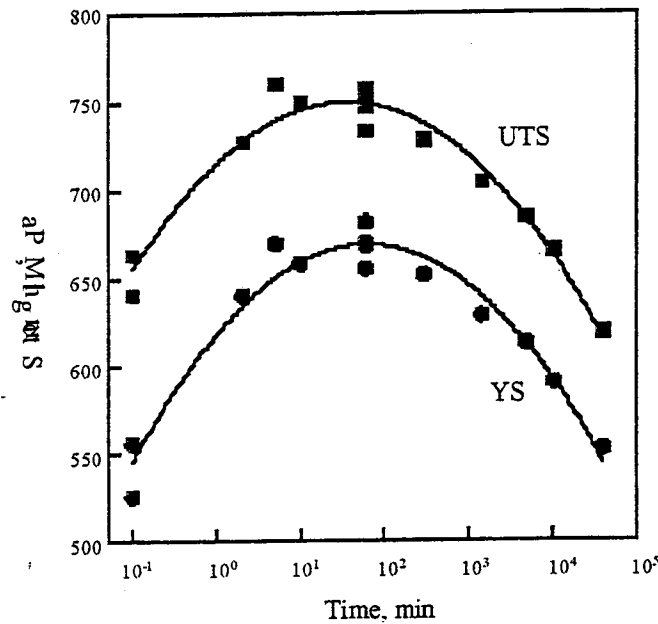
Figure 2.5.3: Mechanical properties of HSLA-Nb/Ti80 torsion samples during aging at 650°C.
