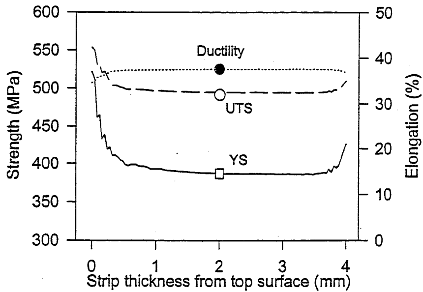
Figure 1.16b Predictions of mechanical properties for a HSLA-V Steel, coil #480733 (4.0mm).
