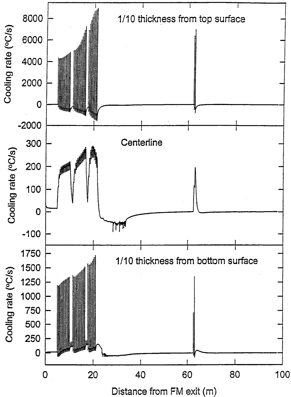
Figure 1.11 Cooling rate at different location through the thickness for 0.17 pct. Carbon steel during ROT cooling (2.6mm).
