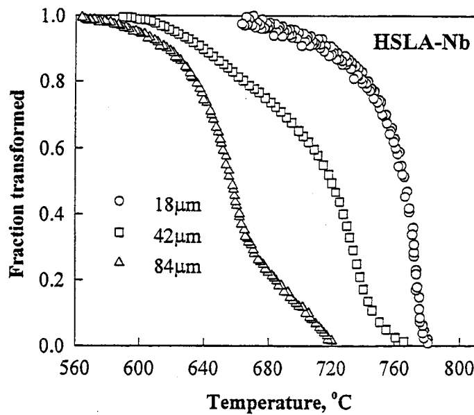
Figure 2.4.2: Austenite decomposition kinetics for initial austenite grain sizes in HSLA-Nb steel without retained strain at a cooling rate of 20^\circ\text{C/s} .
