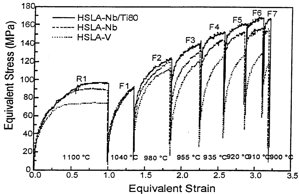
Figure 2.5.1: Comparison of the hot deformation behavior of the HSLA-V, HSLA-Nb and HSLA-Nb/Ti 80 steels.
