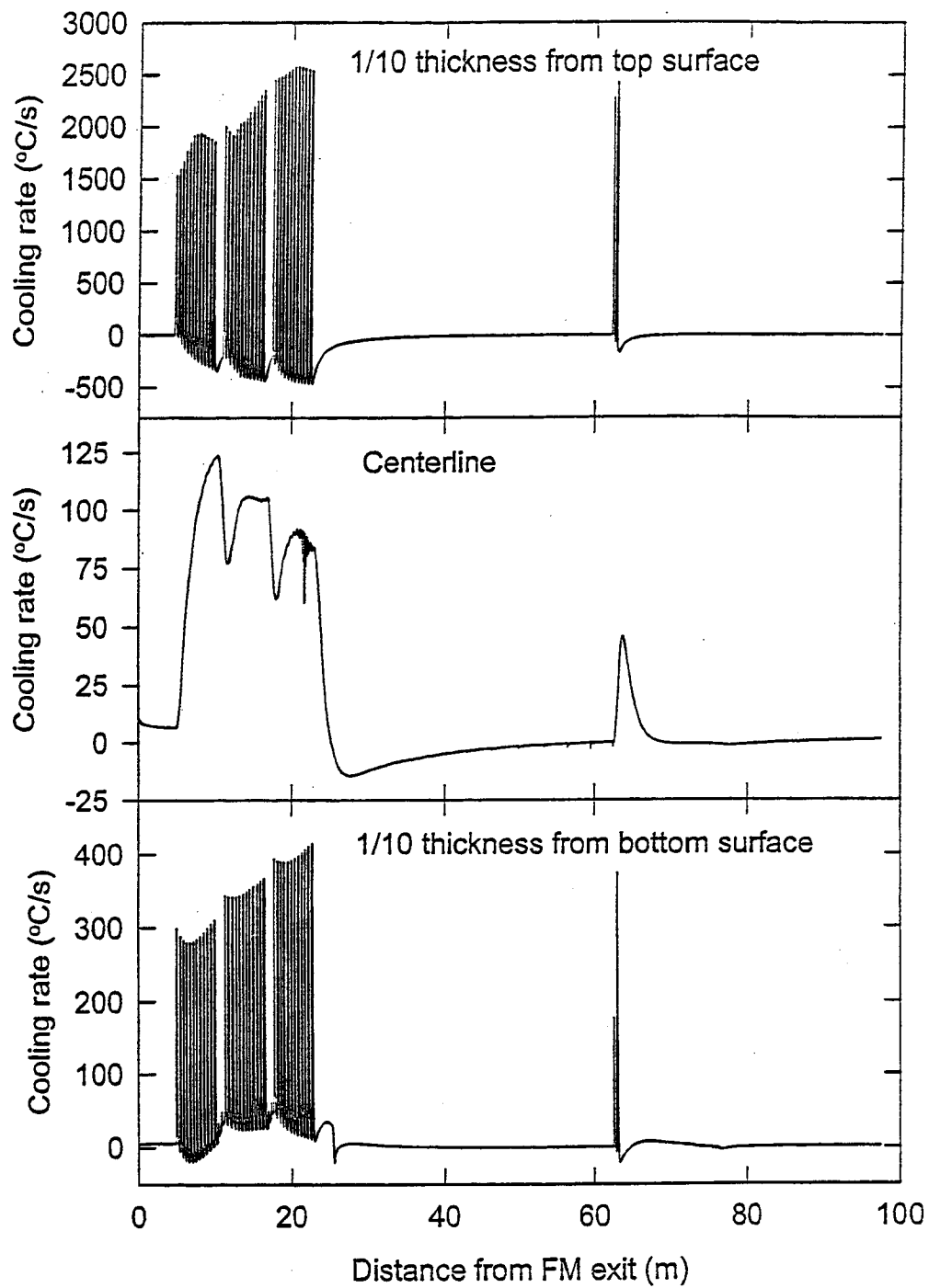
Figure 1.12 Cooling rate at different location through the thickness for 0.17 pct. Carbon steel during ROT cooling (6.2mm)
