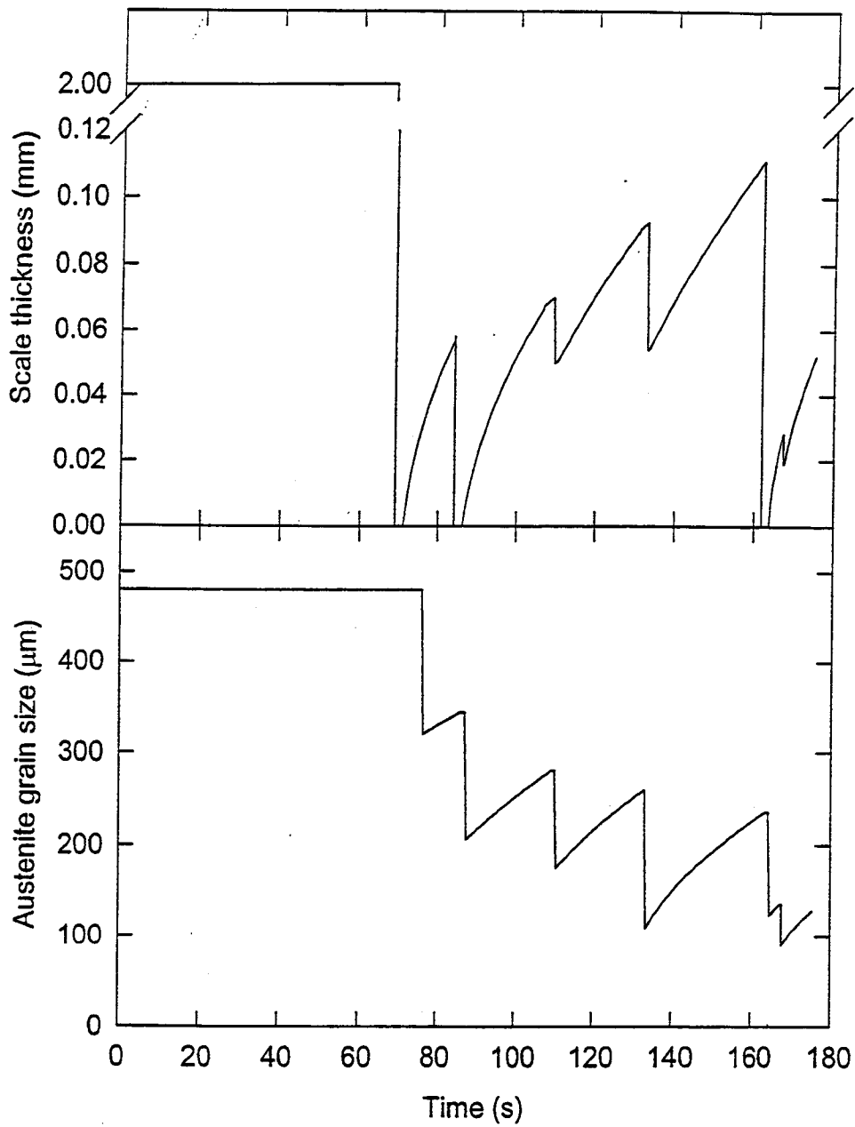
Figure 1.5 Time-oxide scale growth and time-austenite grain size profiles predicted by roughing mill model during 6-pass rough rolling for a HSLA-Nb steel.
