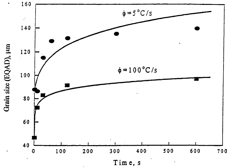
Figure 2.1.1 Austenite grain growth for the as-received A36 steel after heating to 1100 °C at different rates, \phi .
