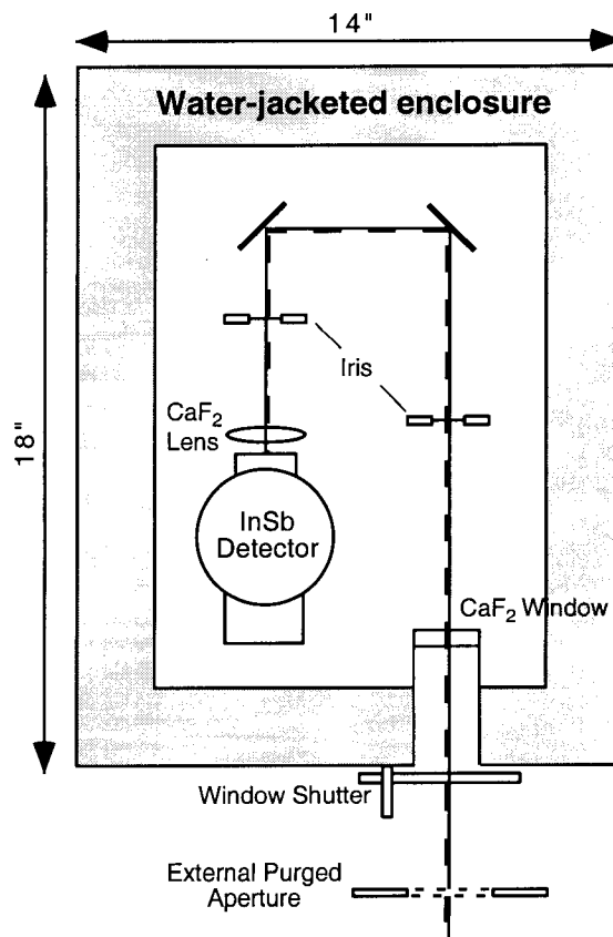
Figure 30. Layout for receiver module in laser-absorption off-gas sensor prototype.
