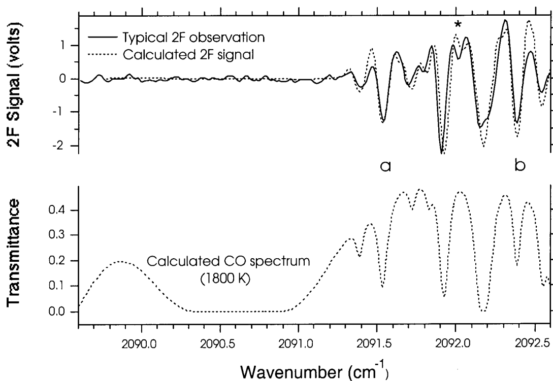
Figure 23. Calculated transmittance spectrum of CO at 1800° K (lower, dashed curve). Experimental 2f signal measured during O 2 blowing at Sparrows Point (upper, solid curve), and calculated 2f signal using 1800° K transmittance spectrum as input (upper, dashed curve). Features identified as “a” and “b” are used to calculate CO temperature and are discussed in the text. Feature marked with asterisk was earlier attributed to CO 2 .
