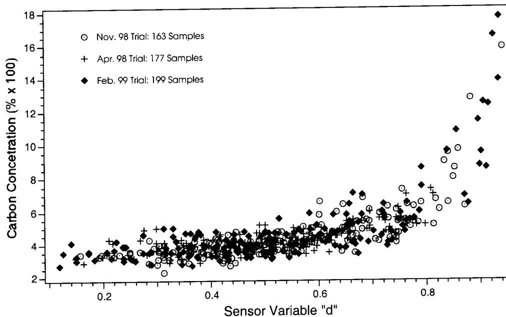
Figure 39. Dependence of final turndown bath carbon concentration on off-gas infrared emission sensor variable “d” (defined above, Fig. 32). Data are shown for the April 1998 field trial, and two supplementary field trials in November 1998 and February 1999.
