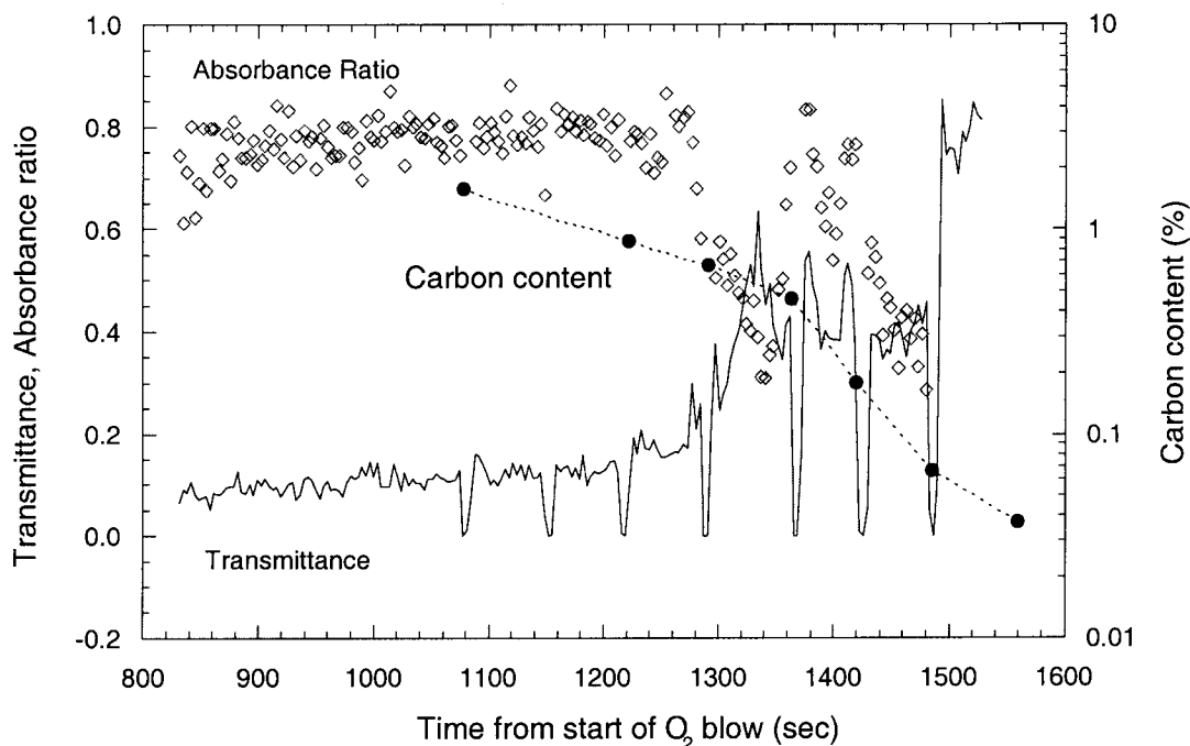
Figure 12. Comparison of metal carbon content (filled circles, right-hand axis) with laser transmittance (solid curve, left-hand axis) and a ratio of absorption line intensities, \text{Abs}_{\text{CO}}/(\text{Abs}_{\text{CO}} + f \cdot \text{Abs}_{\text{CO}_2}) (diamonds, left-hand axis) during oxygen blow. The sample lance causes dips in the laser transmittance.
