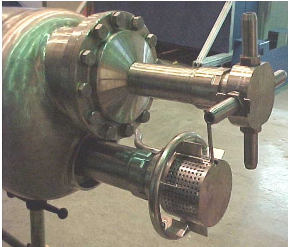
Figure 1. Bottom of Russian pulsating mixer pump pressure vessel (lying on its side), with screened intake at bottom and four discharge nozzles at upper right.
