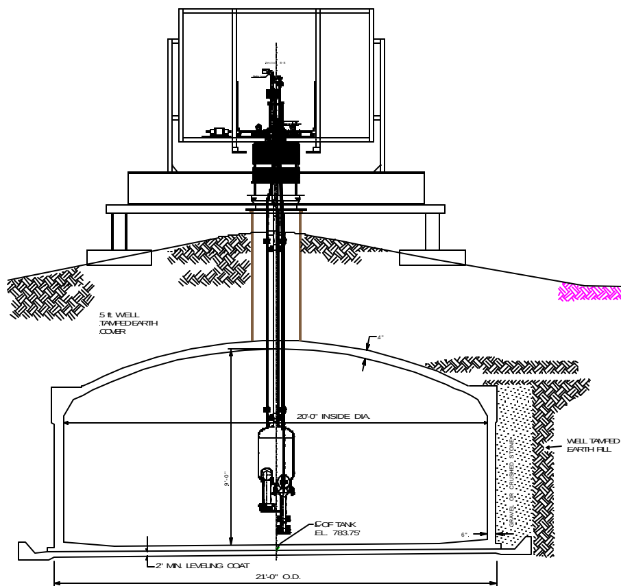
Figure 4. Mixer installation in Oak Ridge tank TH-4.
