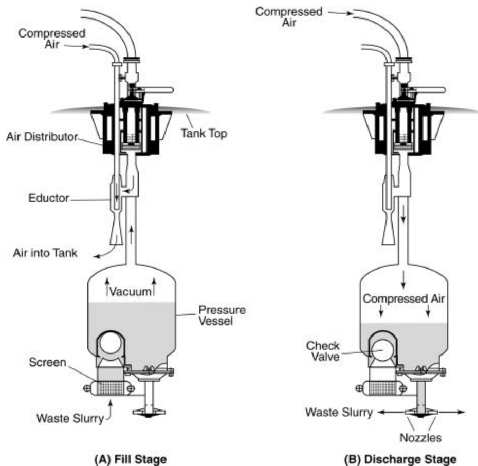
Figure 3. Material movement during alternating mixer stages.
