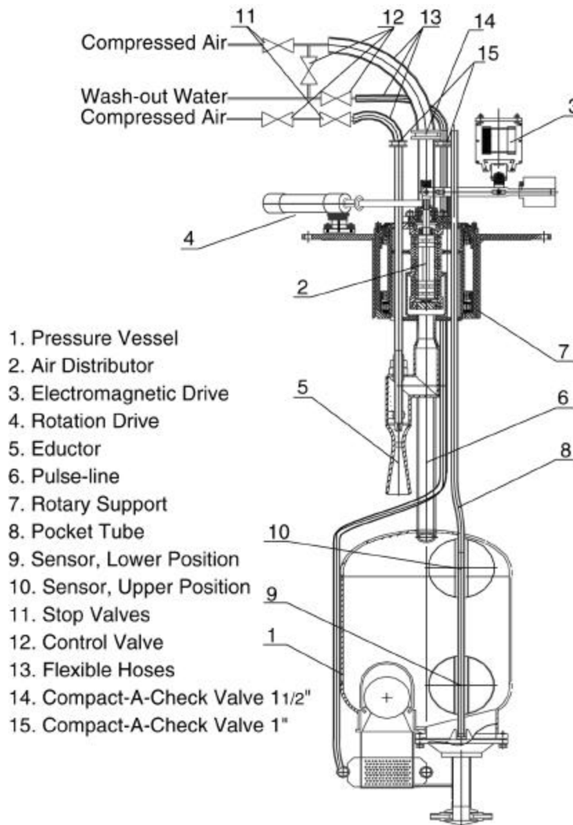
Figure 2. Russian pulsating mixer pump schematic.
