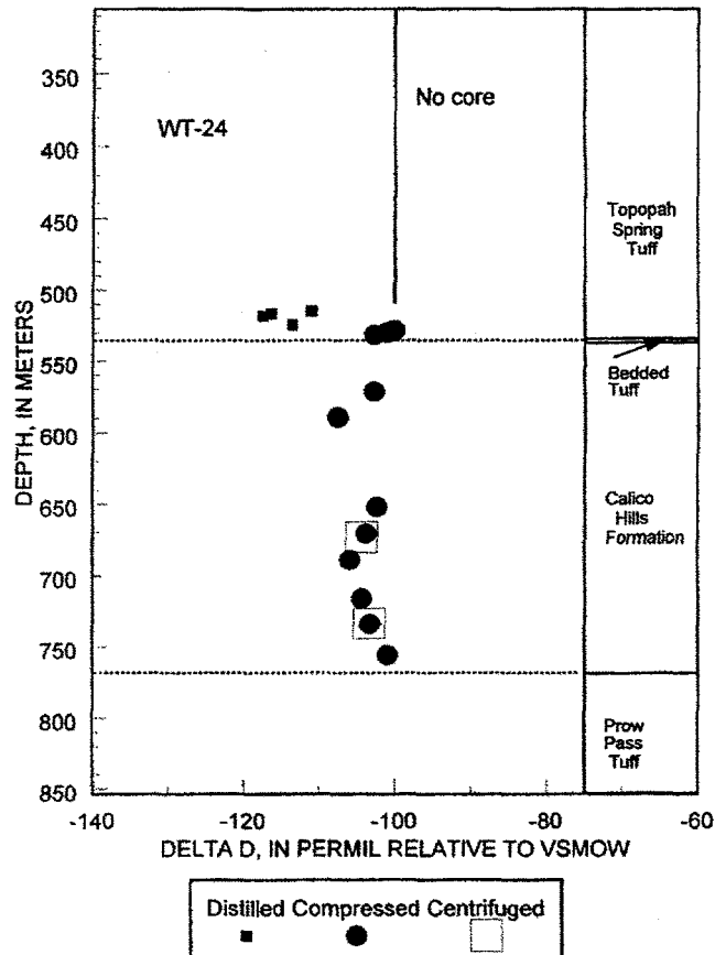
Figure 6. Delta O-18 and Delta D values of pore water from borehole WT-24. Symbol sizes are larger than 2 sigma deviations.
