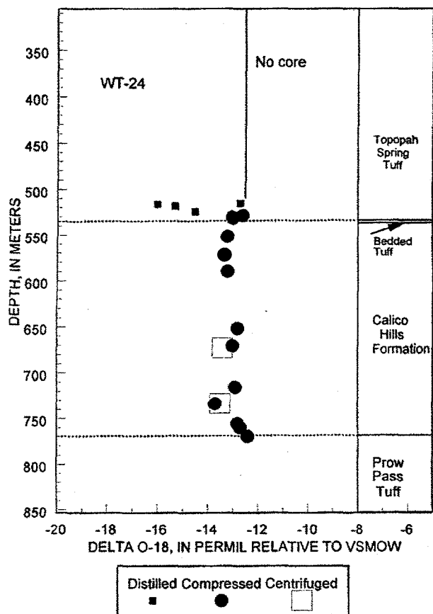
Figure 6. Delta O-18 and Delta D values of pore water from borehole WT-24. Symbol sizes are larger than 2 sigma deviations.
