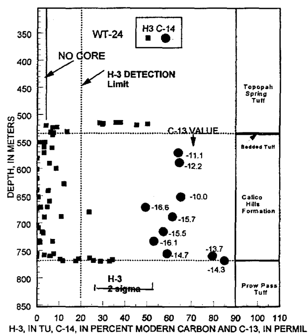
Figure 4. Tritium (H-3) and carbon-14 (C-14) concentrations of pore water in borehole USW WT-24.
