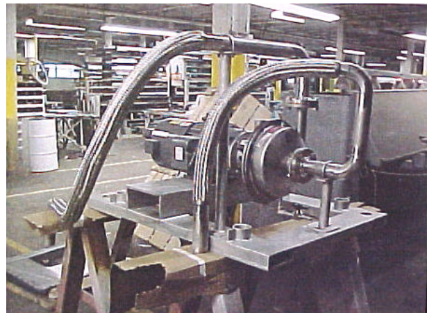
Figure 7. Booster pump assembly.
