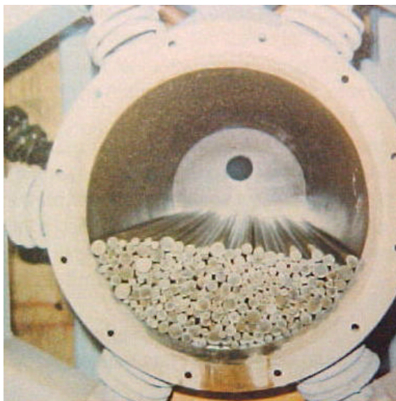
Figure 5. Grinder chamber interior with rods.
