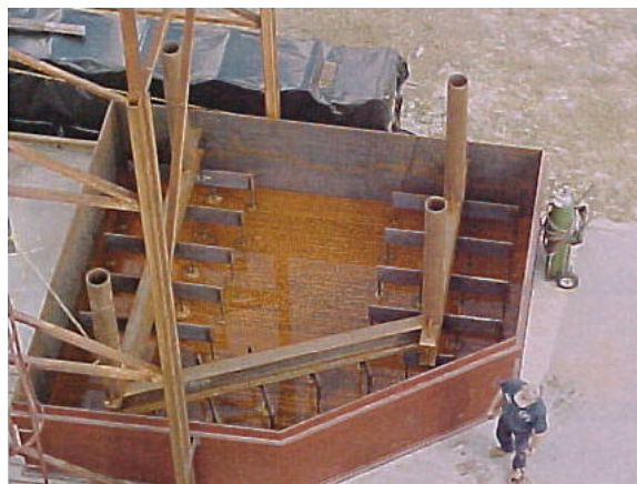
Figure 9. Aerial view of the test tank.
