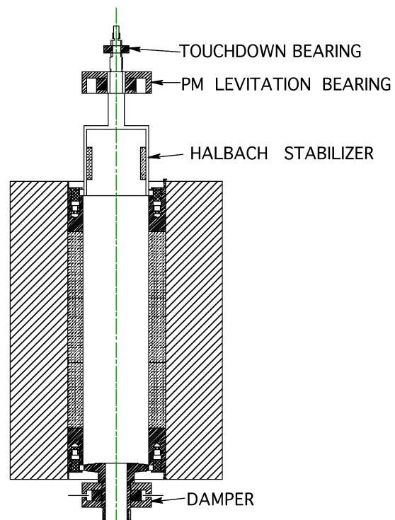
FIGURE 2: Section drawing of pendulous passive magnetic bearing system supporting the flywheel rotor
