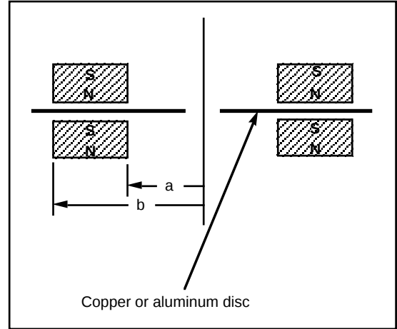
FIGURE 3: Schematic drawing of eddy-current damper
