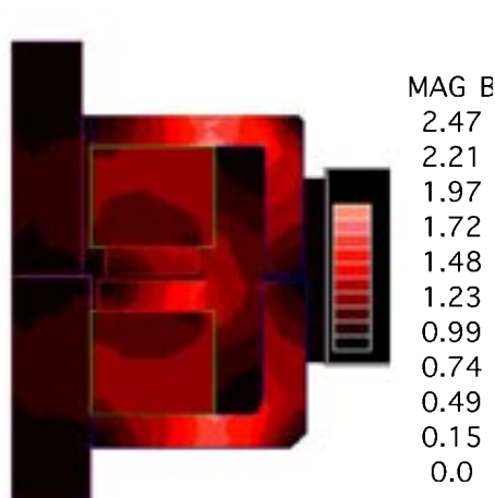
FIGURE 1: Section drawing of passive bearing element with calculated field strengths in kilogauss indicated by shading.
