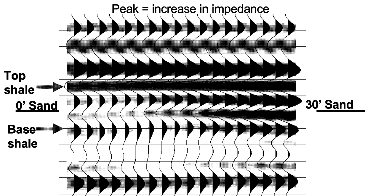
Figure 3.1.2e. PSV converted-wave seismic model response to Eva sandstone of increasing thickness (Wilson, 2002). Note the increase in amplitude from zero to 30 feet of sandstone.
