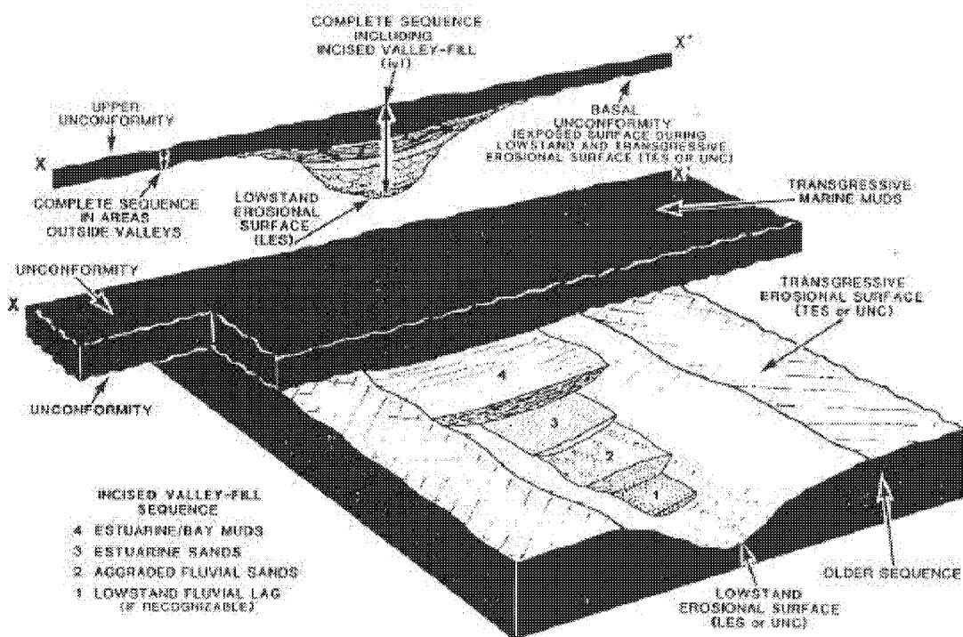
Figure 1.3a. Transgressive valley-fill model for deposition of upper Morrow reservoirs (Wheeler et al., 1990). Upper Morrow reservoirs are dominantly aggraded fluvial and estuarine sandstones (units 2 and 3).
