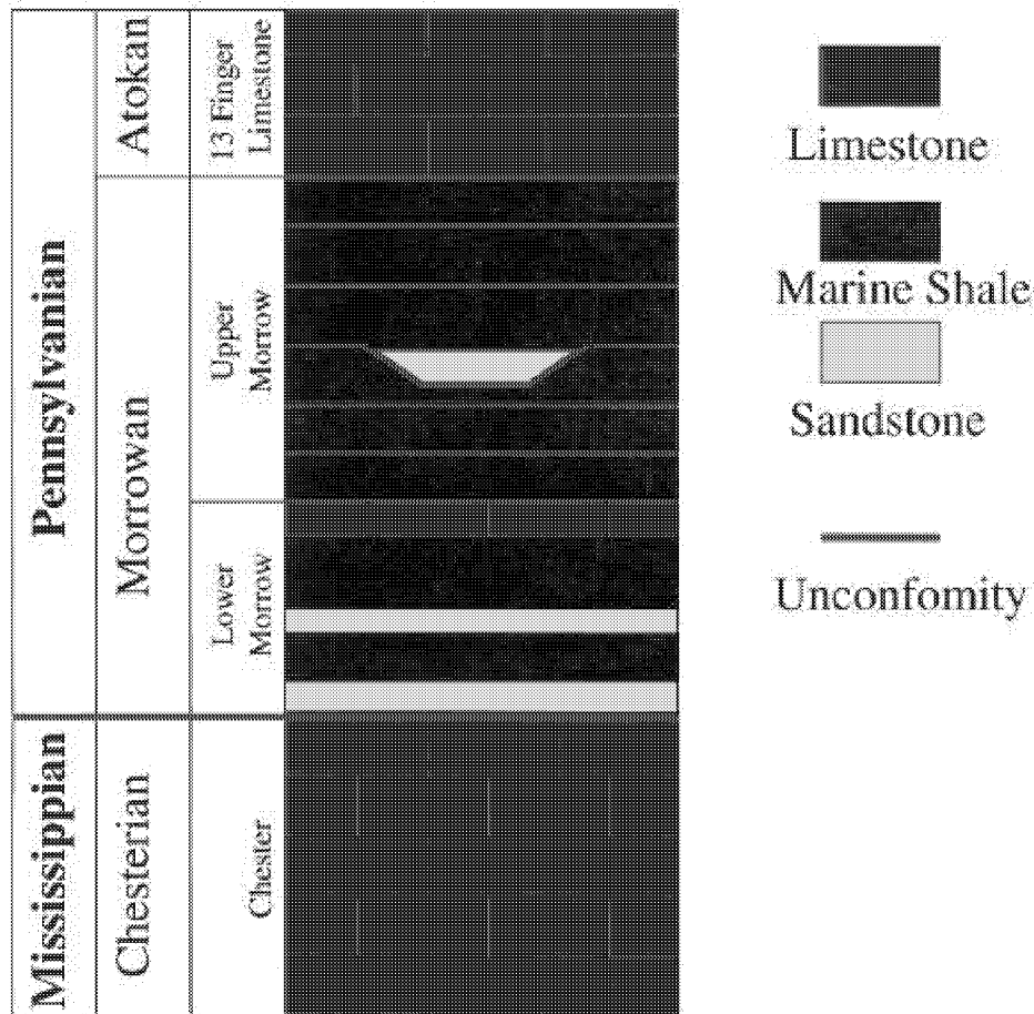
Figure 1.1b. Stratigraphic column for the area of Eva South (Wilson, 2002). The relative position of the Eva sandstone is schematically represented in the upper Morrow.
