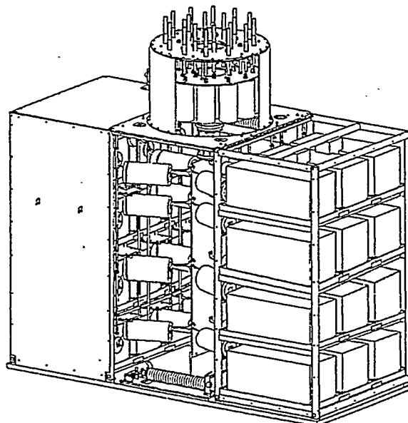
Figure 1. View of uncovered 24 capacitor PCS module.
