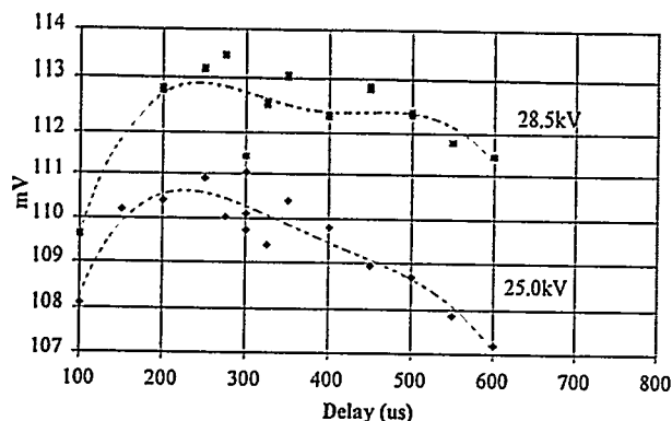
Figure 10. Fluorescence vs PILC delay for two PILC charge voltages.
