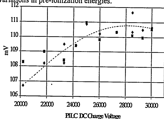
Figure 11. Fluorescence vs PILC charge voltage
