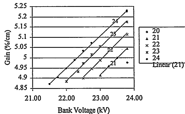
Figure 9. Gain scaling with PCS bank voltage, for a range of voltages and number of capacitors.
