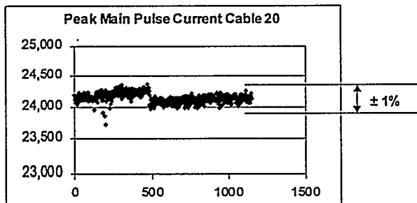
Figure 7. Pulse current reproducibility meets specifications.
