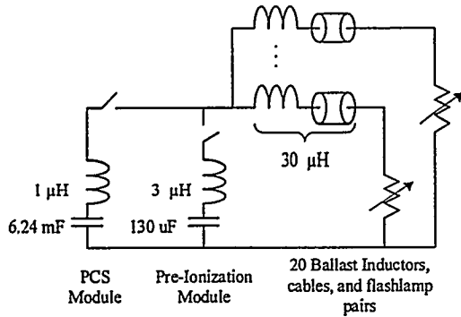
Figure 2. Simplified Circuit showing a PCS Module and PILC driving flashlamp loads, for the 20-capacitor PCS.
