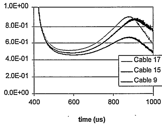
Figure 8. Variations in the resistance profiles for three lamp pairs.
