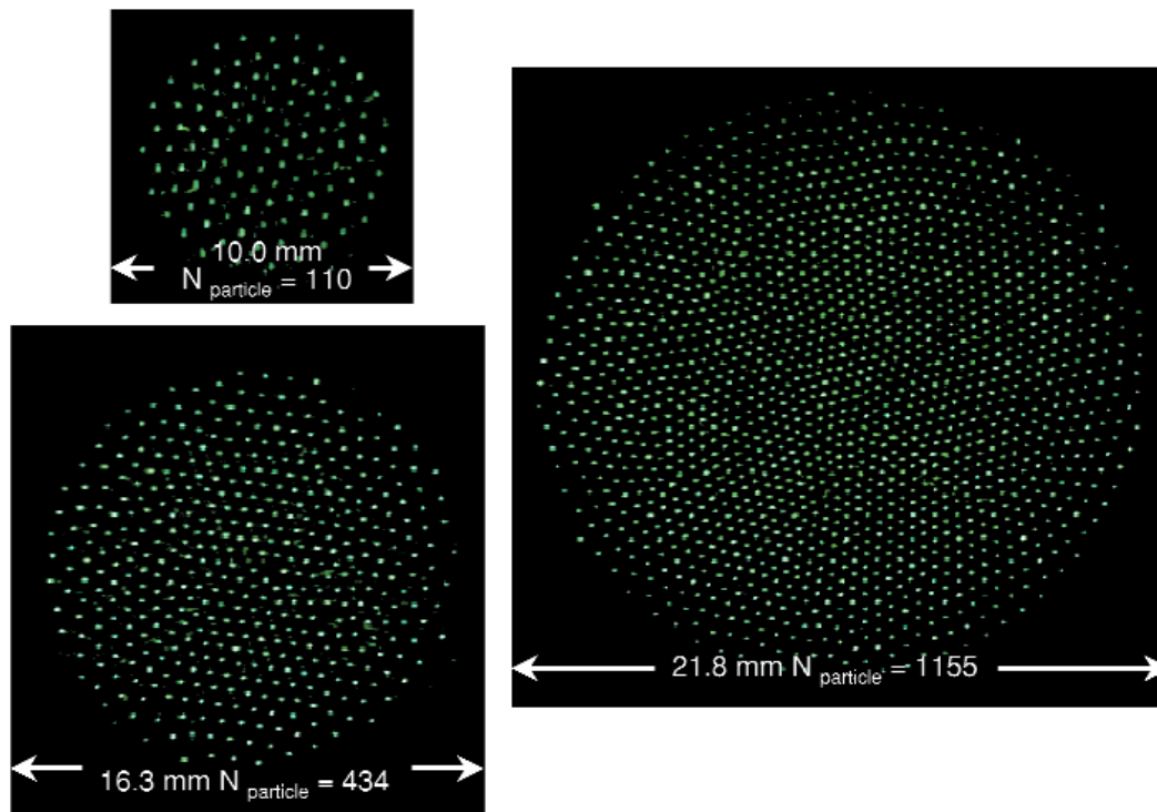
Figure 1. Top view of light scattering from plasma crystals comprised of different numbers of 8.3 \mu\text{m} diameter, melamine formaldehyde particles suspended in a 1.8 W, 110 mTorr argon plasma. The length scale is shown in each image. Horizontal confinement is provided by curvature of the lower electrode. The radial variation in nearest neighbor spacing is visible for the larger crystals.
