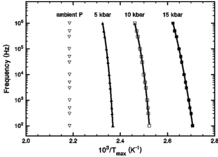
Figure 2. Frequency dispersion of T_{\max} and Vogel-Fulcher fits at 5, 10 and 15 kbar.
