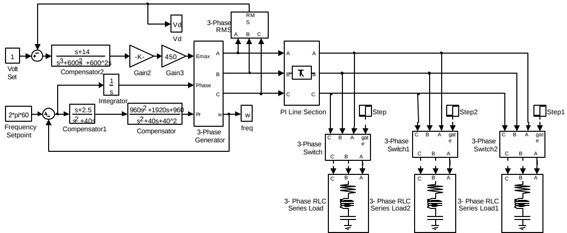
Figure 1. Three-Phase Power System Simulation Diagram with Load Disturbances. (The nominal load consists of 42 p.u. W resistance with a series inductance of 6 p.u. mH. At t=5 seconds, the resistance is instantly switched to 42 p.u. W, the inductance is switched to 12 p.u. mH, and a series capacitor of 10 p.u. F is also added. At t=10 seconds, a parallel load is instantly added with resistance of 2 p.u. W and series inductance of 3 p.u. mH. Results of this simulation are shown in Figure 2.)
