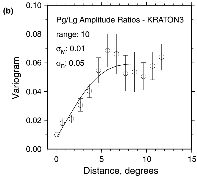
Figure 6. (a) Map of Pg/Lg ratios (0.5-5.0 Hz) for the KRATON3 PNE. Ratios are color coded according to the scale. The distance trend was removed revealing path and site effects. (b) Variogram of the Pg/Lg ratios along with our model. The model is parameterized by a range, the measurement error ( \sigma_M ) and the background error ( \sigma_B ), similar to that for the travel times.
