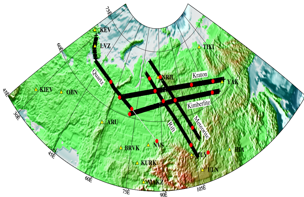
Figure 1. Soviet Peaceful Nuclear Explosion (PNE) datasets available at LLNL. Permanent three component, broadband stations in the region are also shown. The PNE shot points are shown by circles and PNE stations are shown by +. The permanent stations are shown by the triangles. The names of each PNE profile are indicated.
