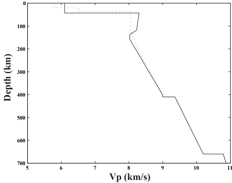
Figure 3. Best-fitting 1-dimensional model for the KRATON3 profile is shown in the solid line. The global reference model, AK135, is shown in the dotted line. The crust and the uppermost mantle are significantly faster for KRATON3 compared to the global average. We also find evidence for a significant low-velocity zone below the mantle lid at depths between 150 - 200 km. Note the negative velocity gradient in the mantle lid.
