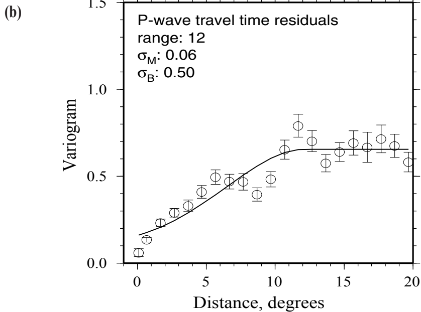
Figure 4. Spatial variation of travel-time residuals for the best-fitting 1-D model for KRATON3 (Model_2 as described in text). (a) Map of residuals plotted at station locations on top of topography. Removal of the travel-time predictions of the best-fitting model largely reduces the distance trend revealing path and site effects. We observe faster (negative) residuals for the Eastern stations. (b) Variogram of the travel-time residuals along with our model. The model is parameterized by a range, the measurement error ( \sigma_M ) and the background error ( \sigma_B ). The range gives us an estimate of the correlation length for the region. The low background variance suggests that the fit to the data is excellent. The low measurement error indicates the robustness of the travel-time picks.
