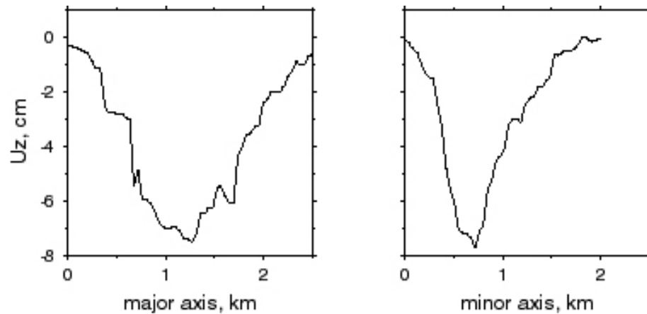
Figure 2: Vertical displacement cross sections (unwrapped phase) along the major and minor axes of the interferogram in Figure 1
