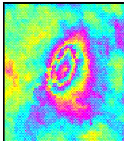
Figure 1: 4/24/92-6/18/93 interferogram imaging ground deformation associated with the JUNCTION event.
