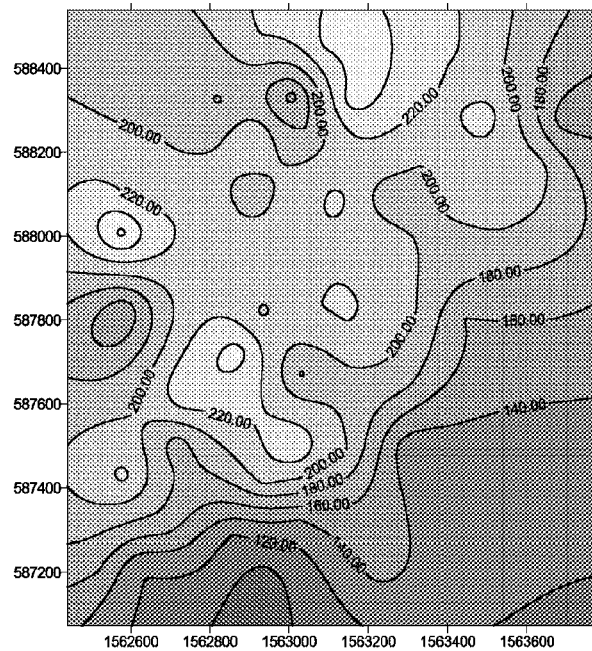
Figure 6-13: Contoured flow line temperatures ( ^{\circ} F) for individual producers averaged for the first three quarters of 2000. The highest temperatures are associated with the pilot, which has been in steam flood since early 1997, but oil rates are high, and the two oil depleted regions in the north and northwest, where oil rates are very low.
