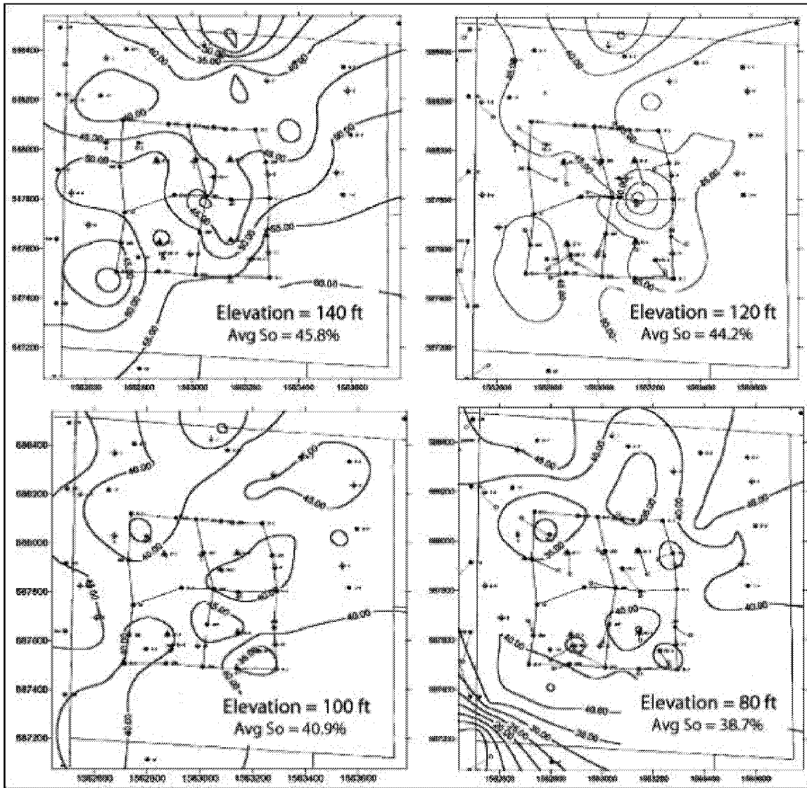
Figure 3-39: Maps showing the distribution of oil within the Monarch Sand reservoir at 140 ft to 80 ft elevations. The values contoured are the 20-ft moving average of S_o -arco at the elevation of the map. The maps depict the lateral variability in oil saturation within a 20 ft thick interval of the reservoir 10 ft above to 10 ft below the map datum.
