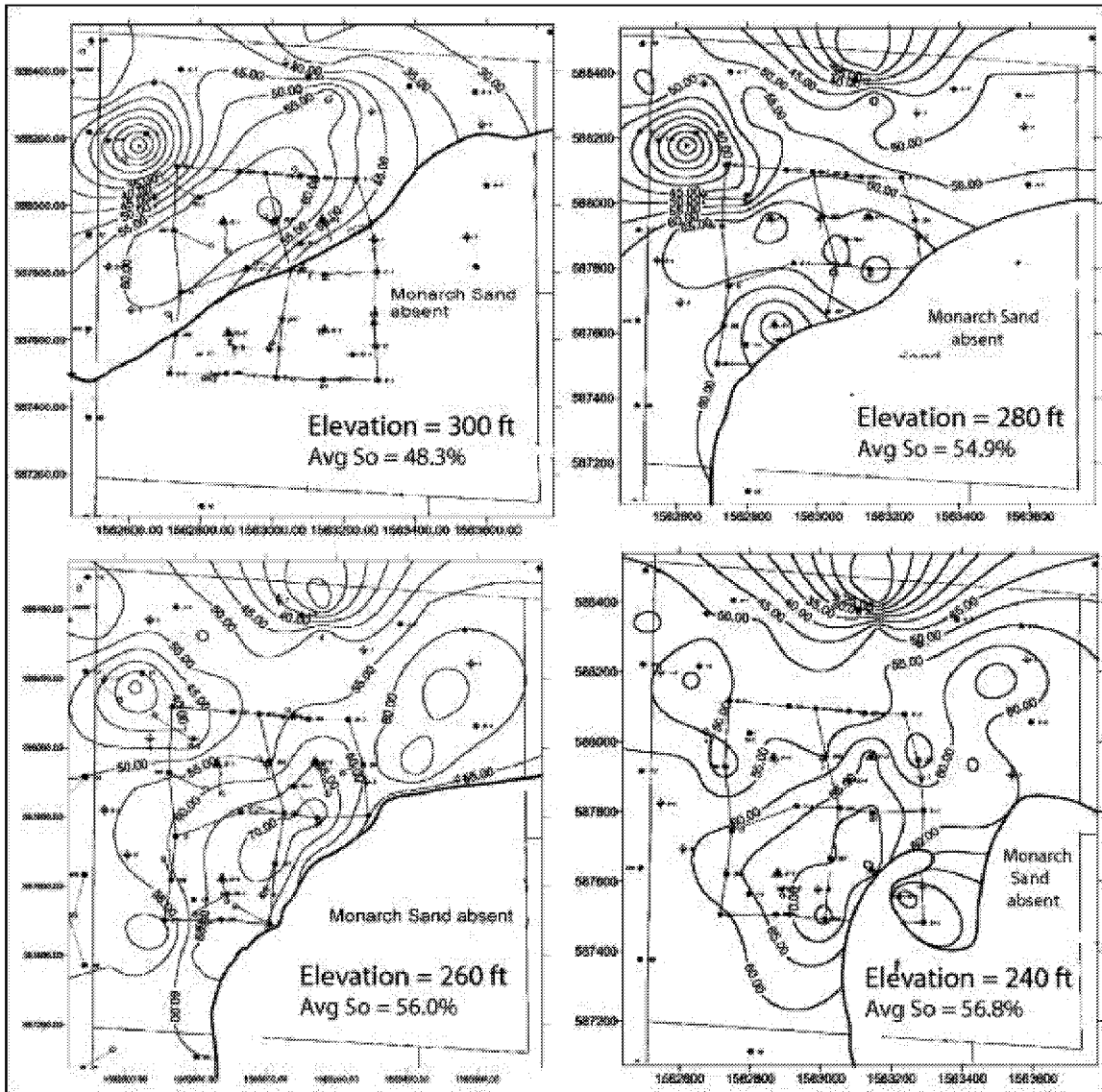
Figure 3-37: Maps showing the distribution of oil within the Monarch Sand reservoir at different elevation slices. The values contoured are the 20-ft moving average of So-arc0 at the elevation of the map. The maps depict the lateral variability in oil saturation within a 20 ft thick interval of the reservoir 10 ft above to 10 ft below the map datum.
