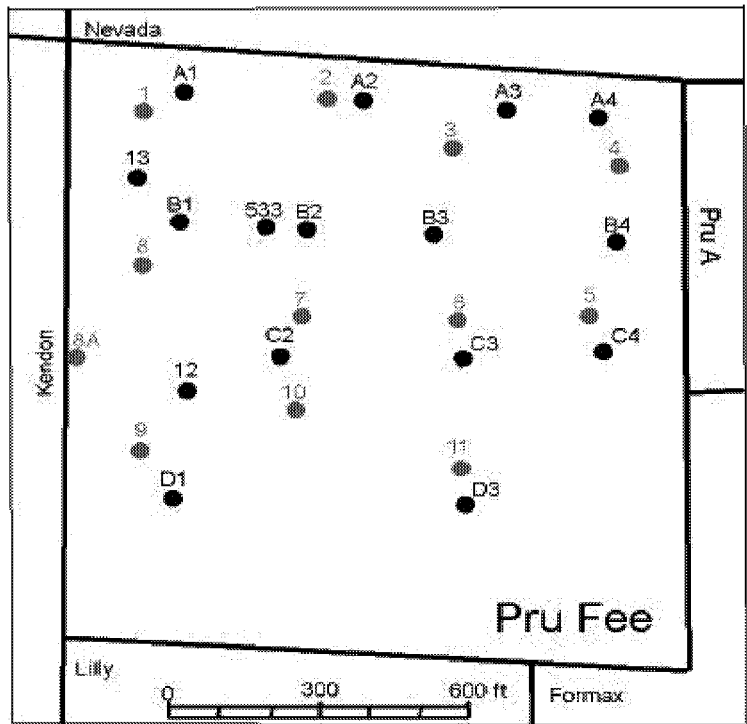
Figure 2-6: Map showing the thermal recovery wells operating during the period 1966-1986. Most of the wells were put on-line between late 1970 and early 1972. The shaded wells are the original primary producers shut-in between December 1969 and April 1970.
