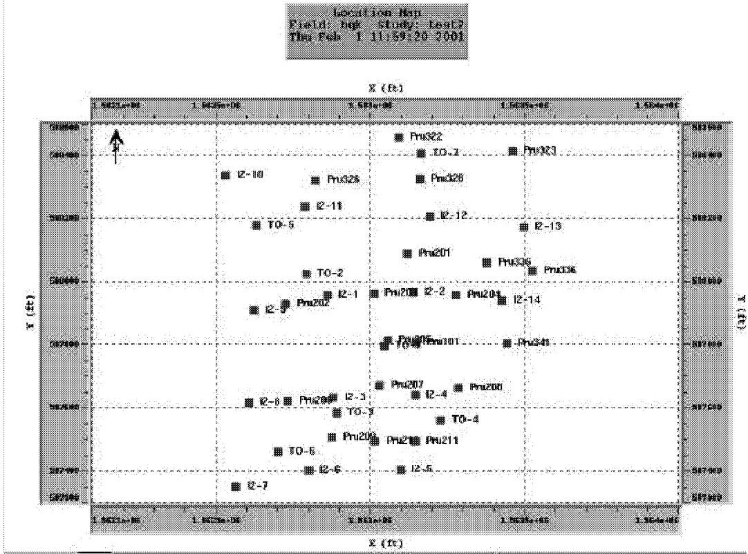
Figure 5-1: Heresim3D base map of the Pru Fee property showing top-reservoir locations of the wells used in geostatistical modeling of the Monarch Sand reservoir.
