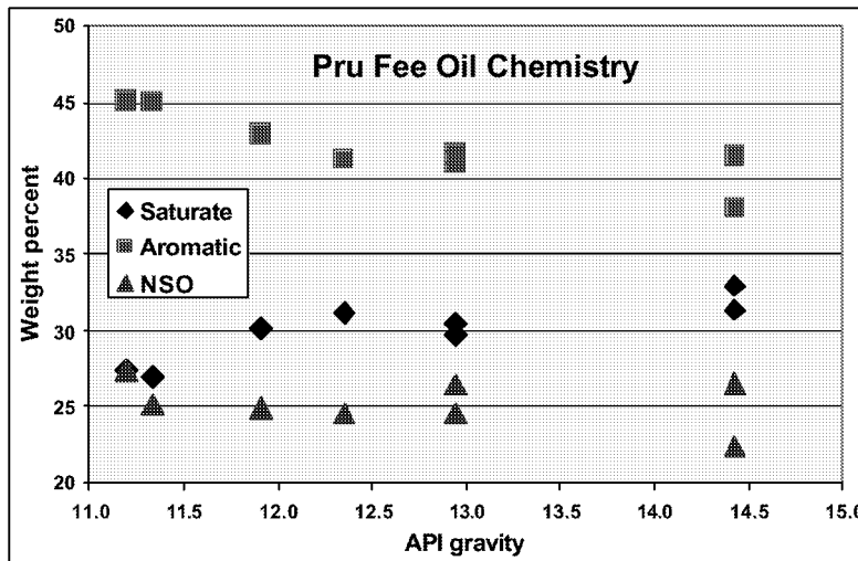
Figure 3-22: Variations in oil composition with API gravity. The heavier oils have higher aromatic fractions and relatively low saturate fractions. The NSO fraction does not vary with oil gravity.
