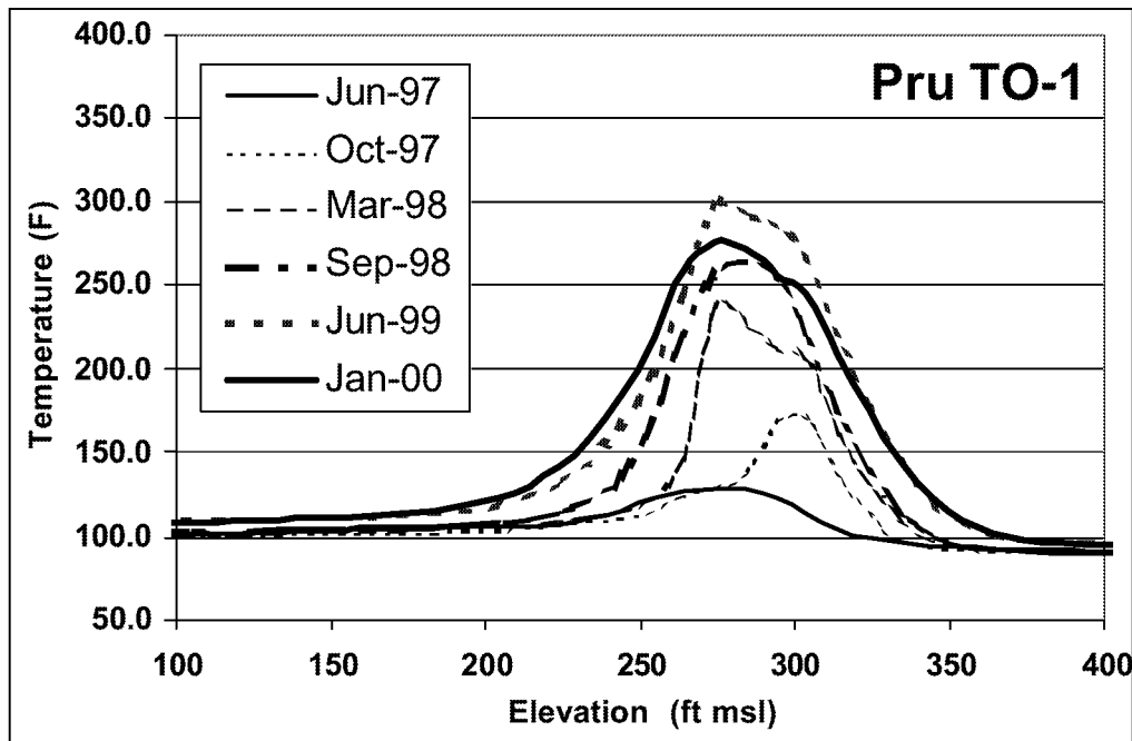
Figure 4-5: Stacked temperature logs for the Pru TO-1 well, which is 100 ft from the nearest injector well. Top of Monarch Sand = 300 ft; OWC = 30.5 ft.
