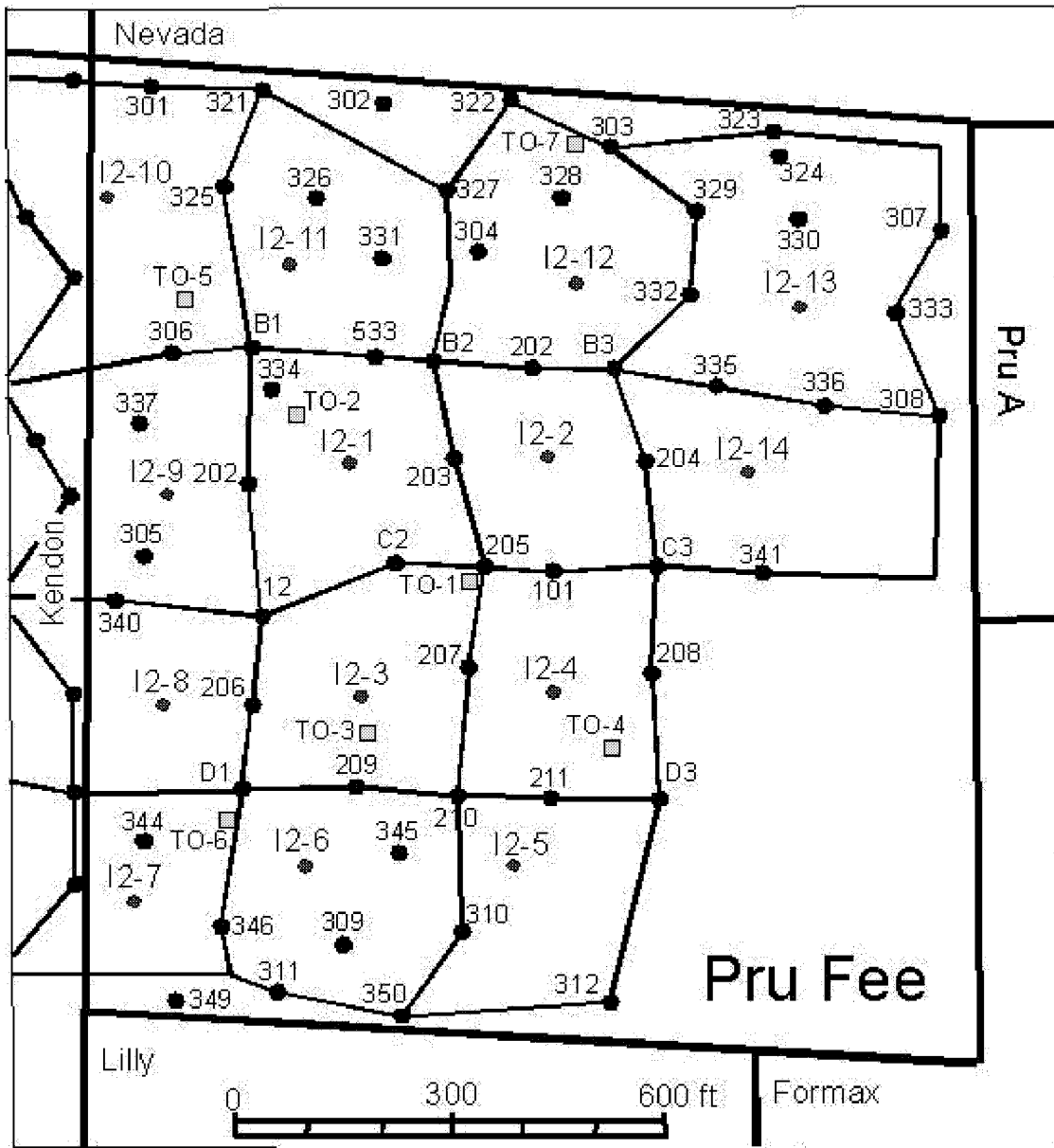
Figure 2-1: Location of the temperature observation wells on the Pru Fee property.
