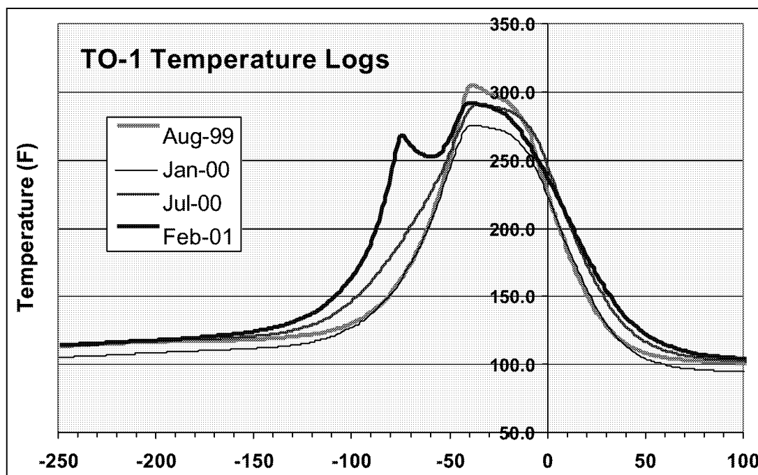
Figure 4-10: Temperature logs for the TO-1 well near the center of the Pru Fee property. At this location the "middle barrier" unit is 76 to 88 ft below the top of the Monarch Sand, which serves as the datum in this and the following log plots.
