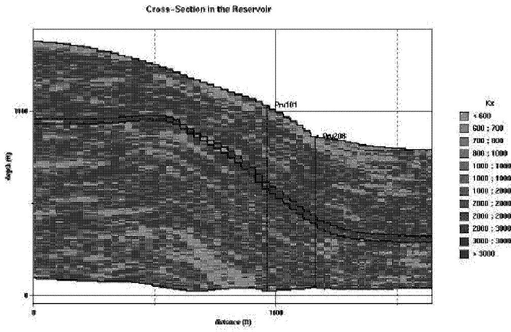
Figure 5-15: Permeability distribution in the NW-SE cross section of the entire reservoir (all lithounits).
