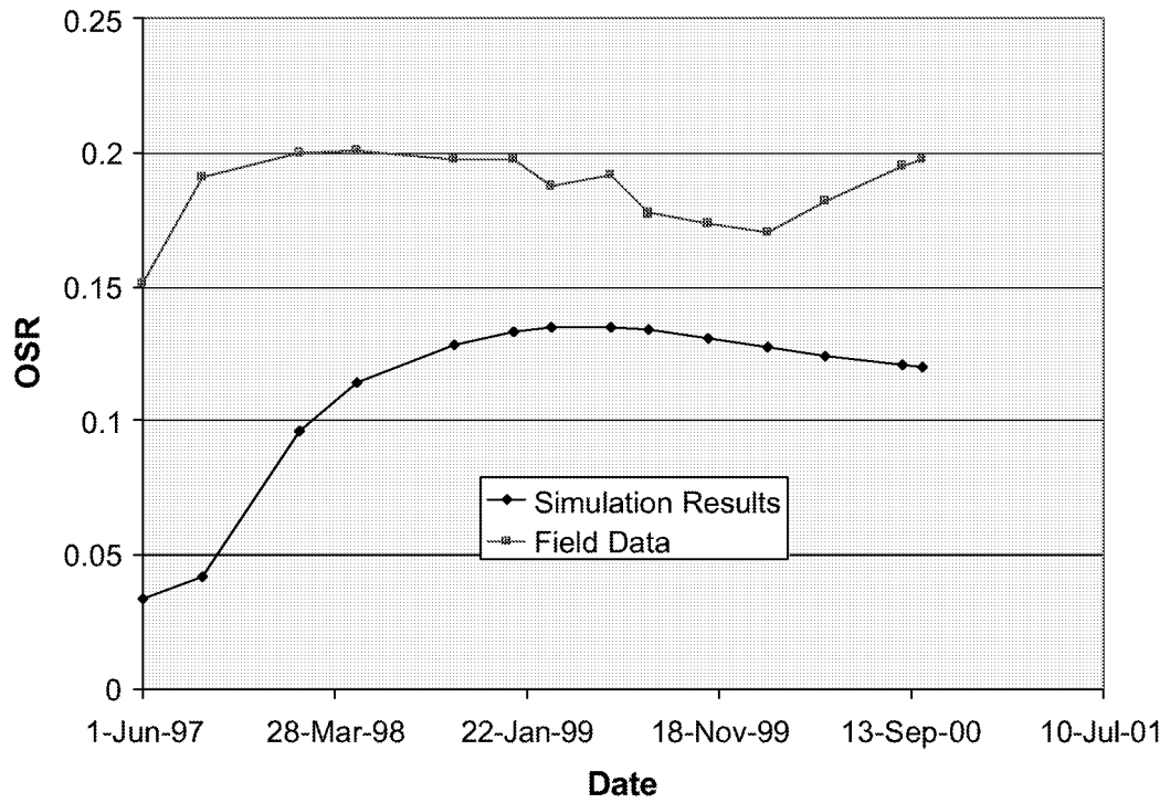
Figure 5-25: Comparison of the oil-steam ratios (OSR) predicted by the simulations to actual field data.
