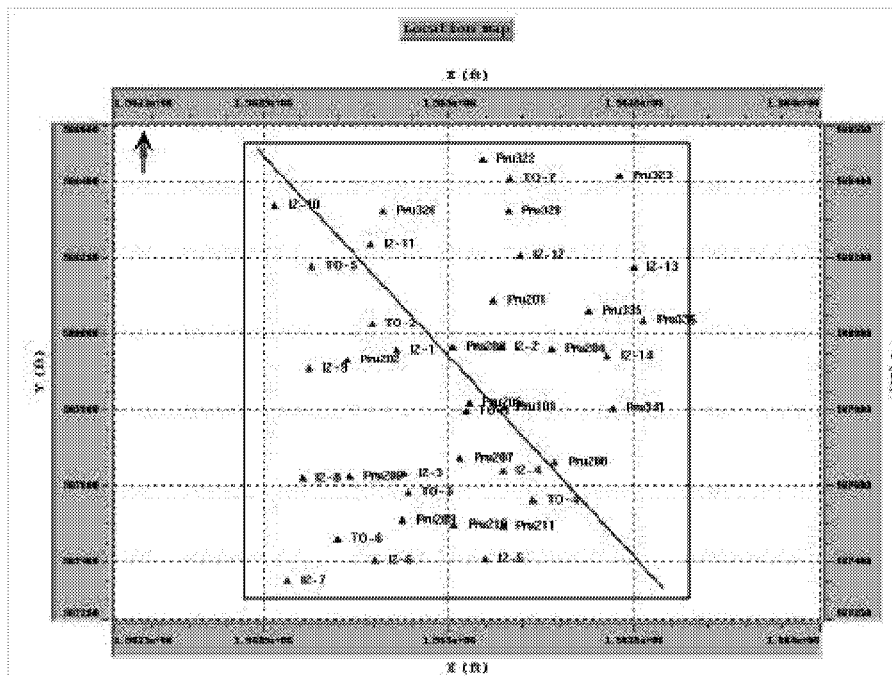
Figure 5-4: Location of the northwest-southeast model cross section through the Monarch Sand reservoir at the Pru Fee property.
