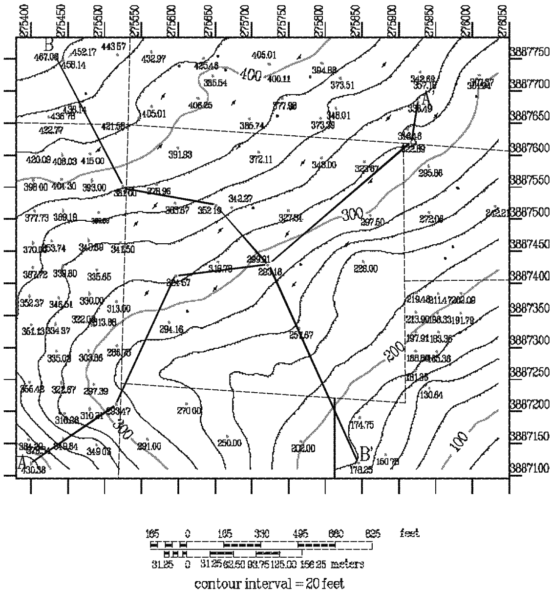
Figure 1-5: Structure of the top of the Monarch Sand reservoir at Pru Fee showing the very low dip, about 10° SE, which is seen as a major impediment to gravity drainage of heated oil towards producers. This is the mechanism responsible for success in the high-dip portions of the Kendon lease southwest of Pru Fee.
