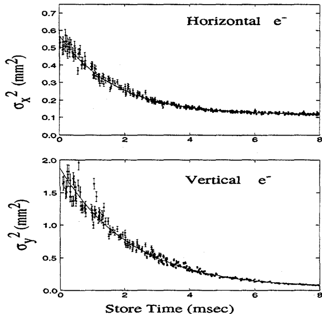
Figure 1. Sample of data for the electron damping ring. The vertical scale represents the size of the bunch image on the photocathode. The bunch itself is 2.5 times smaller
