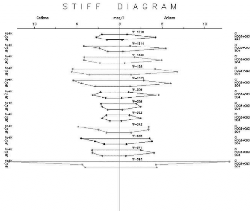
Figure 3. Output of the “Stiff” tool.
