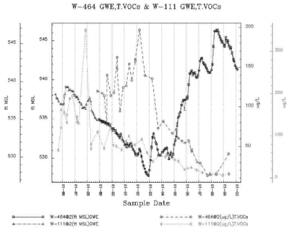
Figure 4. Output of the “Multiple Well/Multiple Parameter Time Series Plot” tool.
