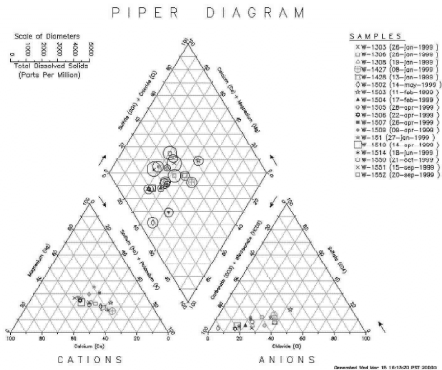
Figure 2. Output of the “Piper” tool.
