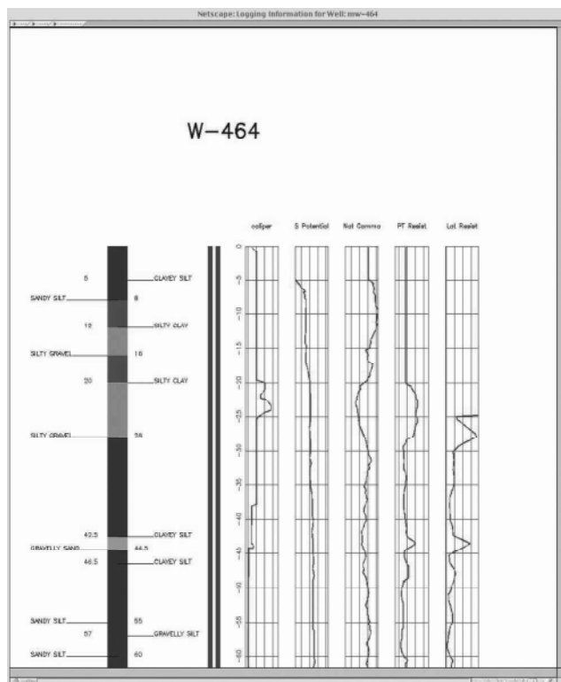
Figure 1. Output of the “Geophysical Curves Display” tool.
