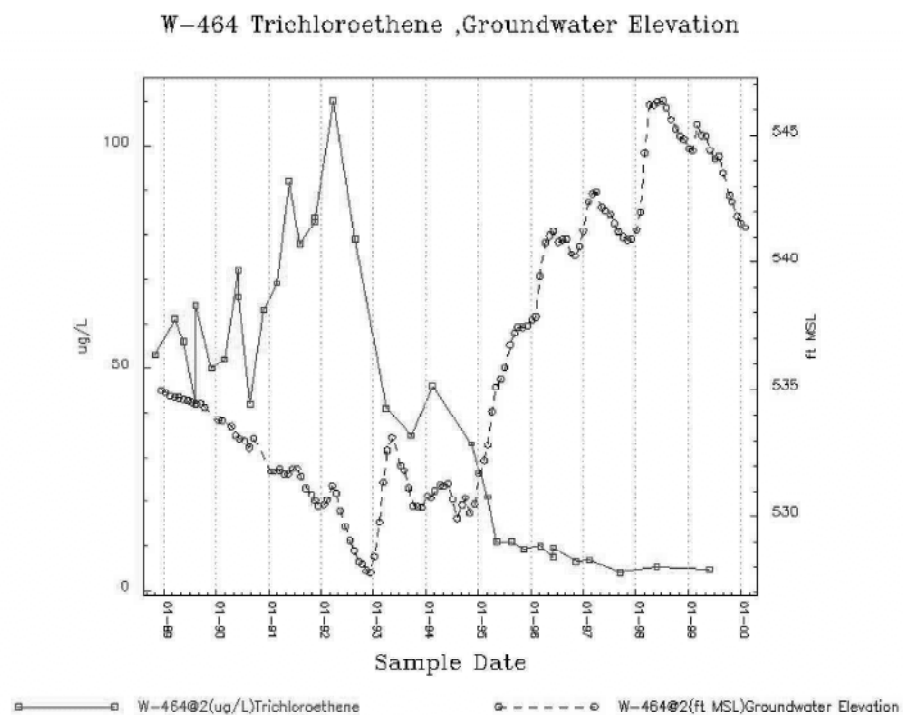
Figure 8. Output of the "Multiple Well/Multiple Parameter Time Series Plot" tool for TCE at W-464.
