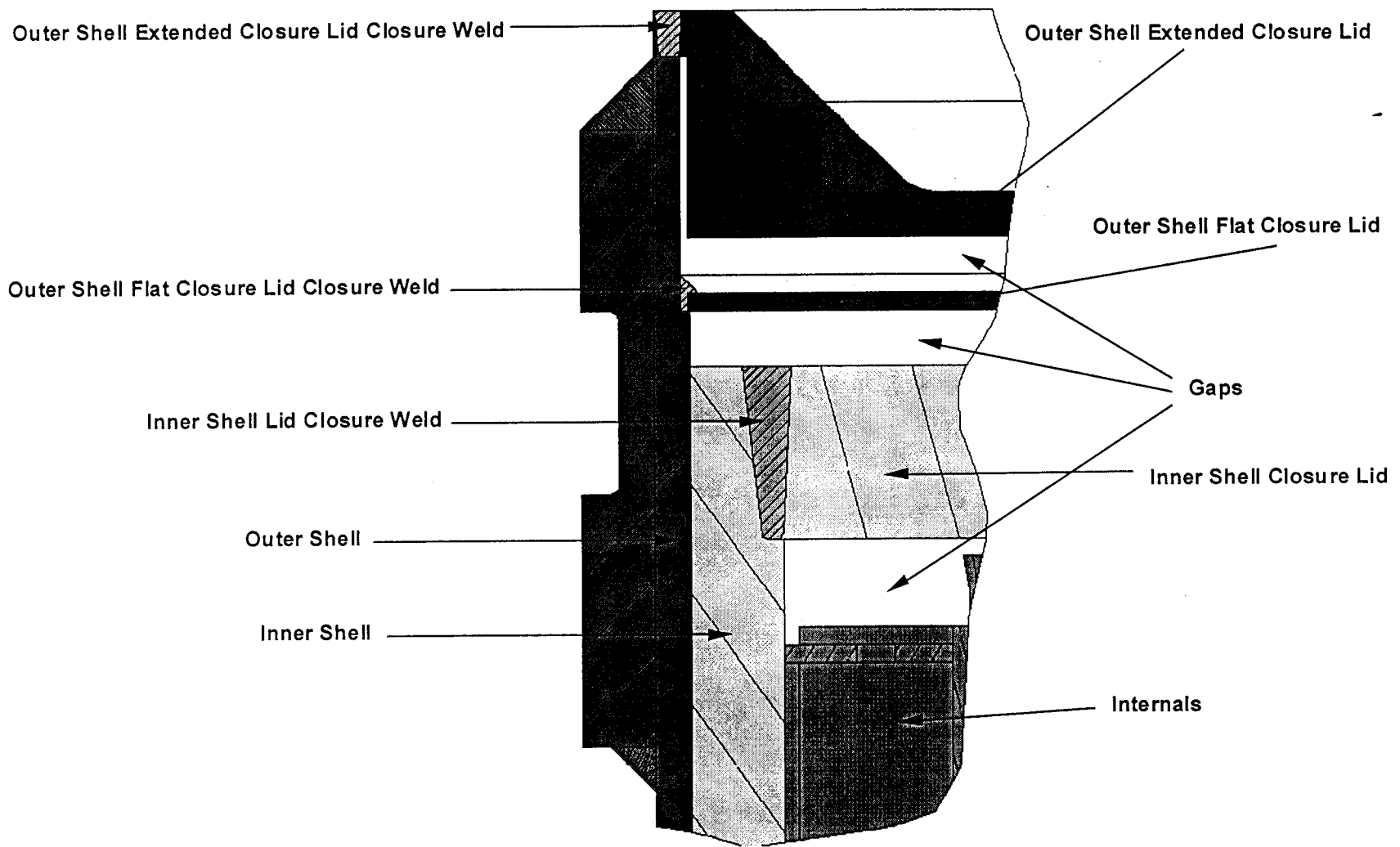
Figure 2. Closure Welds Configuration
