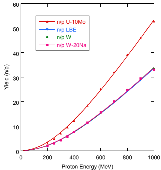
Figure 3 Number of spallation neutrons per proton as a function of proton beam energy.
