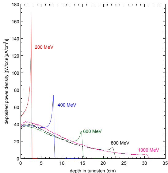
Figure 2 Profiles of deposited power density as a function of depth in a tungsten spallation target for proton beam of various energies.
