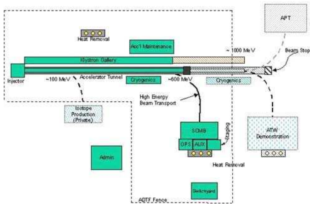
Figure 1 A schematic layout of the Accelerator Demonstration Test Facility.
