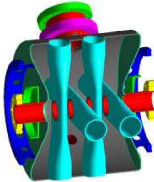
Figure 4 Engineering model of a \beta=0.125 , 5-gap spoke cavity at 350 MHz
